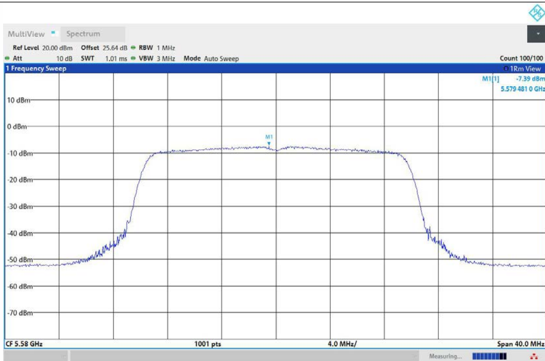
11AX20MIMO-Ant3-5580-PASS
