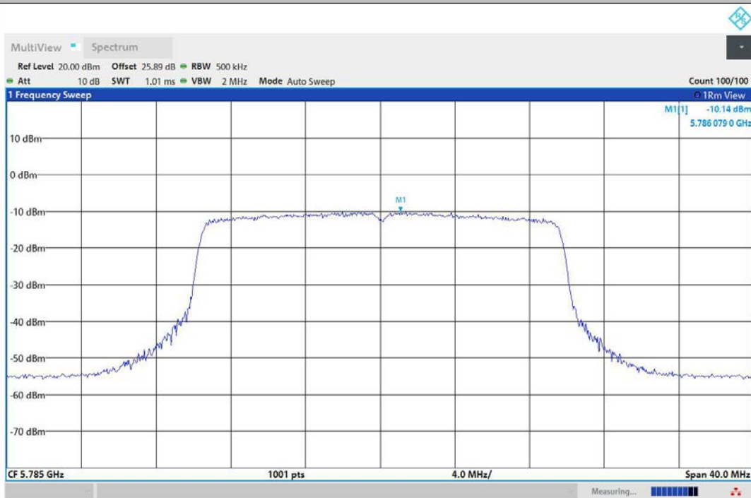
11AX20MIMO-Ant3-5785-PASS
