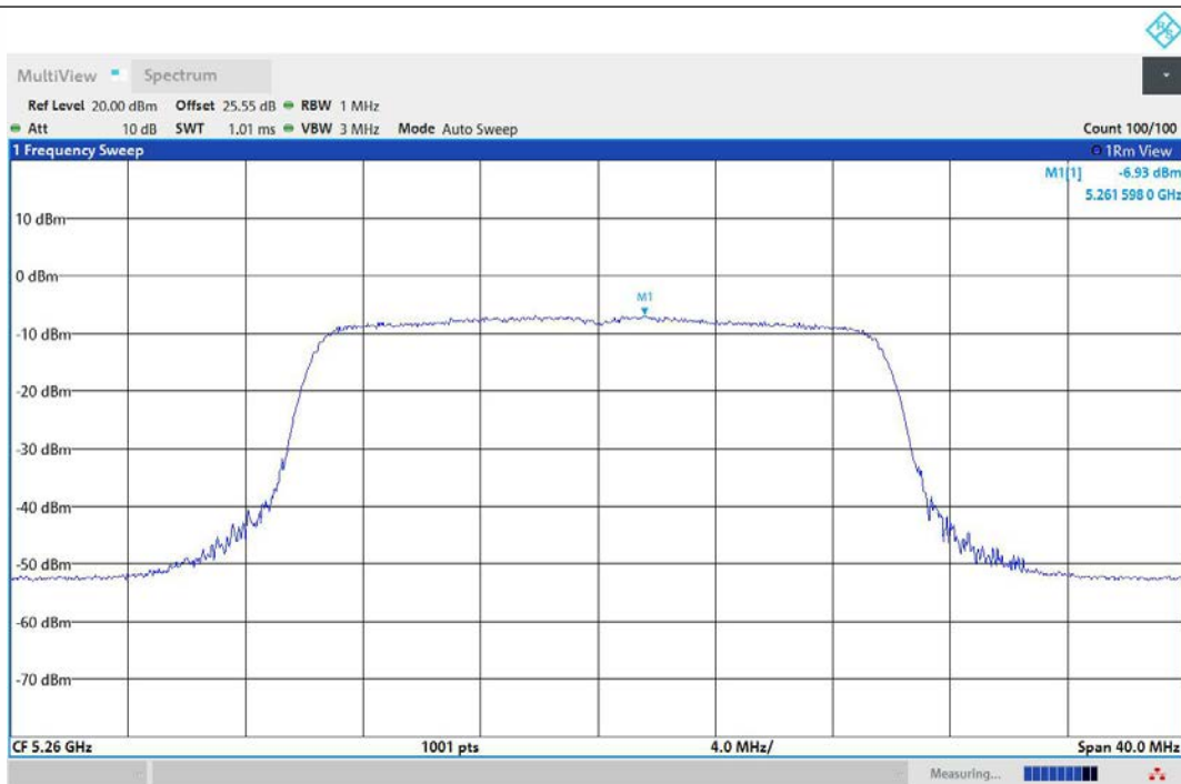
11AX20MIMO-Ant3-5260-PASS
