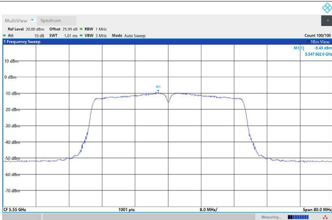
11AC40MIMO-Ant3-5550-PASS
