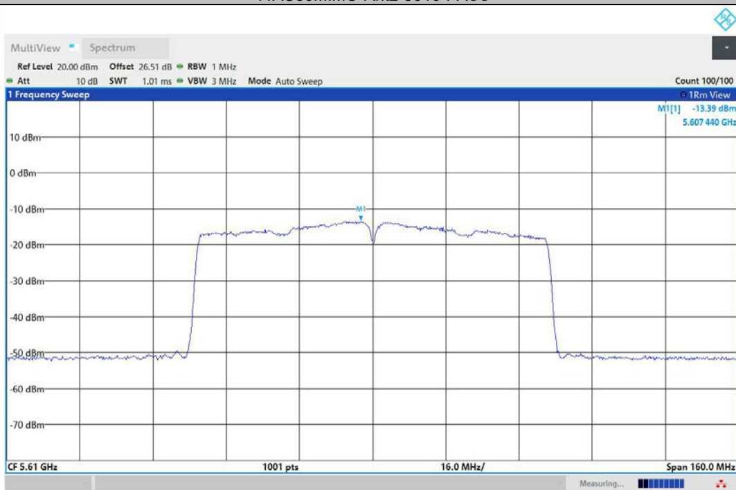
11AC80MIMO-Ant3-5610-PASS
