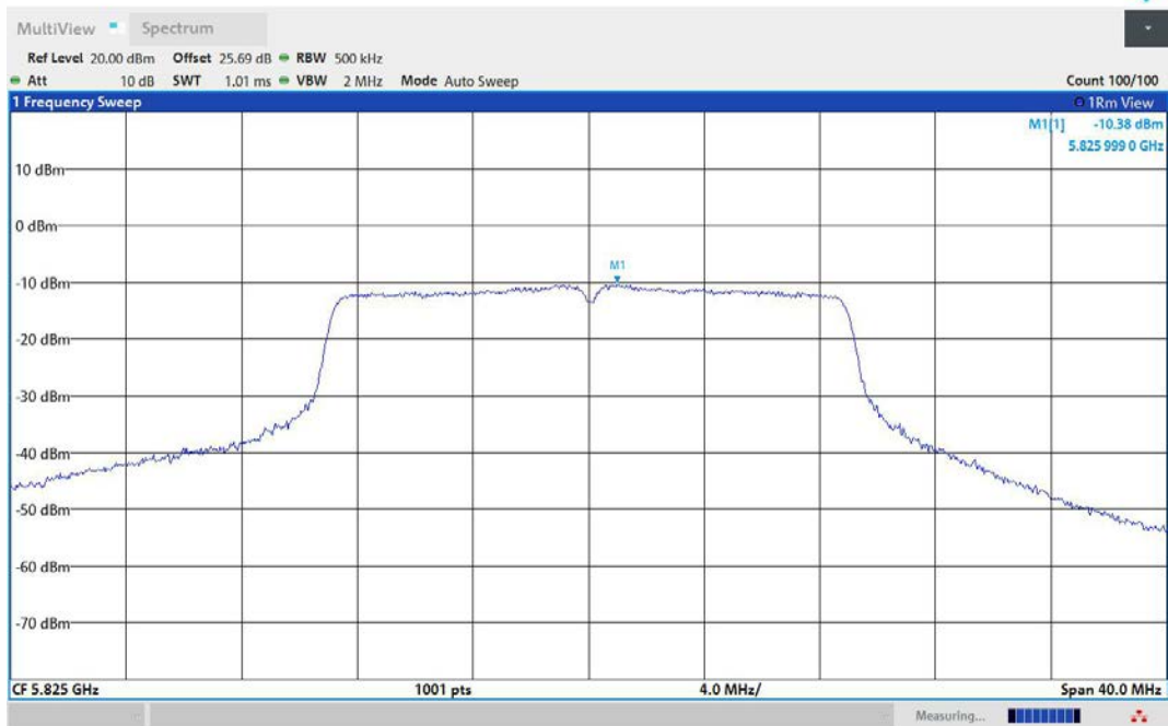
11AC20MIMO-Ant3-5825-PASS
