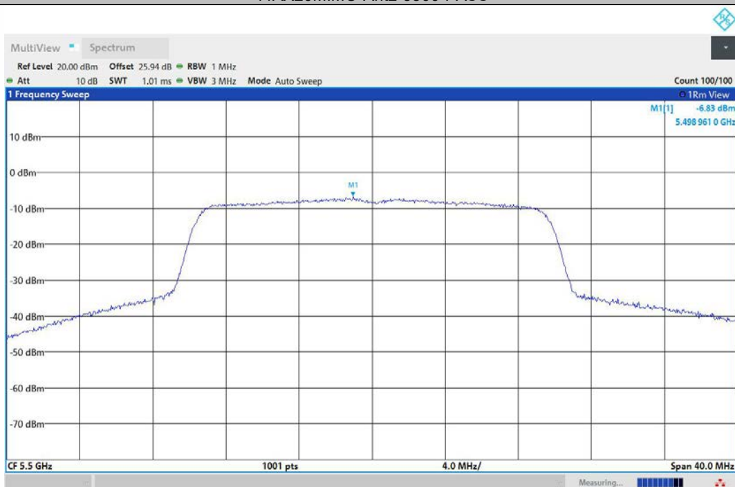
11AX20MIMO-Ant3-5500-PASS
