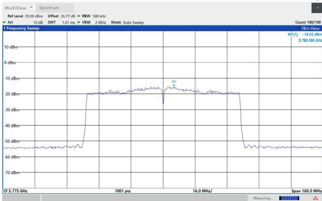
11AC80MIMO-Ant3-5775-PASS
