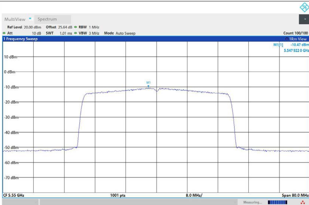
11AX40MIMO-Ant1-5550-PASS
