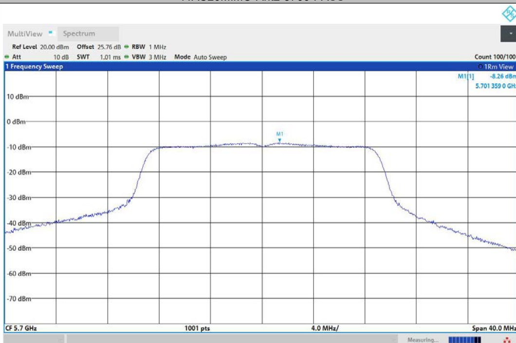
11AC20MIMO-Ant3-5700-PASS
