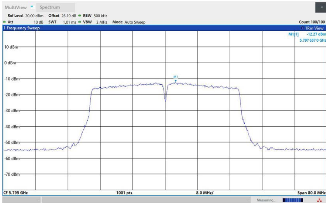
11AC40MIMO-Ant3-5795-PASS
