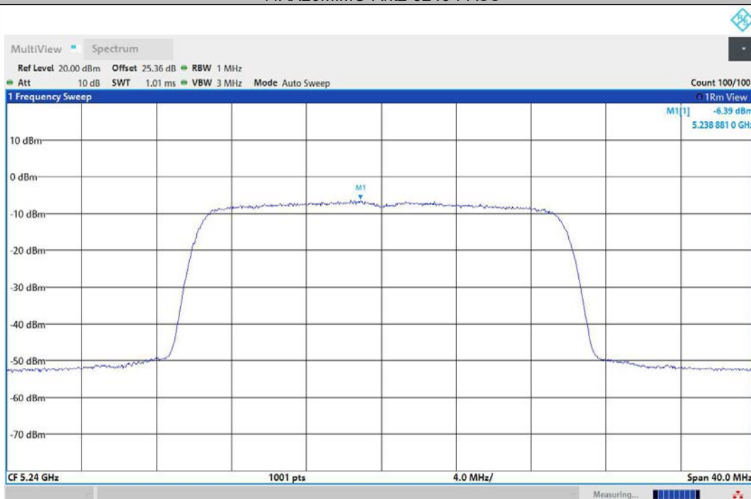
11AX20MIMO-Ant3-5240-PASS
