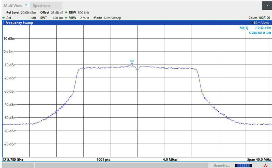
11AC20MIMO-Ant1-5785-PASS
