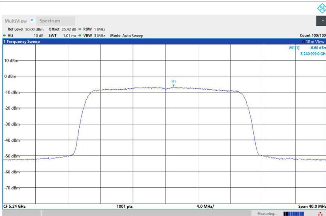
11AX20MIMO-Ant2-5240-PASS
