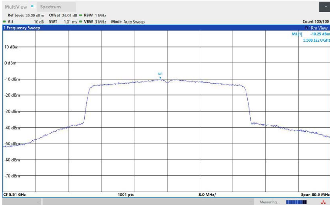
11AX40MIMO-Ant1-5510-PASS
