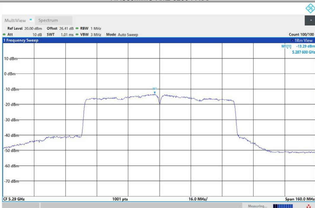
11AC80MIMO-Ant3-5290-PASS
