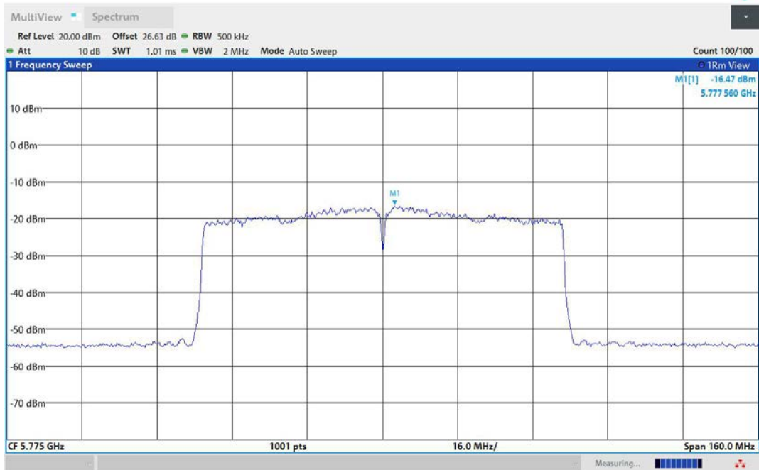
11AC80MIMO-Ant2-5775-PASS
