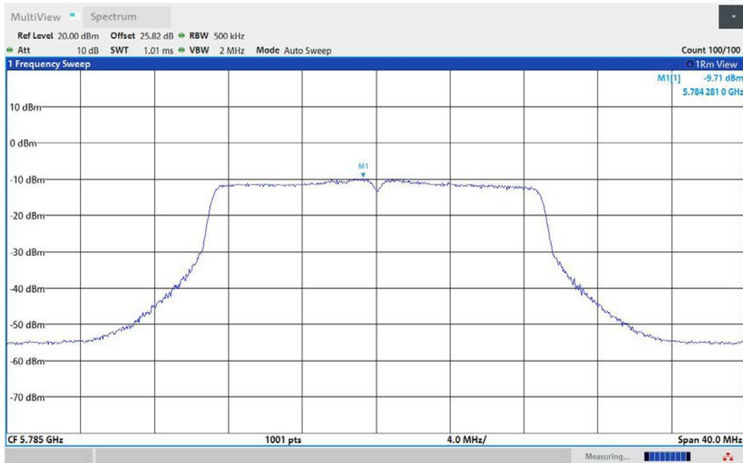
11AC20MIMO-Ant3-5785-PASS
