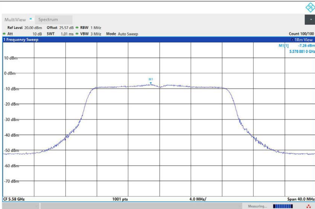
11AC20MIMO-Ant3-5580-PASS
