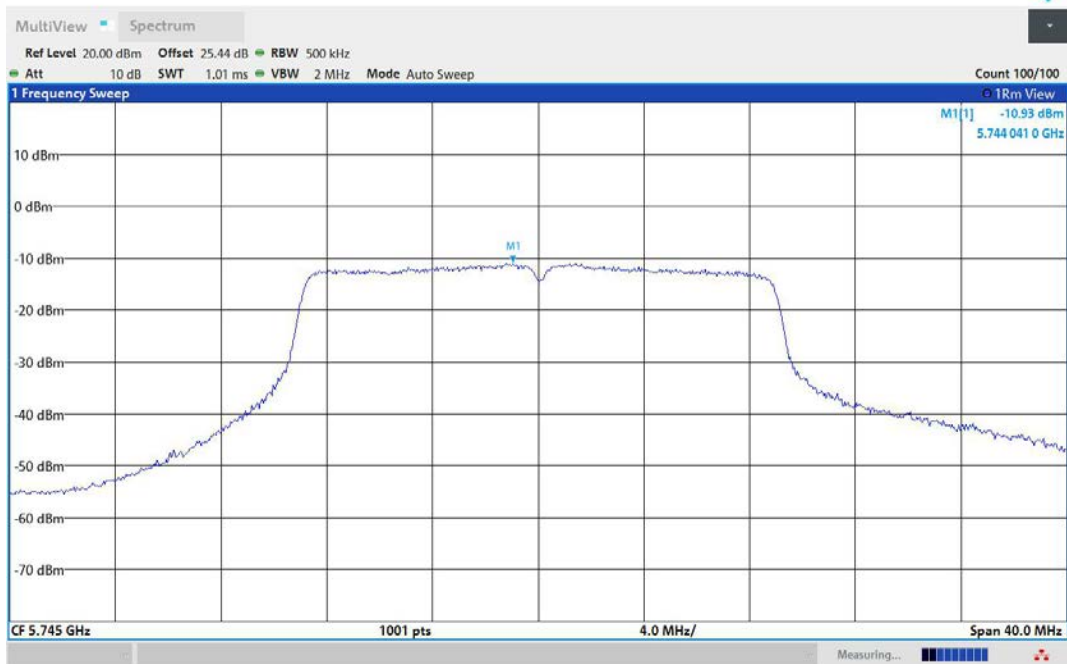
11AC20MIMO-Ant3-5745-PASS
