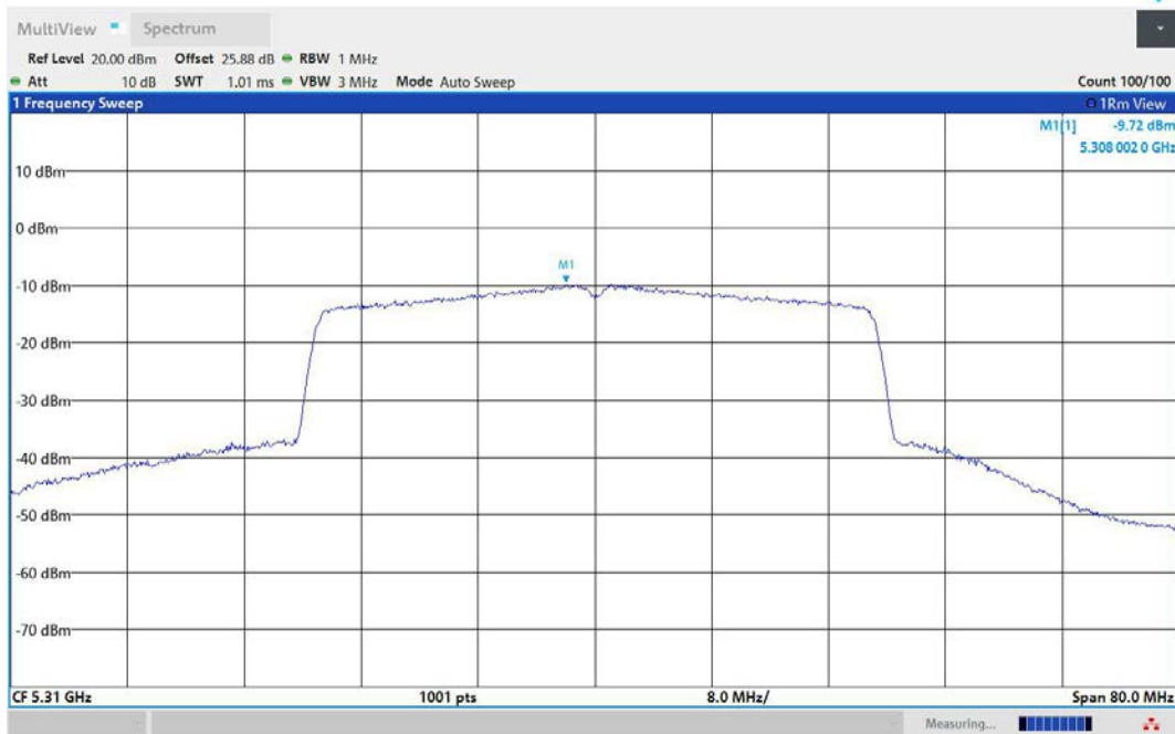
11AX40MIMO-Ant3-5310-PASS
