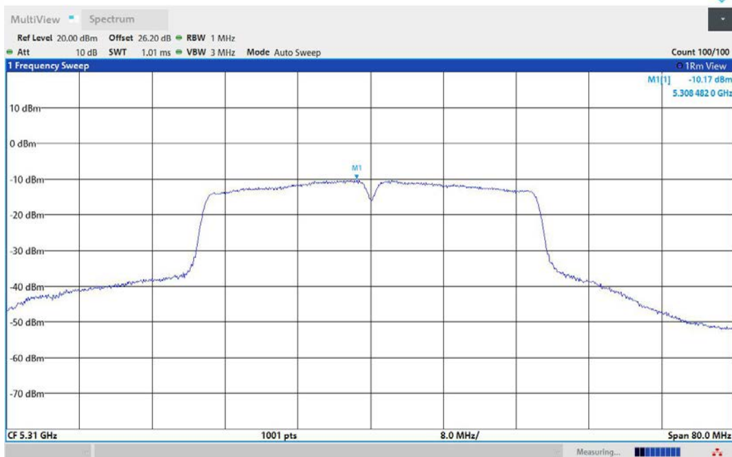
11AC40MIMO-Ant3-5310-PASS
