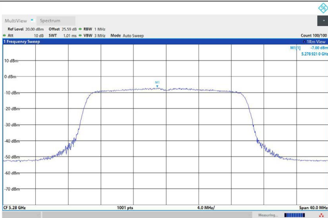
11AX20MIMO-Ant3-5280-PASS
