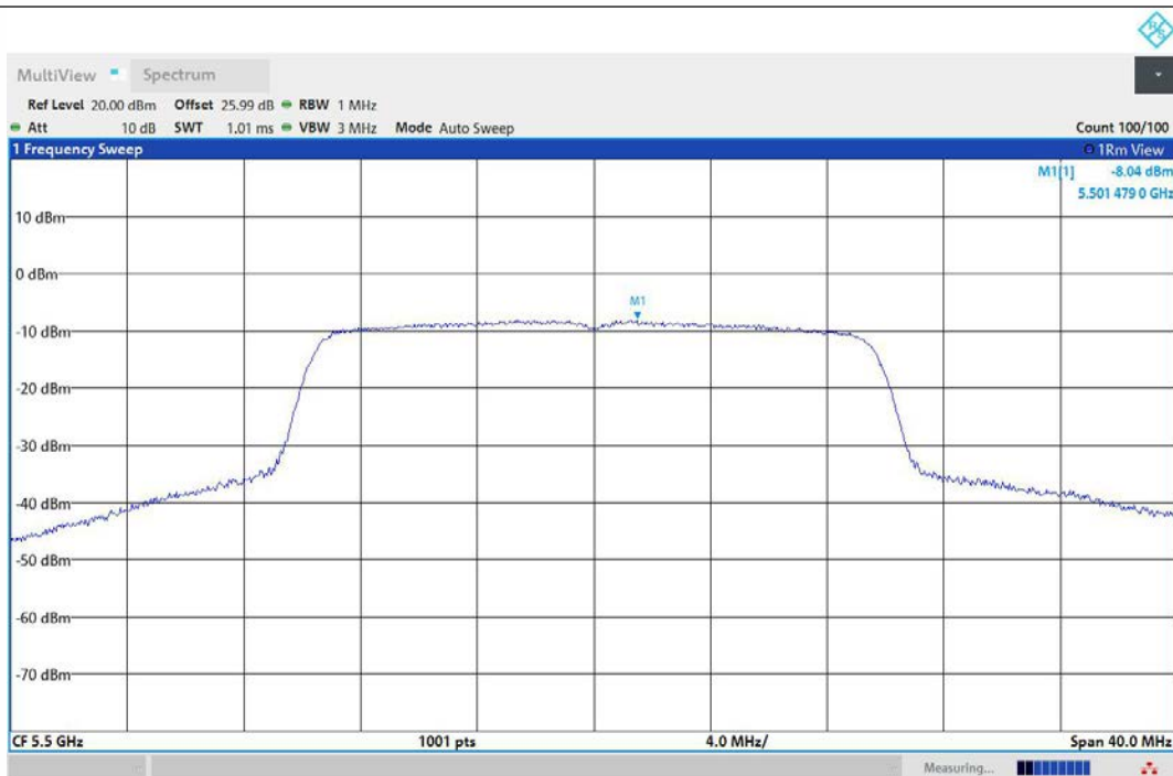
11AX20MIMO-Ant2-5500-PASS
