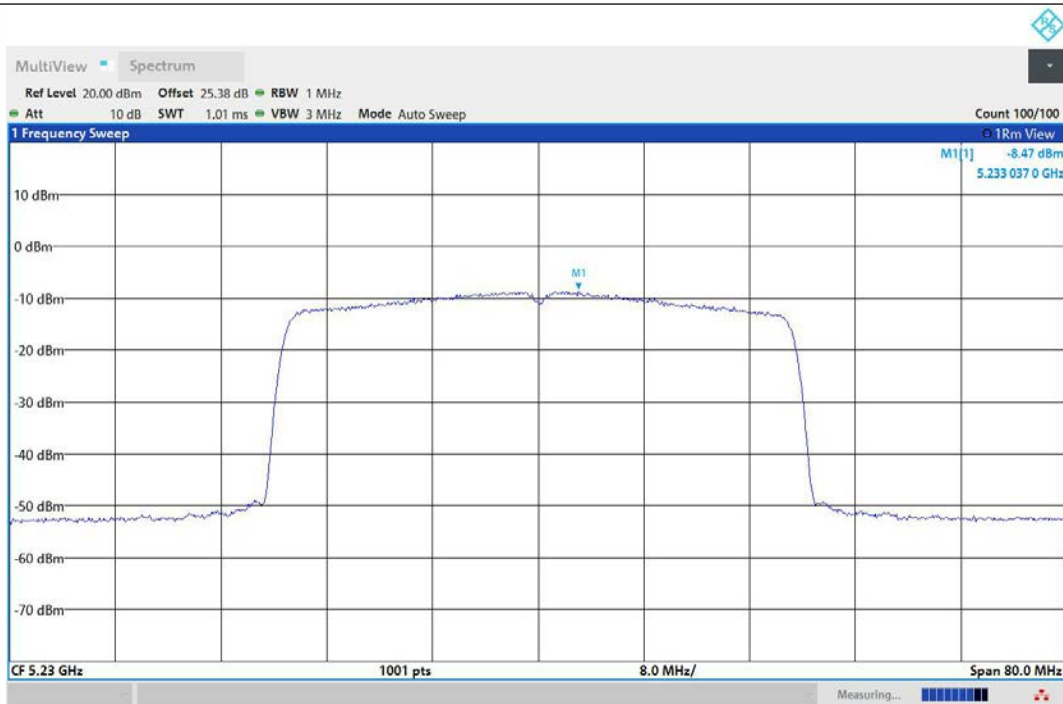
11AX40MIMO-Ant3-5230-PASS
