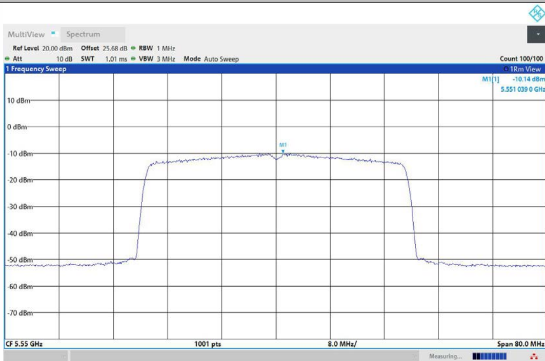
11AX40MIMO-Ant2-5550-PASS
