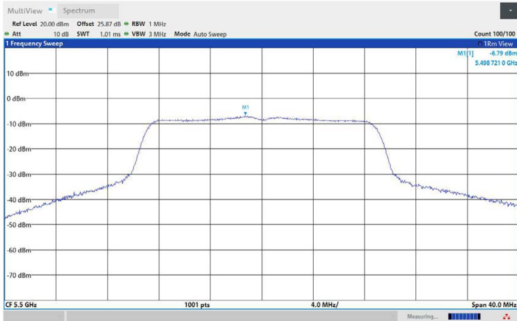
11AC20MIMO-Ant3-5500-PASS
