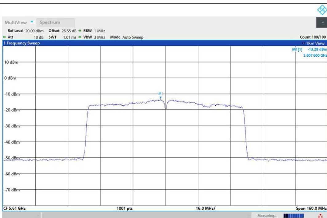
11AC80MIMO-Ant2-5610-PASS
