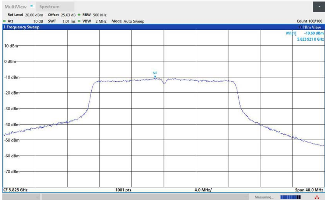
11AC20MIMO-Ant2-5825-PASS
