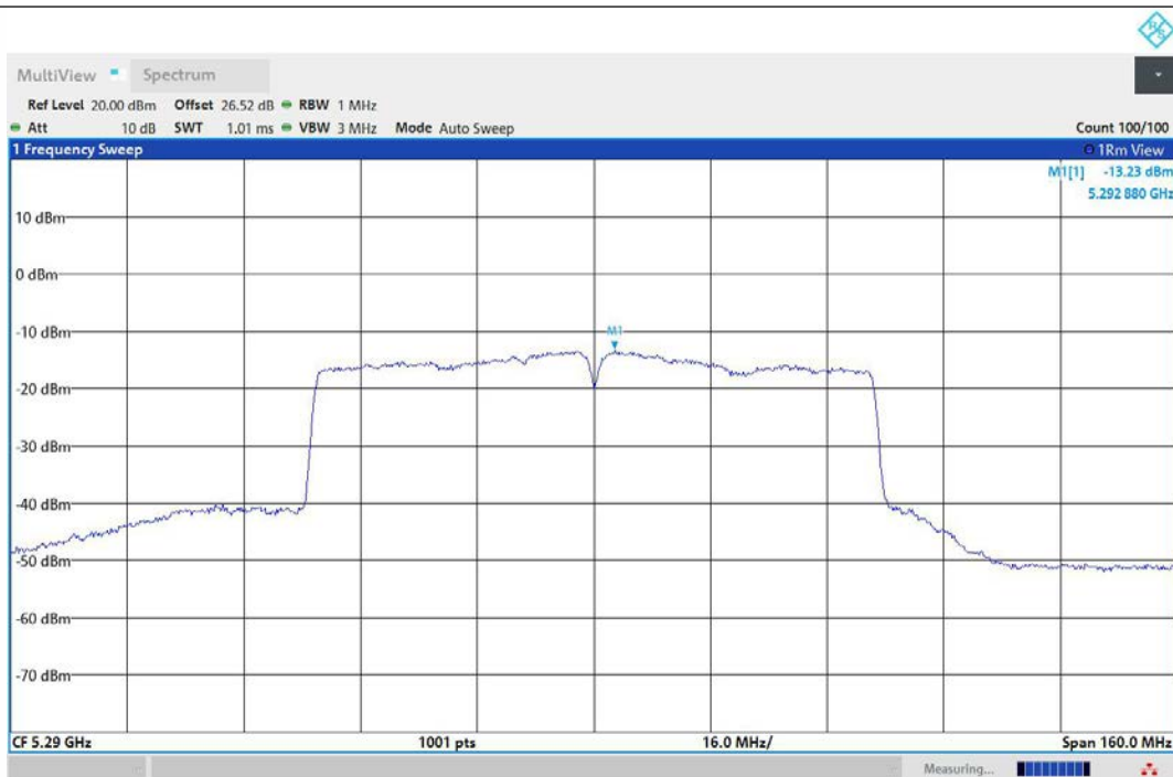
11AC80MIMO-Ant2-5290-PASS
