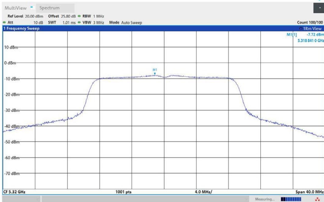
11AC20MIMO-Ant3-5320-PASS
