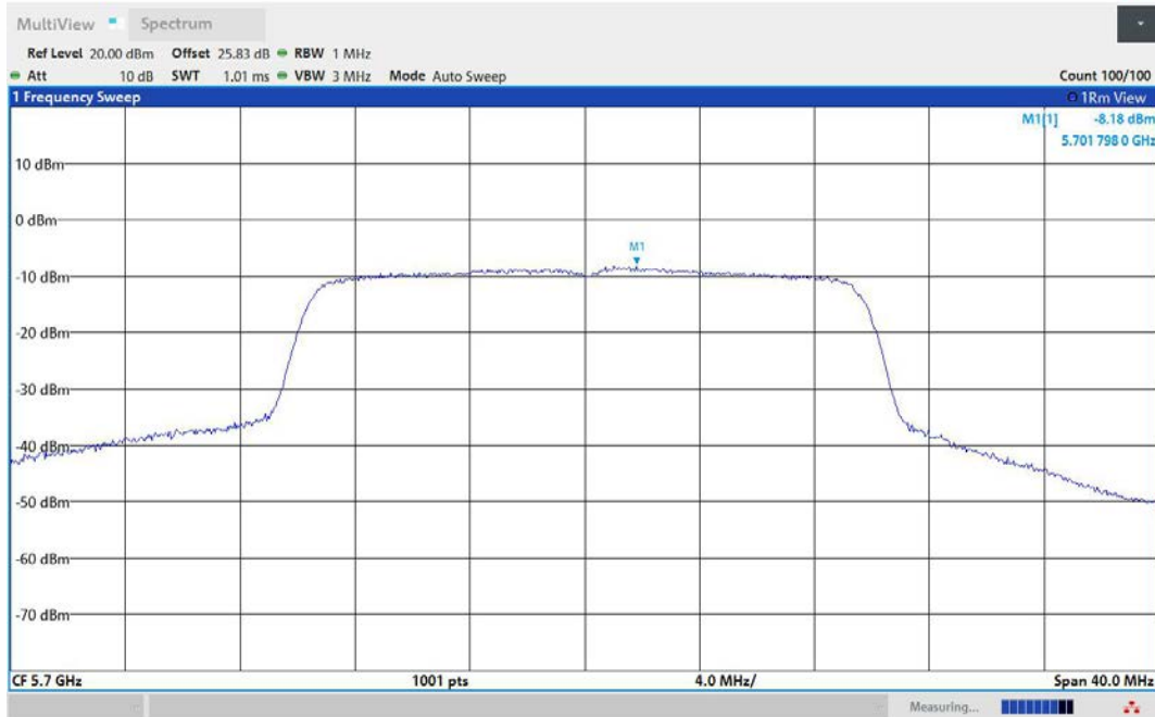
11AX20MIMO-Ant3-5700-PASS
