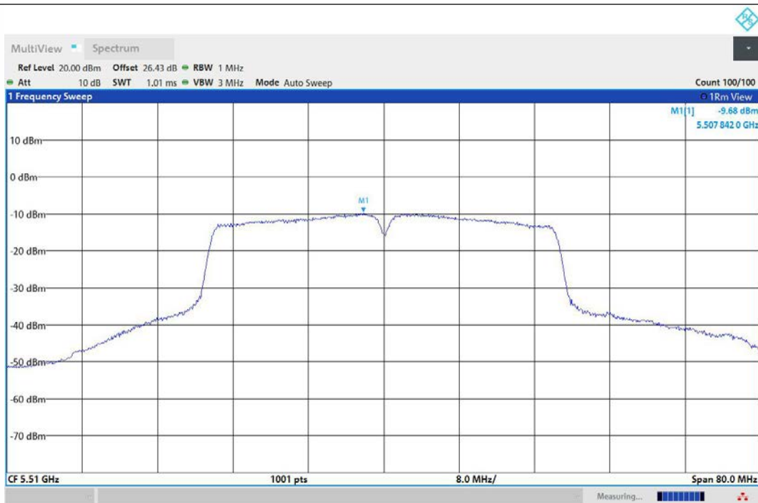
11AC40MIMO-Ant2-5510-PASS
