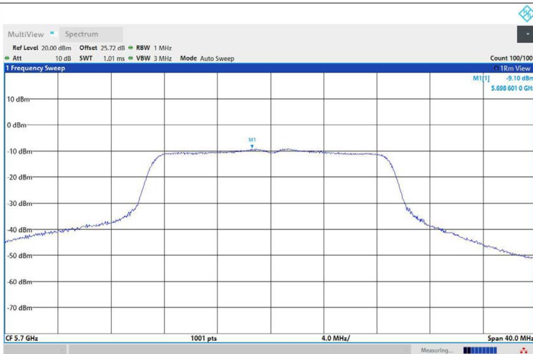
11AC20MIMO-Ant2-5700-PASS
