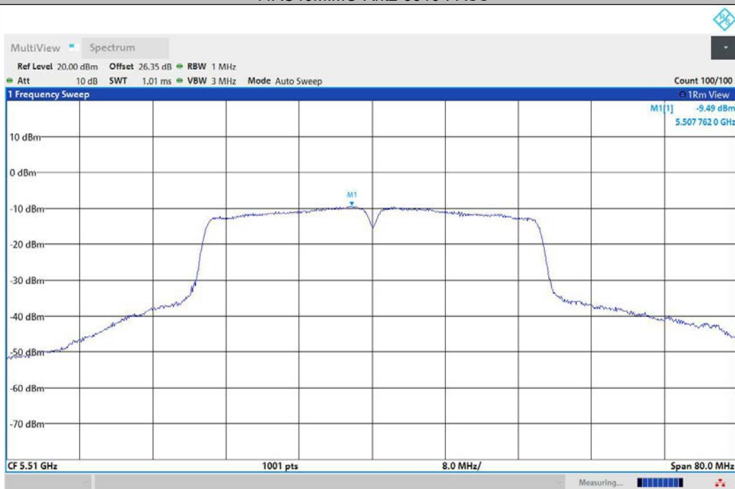
11AC40MIMO-Ant3-5510-PASS
