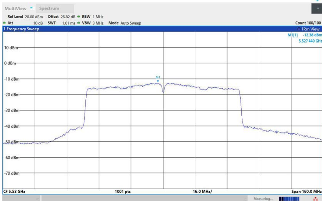
11AC80MIMO-Ant3-5530-PASS
