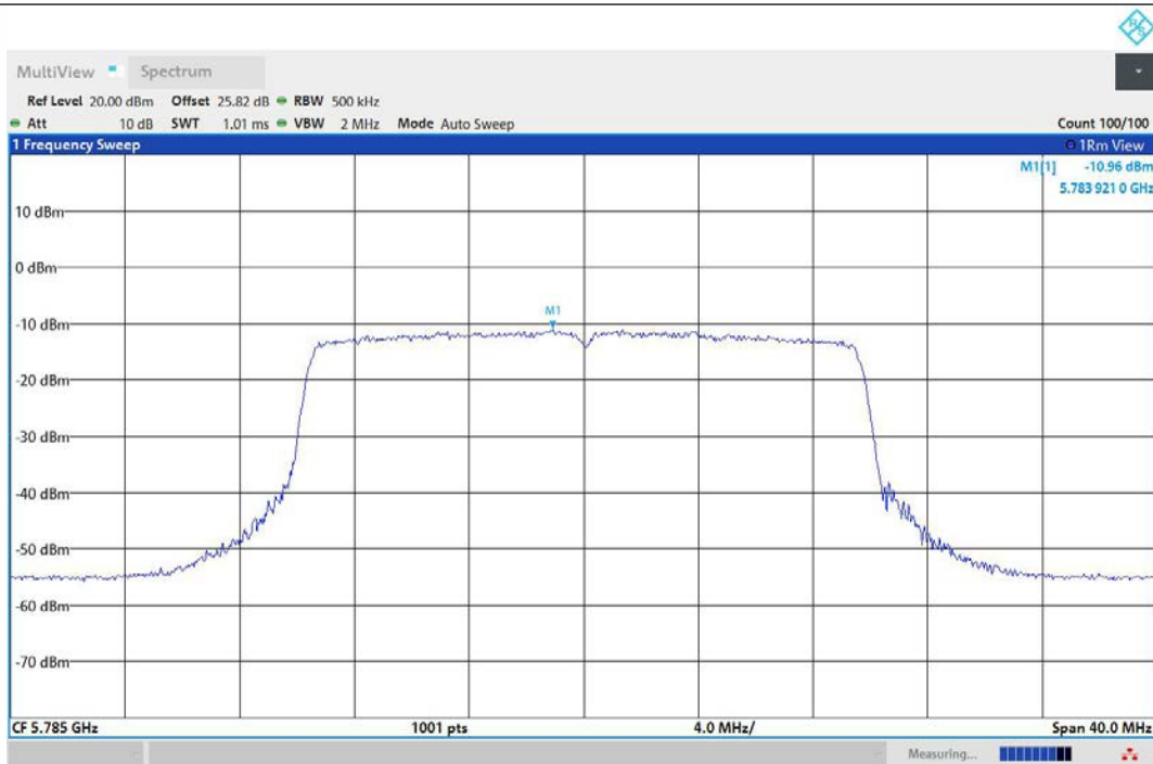
11AX20MIMO-Ant2-5785-PASS
