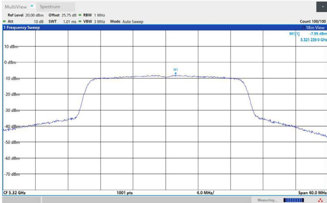
11AX20MIMO-Ant2-5320-PASS
