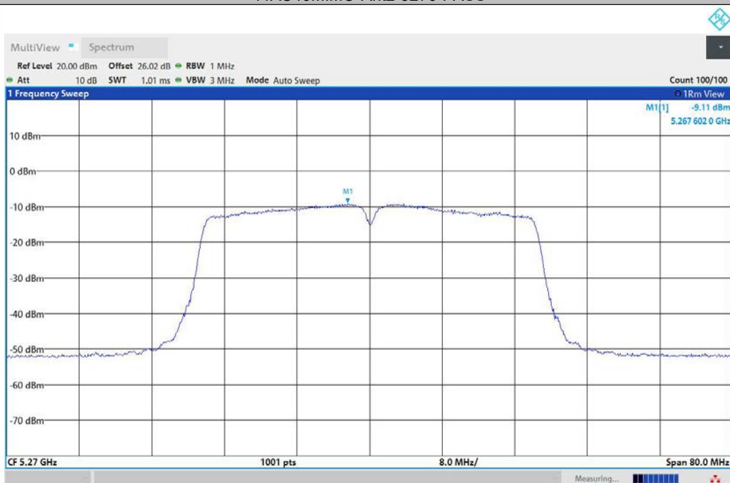
11AC40MIMO-Ant3-5270-PASS
