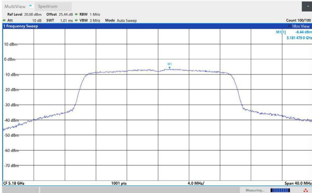
11AX20MIMO-Ant3-5180-PASS
