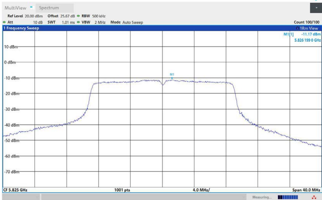
11AC20MIMO-Ant1-5825-PASS
