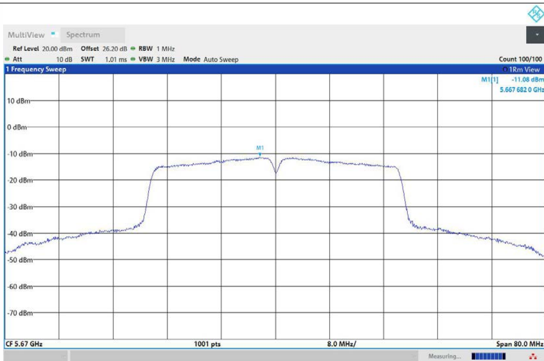
11AC40MIMO-Ant2-5670-PASS
