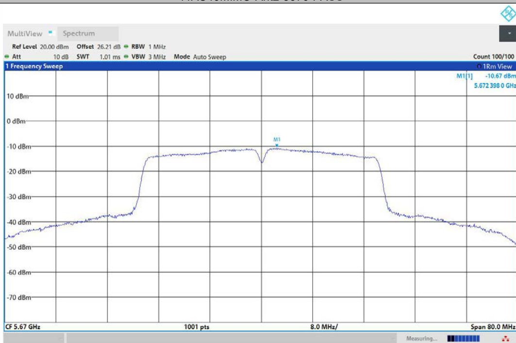
11AC40MIMO-Ant3-5670-PASS
