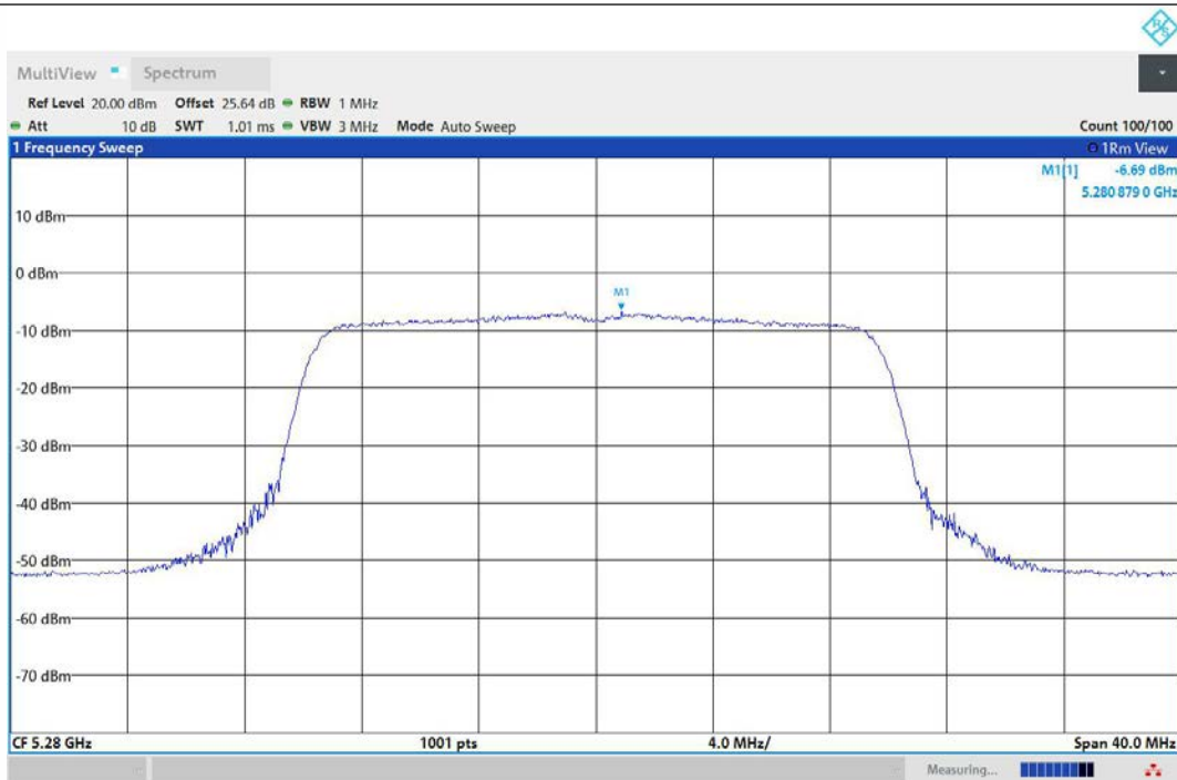
11AX20MIMO-Ant2-5280-PASS
