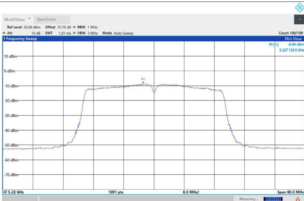
11AC40MIMO-Ant3-5230-PASS
