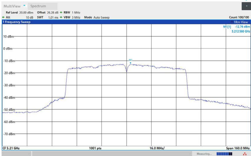
11AC80MIMO-Ant3-5210-PASS
