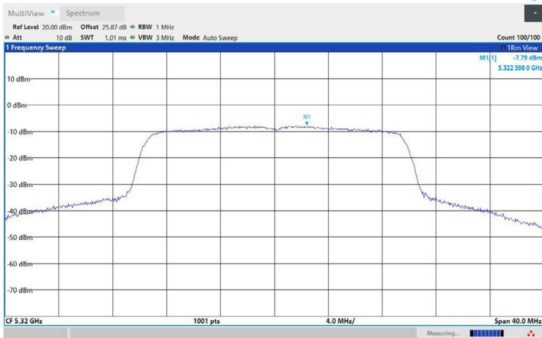
11AX20MIMO-Ant3-5320-PASS
