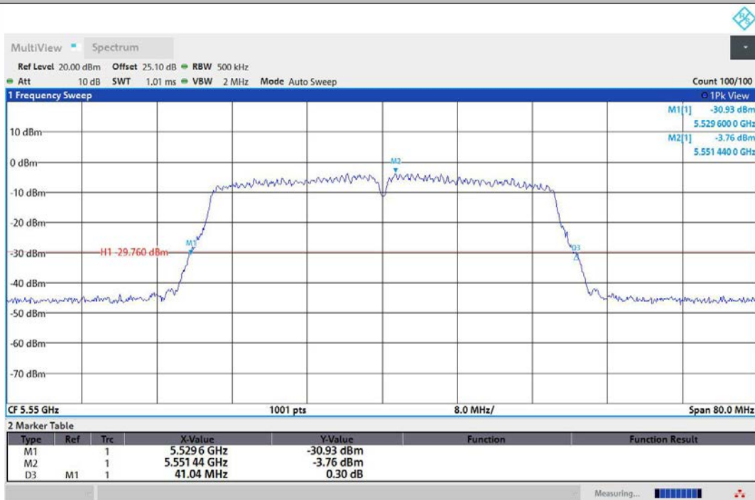
11AC40MIMO-Ant2-5550
