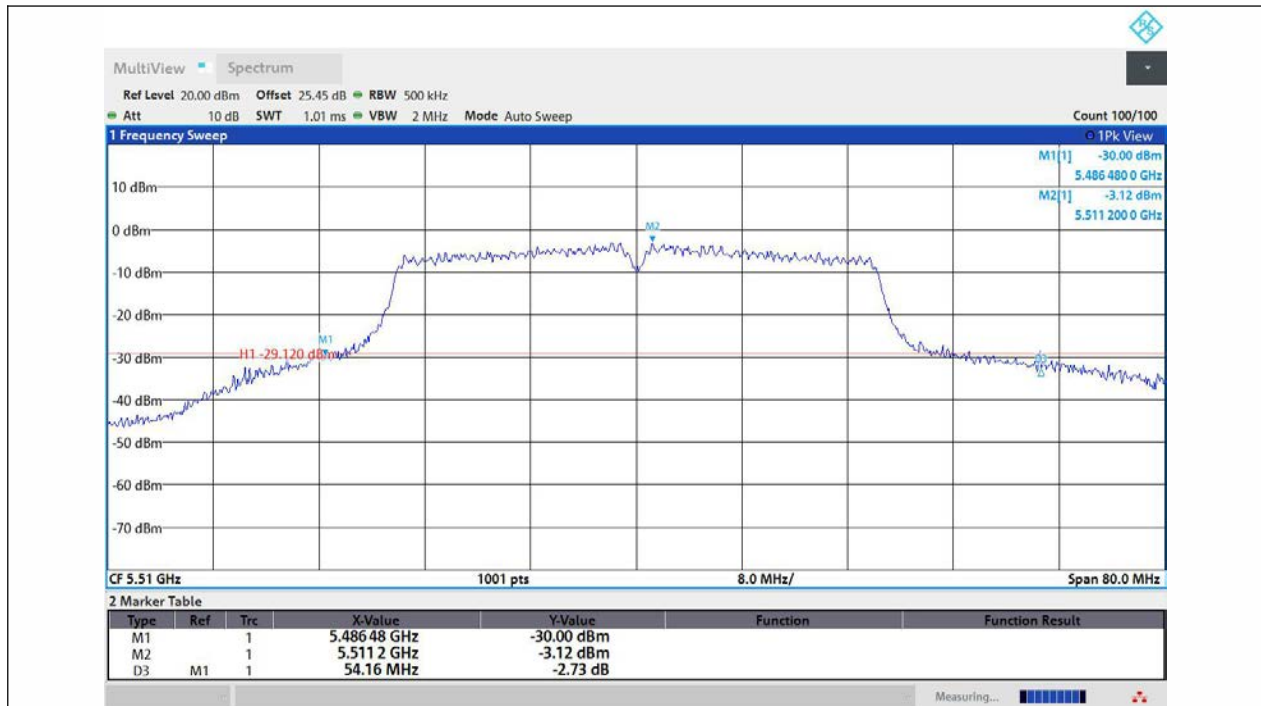
11N40MIMO-Ant3-5510
