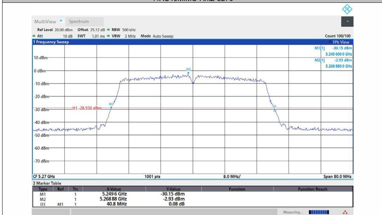
11AC40MIMO-Ant3-5270
