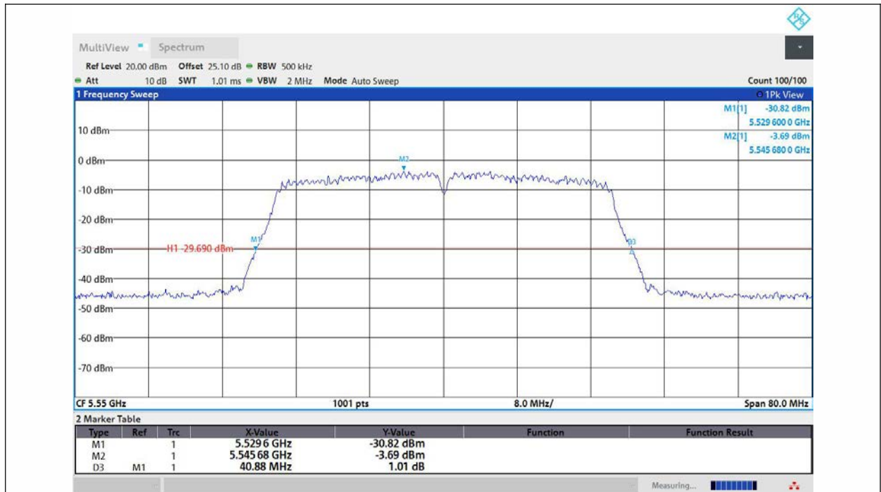
11N40MIMO-Ant2-5550
