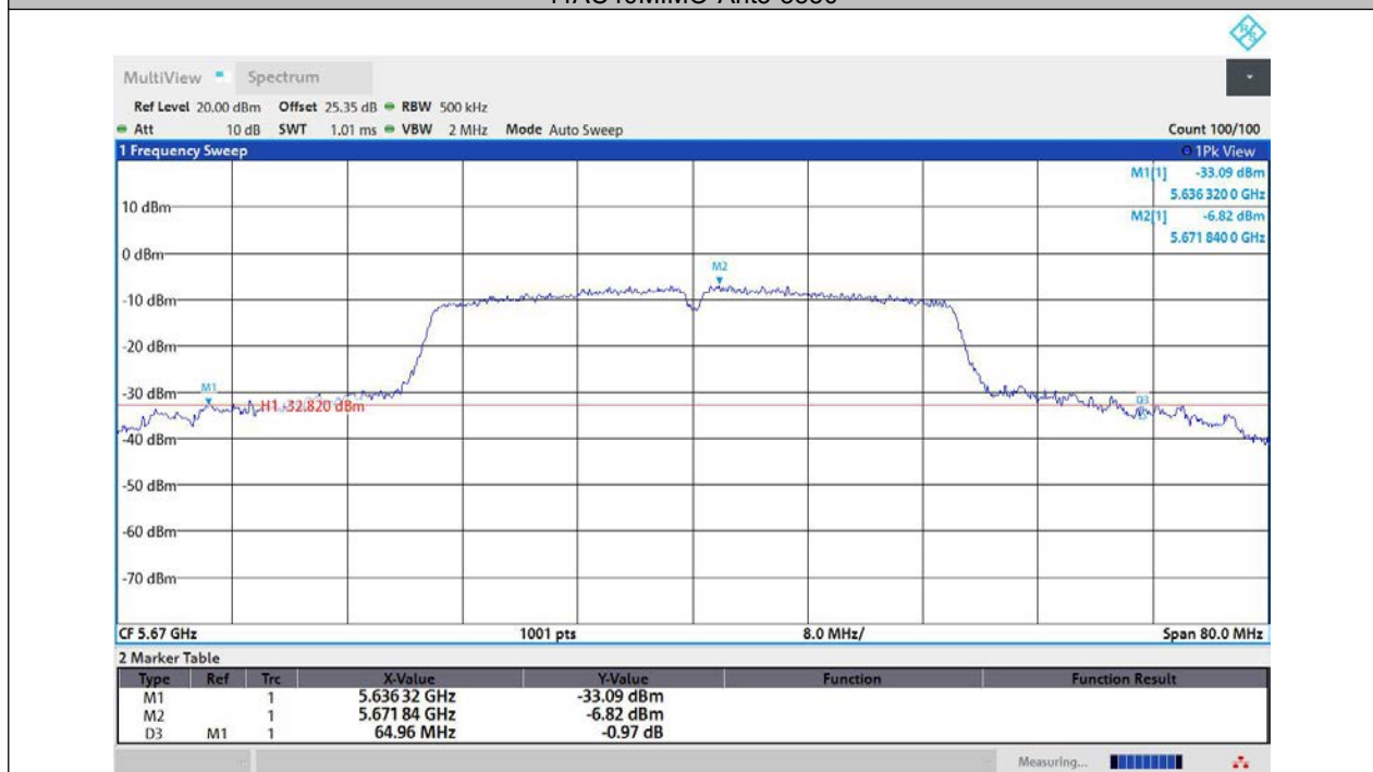
11AC40MIMO-Ant1-5670
