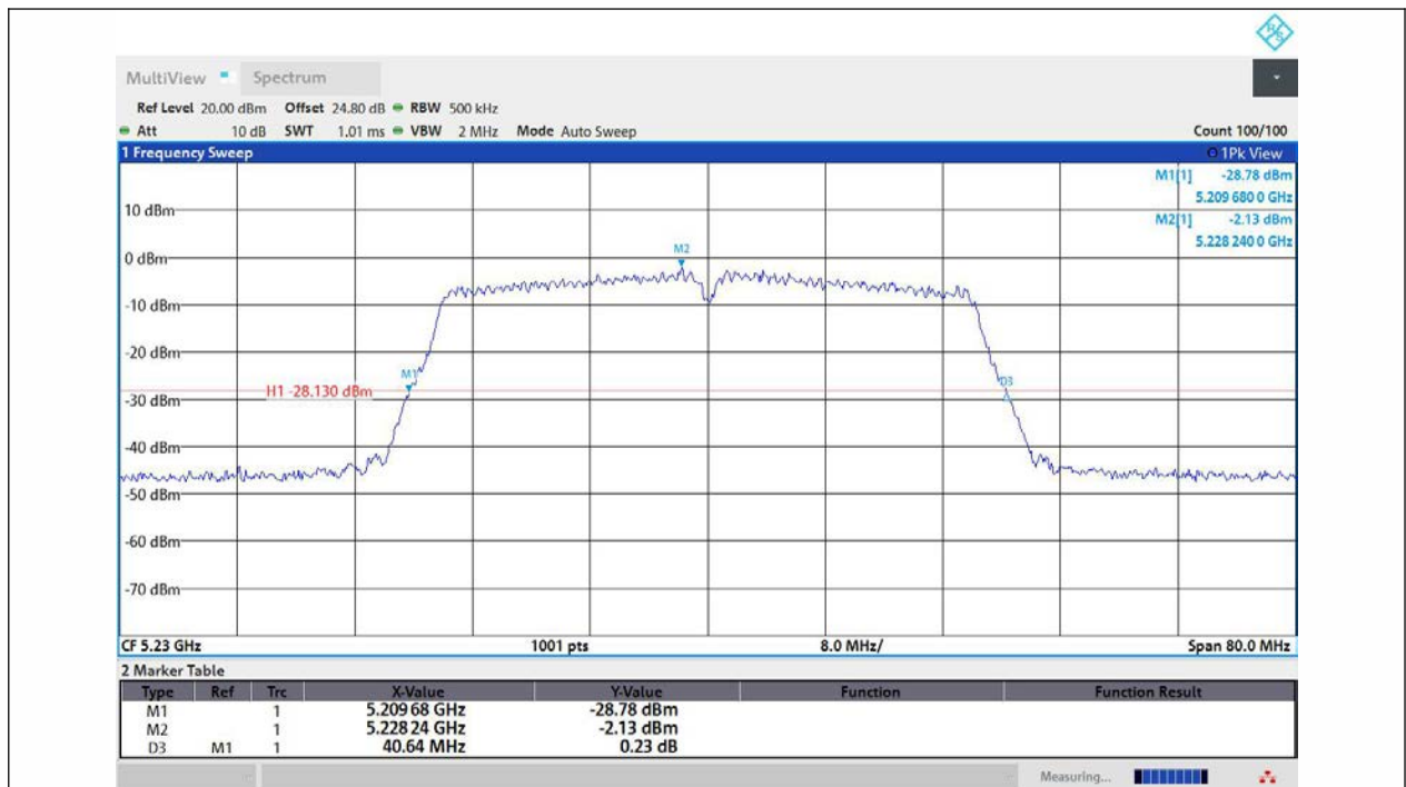
11AC40MIMO-Ant3-5230
