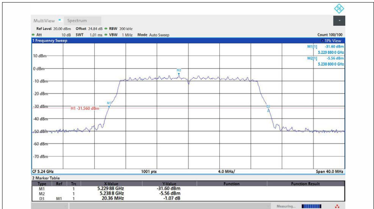
11AC20MIMO-Ant2-5240
