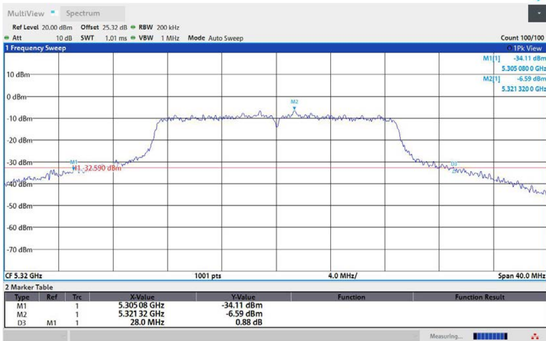
11AC20MIMO-Ant1-5320
