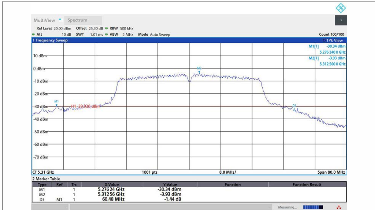
11AC40MIMO-Ant3-5310
