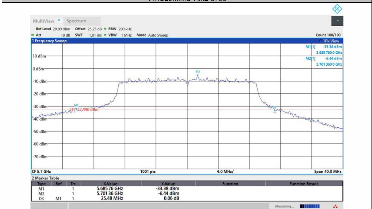
11AC20MIMO-Ant3-5700
