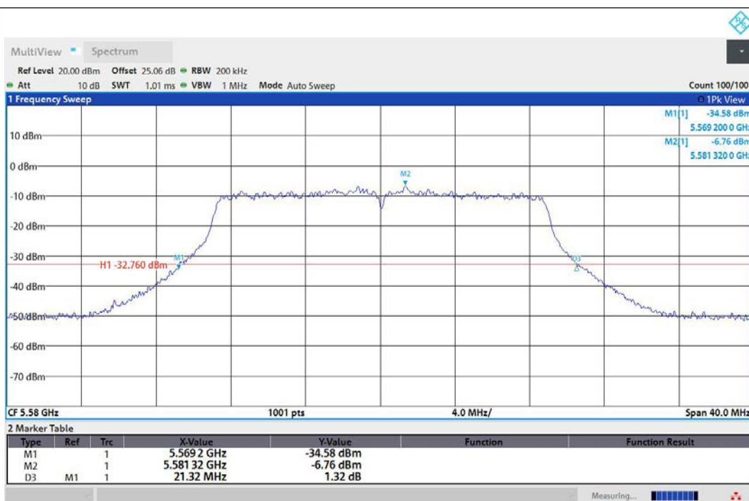
11AC20MIMO-Ant1-5580
