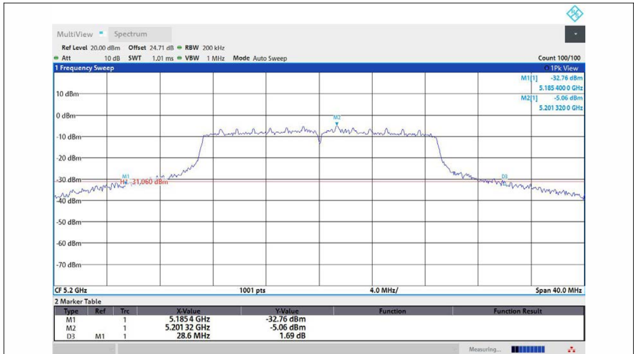
11AC20MIMO-Ant3-5200
