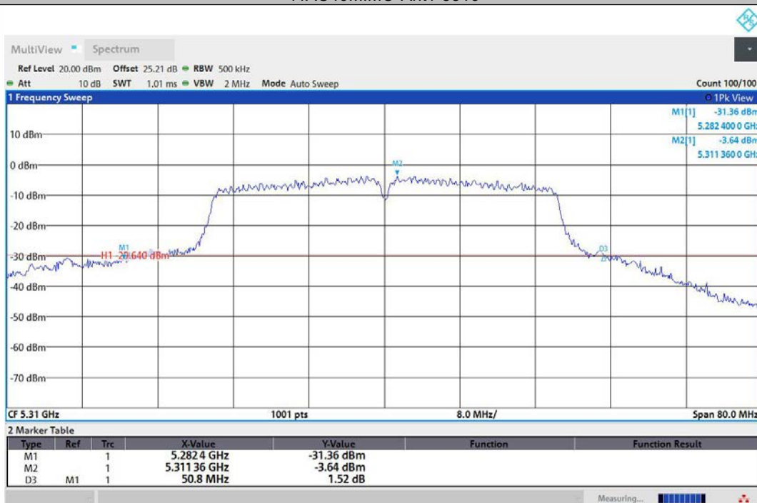
11AC40MIMO-Ant2-5310
