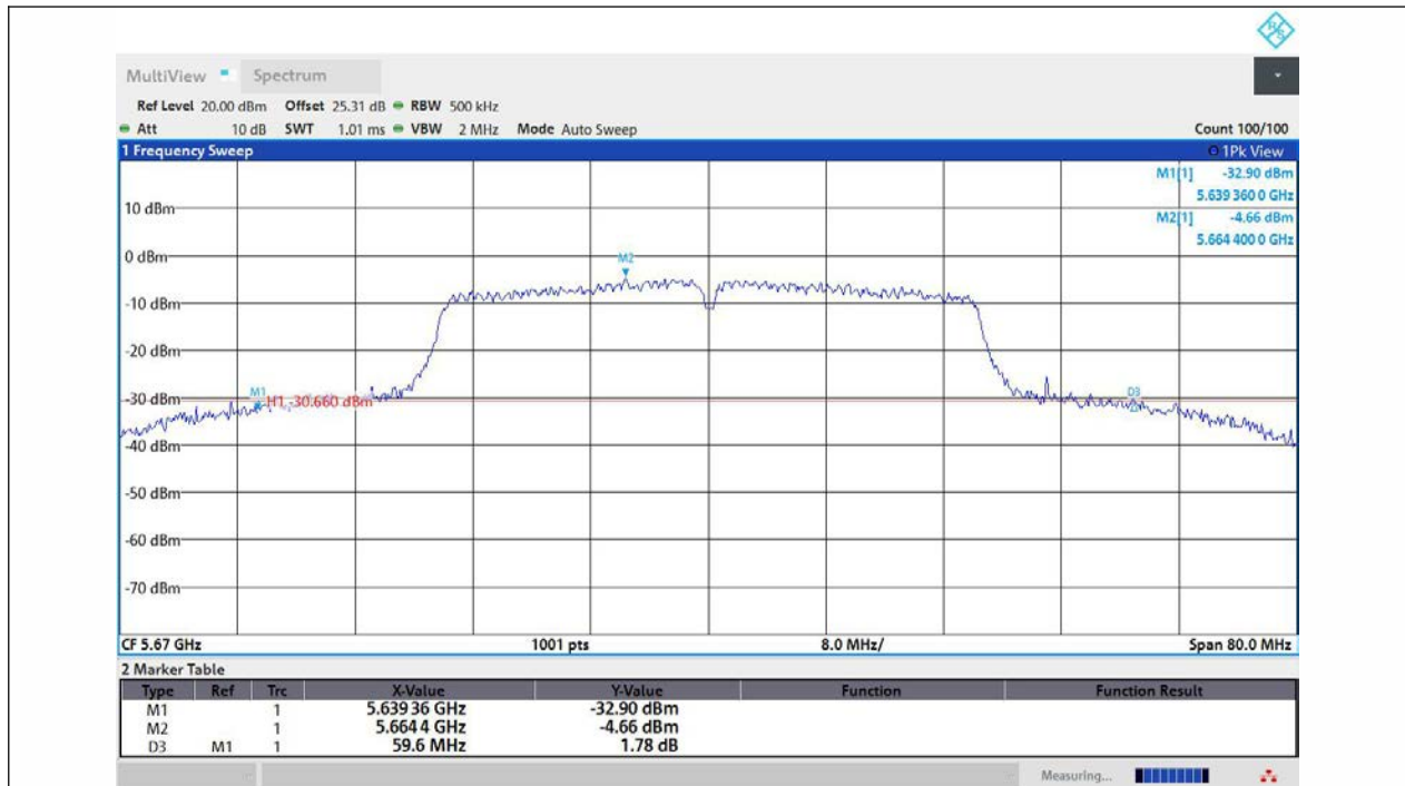
11N40MIMO-Ant3-5670
