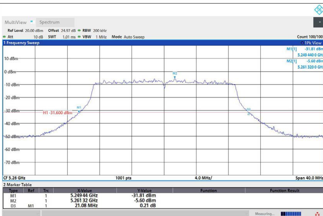
11AC20MIMO-Ant3-5260
