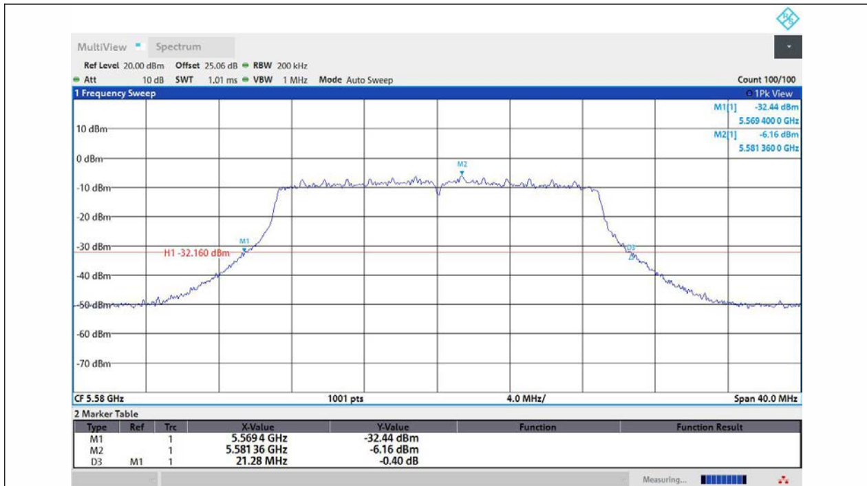
11AC20MIMO-Ant3-5580
