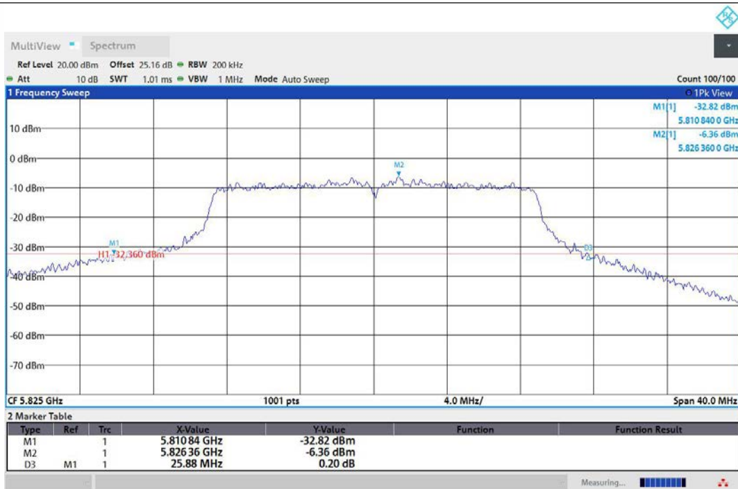
11AC20MIMO-Ant1-5825
