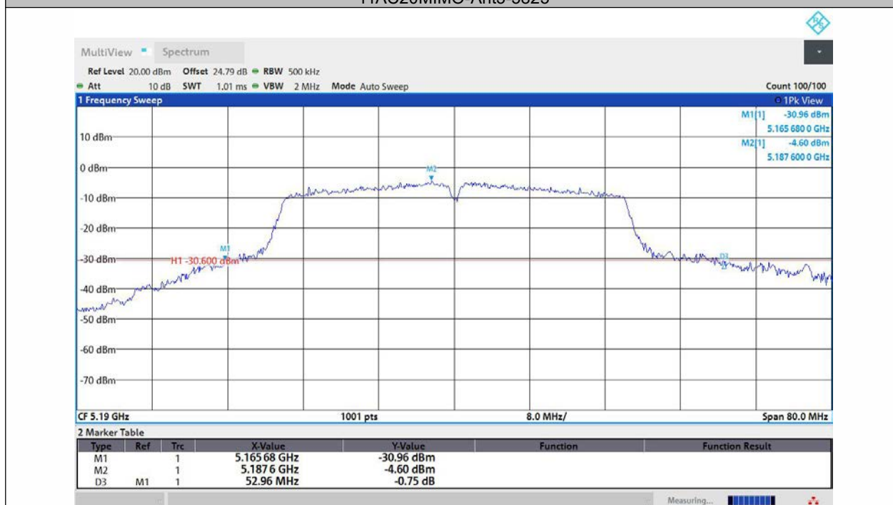
11AC40MIMO-Ant1-5190
