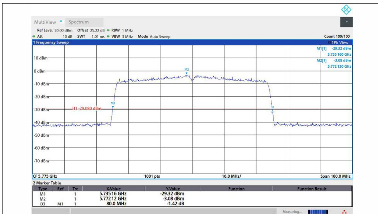
11AC80MIMO-Ant3-5775
