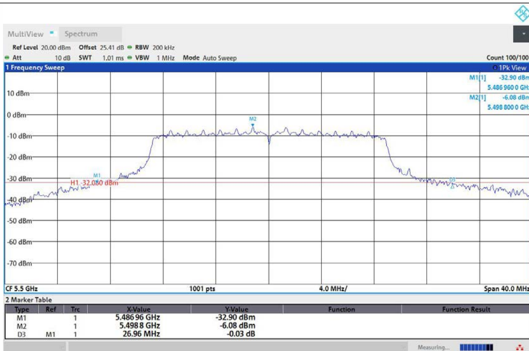
11AC20MIMO-Ant2-5500
