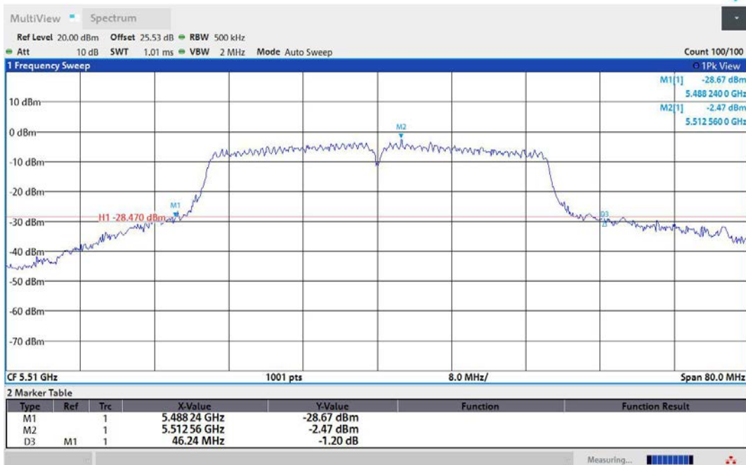
11AC40MIMO-Ant2-5510
