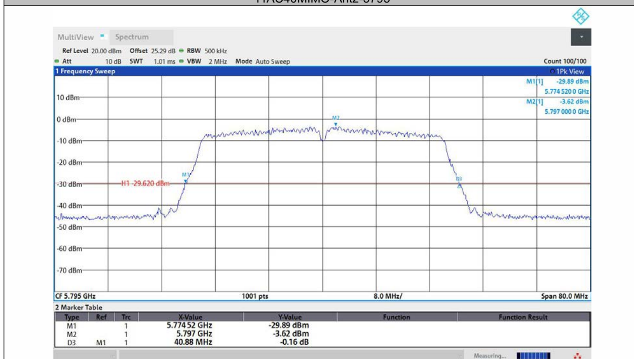
11AC40MIMO-Ant3-5795
