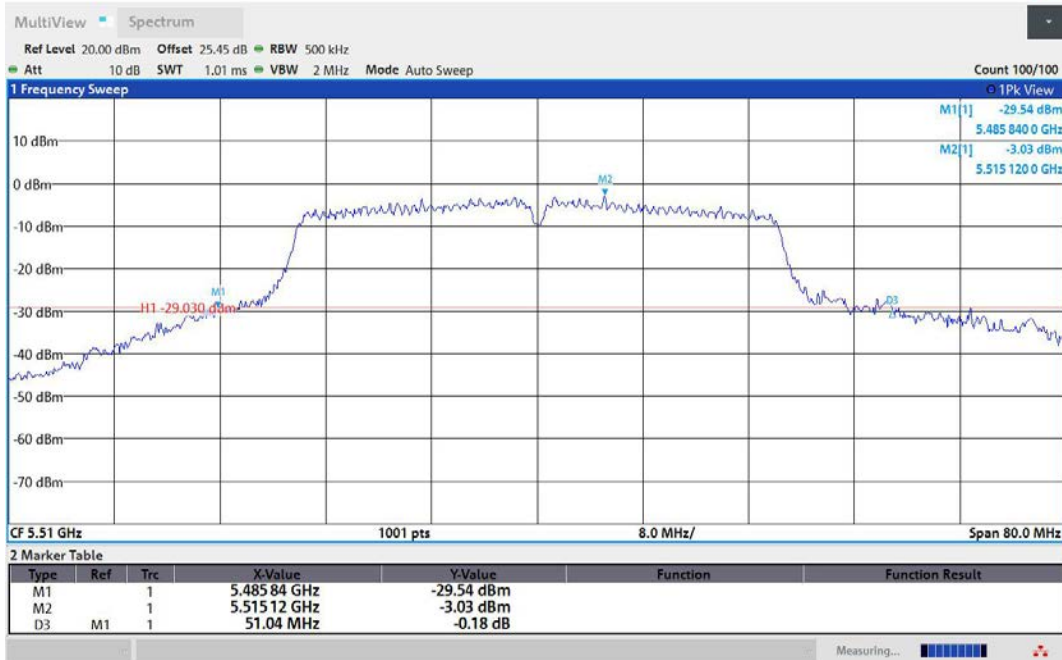
11AC40MIMO-Ant3-5510
