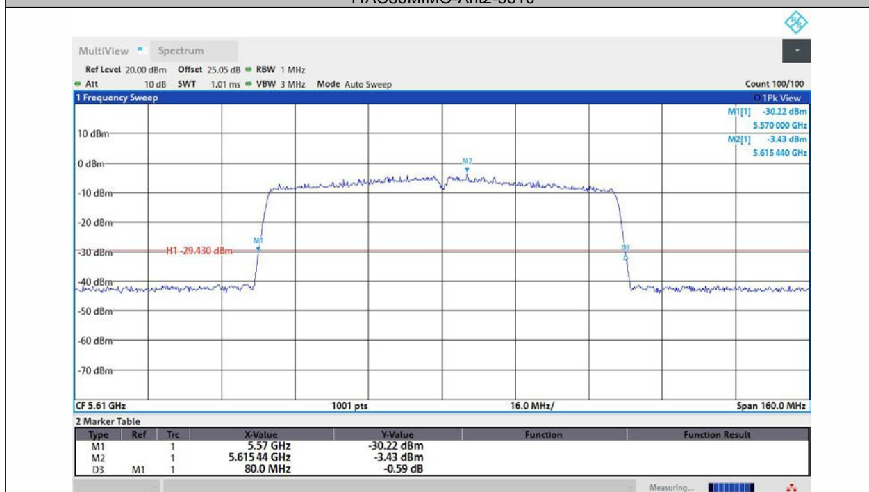
11AC80MIMO-Ant3-5610
