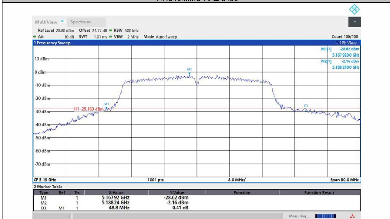
11AC40MIMO-Ant3-5190
