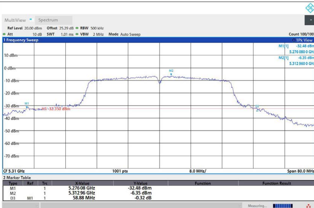
11AC40MIMO-Ant1-5310
