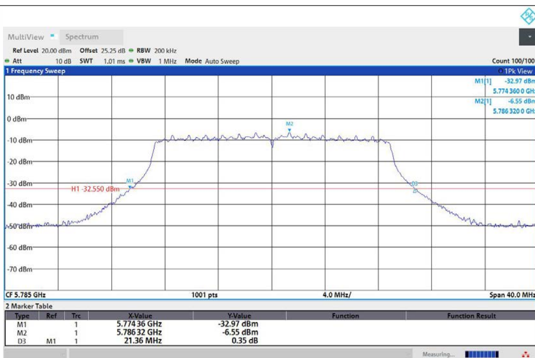
11AC20MIMO-Ant2-5785
