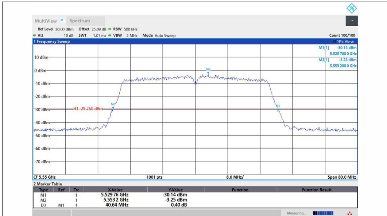
11AC40MIMO-Ant3-5550
