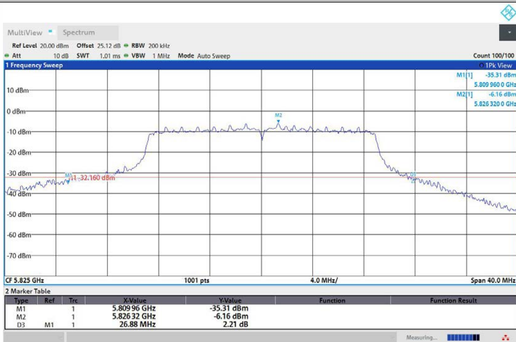
11AC20MIMO-Ant2-5825
