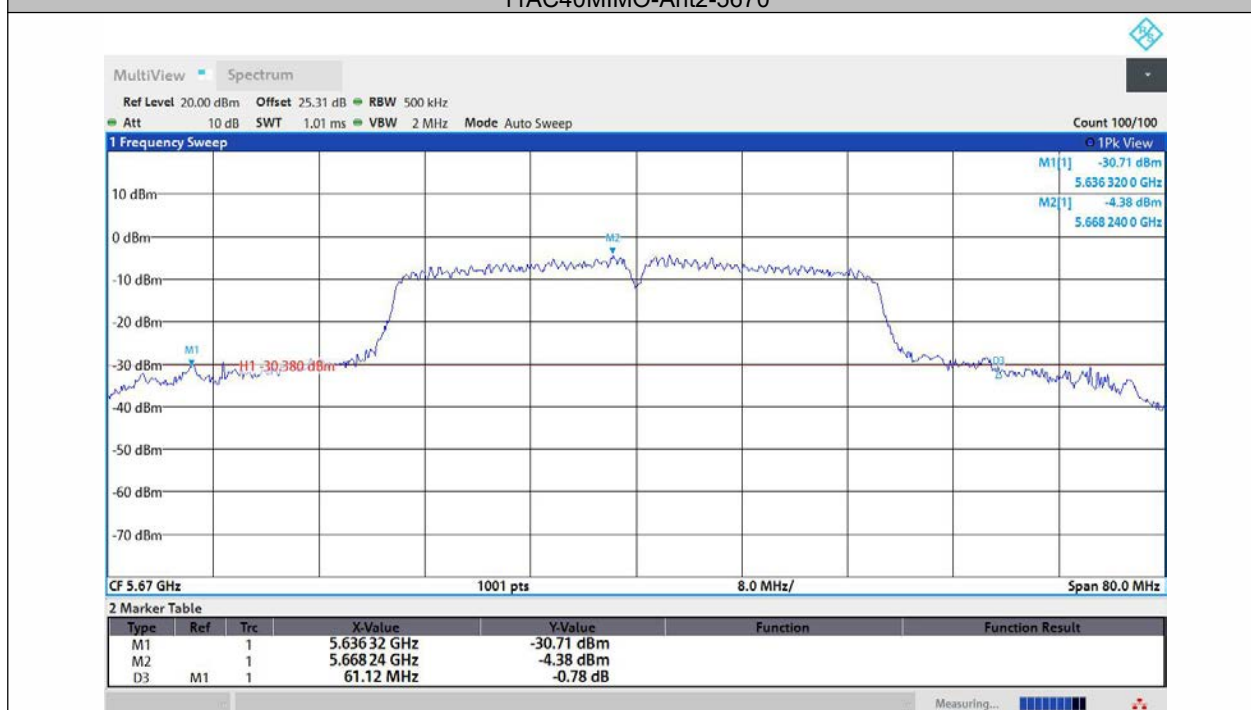
11AC40MIMO-Ant3-5670
