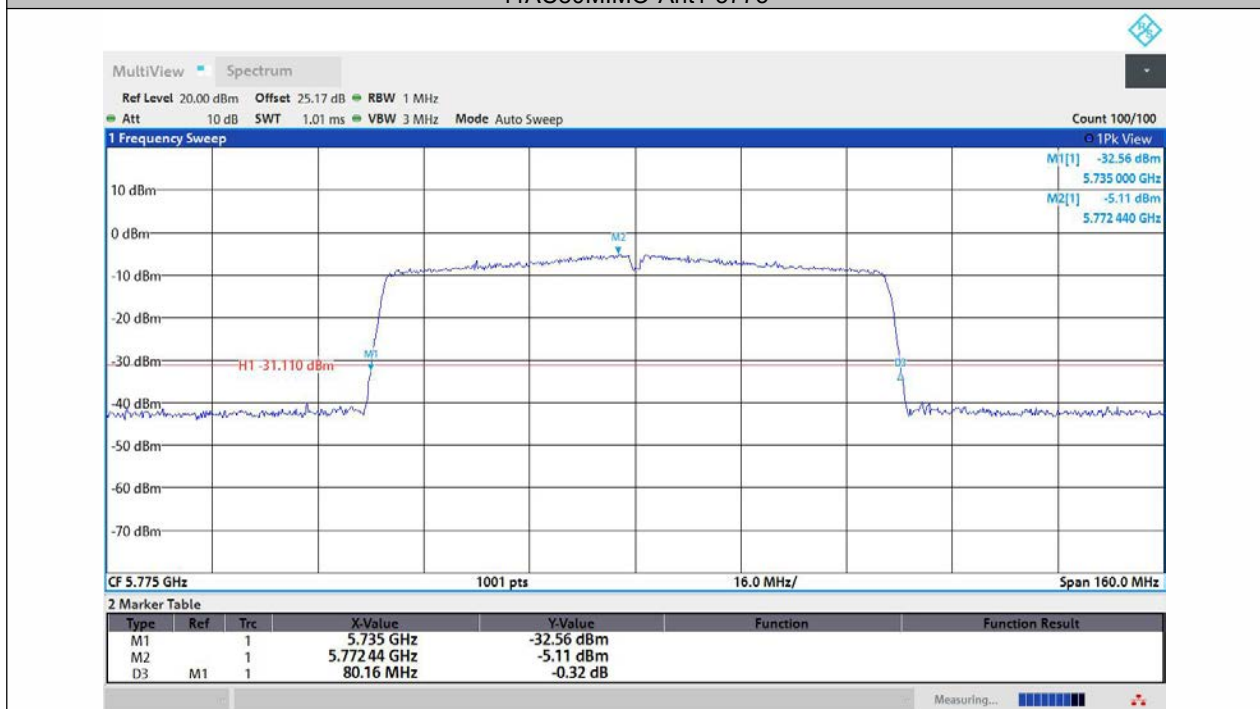
11AC80MIMO-Ant2-5775
