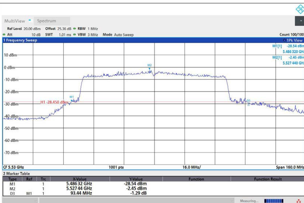
11AC80MIMO-Ant3-5530
