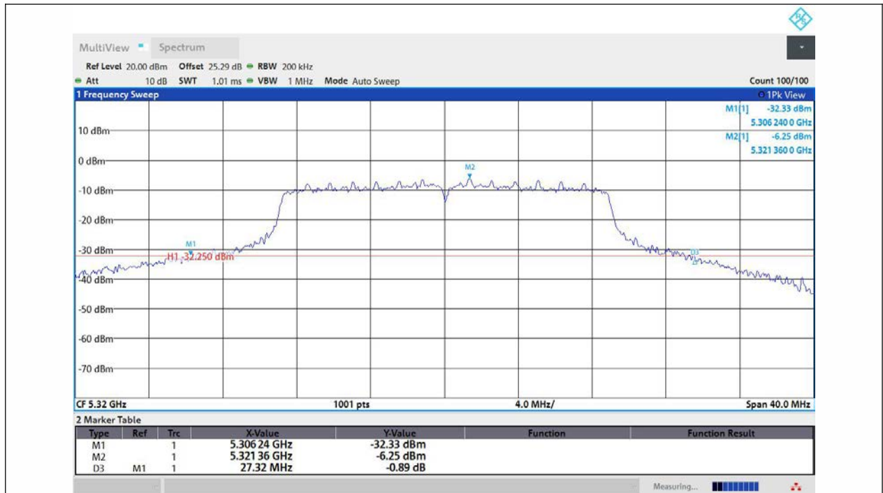
11AC20MIMO-Ant3-5320
