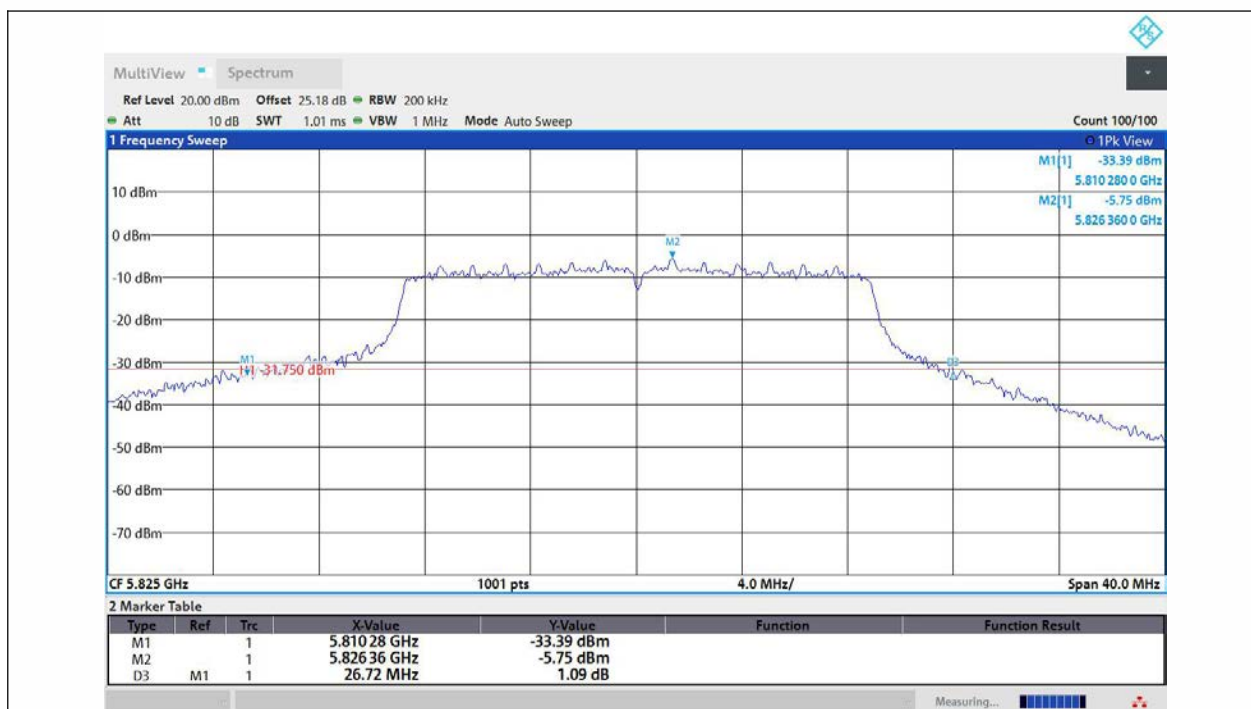
11AC20MIMO-Ant3-5825
