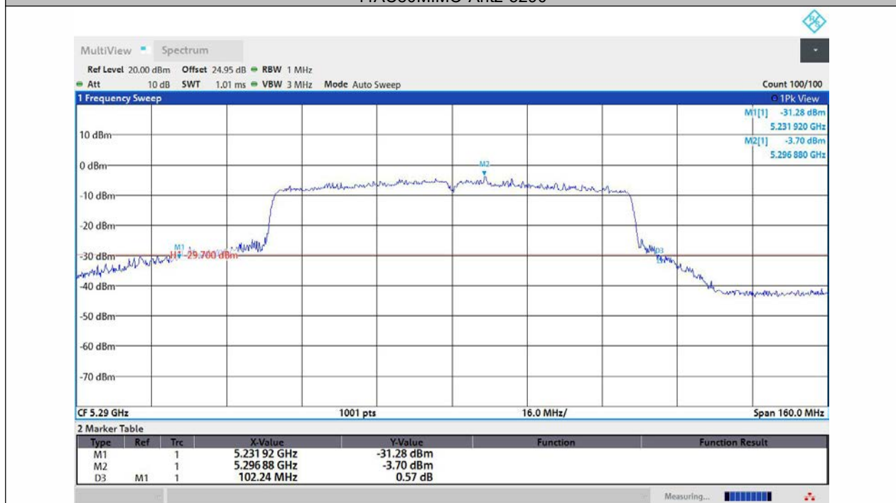
11AC80MIMO-Ant3-5290
