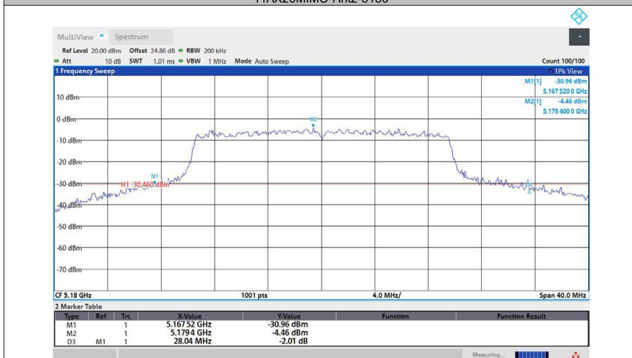
11AX20MIMO-Ant3-5180
