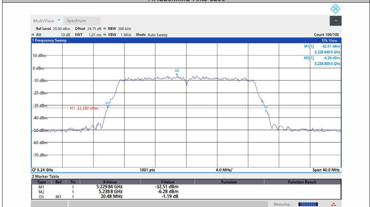
11AC20MIMO-Ant1-5240
