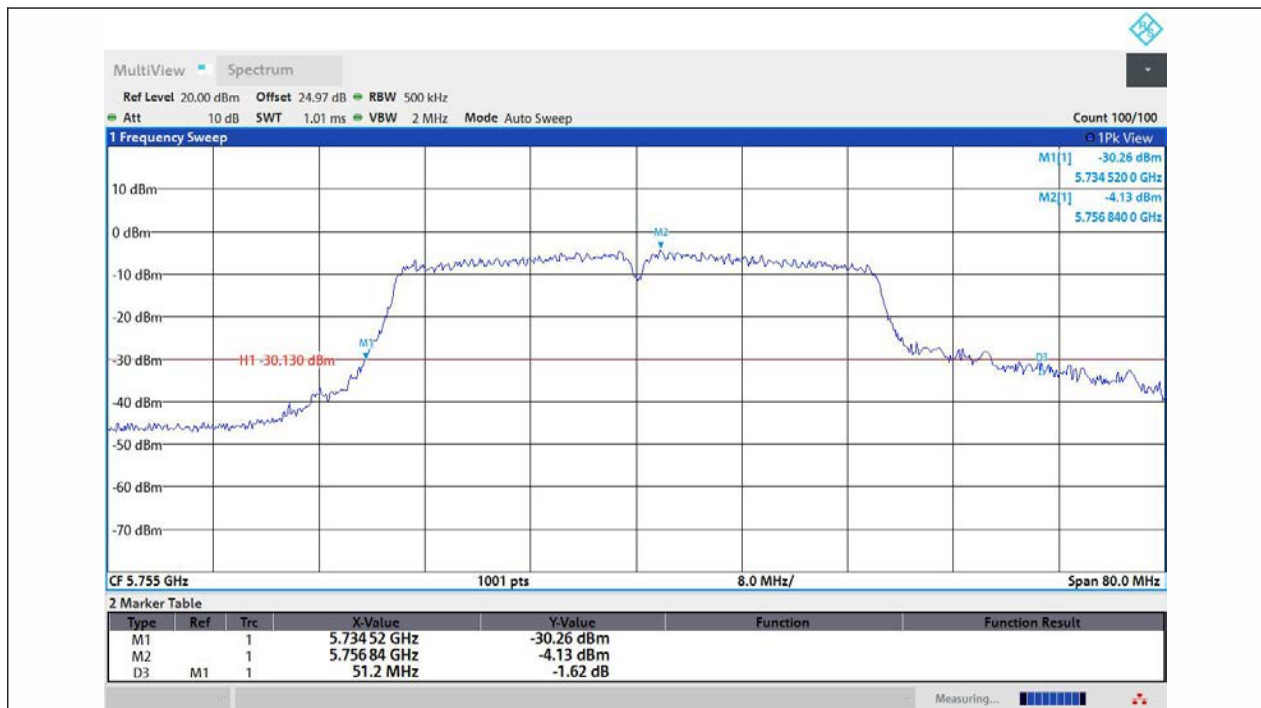
11AC40MIMO-Ant3-5755
