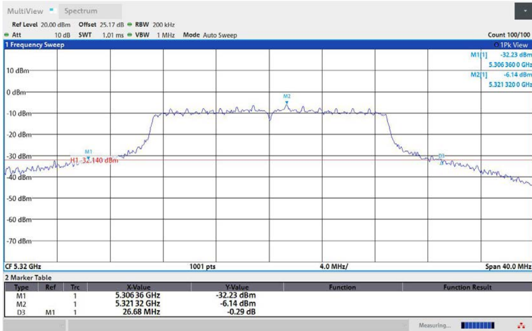
11AC20MIMO-Ant2-5320
