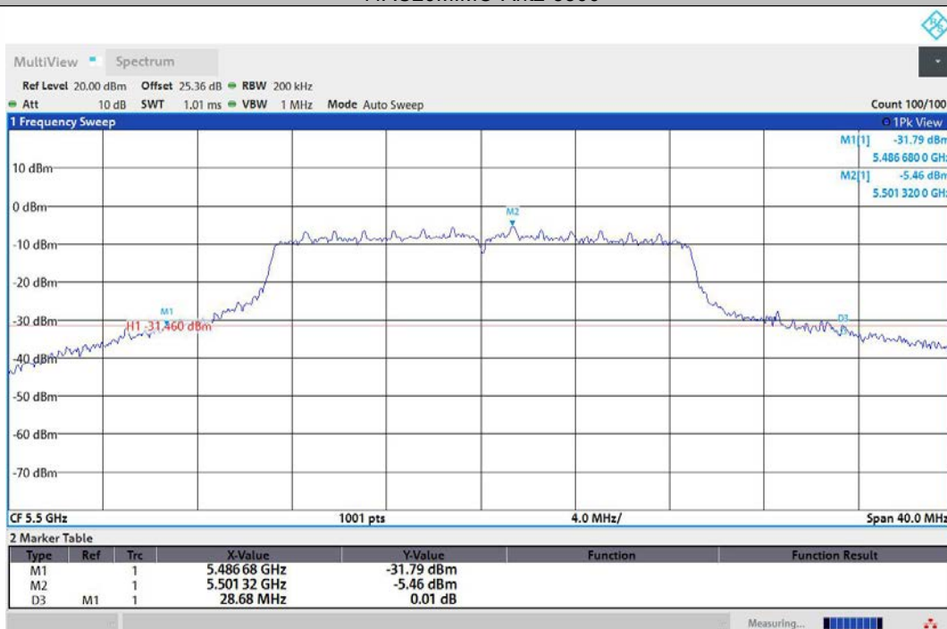
11AC20MIMO-Ant3-5500
