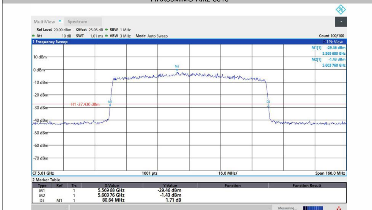
11AX80MIMO-Ant3-5610
