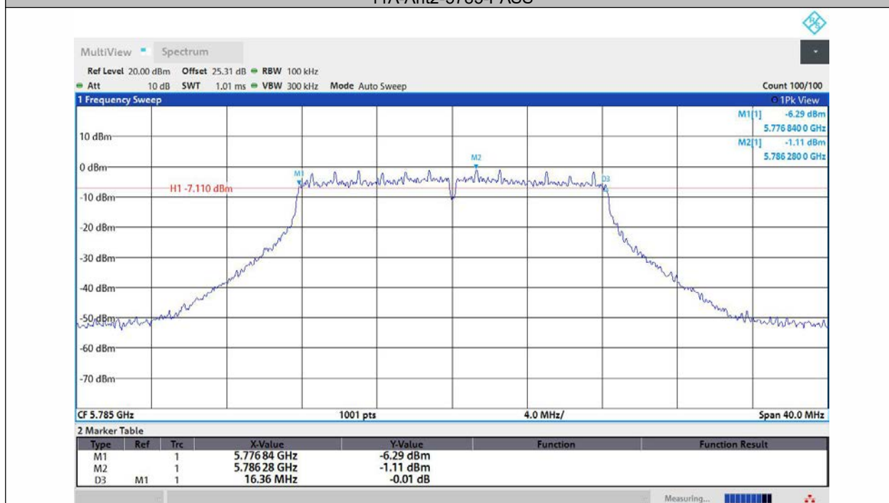
11A-Ant3-5785-PASS
