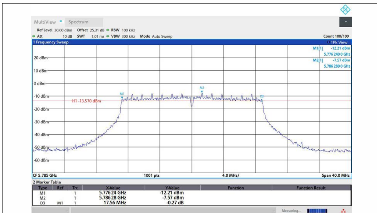
11N20MIMO-Ant3-5785-PASS
