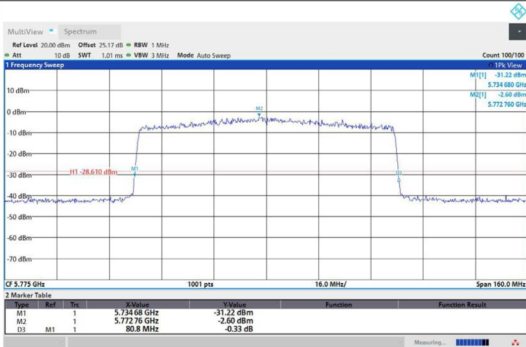
11AX80MIMO-Ant2-5775
