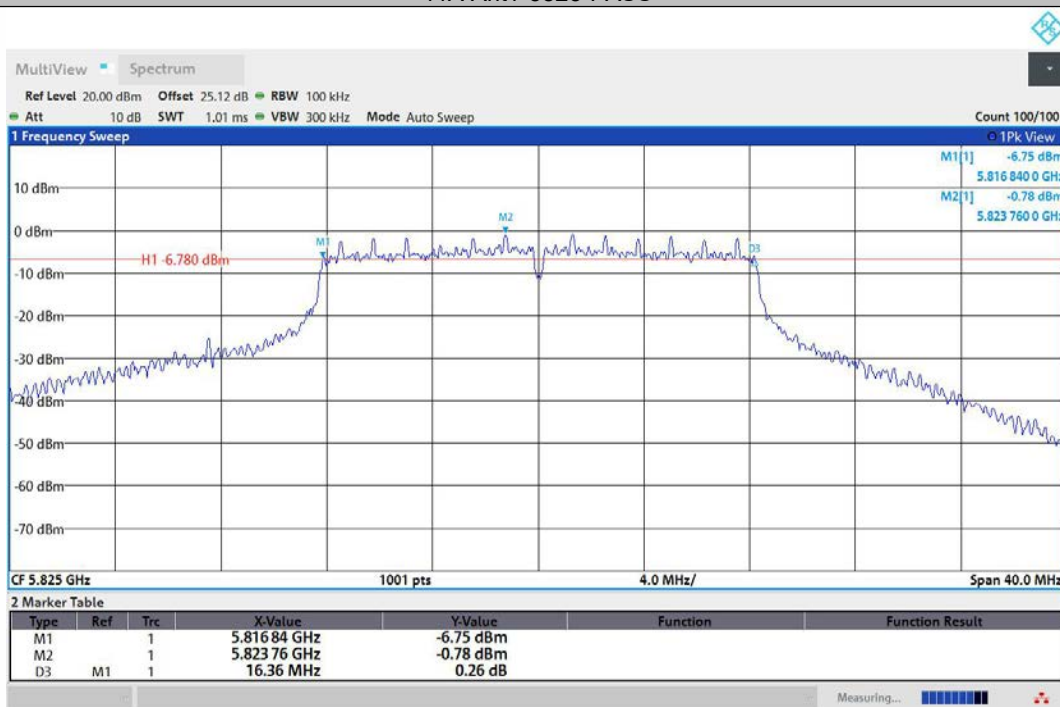
11A-Ant2-5825-PASS
