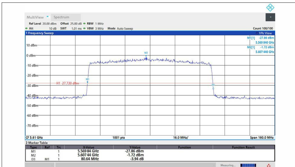
11AX80MIMO-Ant2-5610
