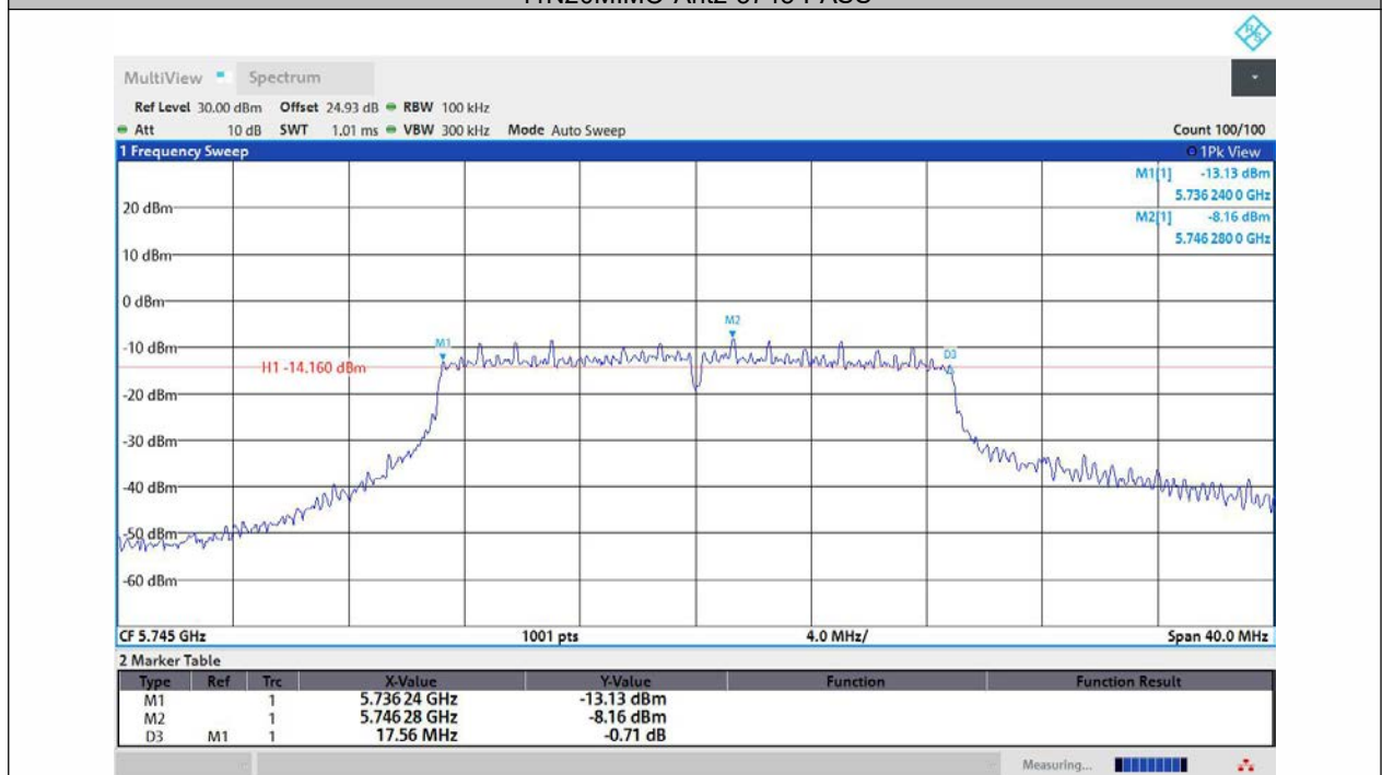
11N20MIMO-Ant3-5745-PASS
