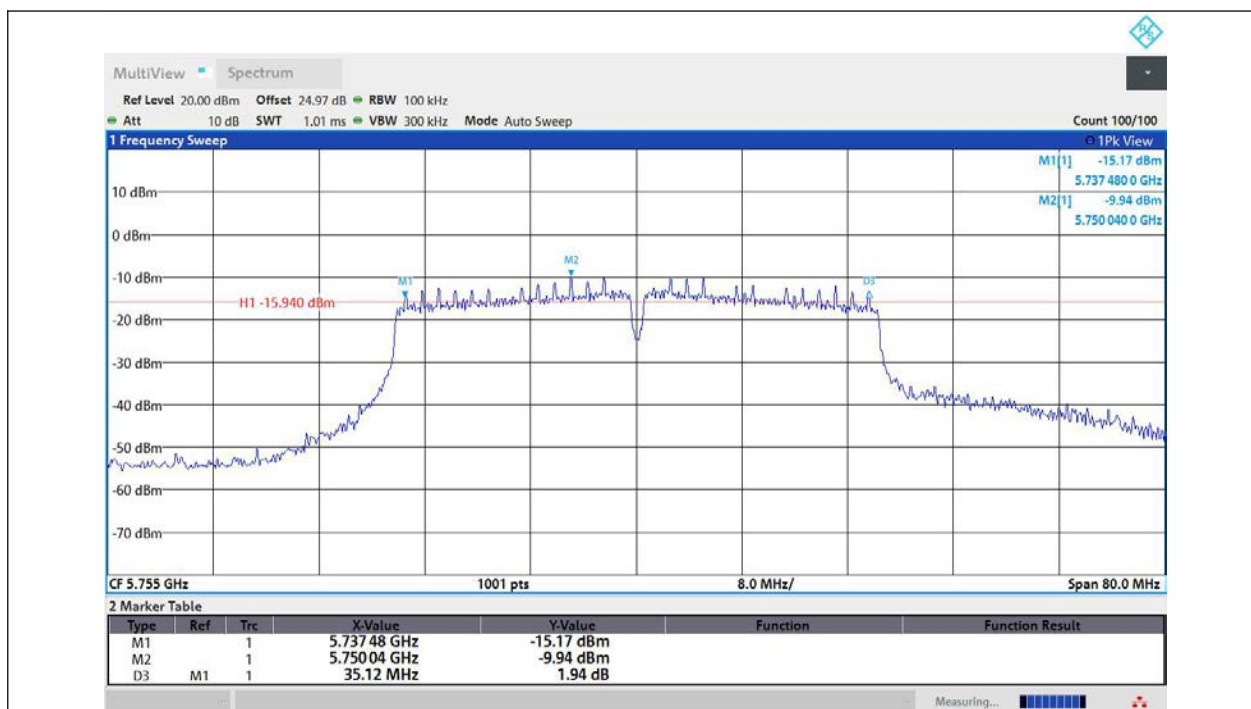
11N40MIMO-Ant3-5755-PASS
