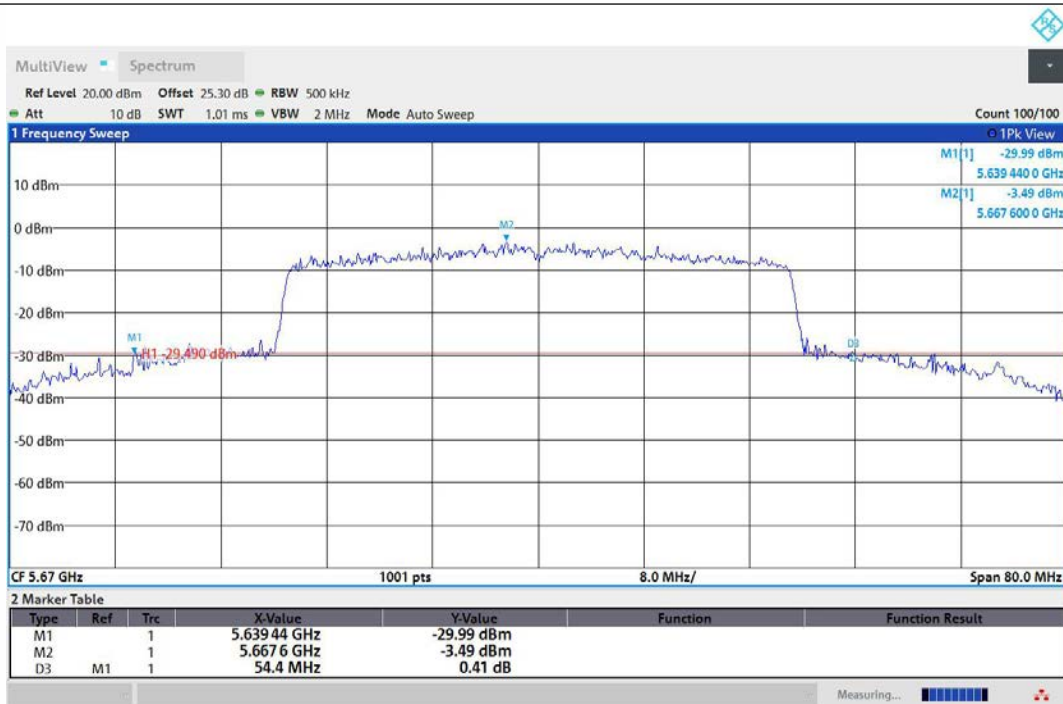
11AX40MIMO-Ant2-5670
