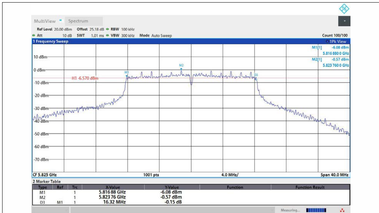
11A-Ant3-5825-PASS
