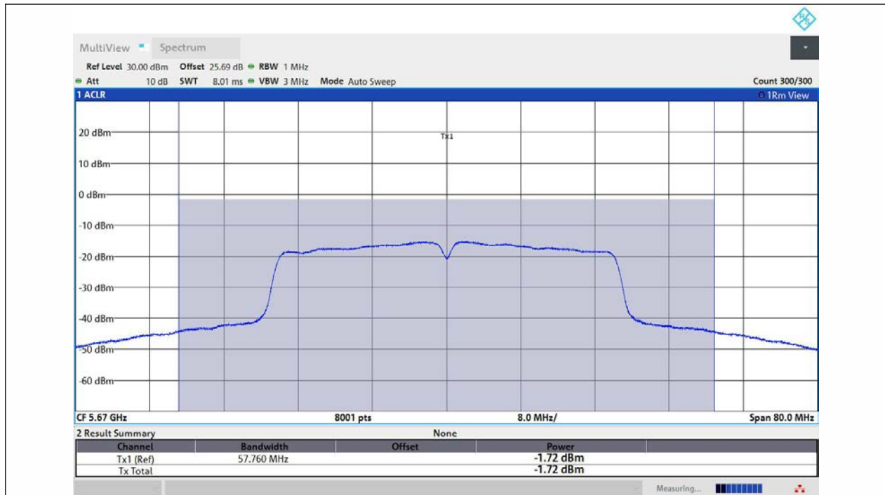
11N40MIMO-Ant2-5670-TPC_L-PASS
