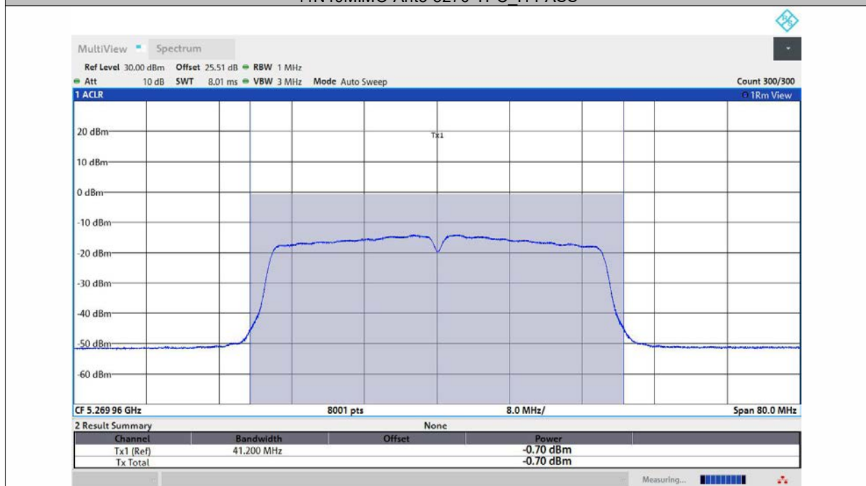
11N40MIMO-Ant1-5270-TPC_L-PASS
