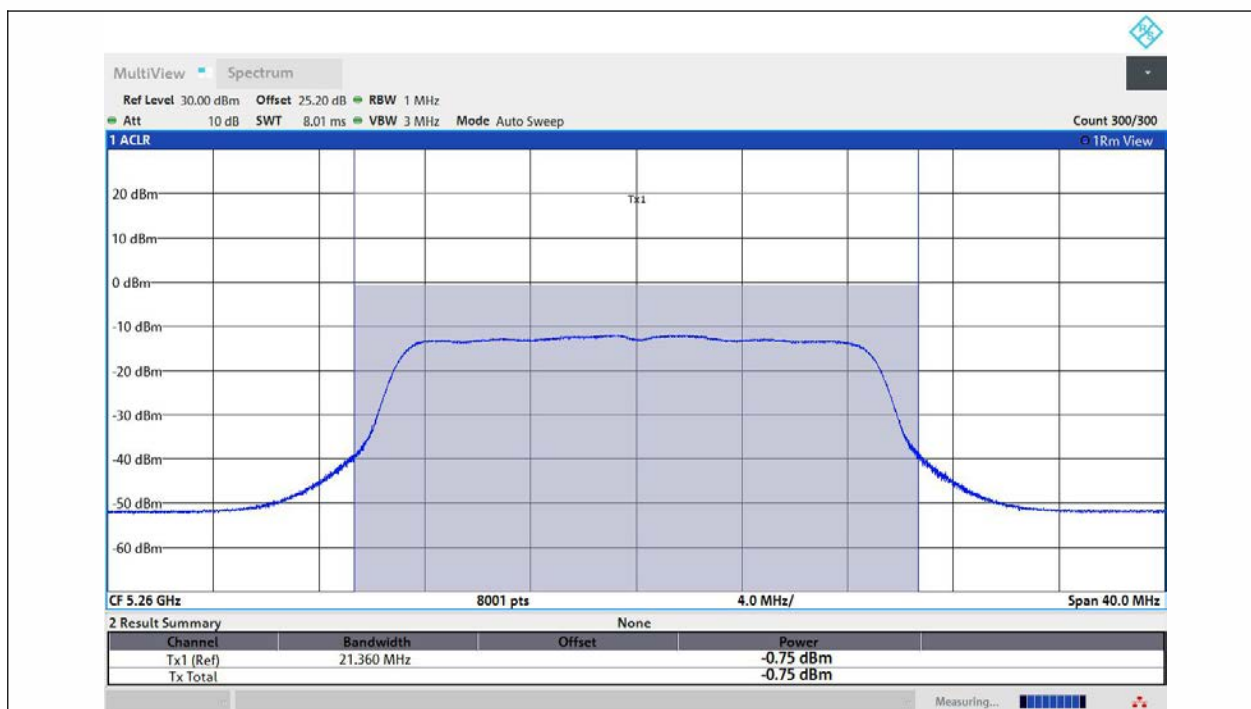
11N20MIMO-Ant1-5260-TPC_L-PASS
