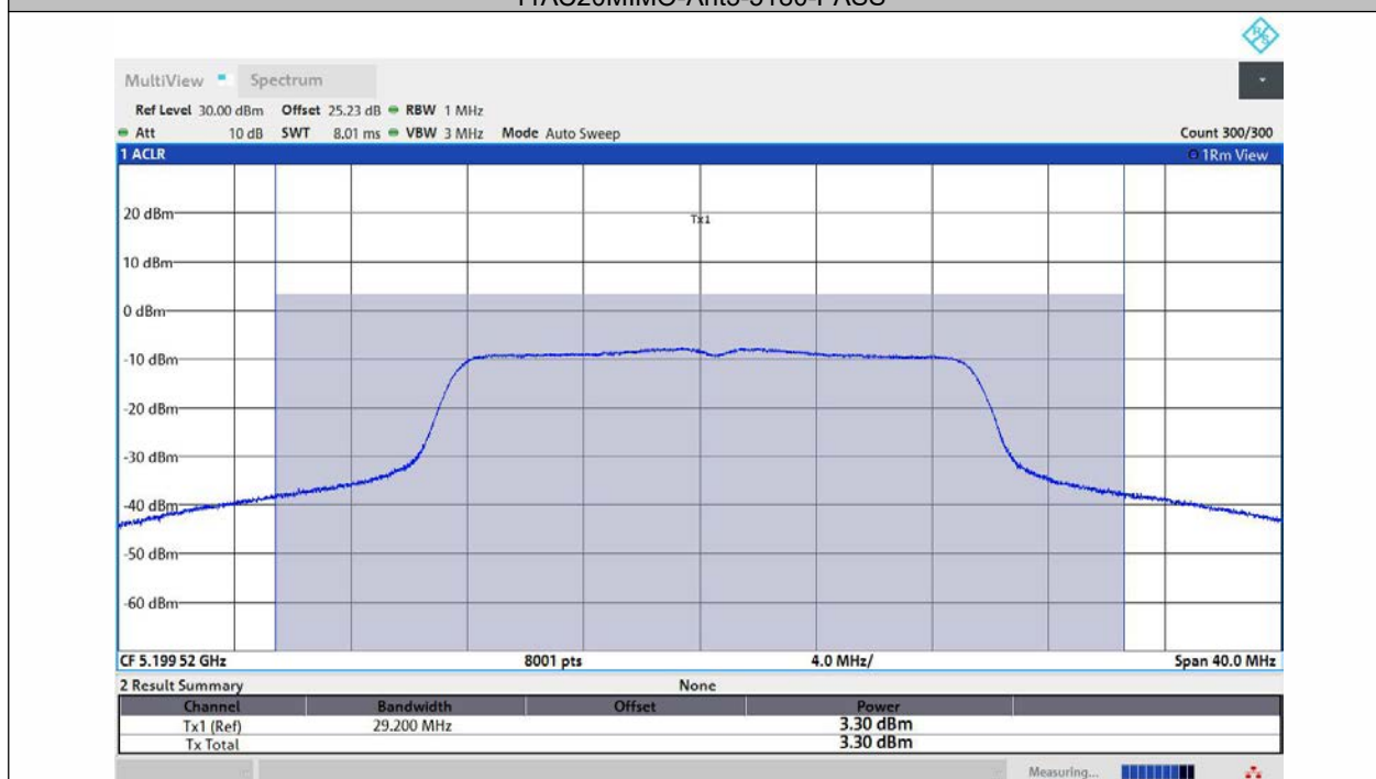
11AC20MIMO-Ant1-5200-PASS
