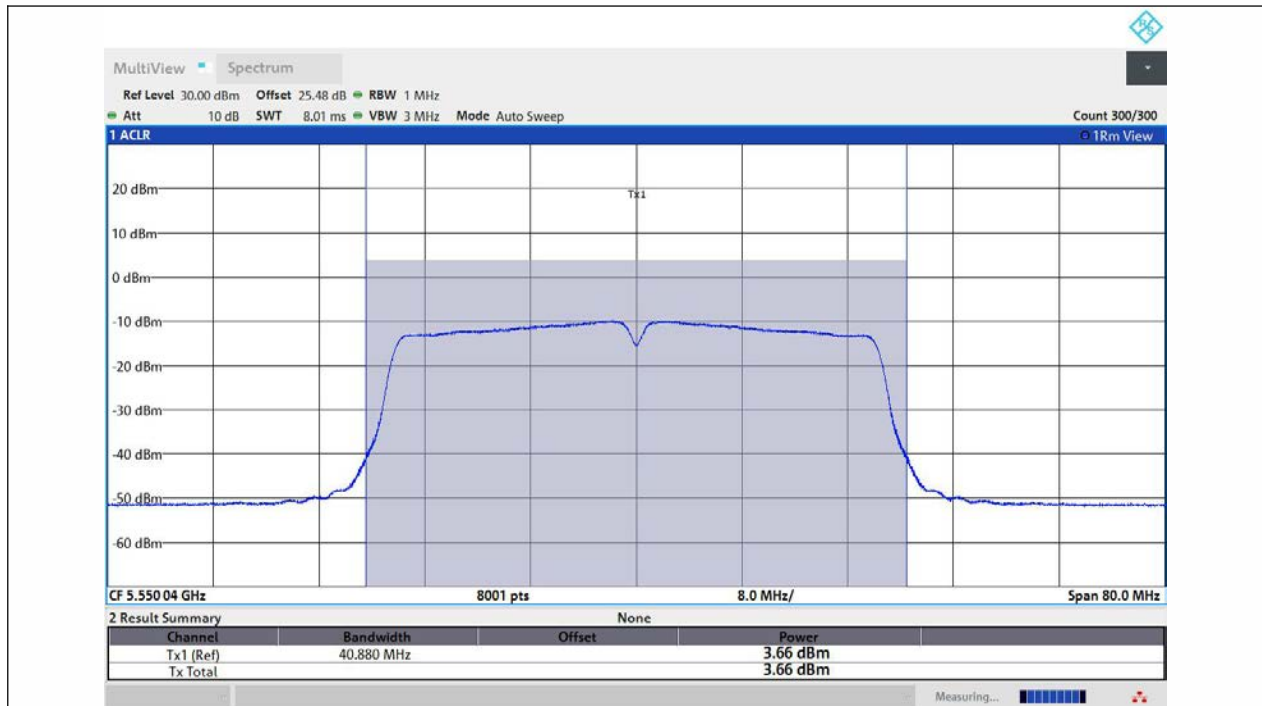
11N40MIMO-Ant3-5550-TPC_H-PASS
