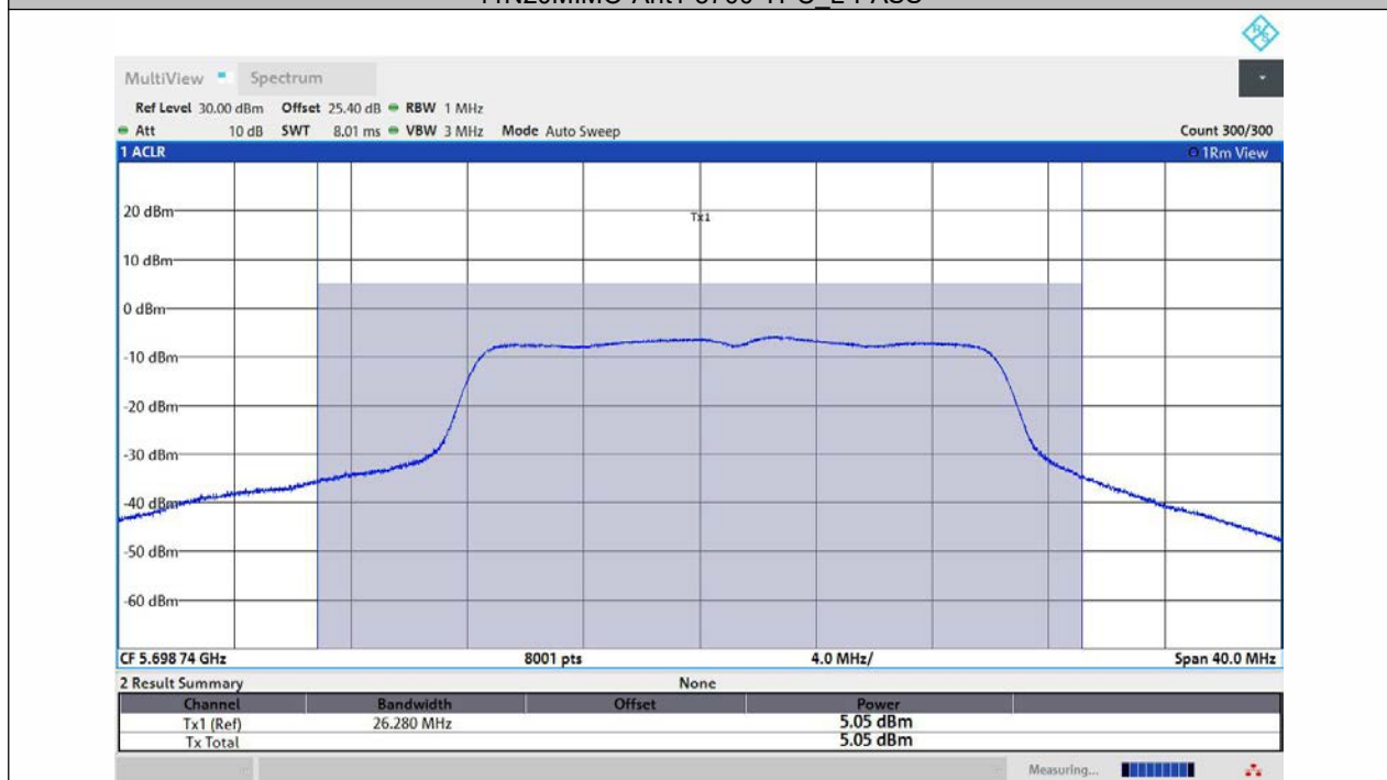
11N20MIMO-Ant2-5700-TPC_L-PASS
