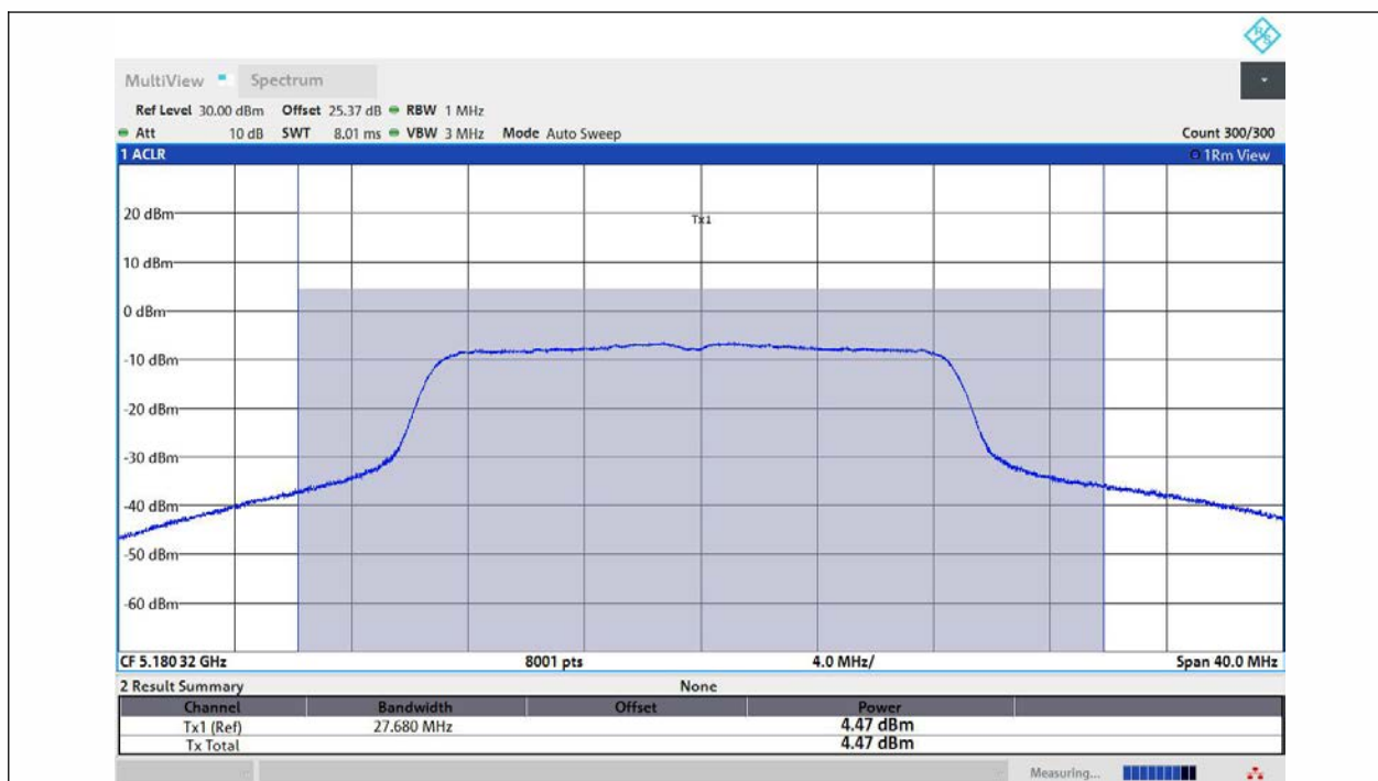
11AC20MIMO-Ant3-5180-PASS
