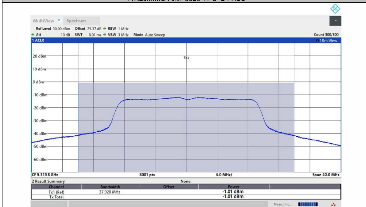
11N20MIMO-Ant2-5320-TPC_L-PASS
