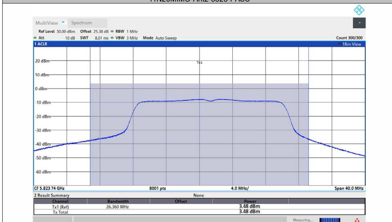
11N20MIMO-Ant3-5825-PASS
