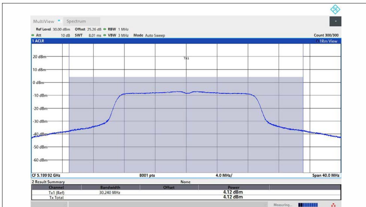
11AC20MIMO-Ant2-5200-PASS
