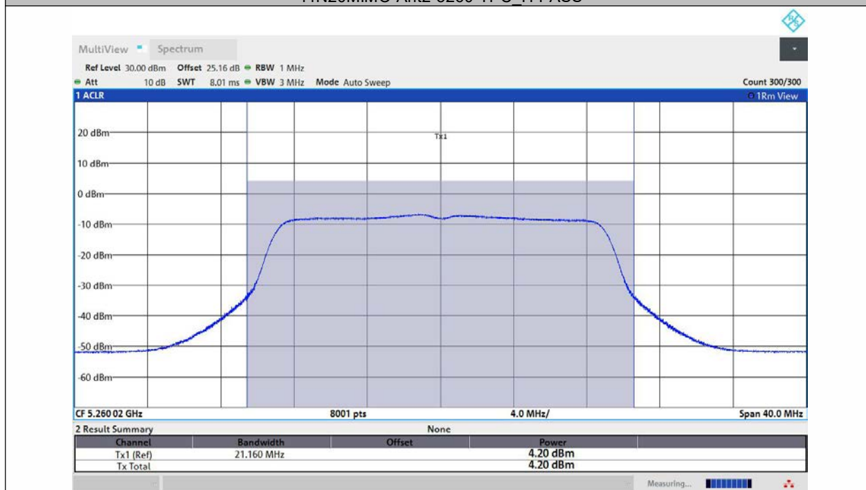
11N20MIMO-Ant3-5260-TPC_H-PASS
