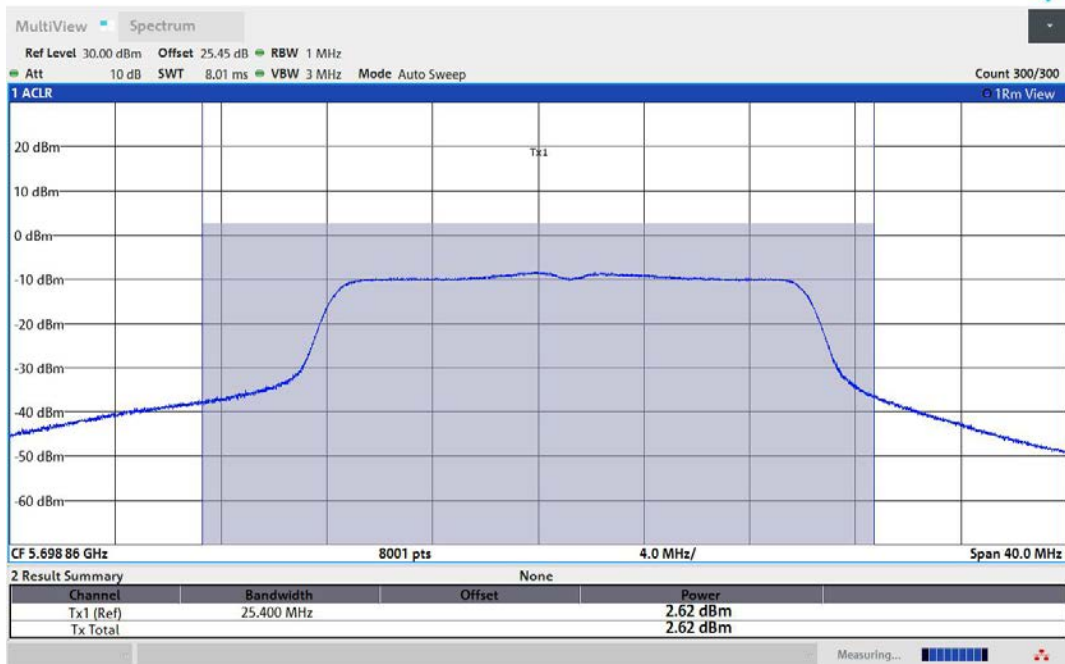
11N20MIMO-Ant3-5700-TPC_H-PASS
