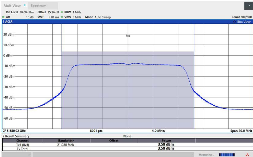
11N20MIMO-Ant3-5580-TPC_H-PASS
