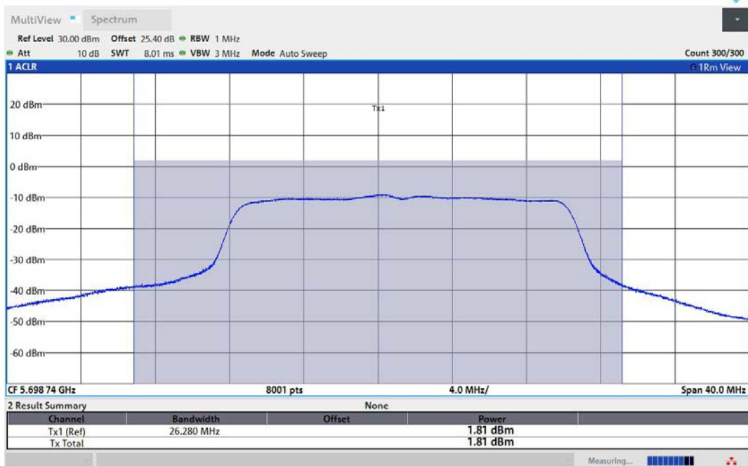
11N20MIMO-Ant2-5700-TPC_H-PASS
