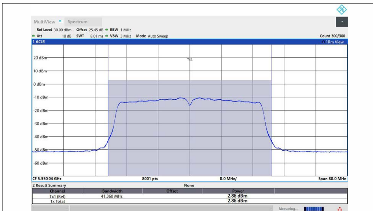
11N40MIMO-Ant1-5550-TPC_H-PASS
