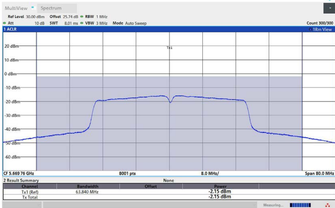
11N40MIMO-Ant1-5670-TPC_L-PASS
