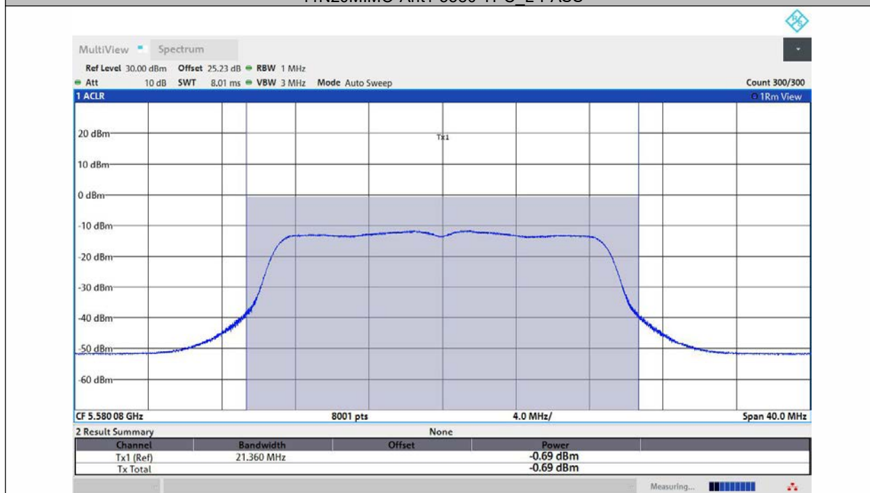
11N20MIMO-Ant2-5580-TPC_L-PASS
