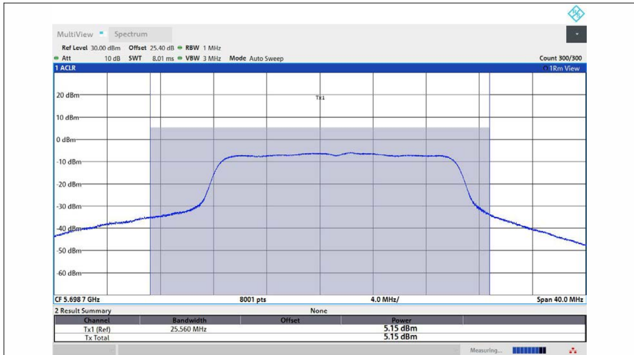
11N20MIMO-Ant1-5700-TPC_L-PASS
