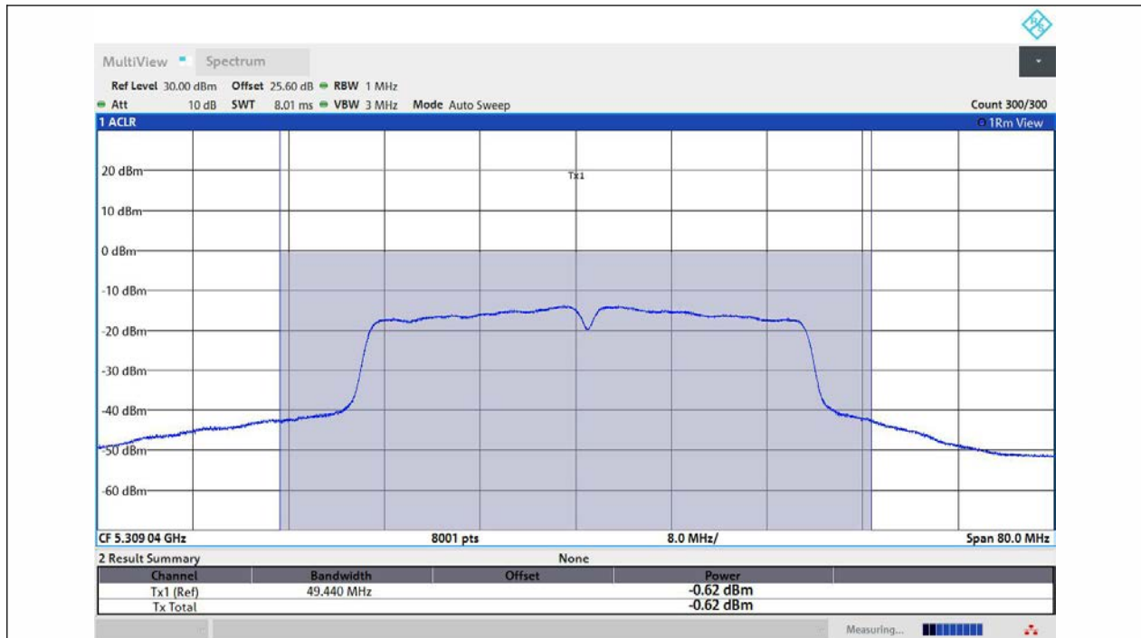
11N40MIMO-Ant2-5310-TPC_L-PASS
