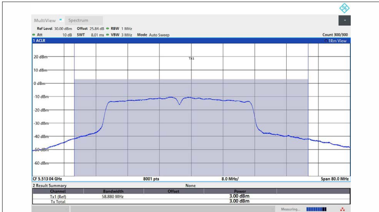
11N40MIMO-Ant1-5510-TPC_H-PASS
