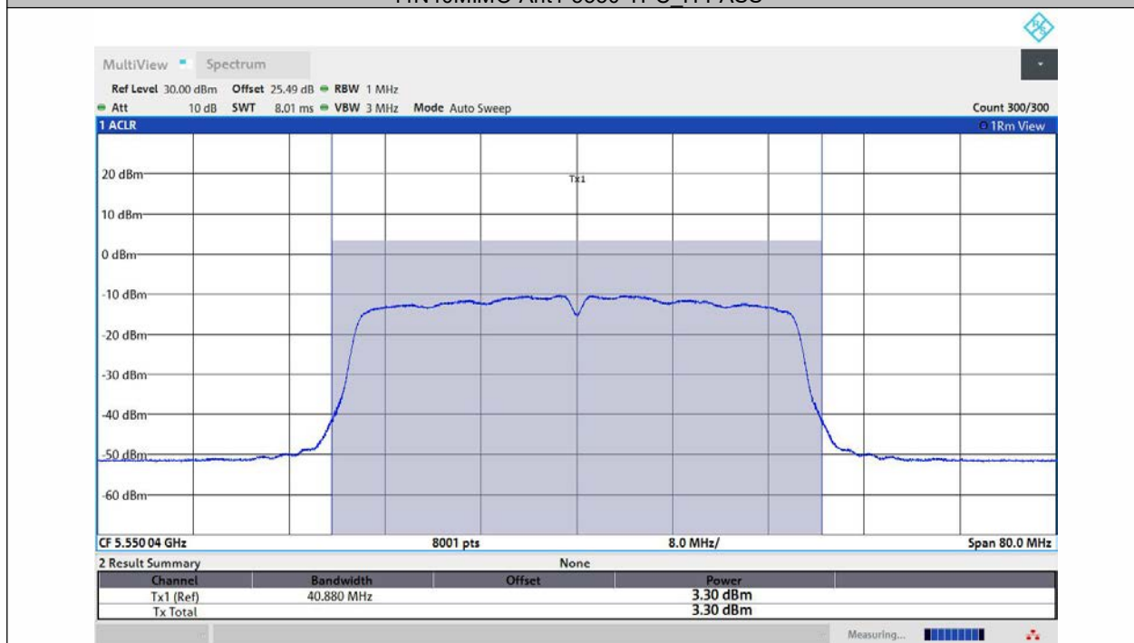
11N40MIMO-Ant2-5550-TPC_H-PASS
