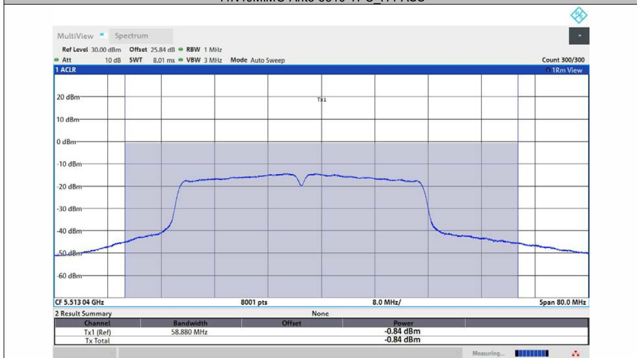
11N40MIMO-Ant1-5510-TPC_L-PASS
