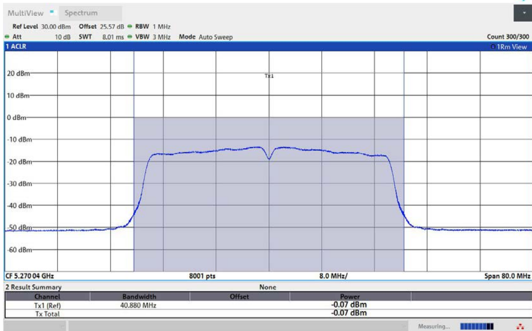
11N40MIMO-Ant2-5270-TPC_L-PASS
