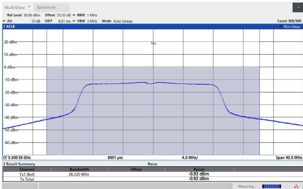
11N20MIMO-Ant3-5500-TPC_L-PASS
