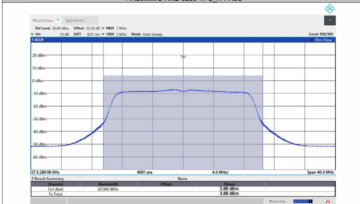
11N20MIMO-Ant3-5280-TPC_H-PASS
