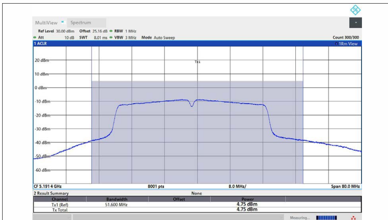
11N40MIMO-Ant3-5190-PASS
