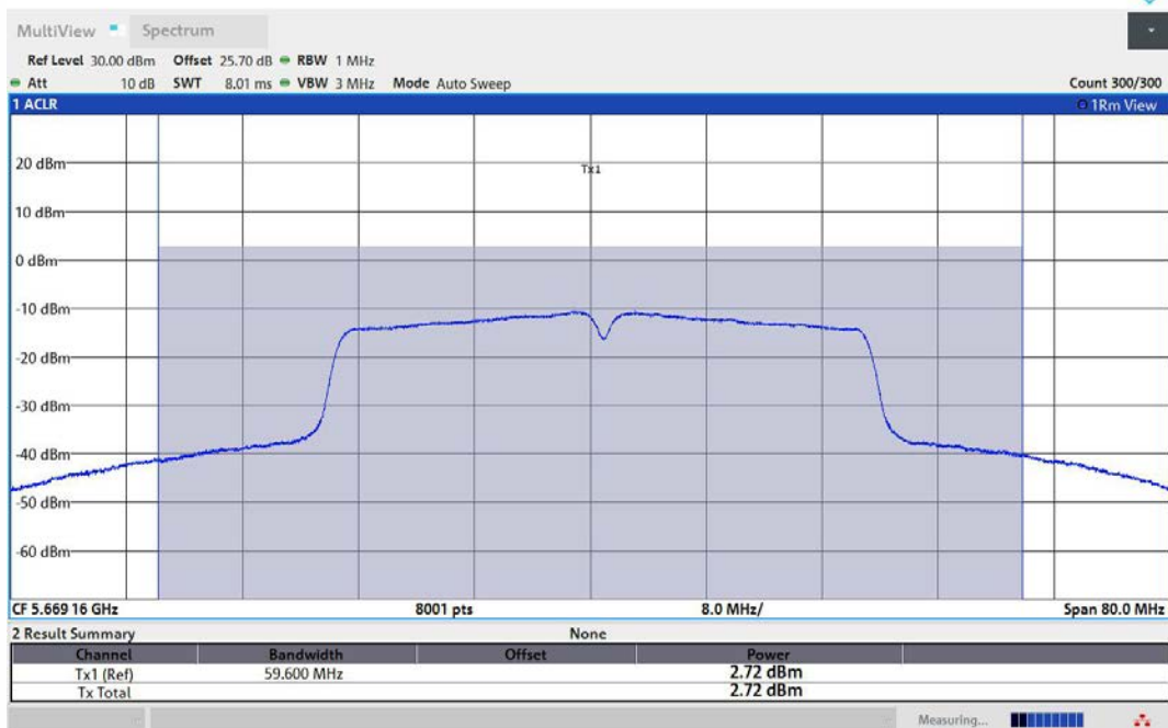
11N40MIMO-Ant3-5670-TPC_H-PASS
