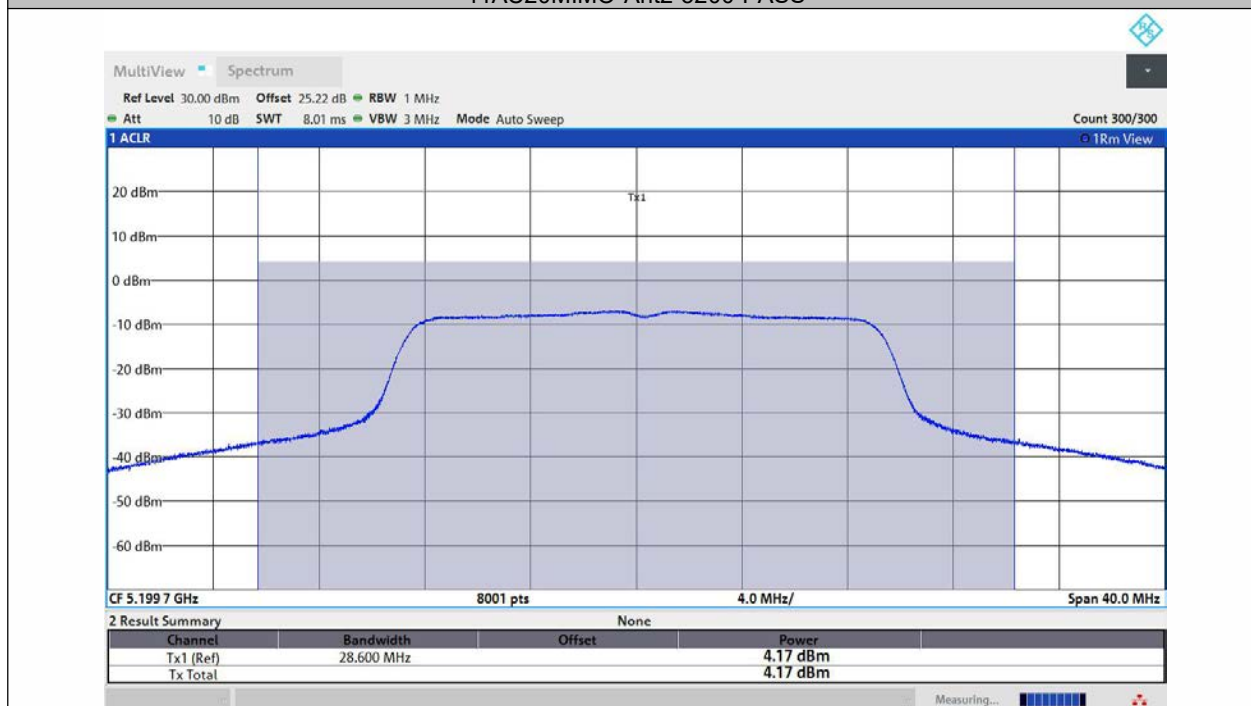
11AC20MIMO-Ant3-5200-PASS
