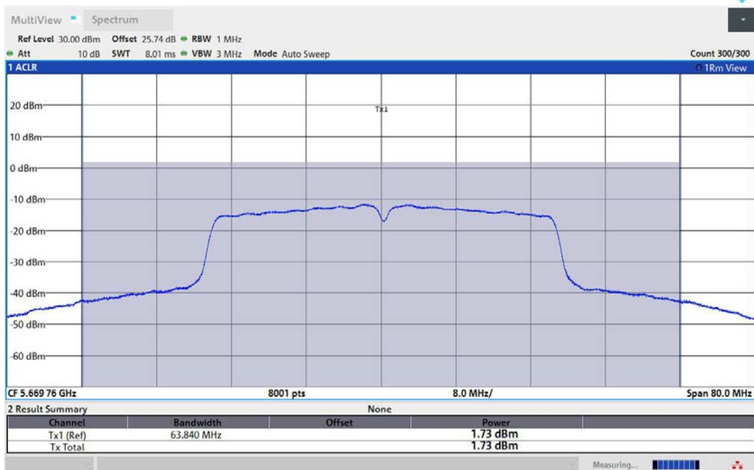
11N40MIMO-Ant1-5670-TPC_H-PASS
