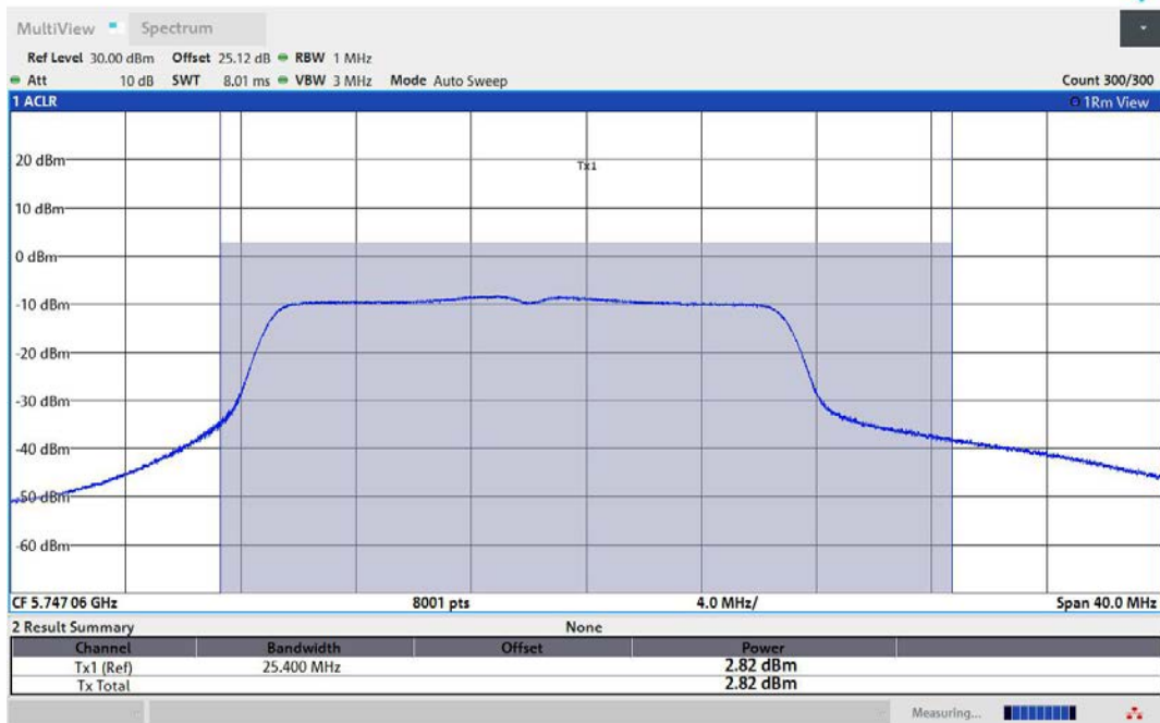
11N20MIMO-Ant3-5745-PASS
