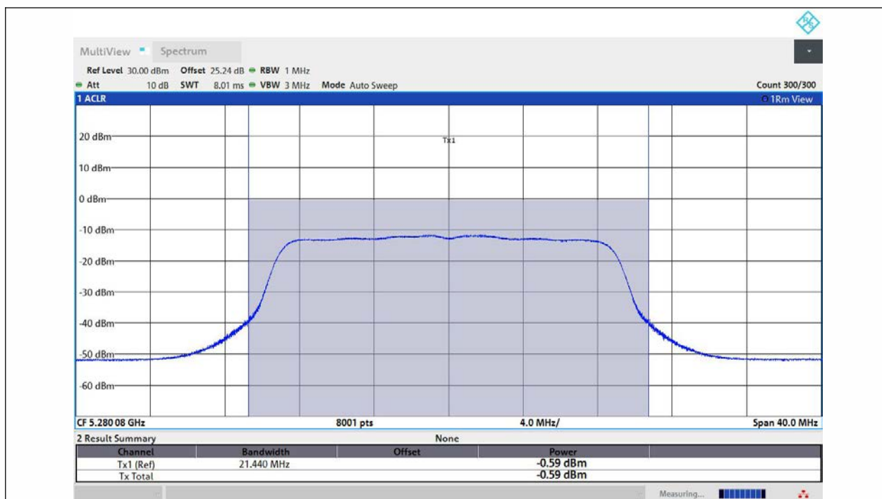
11N20MIMO-Ant1-5280-TPC_L-PASS
