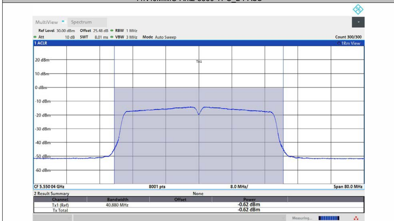
11N40MIMO-Ant3-5550-TPC_L-PASS
