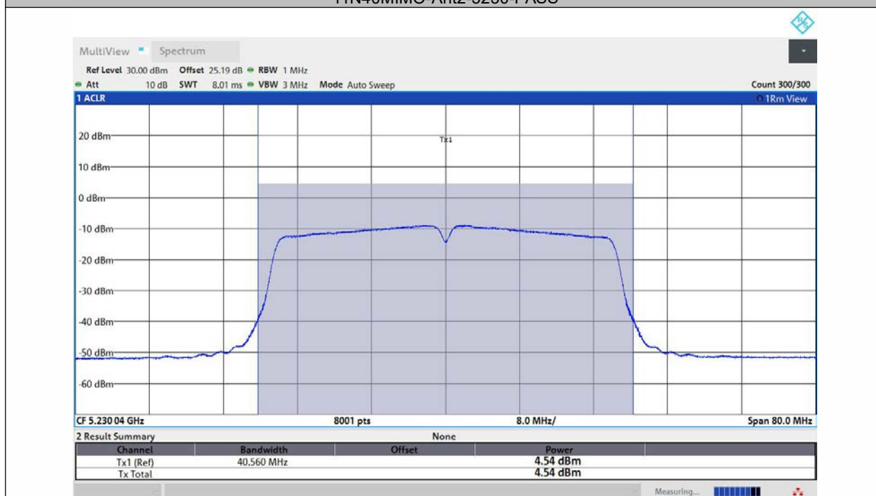
11N40MIMO-Ant3-5230-PASS
