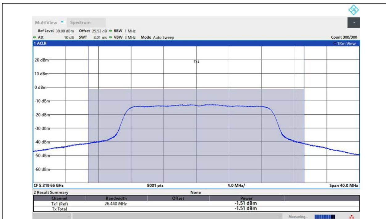
11N20MIMO-Ant1-5320-TPC_L-PASS
