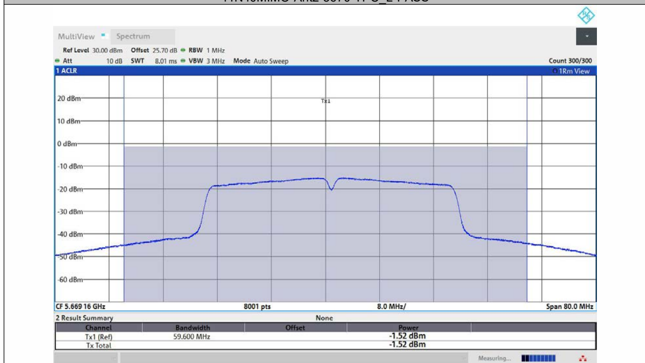
11N40MIMO-Ant3-5670-TPC_L-PASS
