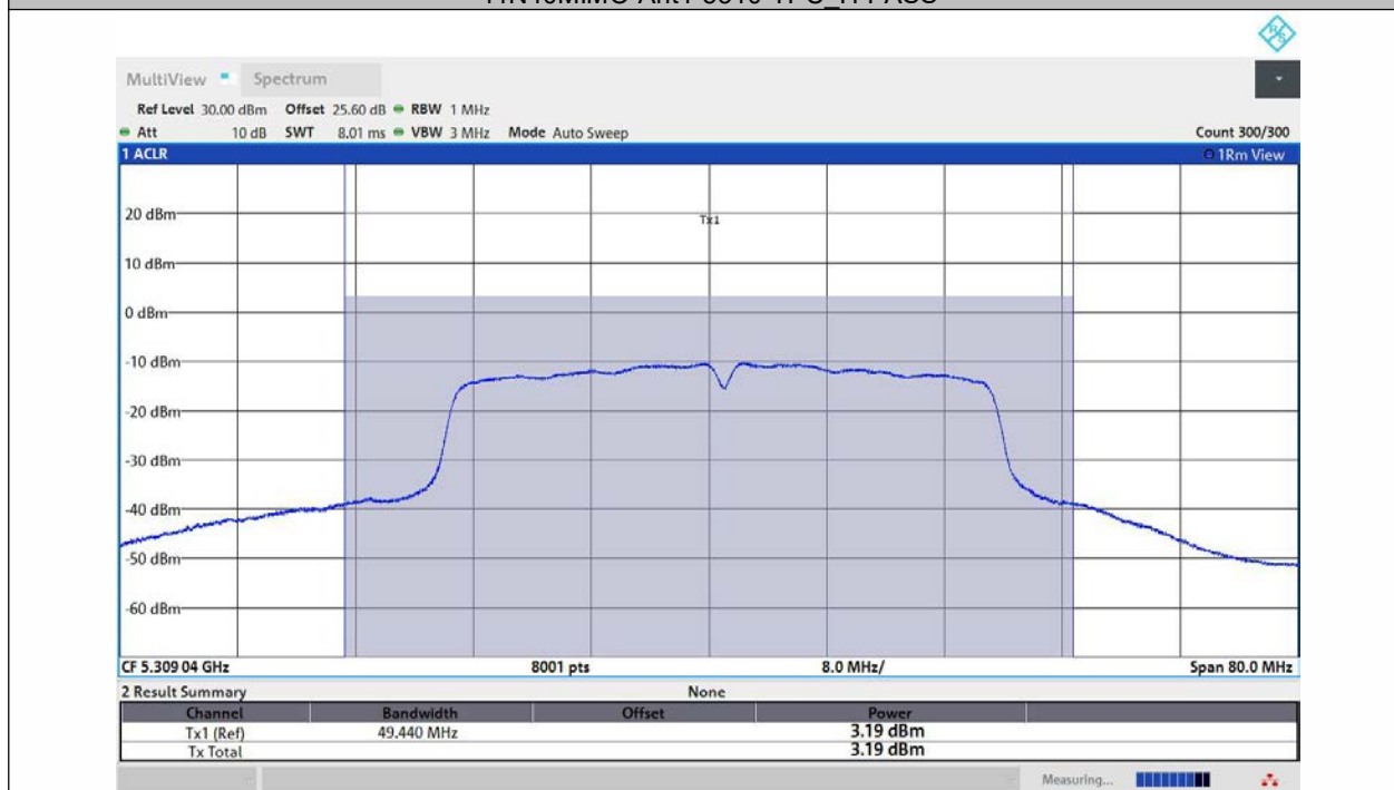
11N40MIMO-Ant2-5310-TPC_H-PASS
