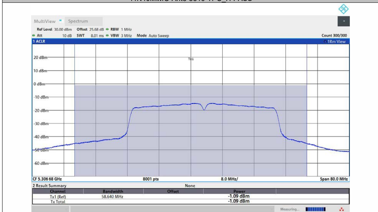
11N40MIMO-Ant1-5310-TPC_L-PASS
