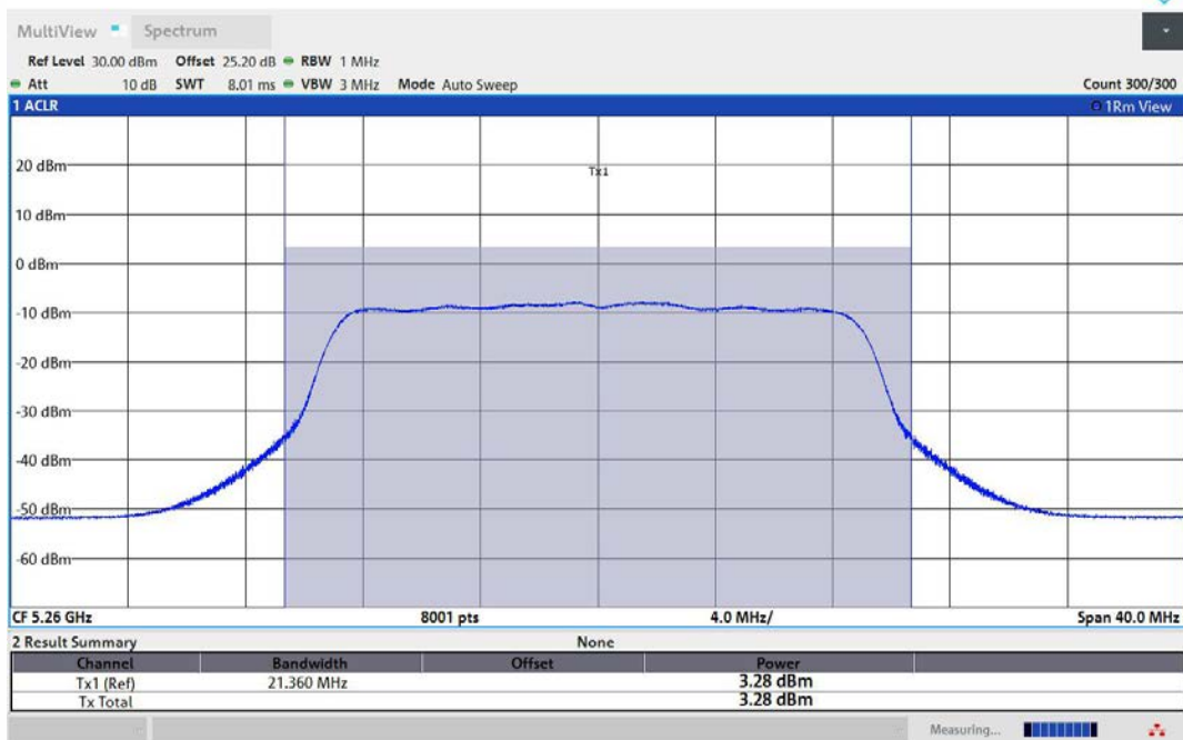
11N20MIMO-Ant1-5260-TPC_H-PASS
