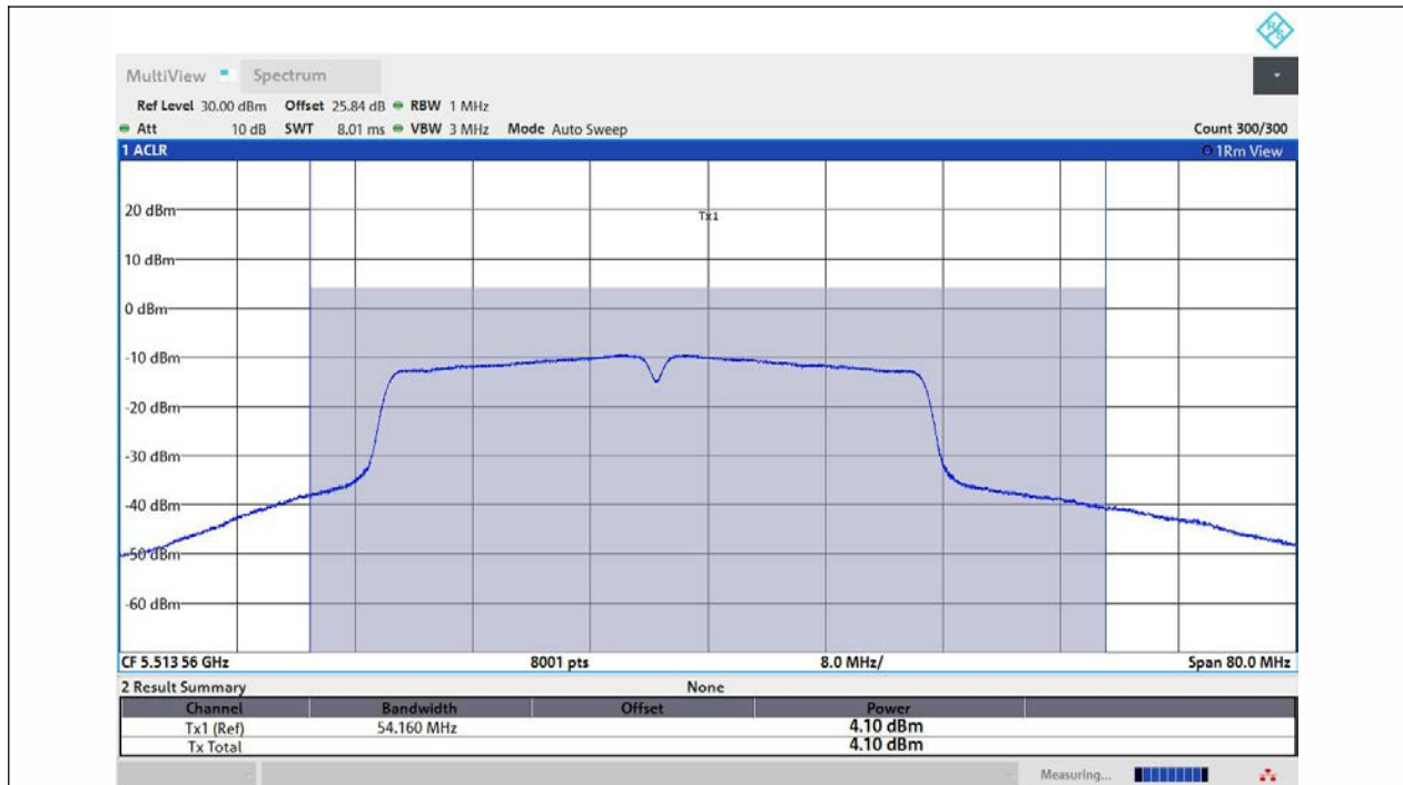
11N40MIMO-Ant3-5510-TPC_H-PASS
