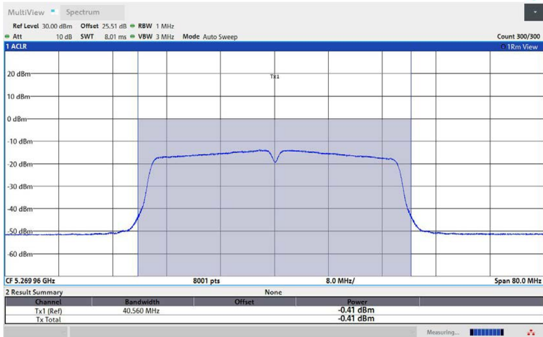
11N40MIMO-Ant3-5270-TPC_L-PASS
