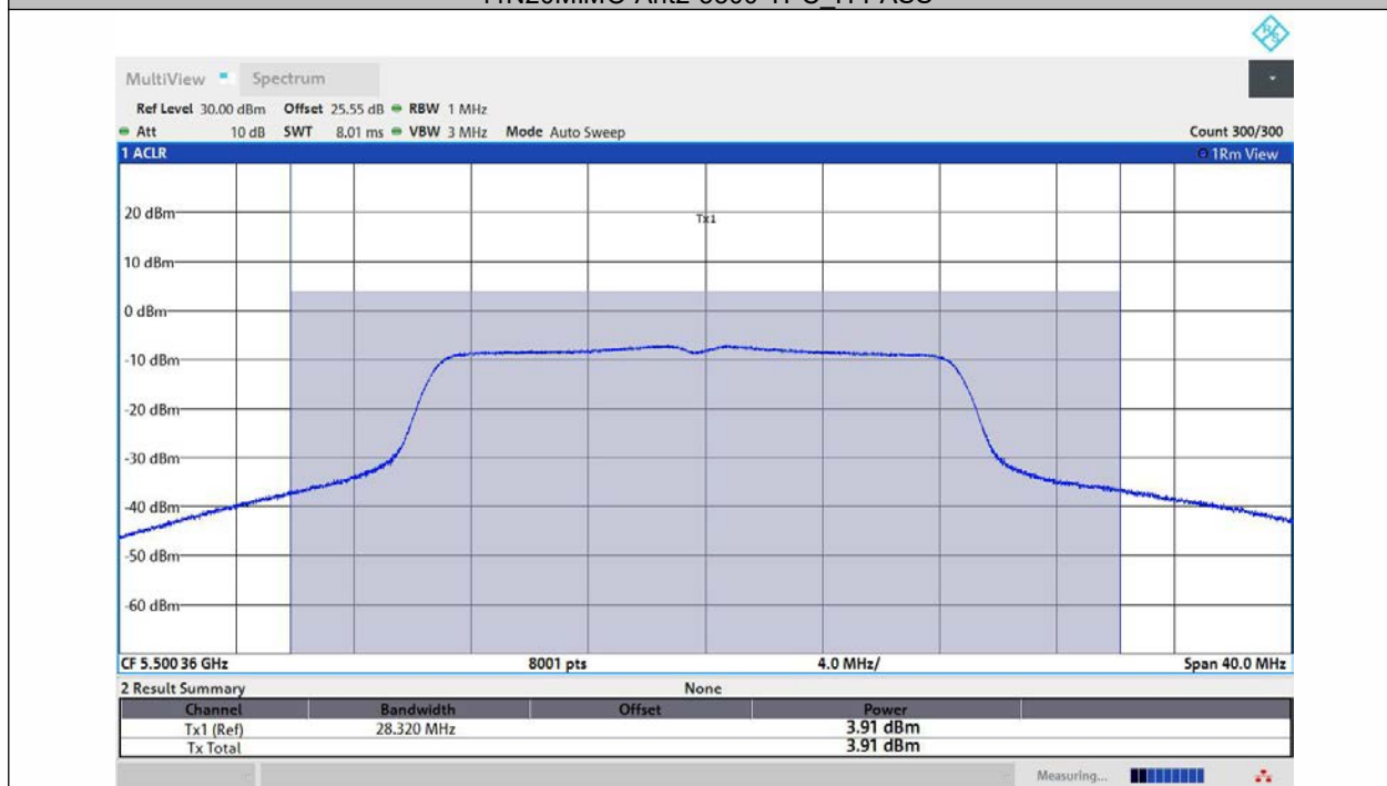
11N20MIMO-Ant3-5500-TPC_H-PASS
