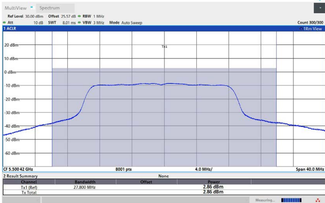
11N20MIMO-Ant1-5500-TPC_H-PASS
