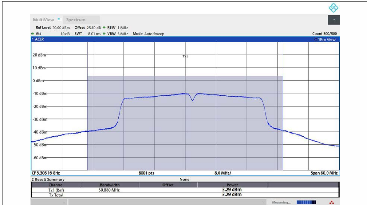
11N40MIMO-Ant3-5310-TPC_H-PASS
