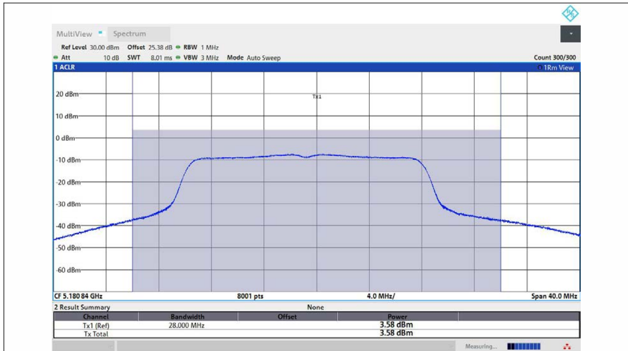
11AC20MIMO-Ant1-5180-PASS
