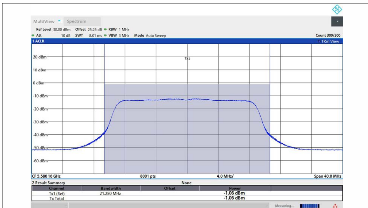
11N20MIMO-Ant1-5580-TPC_L-PASS
