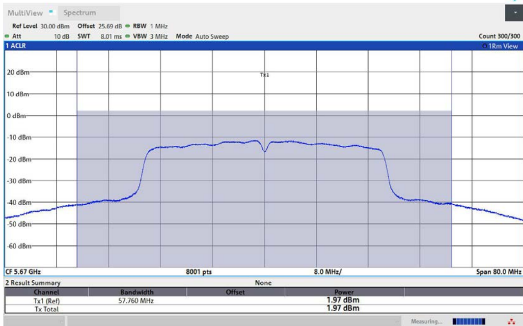
11N40MIMO-Ant2-5670-TPC_H-PASS
