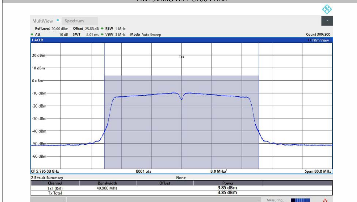
11N40MIMO-Ant3-5795-PASS
