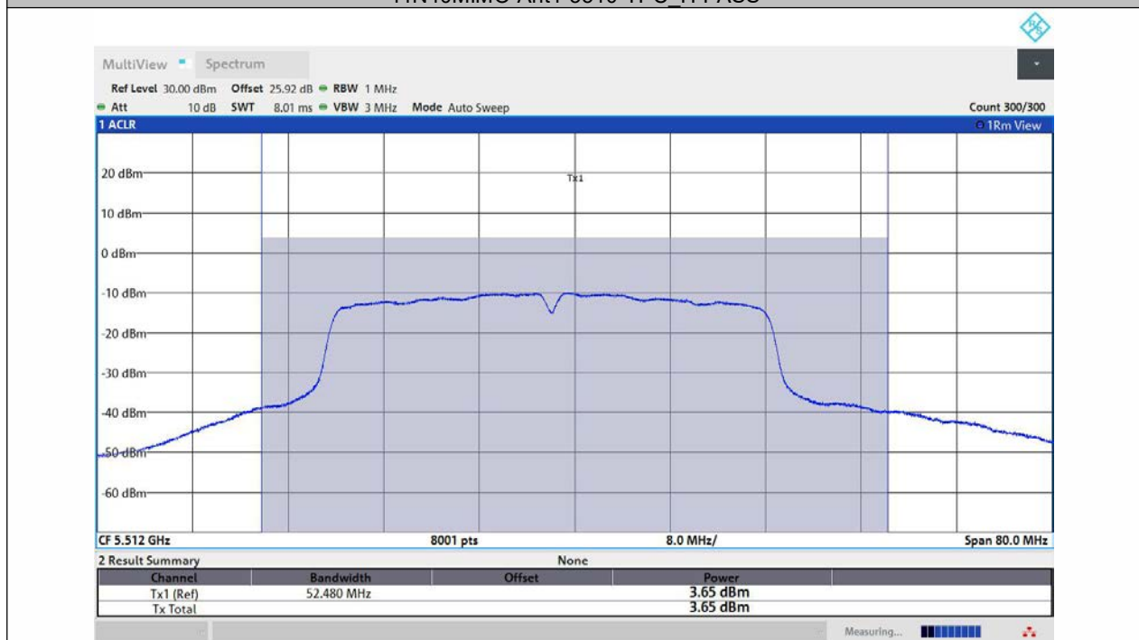
11N40MIMO-Ant2-5510-TPC_H-PASS
