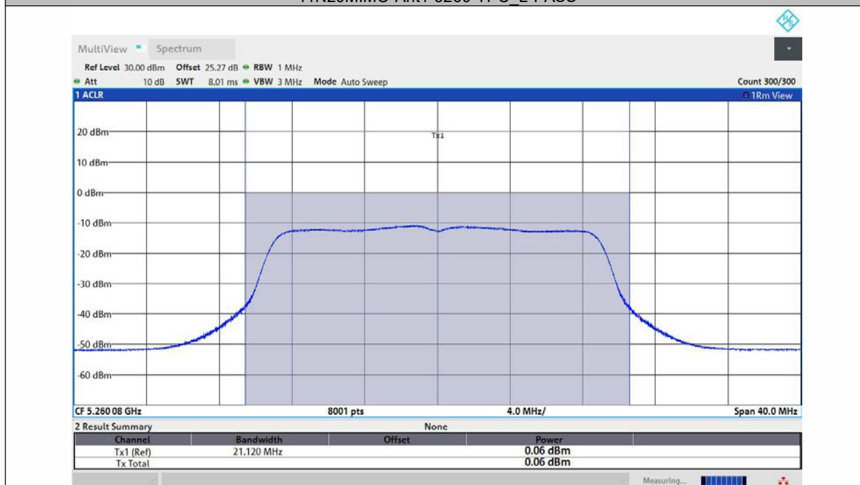
11N20MIMO-Ant2-5260-TPC_L-PASS
