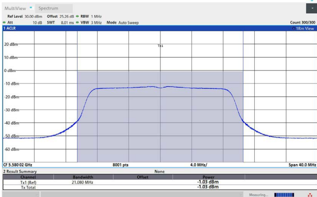
11N20MIMO-Ant3-5580-TPC_L-PASS
