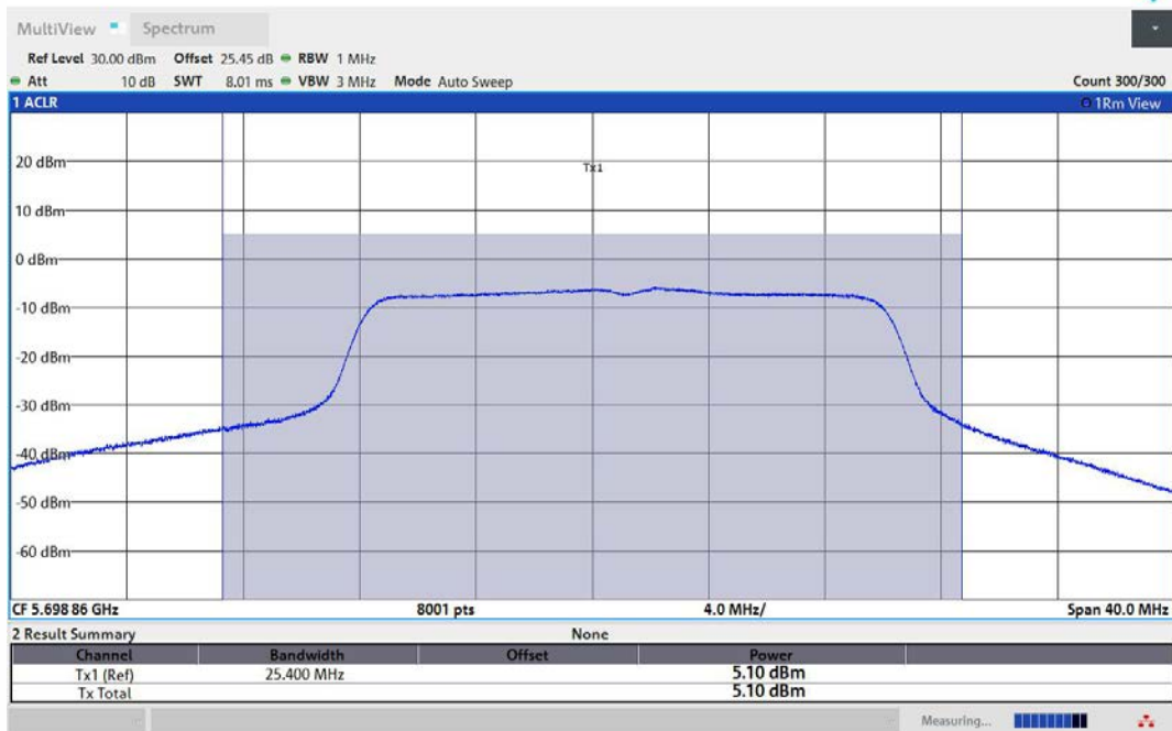
11N20MIMO-Ant3-5700-TPC_L-PASS
