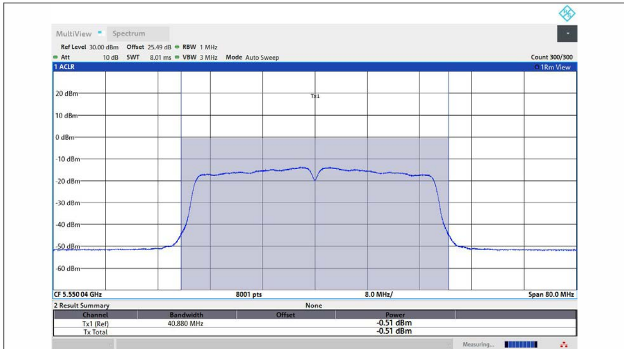
11N40MIMO-Ant2-5550-TPC_L-PASS
