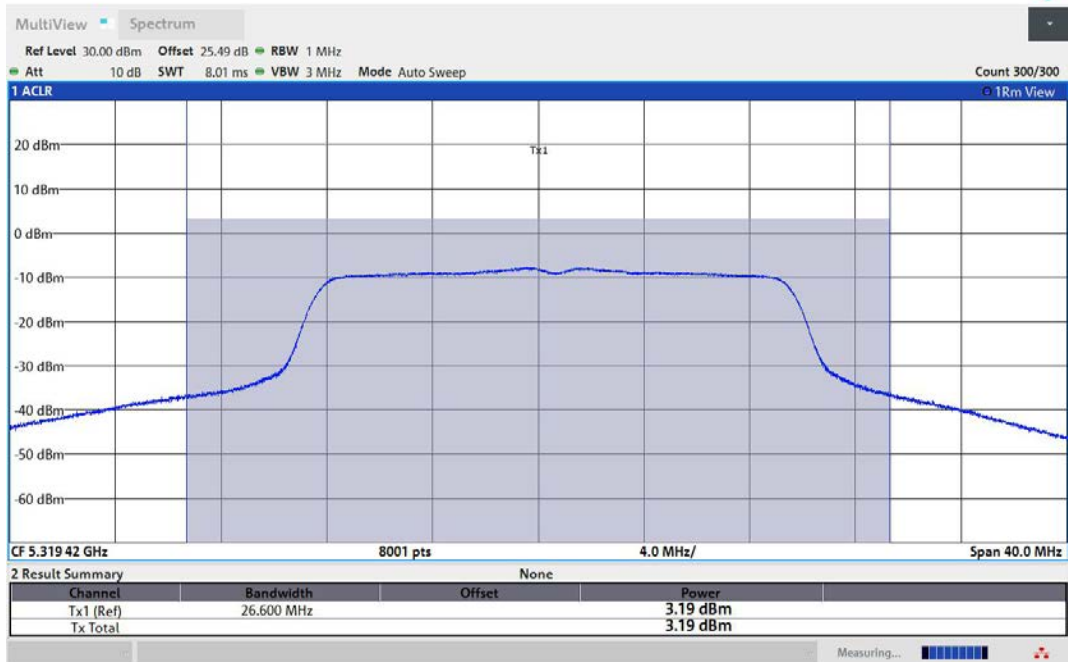
11N20MIMO-Ant3-5320-TPC_H-PASS
