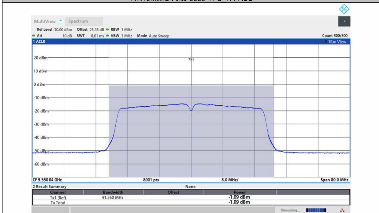
11N40MIMO-Ant1-5550-TPC_L-PASS
