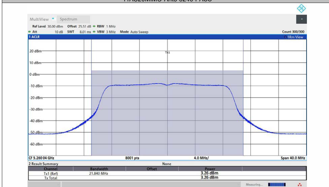
11AC20MIMO-Ant1-5260-TPC_H-PASS
