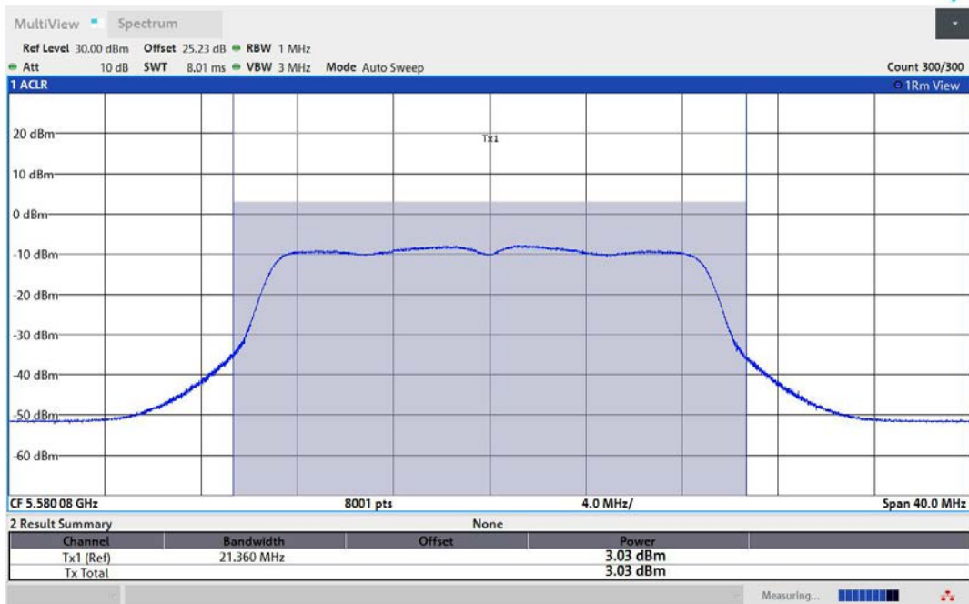
11N20MIMO-Ant2-5580-TPC_H-PASS
