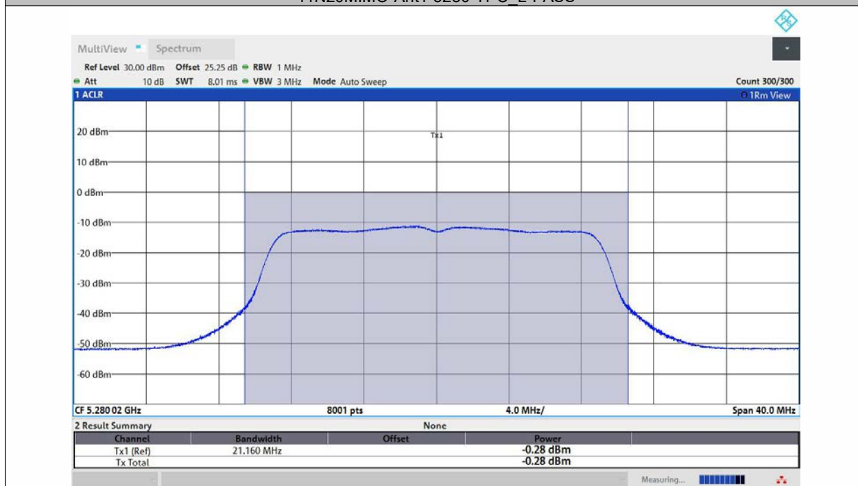
11N20MIMO-Ant2-5280-TPC_L-PASS
