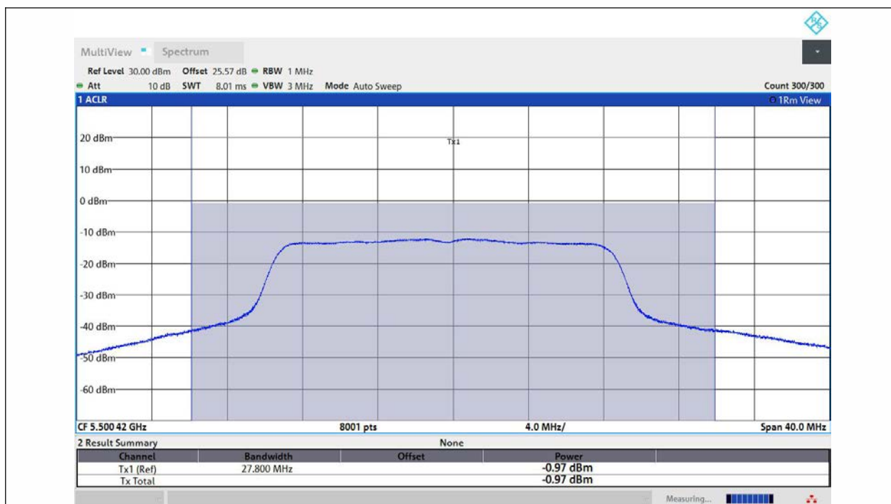
11N20MIMO-Ant1-5500-TPC_L-PASS
