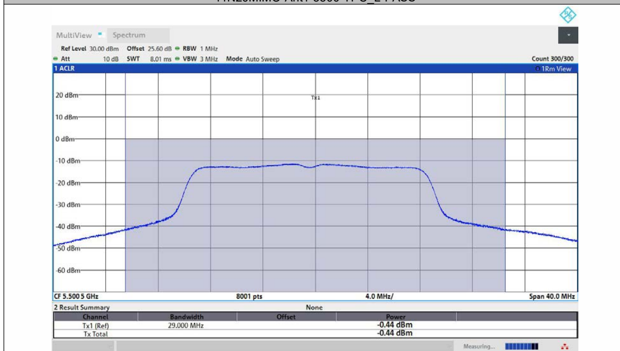
11N20MIMO-Ant2-5500-TPC_L-PASS
