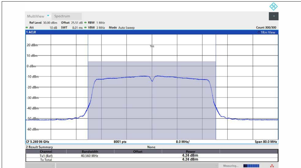
11N40MIMO-Ant3-5270-TPC_H-PASS
