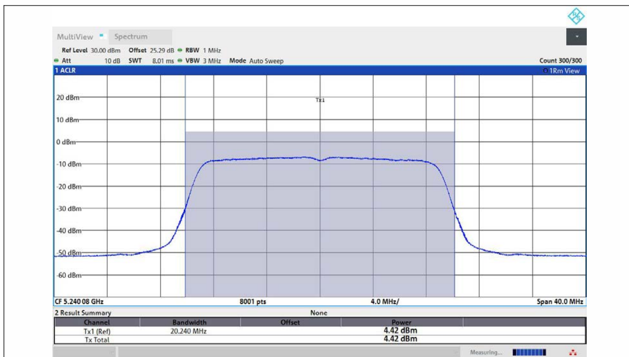
11AC20MIMO-Ant3-5240-PASS
