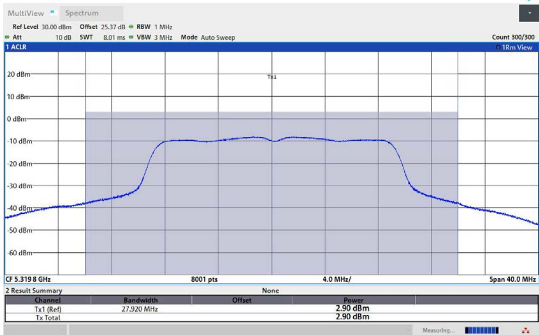
11N20MIMO-Ant2-5320-TPC_H-PASS
