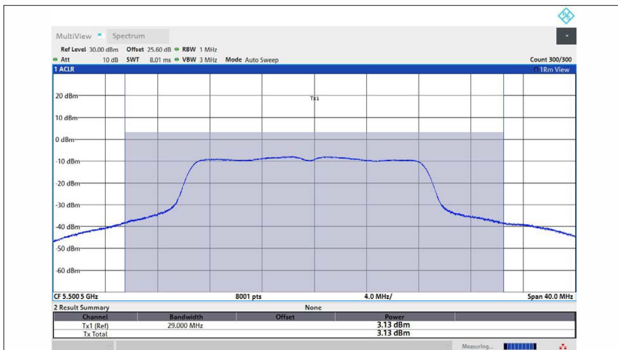
11N20MIMO-Ant2-5500-TPC_H-PASS
