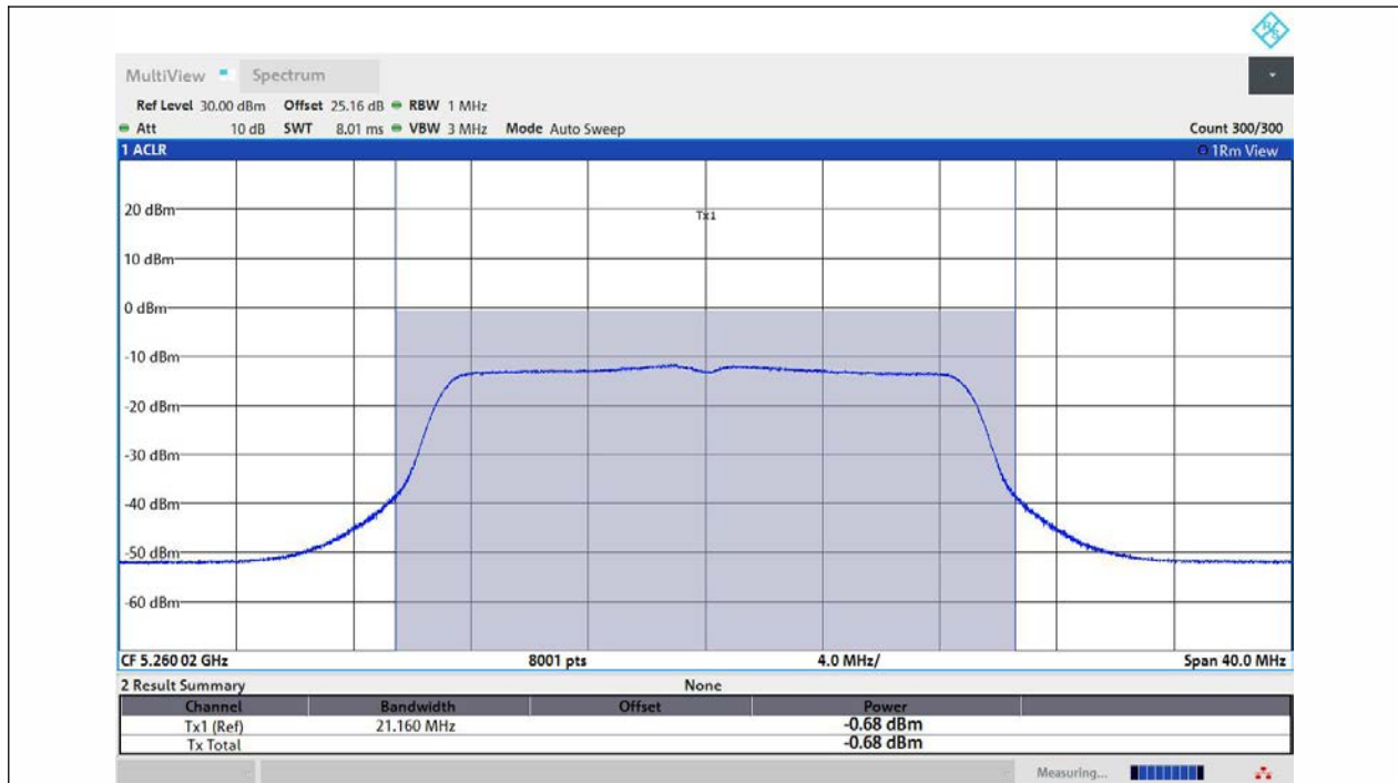
11N20MIMO-Ant3-5260-TPC_L-PASS
