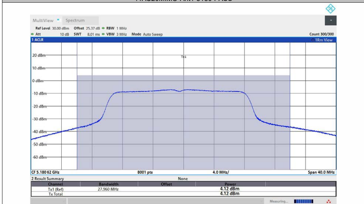
11AC20MIMO-Ant2-5180-PASS
