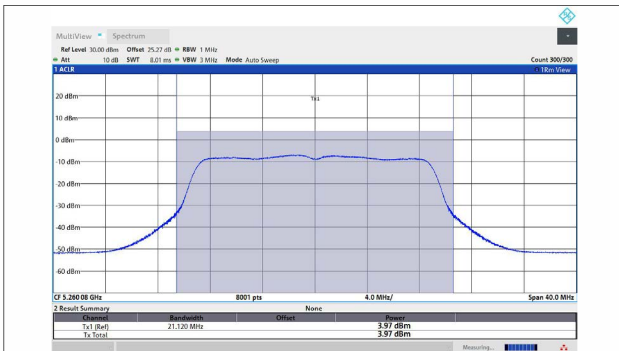
11N20MIMO-Ant2-5260-TPC_H-PASS
