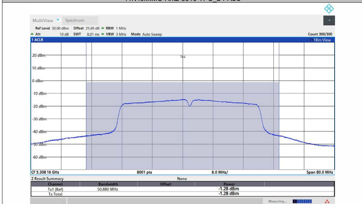
11N40MIMO-Ant3-5310-TPC_L-PASS
