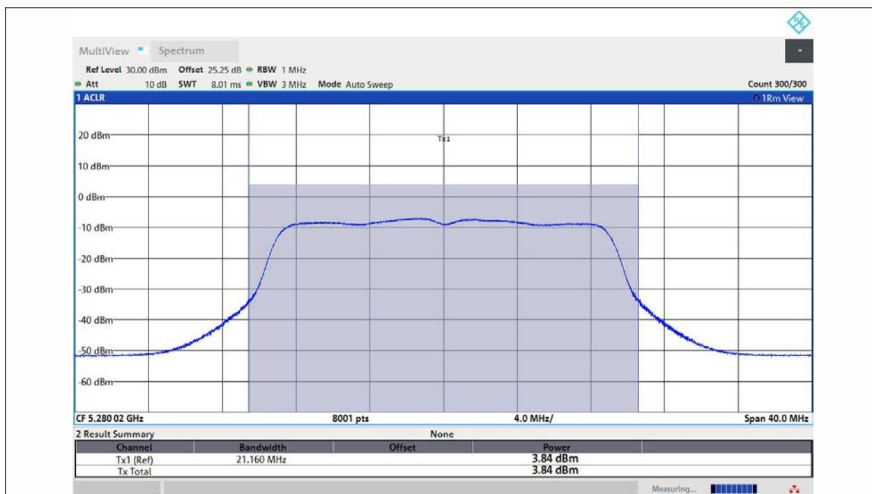
11N20MIMO-Ant2-5280-TPC_H-PASS
