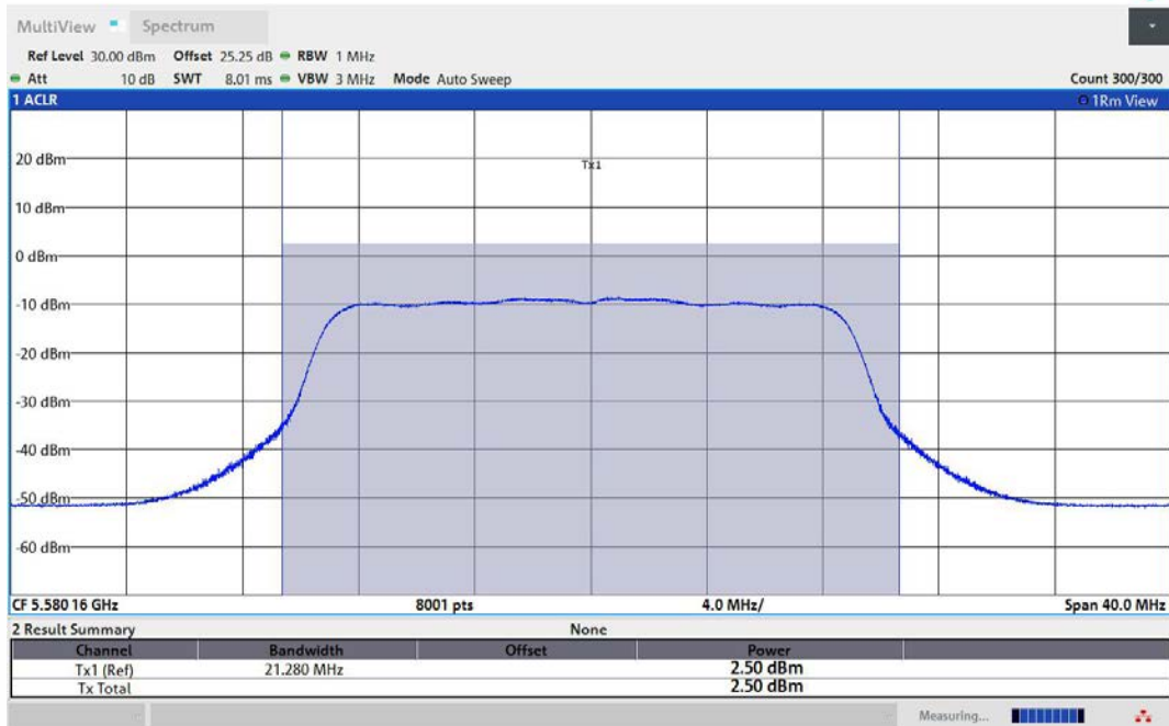
11N20MIMO-Ant1-5580-TPC_H-PASS
