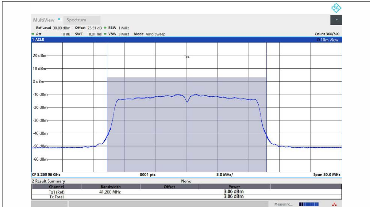
11N40MIMO-Ant1-5270-TPC_H-PASS
