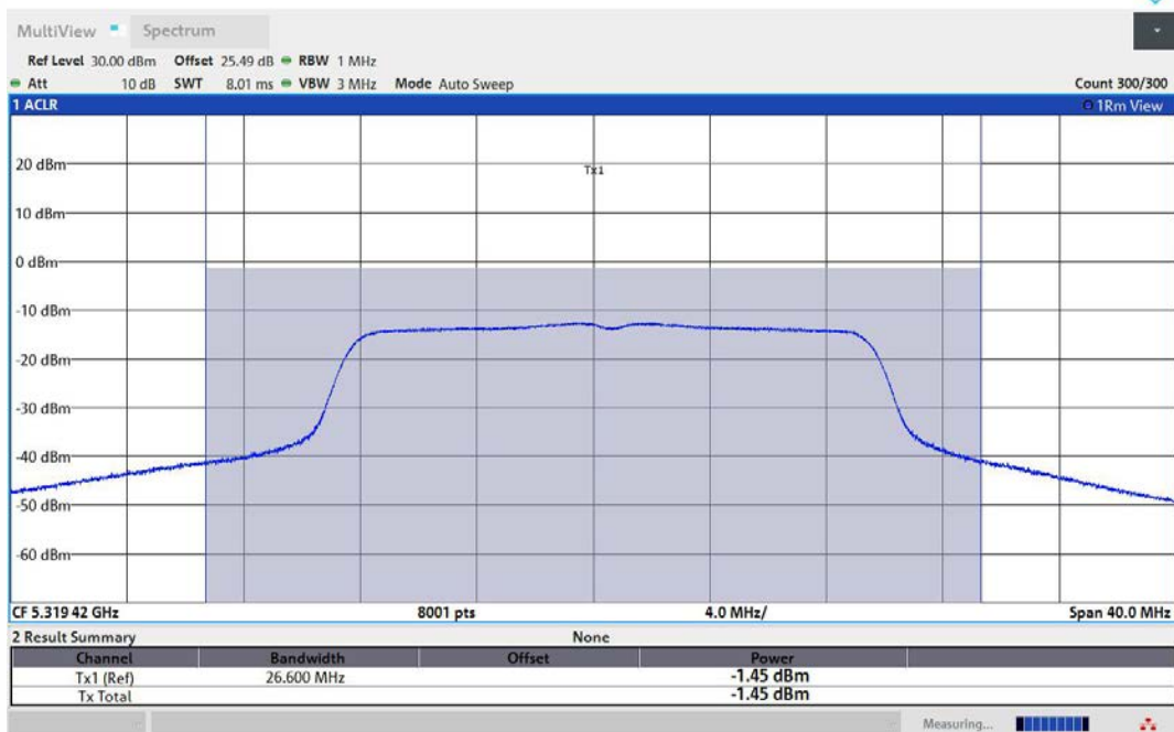
11N20MIMO-Ant3-5320-TPC_L-PASS
