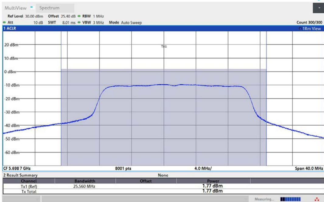
11N20MIMO-Ant1-5700-TPC_H-PASS
