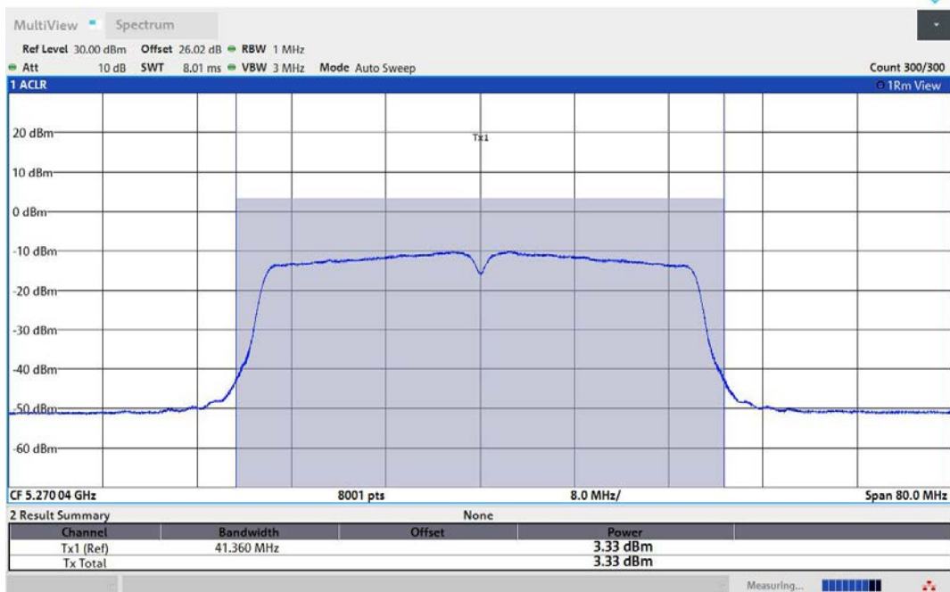
11AC40MIMO-Ant1-5270-TPC_H-PASS
