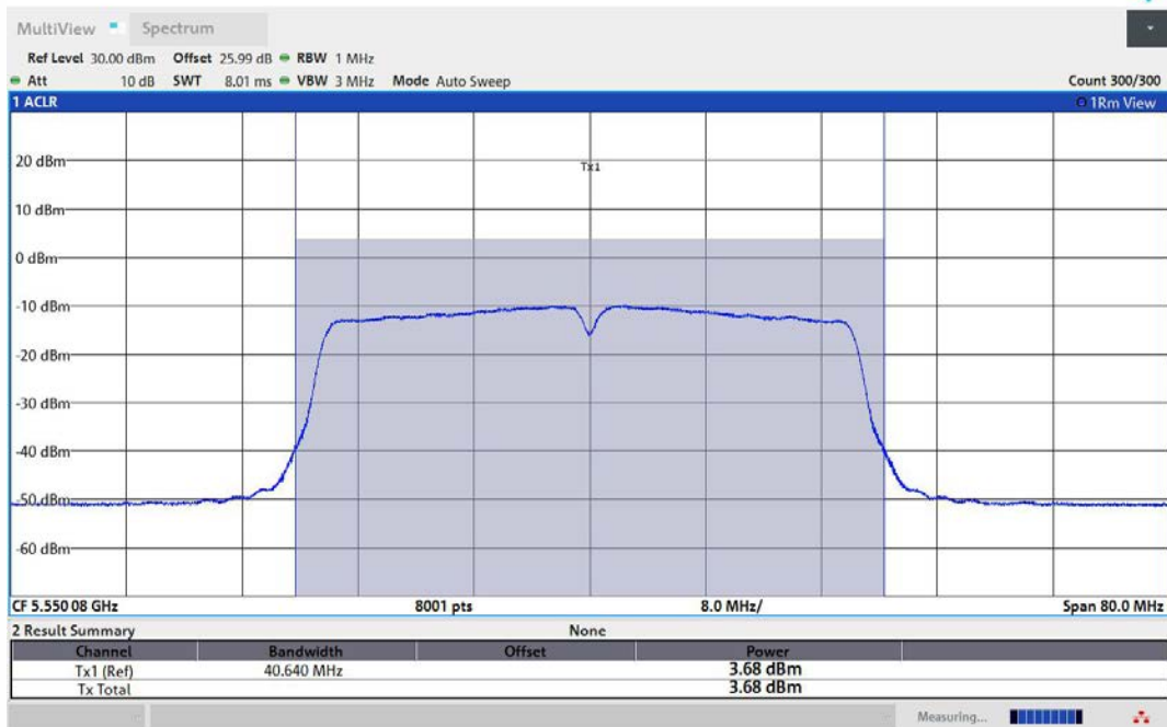
11AC40MIMO-Ant3-5550-TPC_H-PASS
