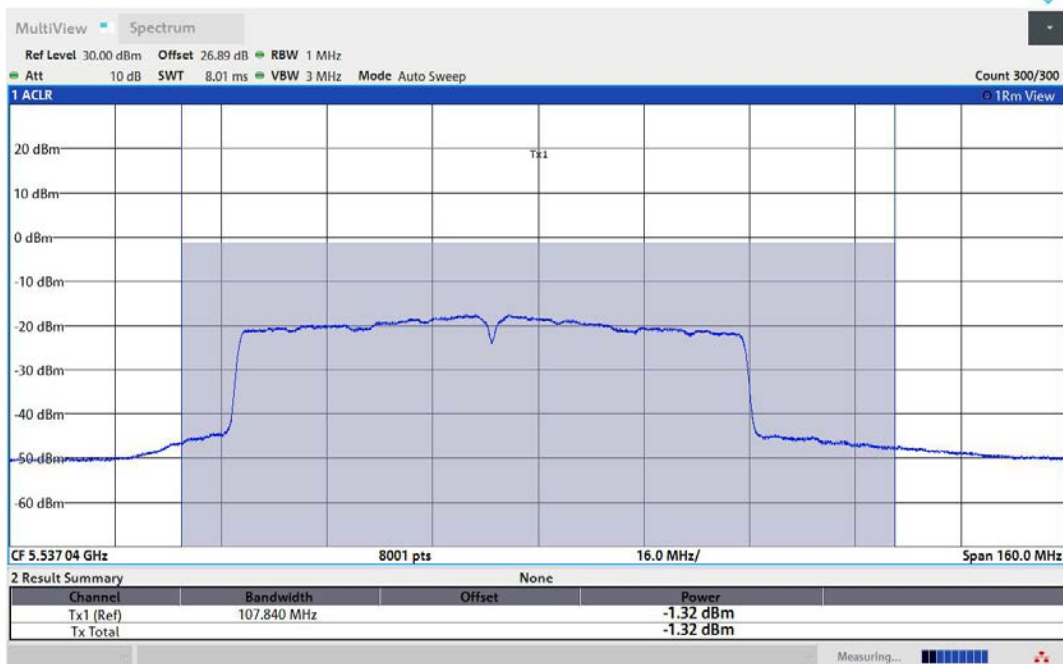
11AC80MIMO-Ant1-5530-TPC_L-PASS
