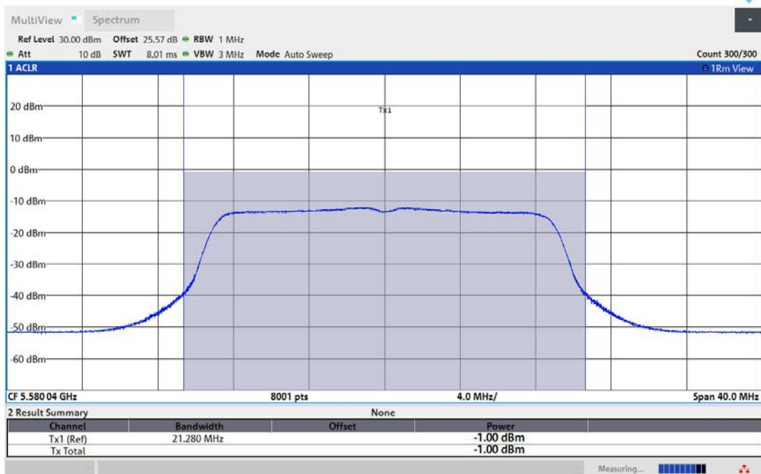
11AC20MIMO-Ant3-5580-TPC_L-PASS
