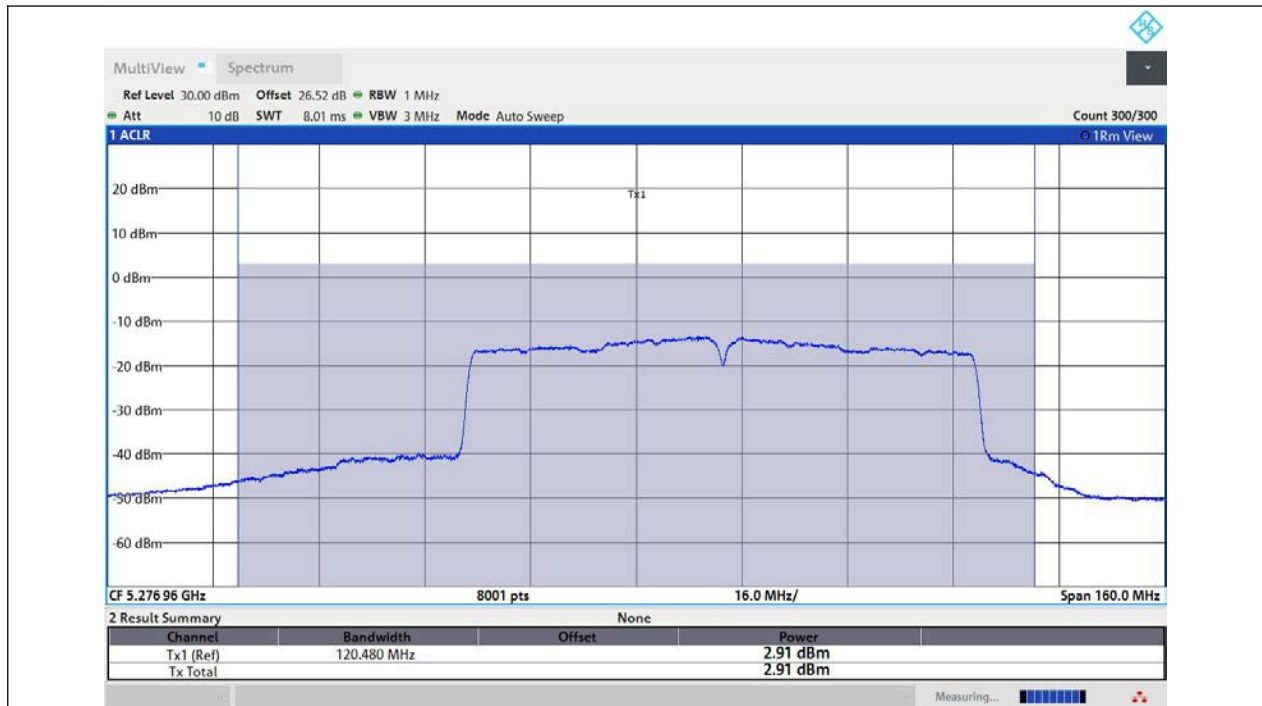
11AC80MIMO-Ant2-5290-TPC_H-PASS
