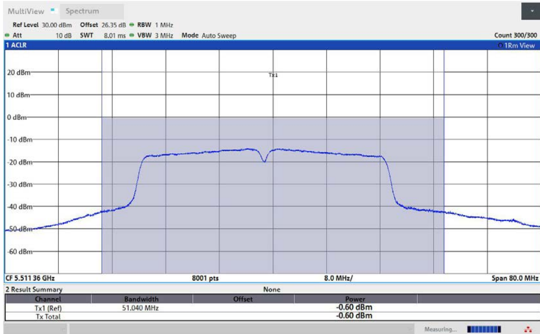
11AC40MIMO-Ant3-5510-TPC_L-PASS
