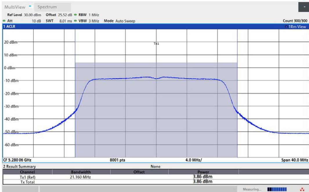
11AC20MIMO-Ant3-5280-TPC_H-PASS
