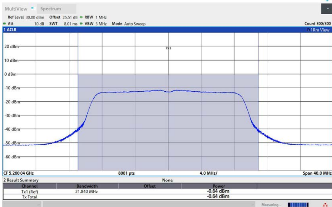
11AC20MIMO-Ant1-5260-TPC_L-PASS
