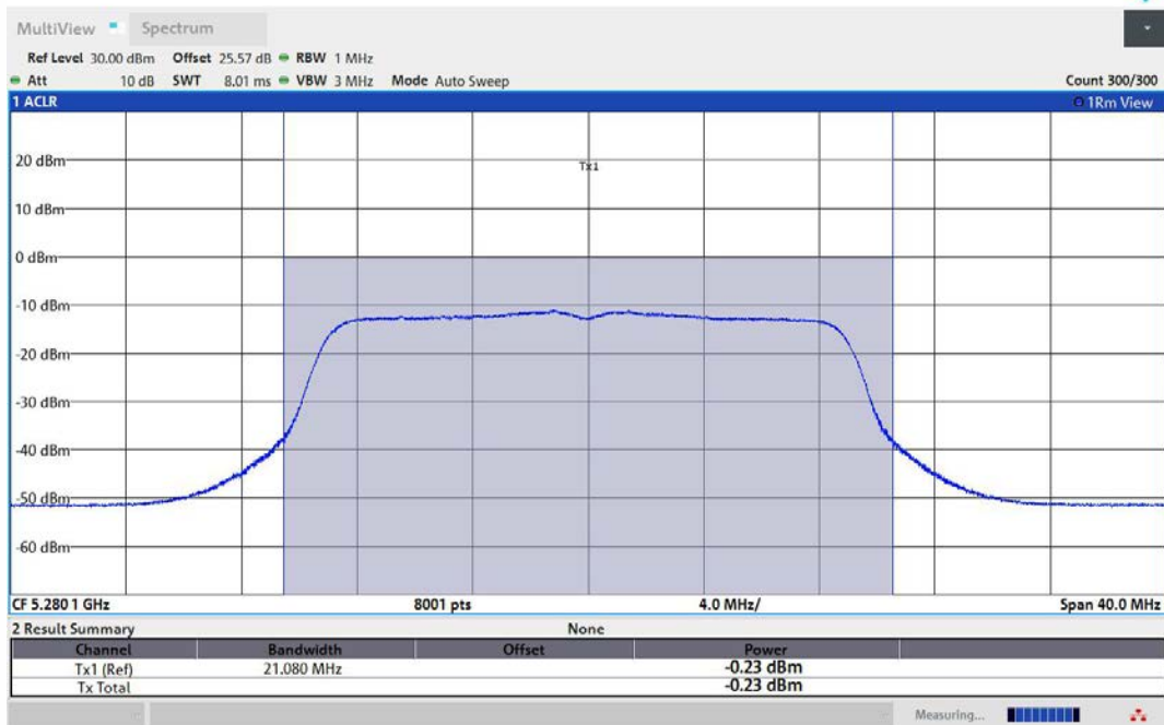
11AC20MIMO-Ant2-5280-TPC_L-PASS
