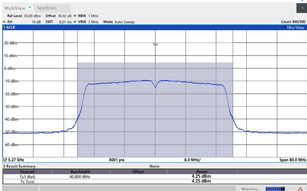
11AC40MIMO-Ant3-5270-TPC_H-PASS
