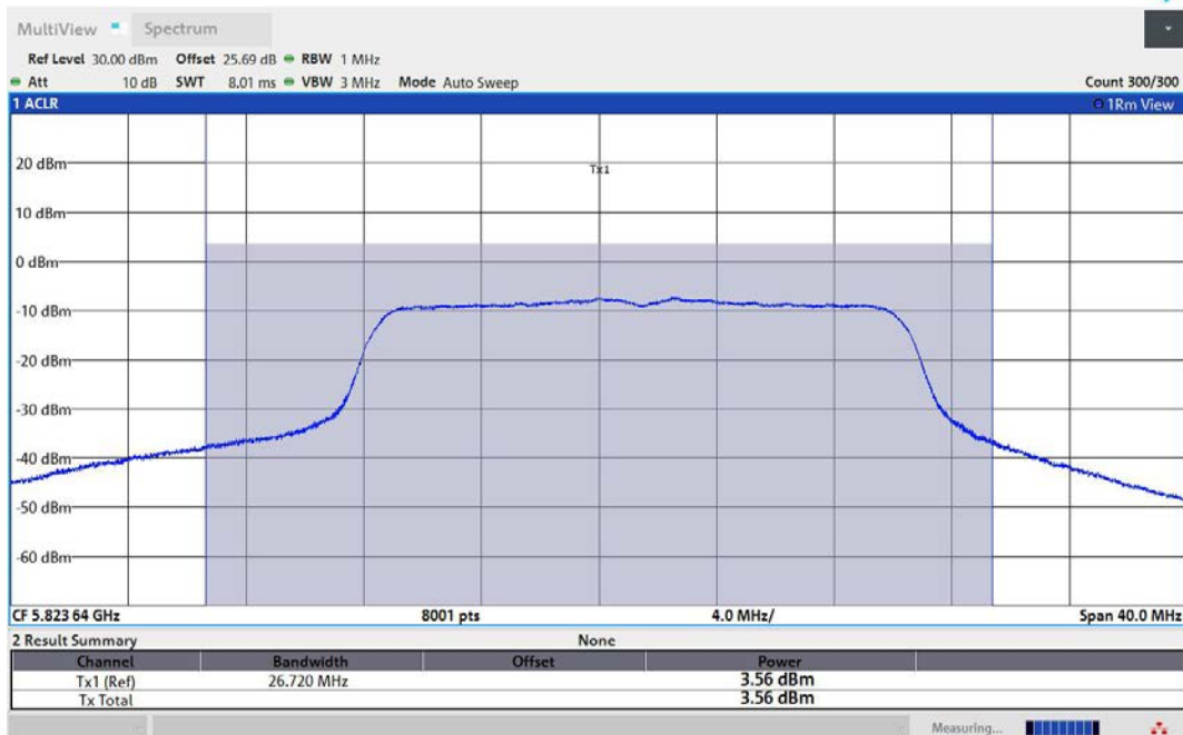
11AC20MIMO-Ant3-5825-PASS
