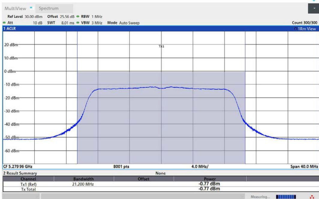
11AC20MIMO-Ant1-5280-TPC_L-PASS
