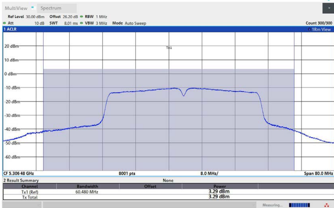
11AC40MIMO-Ant3-5310-TPC_H-PASS
