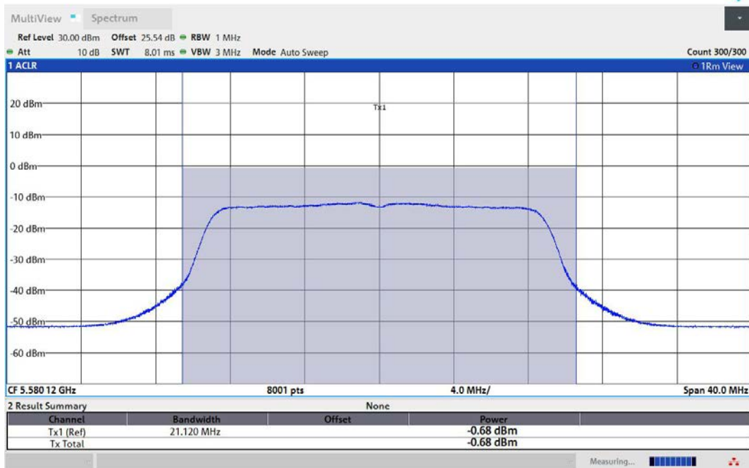
11AC20MIMO-Ant2-5580-TPC_L-PASS
