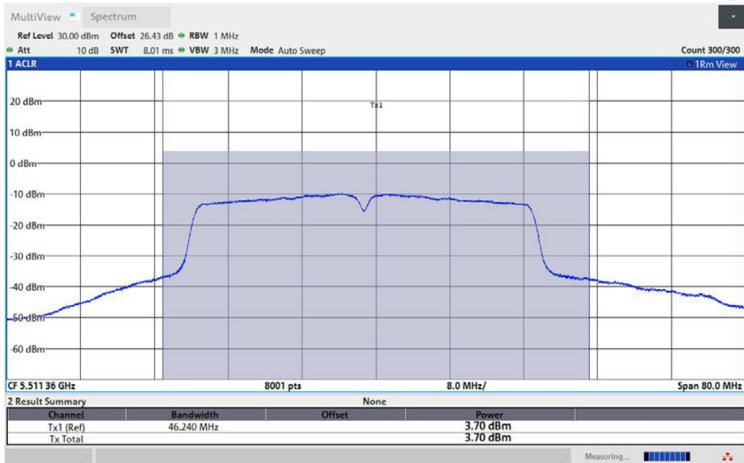
11AC40MIMO-Ant2-5510-TPC_H-PASS
