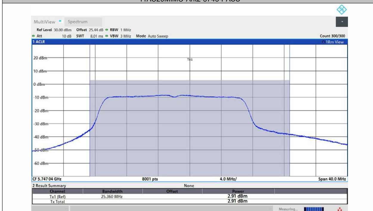
11AC20MIMO-Ant3-5745-PASS
