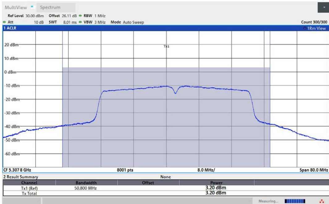
11AC40MIMO-Ant2-5310-TPC_H-PASS
