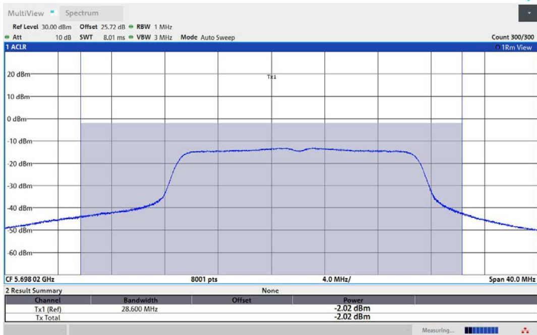
11AC20MIMO-Ant2-5700-TPC_L-PASS
