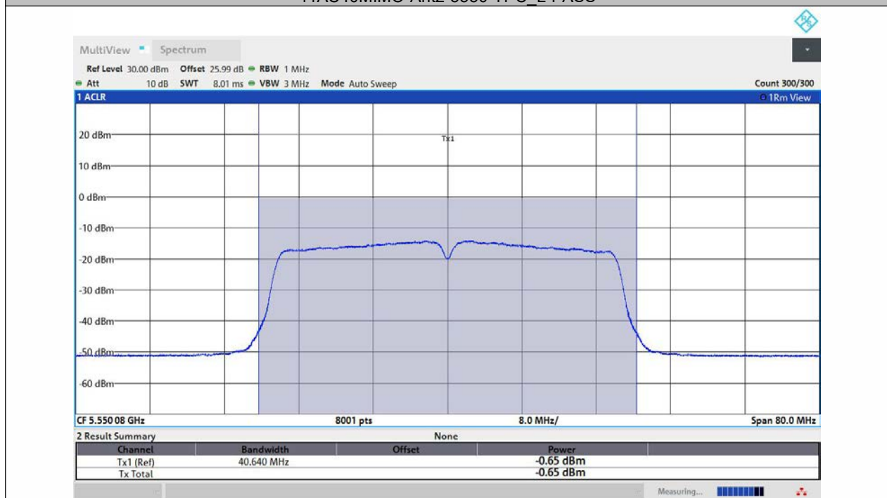
11AC40MIMO-Ant3-5550-TPC_L-PASS
