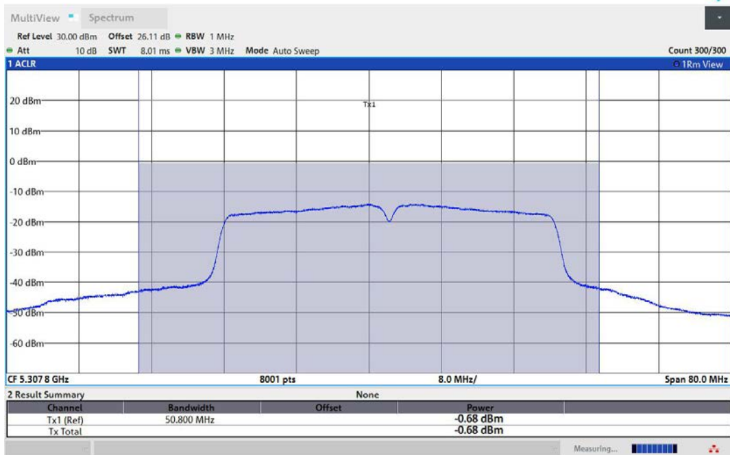
11AC40MIMO-Ant2-5310-TPC_L-PASS
