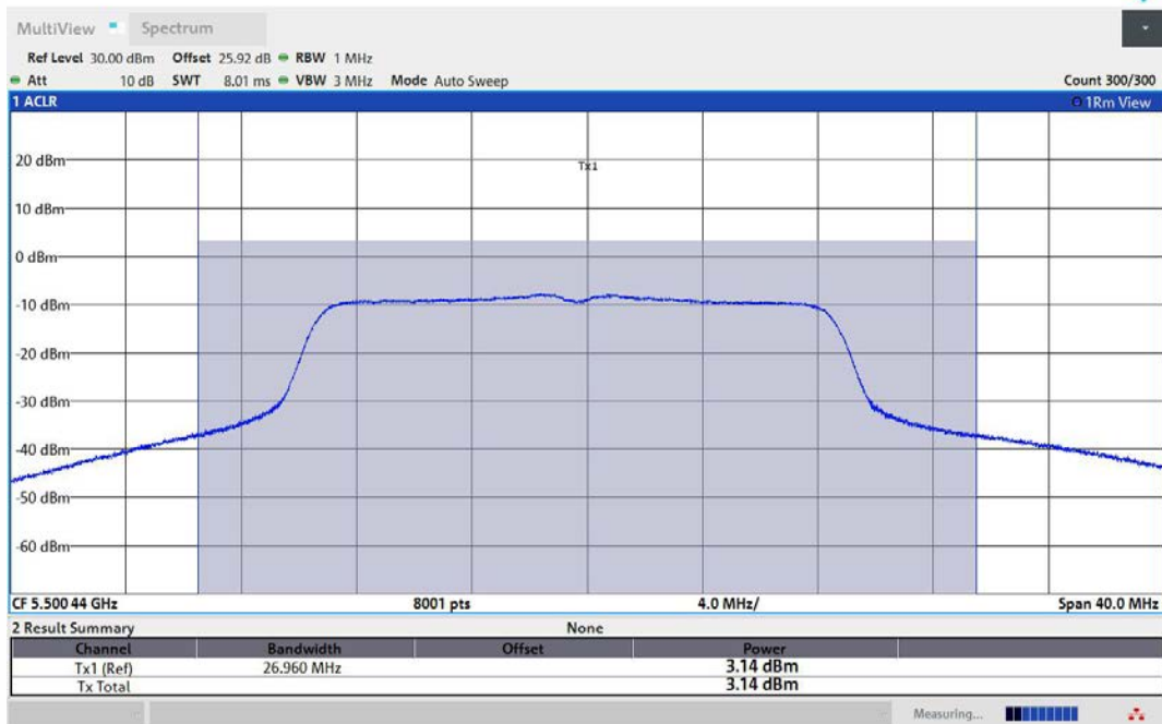
11AC20MIMO-Ant2-5500-TPC_H-PASS
