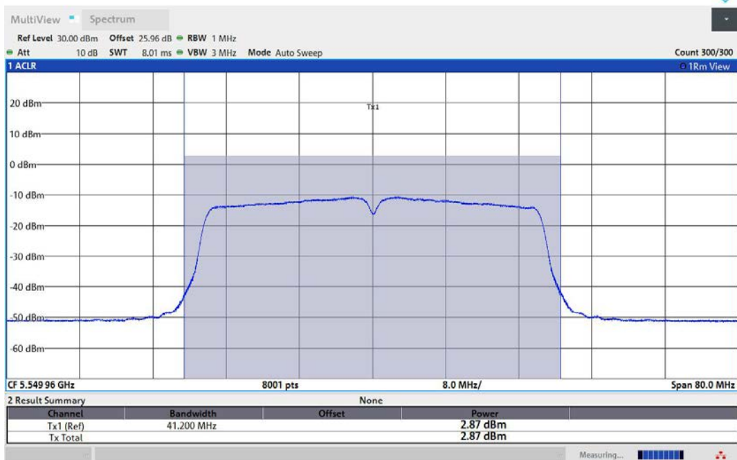
11AC40MIMO-Ant1-5550-TPC_H-PASS
