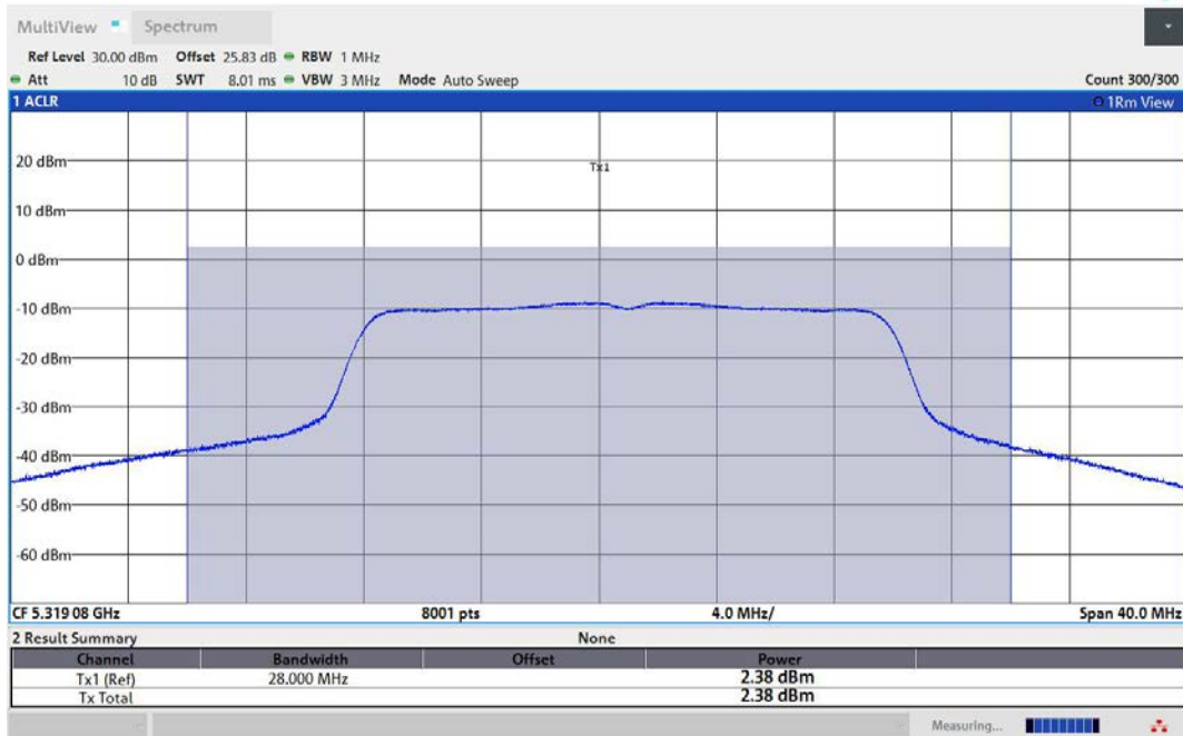
11AC20MIMO-Ant1-5320-TPC_H-PASS
