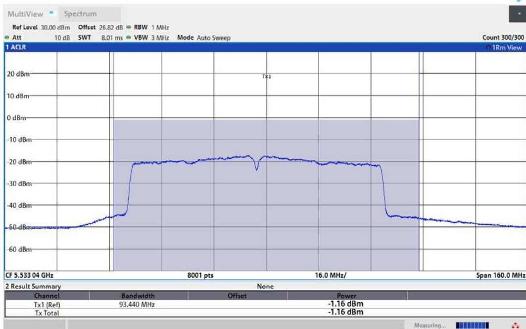
11AC80MIMO-Ant3-5530-TPC_L-PASS
