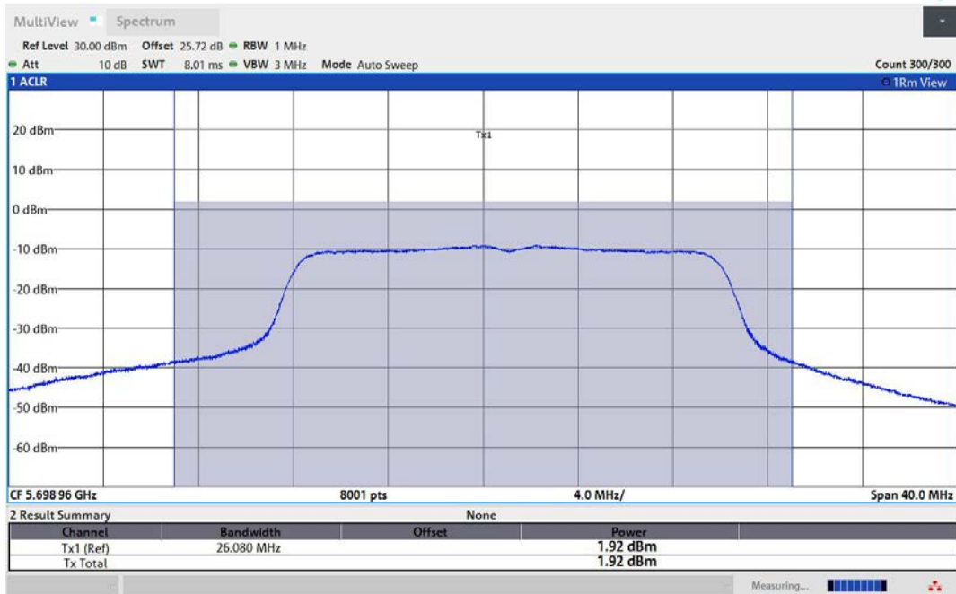
11AC20MIMO-Ant1-5700-TPC_H-PASS
