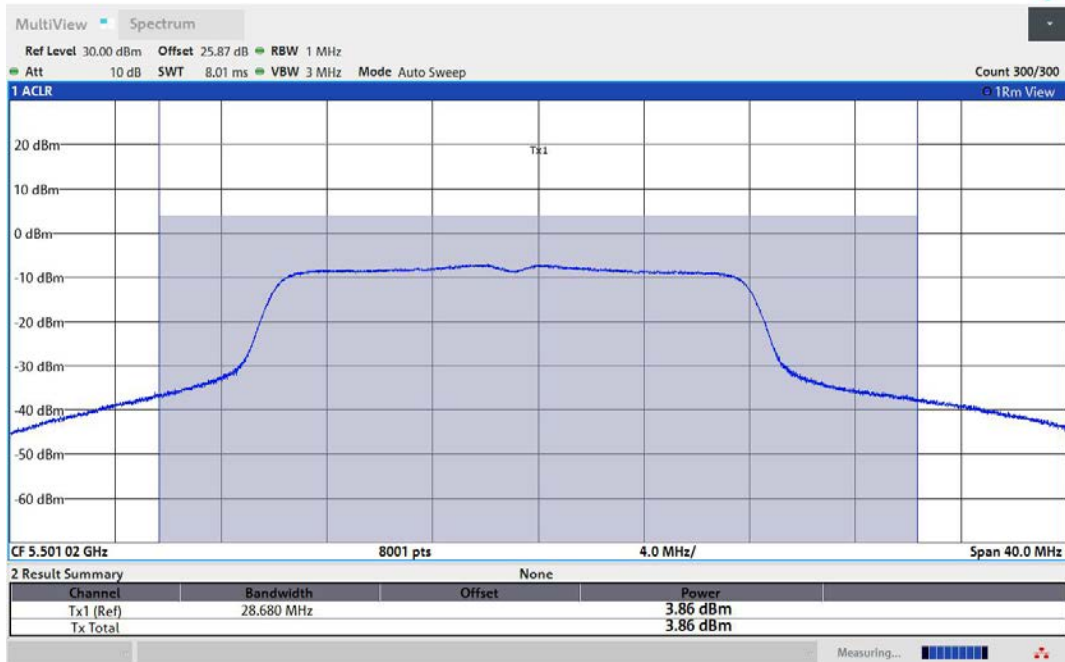
11AC20MIMO-Ant3-5500-TPC_H-PASS
