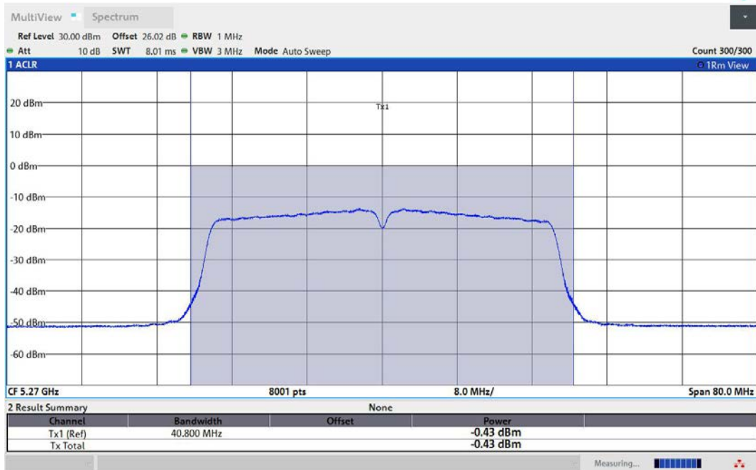
11AC40MIMO-Ant3-5270-TPC_L-PASS
