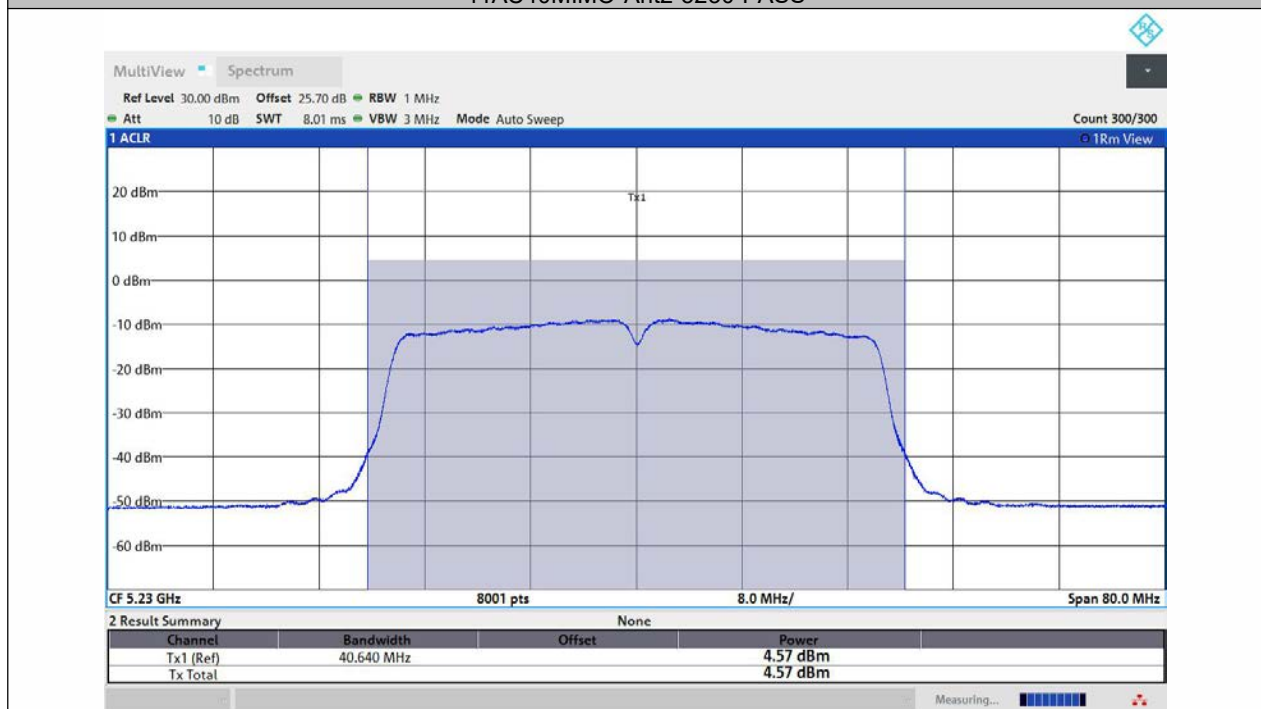
11AC40MIMO-Ant3-5230-PASS
