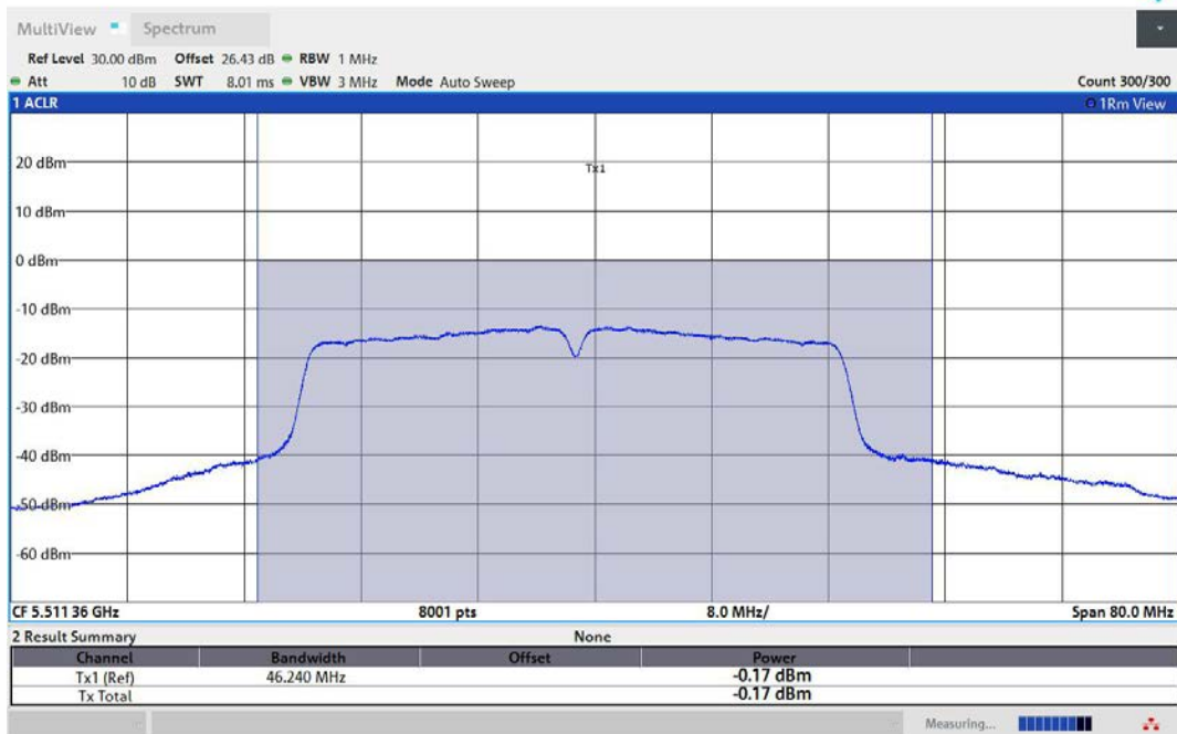
11AC40MIMO-Ant2-5510-TPC_L-PASS
