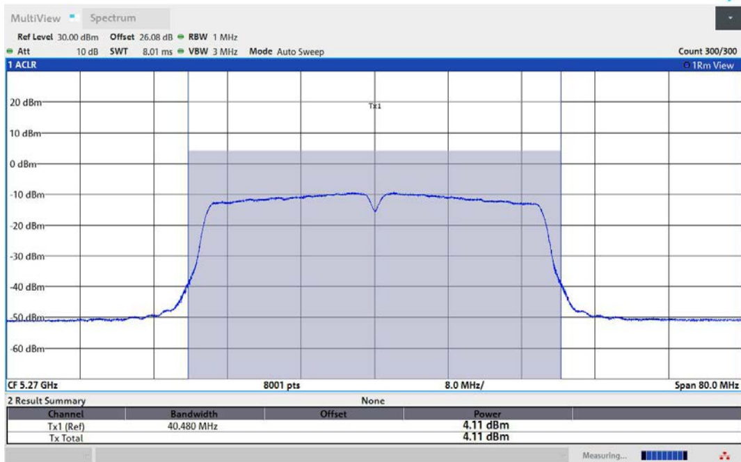
11AC40MIMO-Ant2-5270-TPC_H-PASS
