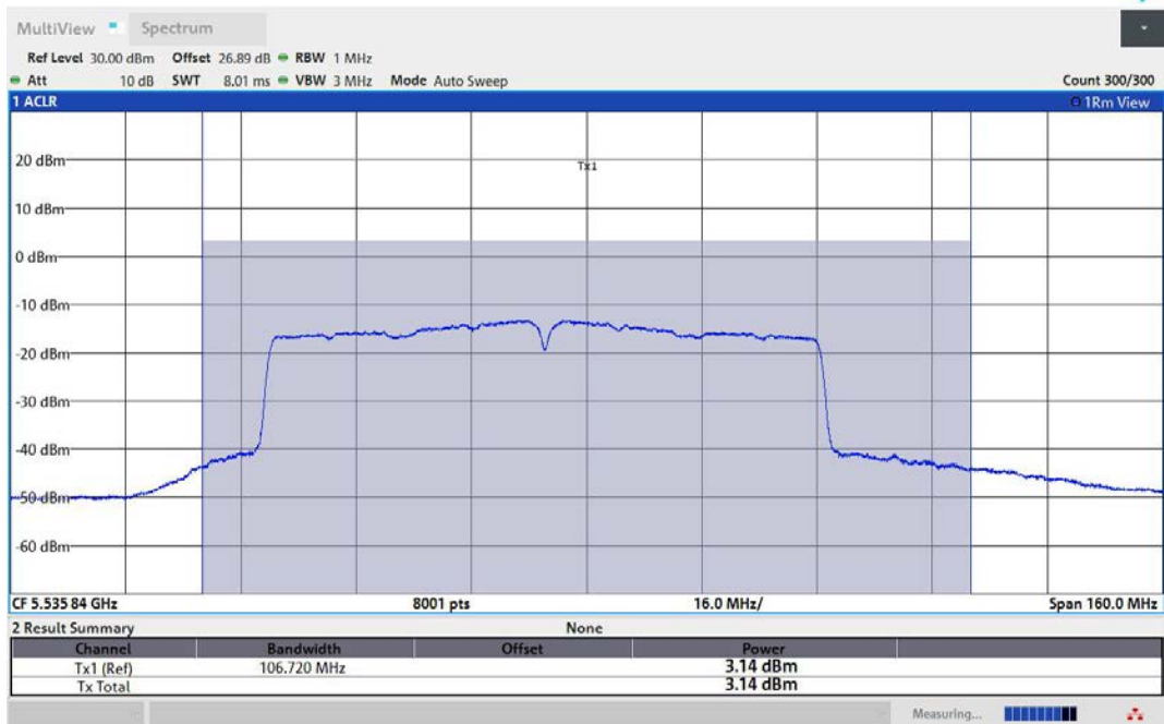
11AC80MIMO-Ant2-5530-TPC_H-PASS
