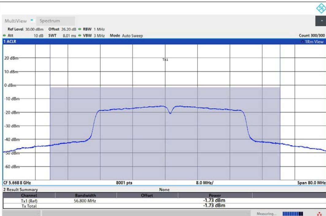
11AC40MIMO-Ant2-5670-TPC_L-PASS
