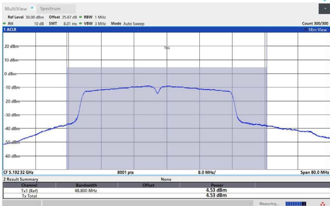
11AC40MIMO-Ant3-5190-PASS
