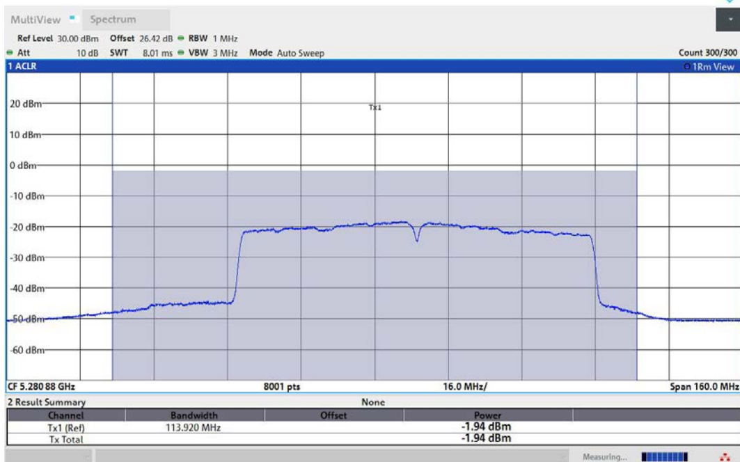
11AC80MIMO-Ant1-5290-TPC_L-PASS
