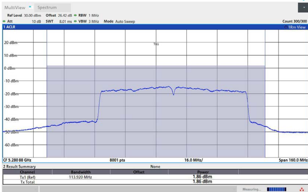
11AC80MIMO-Ant1-5290-TPC_H-PASS
