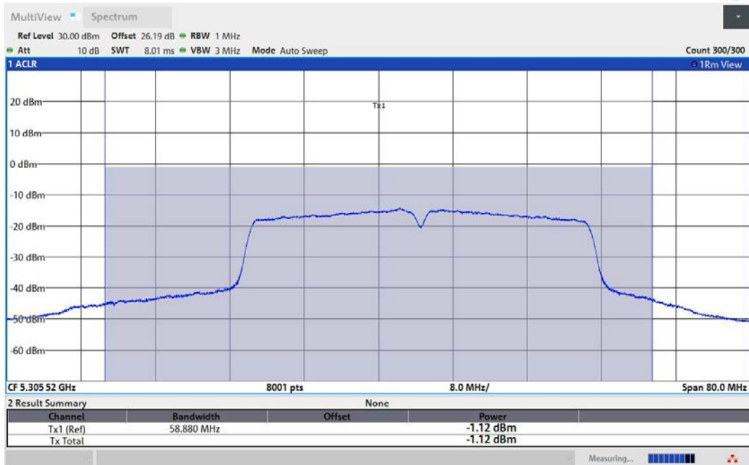
11AC40MIMO-Ant1-5310-TPC_L-PASS
