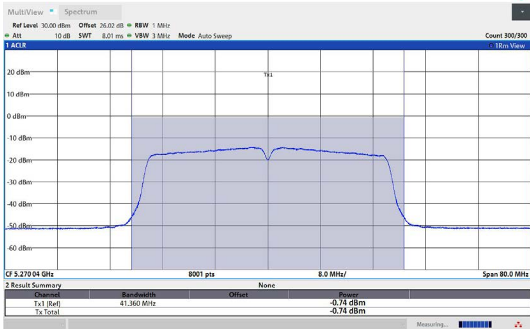
11AC40MIMO-Ant1-5270-TPC_L-PASS
