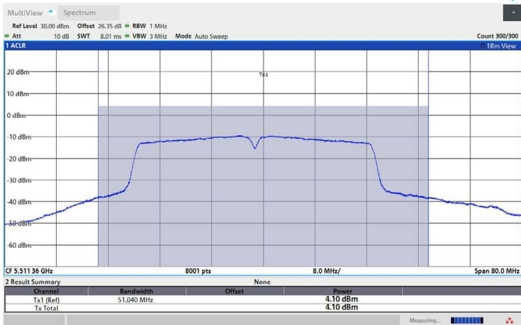
11AC40MIMO-Ant3-5510-TPC_H-PASS
