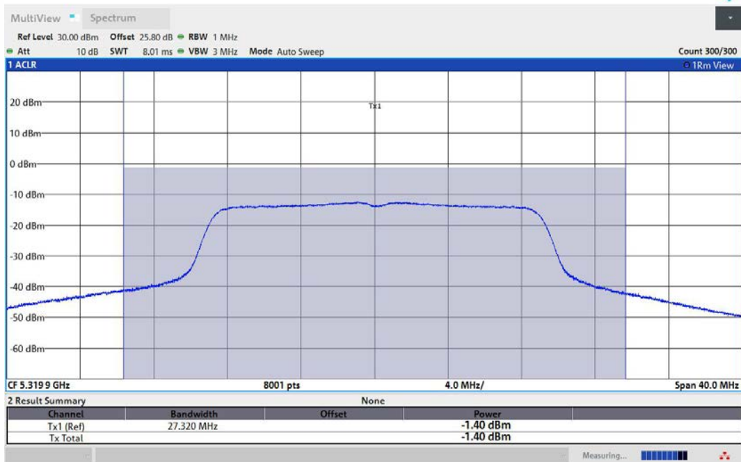
11AC20MIMO-Ant3-5320-TPC_L-PASS
