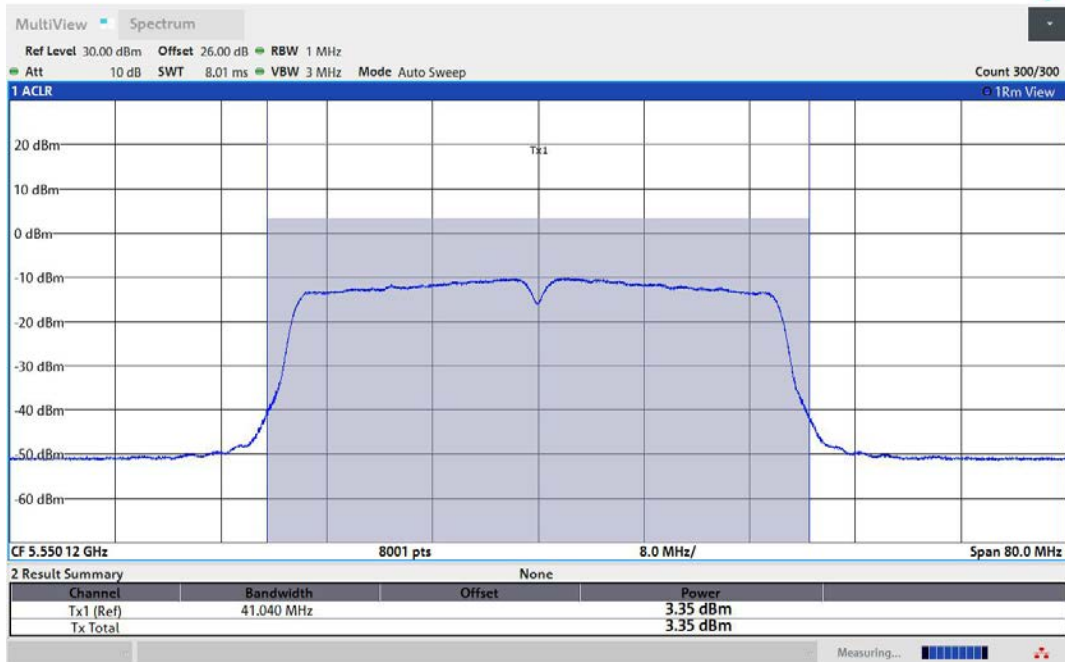
11AC40MIMO-Ant2-5550-TPC_H-PASS
