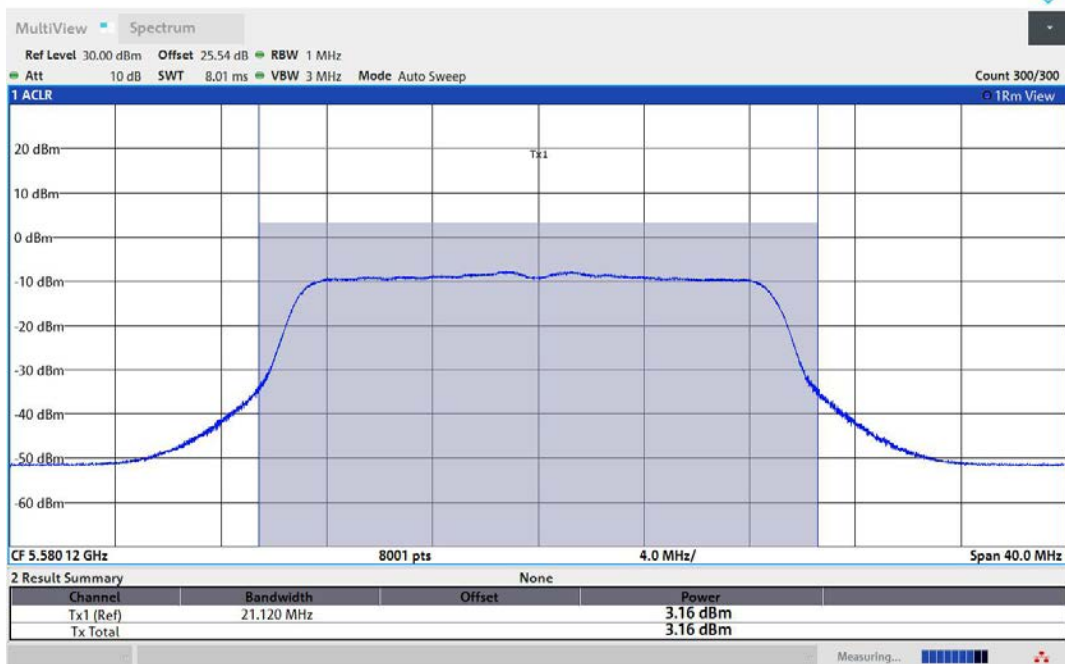
11AC20MIMO-Ant2-5580-TPC_H-PASS
