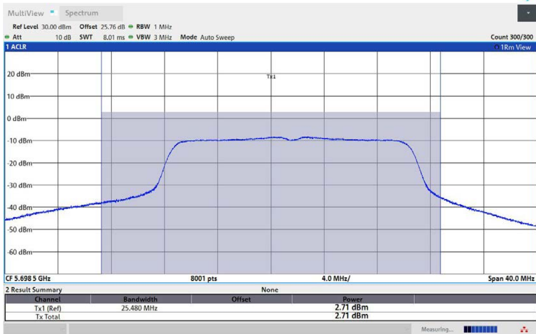
11AC20MIMO-Ant3-5700-TPC_H-PASS
