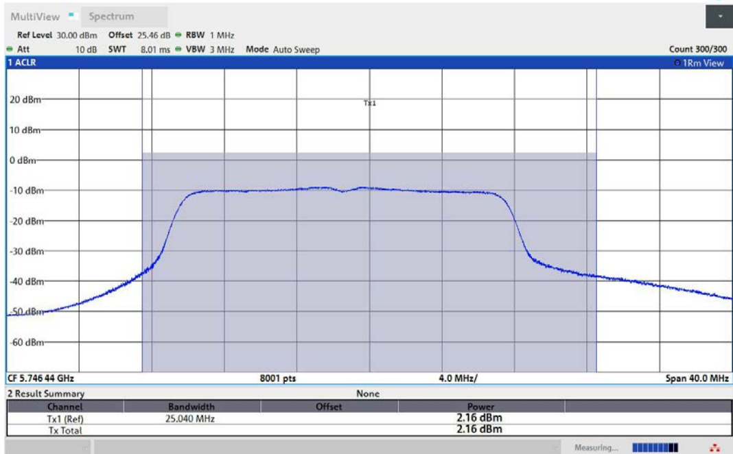
11AC20MIMO-Ant1-5745-PASS
