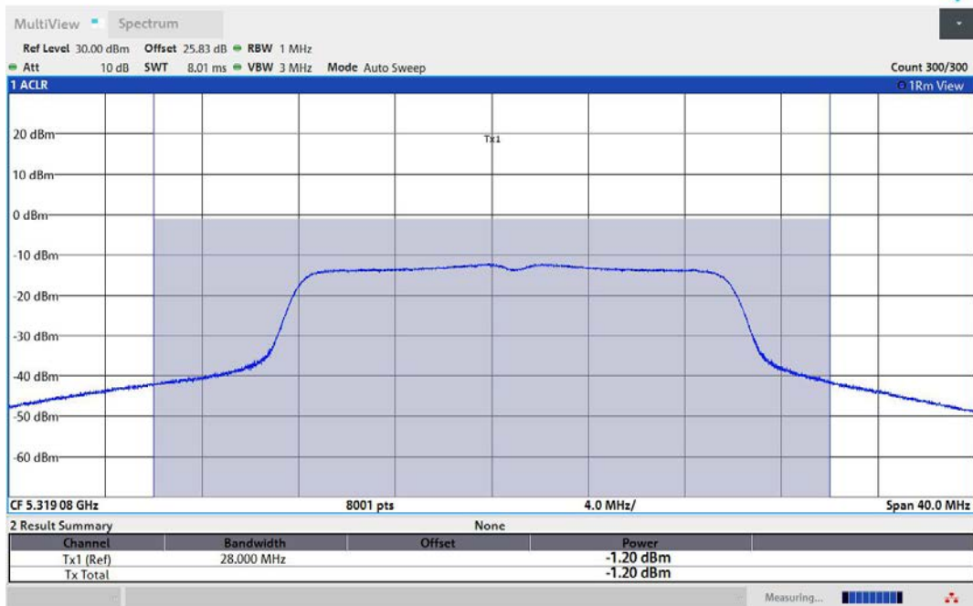
11AC20MIMO-Ant1-5320-TPC_L-PASS
