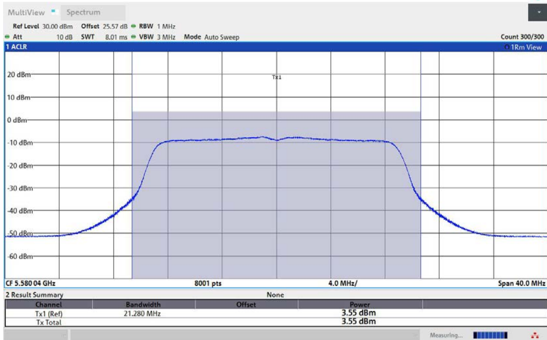
11AC20MIMO-Ant3-5580-TPC_H-PASS
