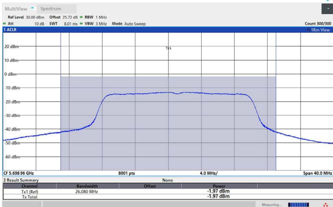
11AC20MIMO-Ant1-5700-TPC_L-PASS
