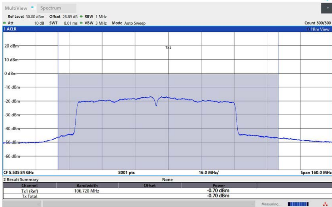
11AC80MIMO-Ant2-5530-TPC_L-PASS
