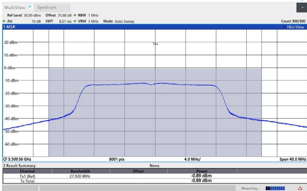
11AC20MIMO-Ant1-5500-TPC_L-PASS
