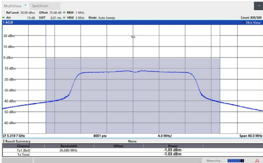
11AC20MIMO-Ant2-5320-TPC_L-PASS
