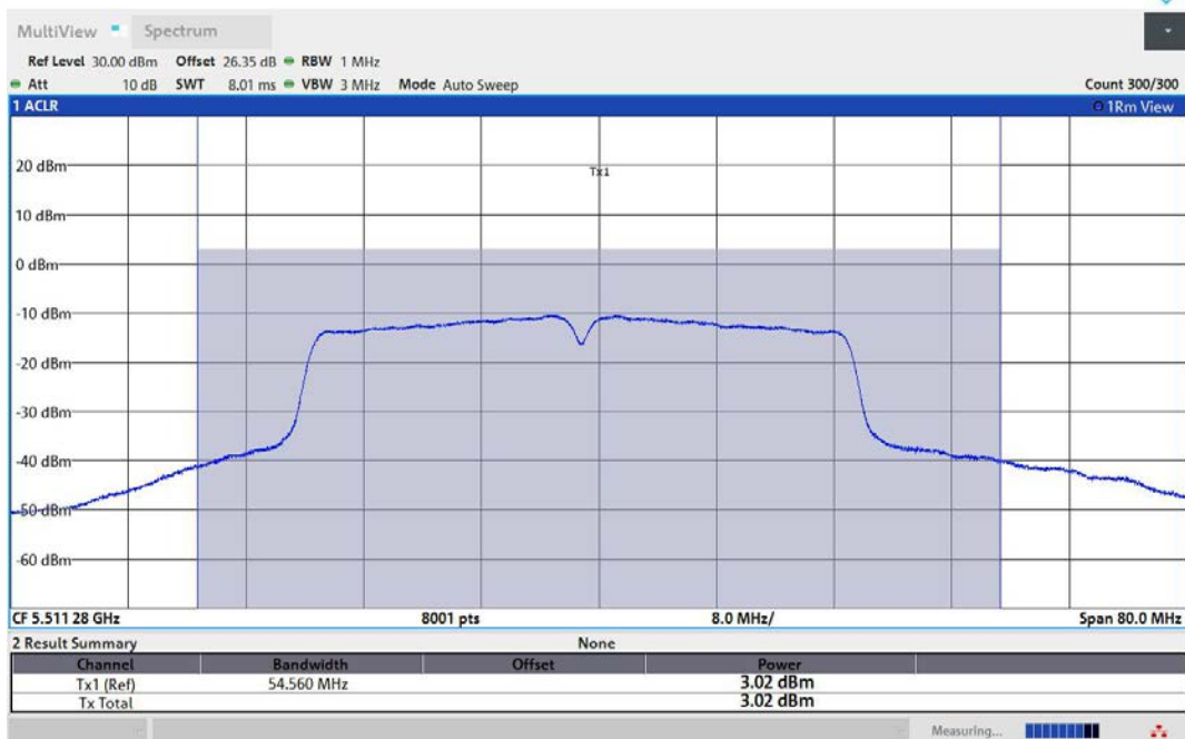
11AC40MIMO-Ant1-5510-TPC_H-PASS
