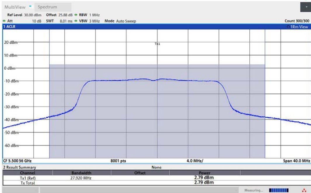
11AC20MIMO-Ant1-5500-TPC_H-PASS
