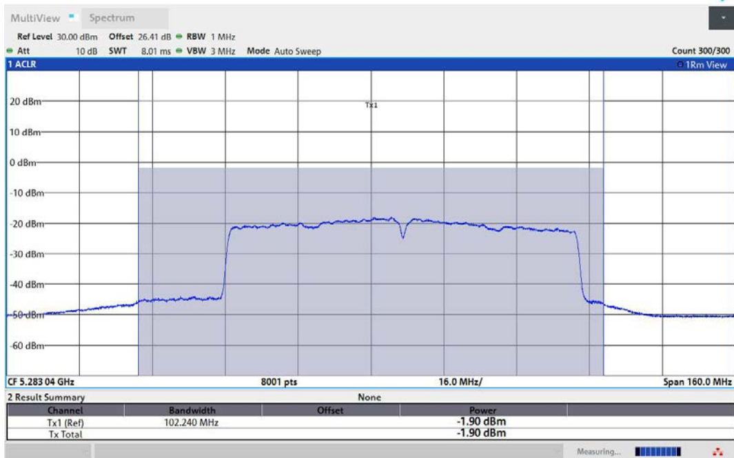
11AC80MIMO-Ant3-5290-TPC_L-PASS
