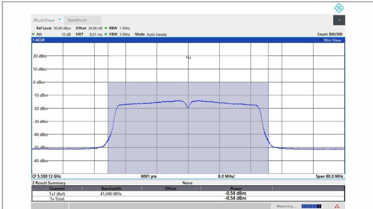
11AC40MIMO-Ant2-5550-TPC_L-PASS
