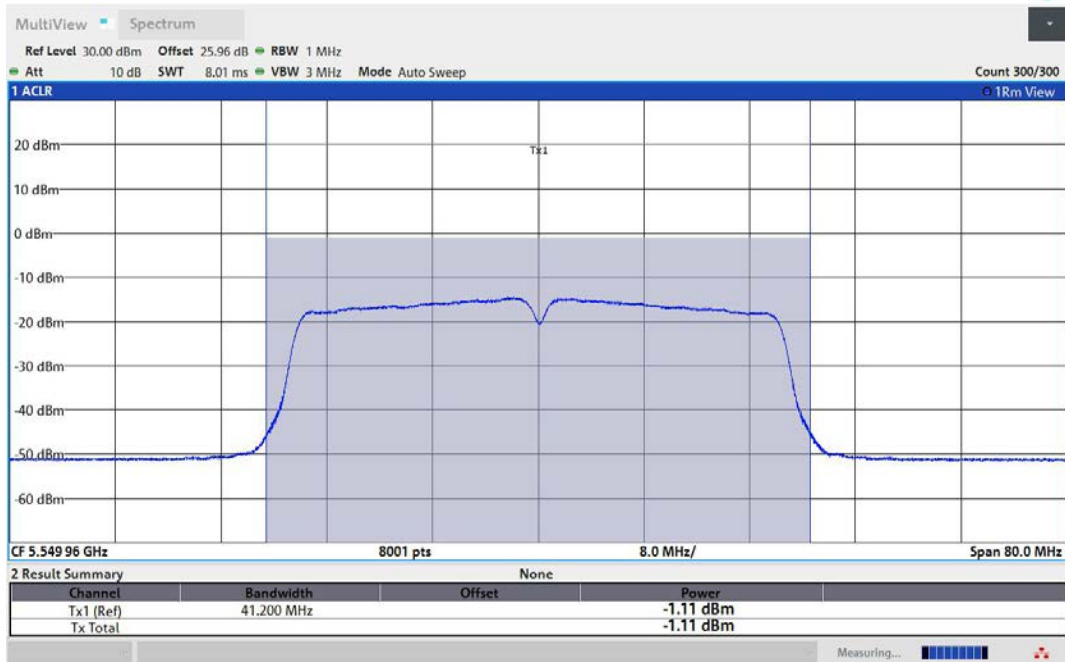
11AC40MIMO-Ant1-5550-TPC_L-PASS
