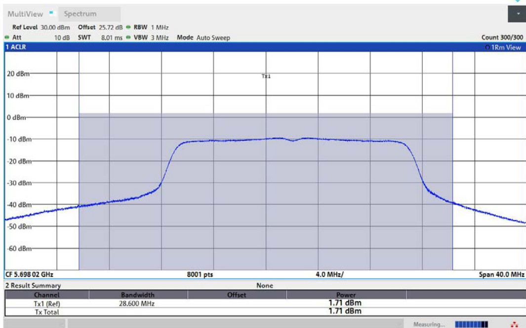
11AC20MIMO-Ant2-5700-TPC_H-PASS
