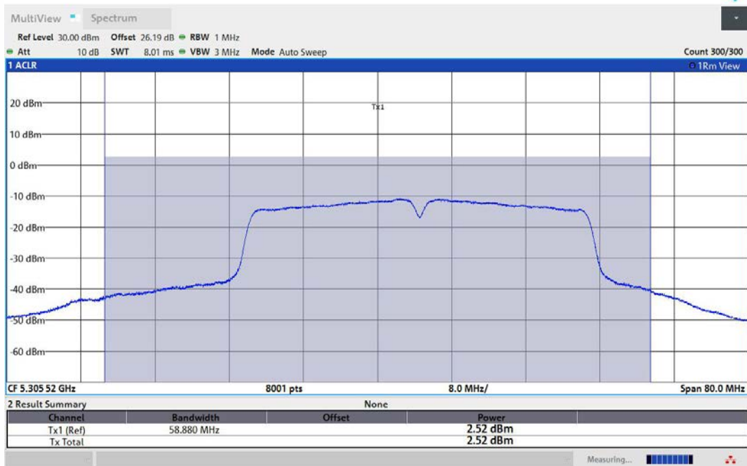
11AC40MIMO-Ant1-5310-TPC_H-PASS
