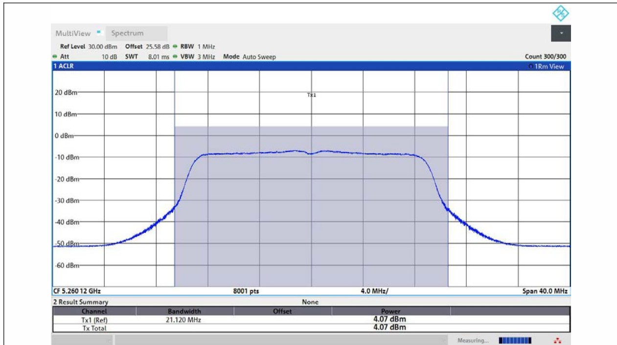
11AC20MIMO-Ant2-5260-TPC_H-PASS
