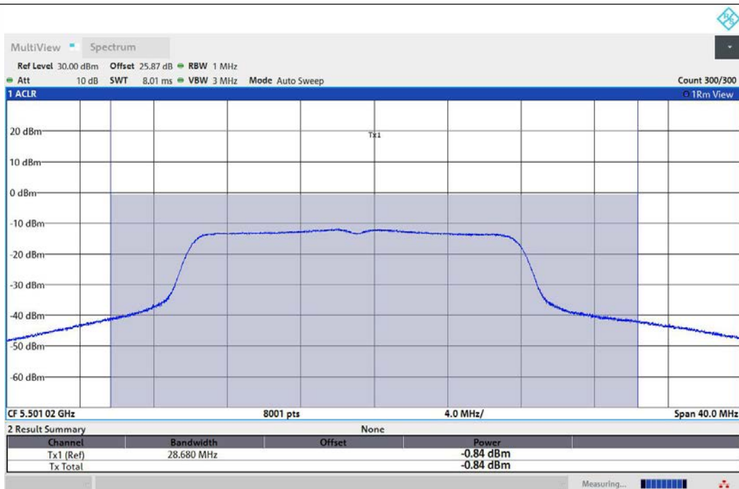
11AC20MIMO-Ant3-5500-TPC_L-PASS
