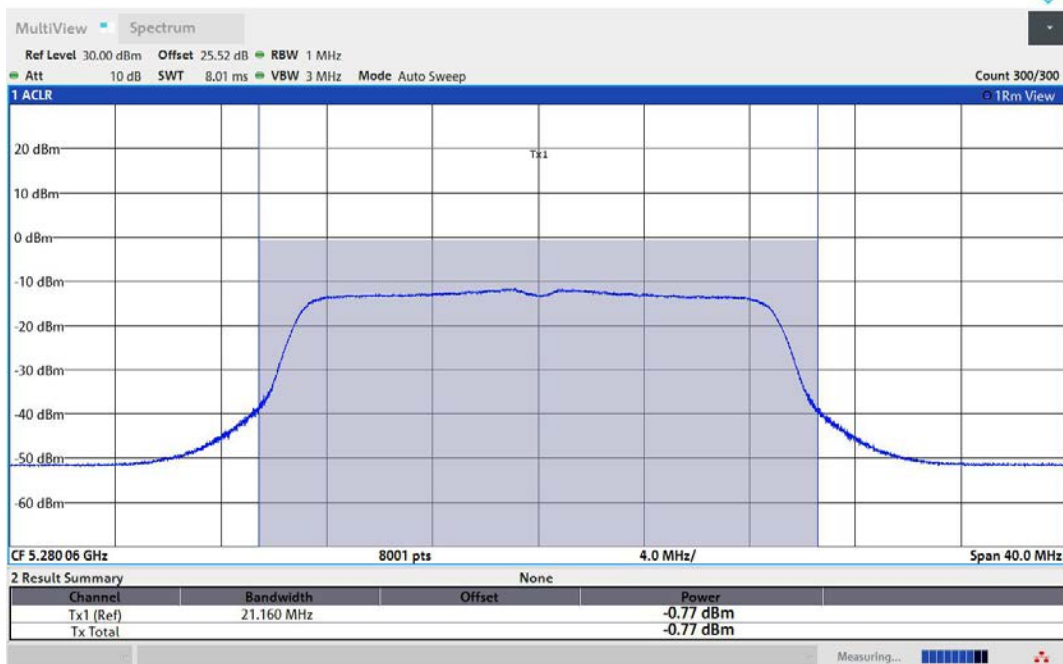
11AC20MIMO-Ant3-5280-TPC_L-PASS
