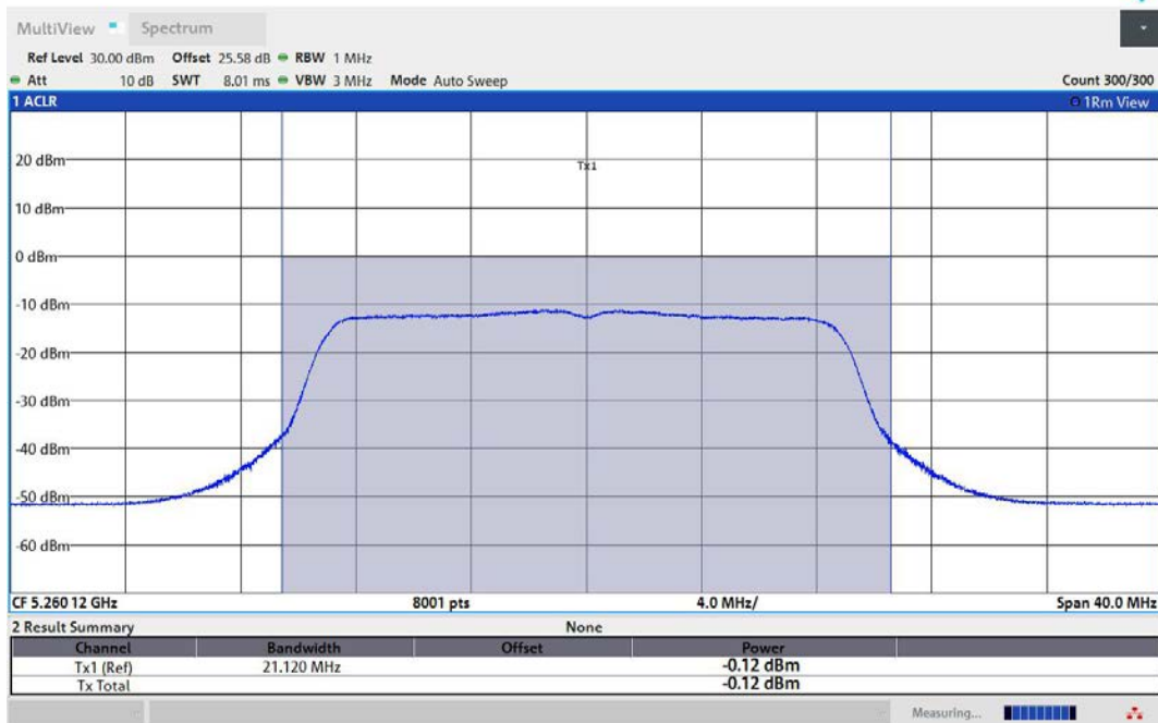
11AC20MIMO-Ant2-5260-TPC_L-PASS
