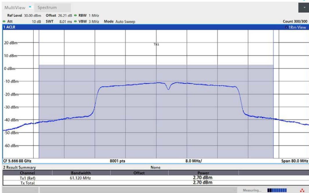
11AC40MIMO-Ant3-5670-TPC_H-PASS
