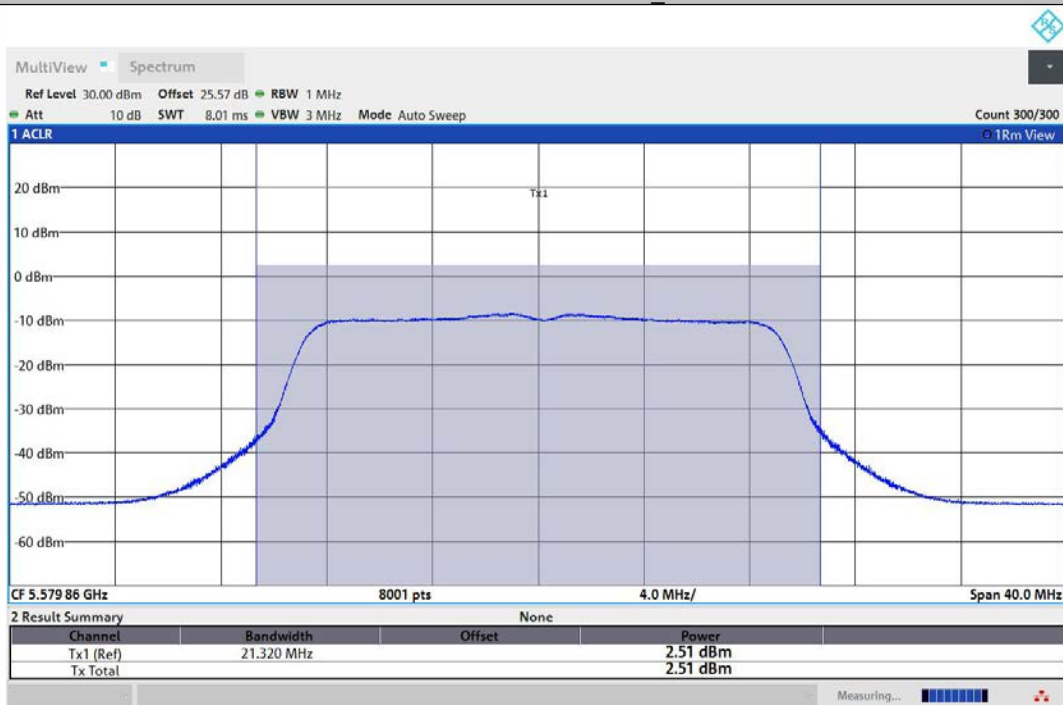
11AC20MIMO-Ant1-5580-TPC_H-PASS
