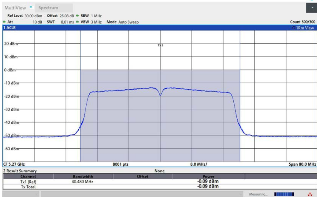
11AC40MIMO-Ant2-5270-TPC_L-PASS
