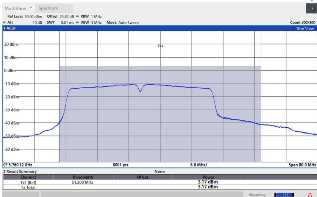
11AC40MIMO-Ant3-5755-PASS
