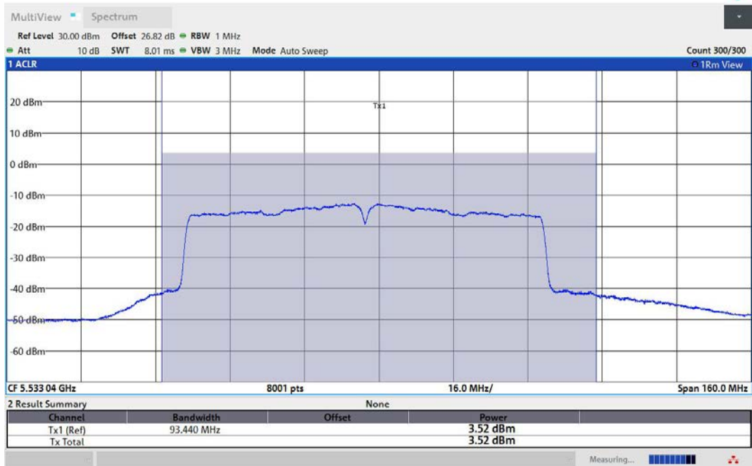
11AC80MIMO-Ant3-5530-TPC_H-PASS
