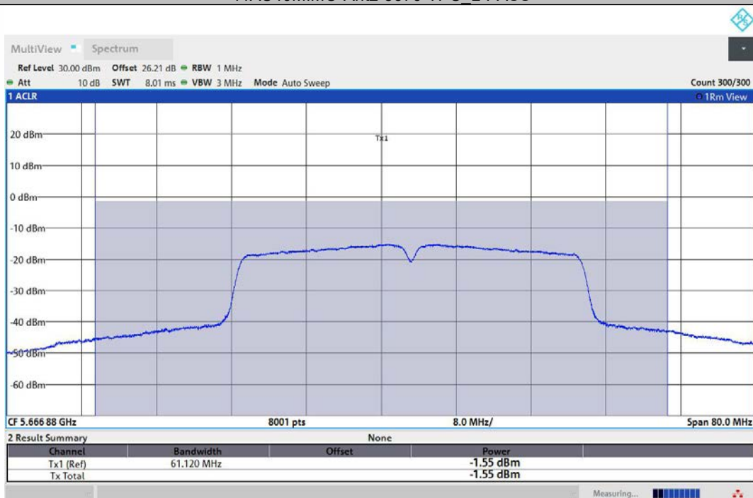
11AC40MIMO-Ant3-5670-TPC_L-PASS
