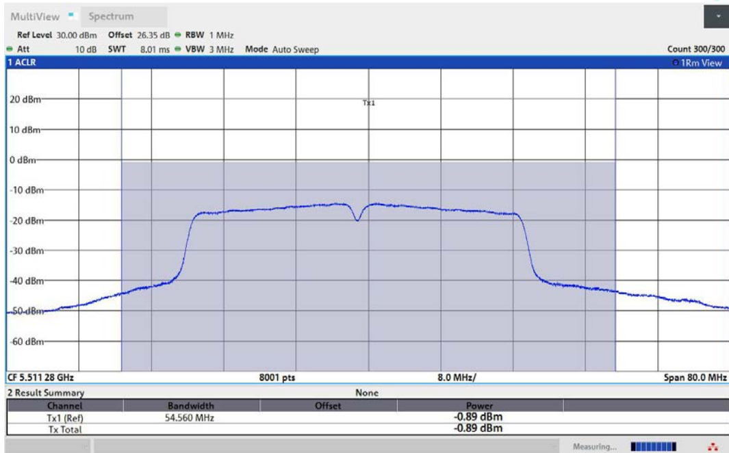
11AC40MIMO-Ant1-5510-TPC_L-PASS
