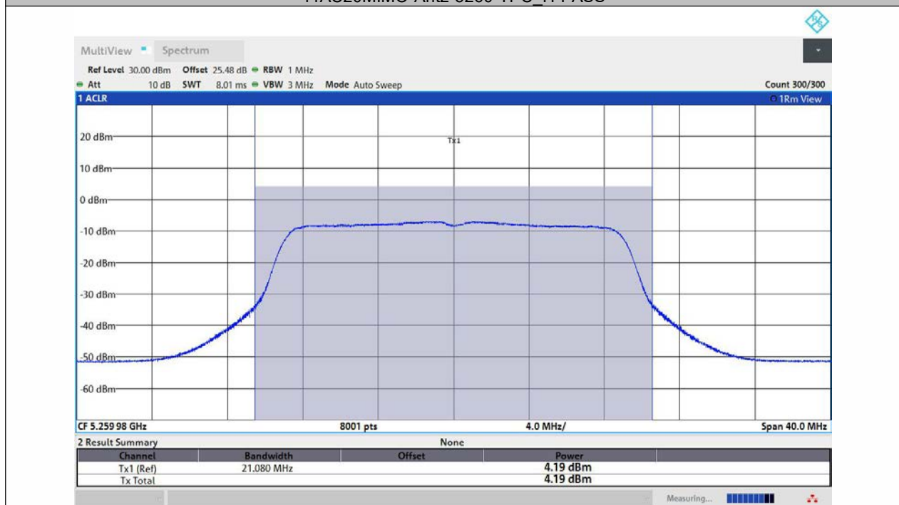
11AC20MIMO-Ant3-5260-TPC_H-PASS
