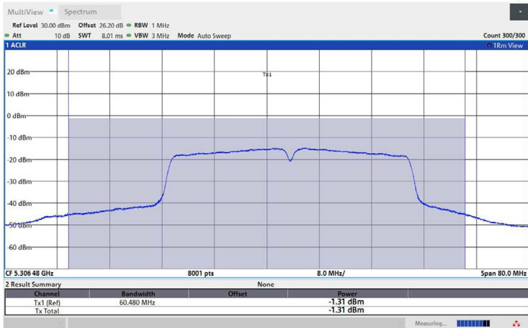
11AC40MIMO-Ant3-5310-TPC_L-PASS
