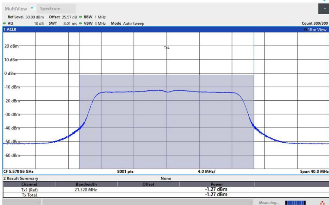
11AC20MIMO-Ant1-5580-TPC_L-PASS
