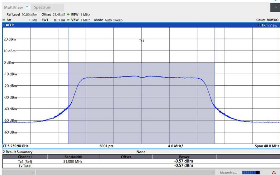
11AC20MIMO-Ant3-5260-TPC_L-PASS
