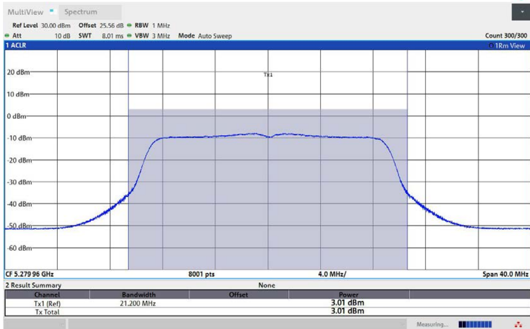
11AC20MIMO-Ant1-5280-TPC_H-PASS
