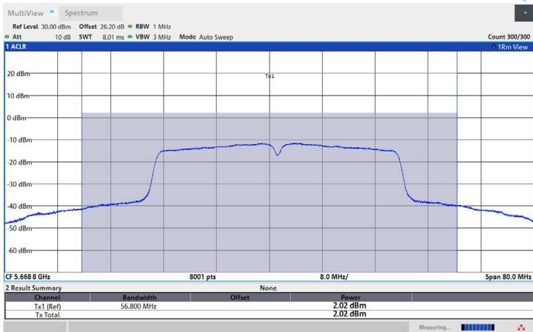
11AC40MIMO-Ant2-5670-TPC_H-PASS
