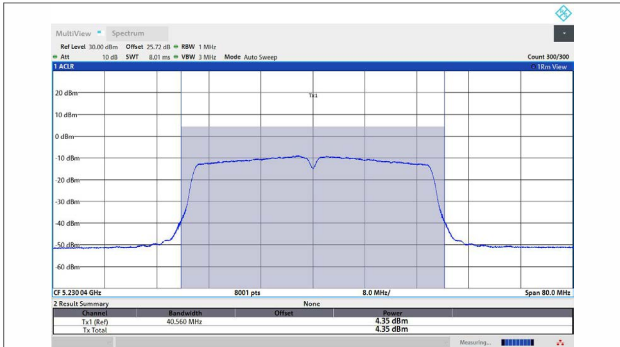
11AC40MIMO-Ant2-5230-PASS
