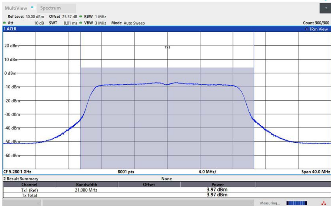
11AC20MIMO-Ant2-5280-TPC_H-PASS
