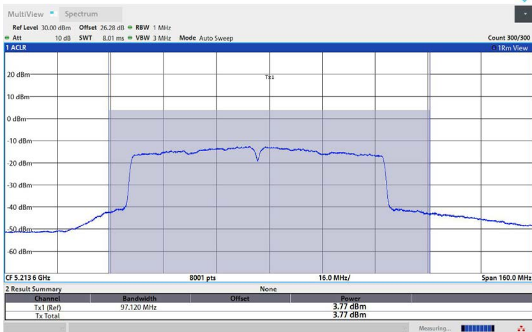
11AC80MIMO-Ant3-5210-PASS
