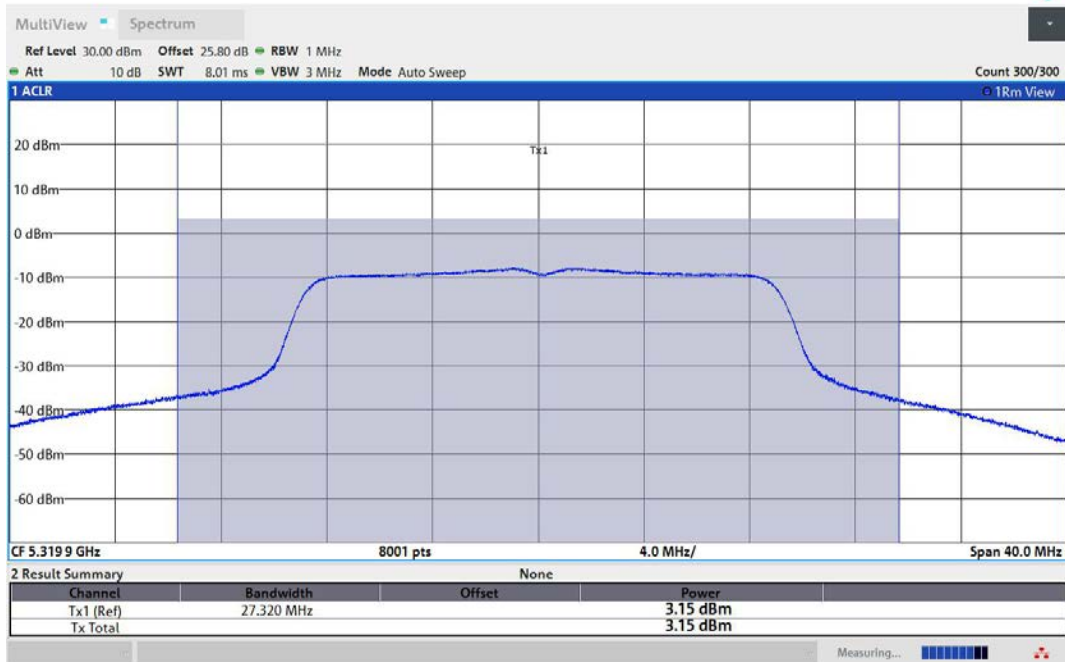
11AC20MIMO-Ant3-5320-TPC_H-PASS
