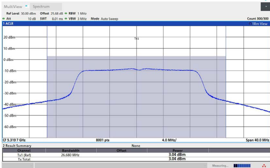
11AC20MIMO-Ant2-5320-TPC_H-PASS
