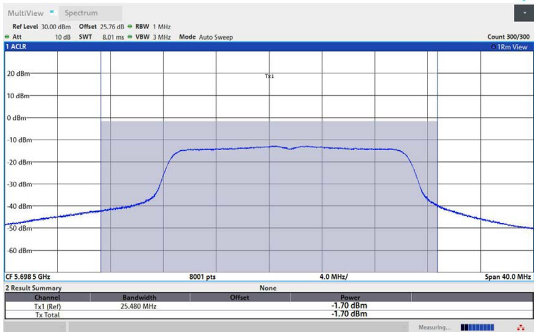
11AC20MIMO-Ant3-5700-TPC_L-PASS
