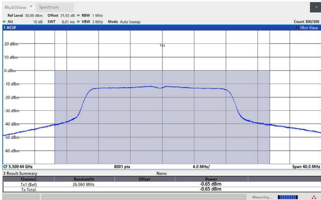
11AC20MIMO-Ant2-5500-TPC_L-PASS
