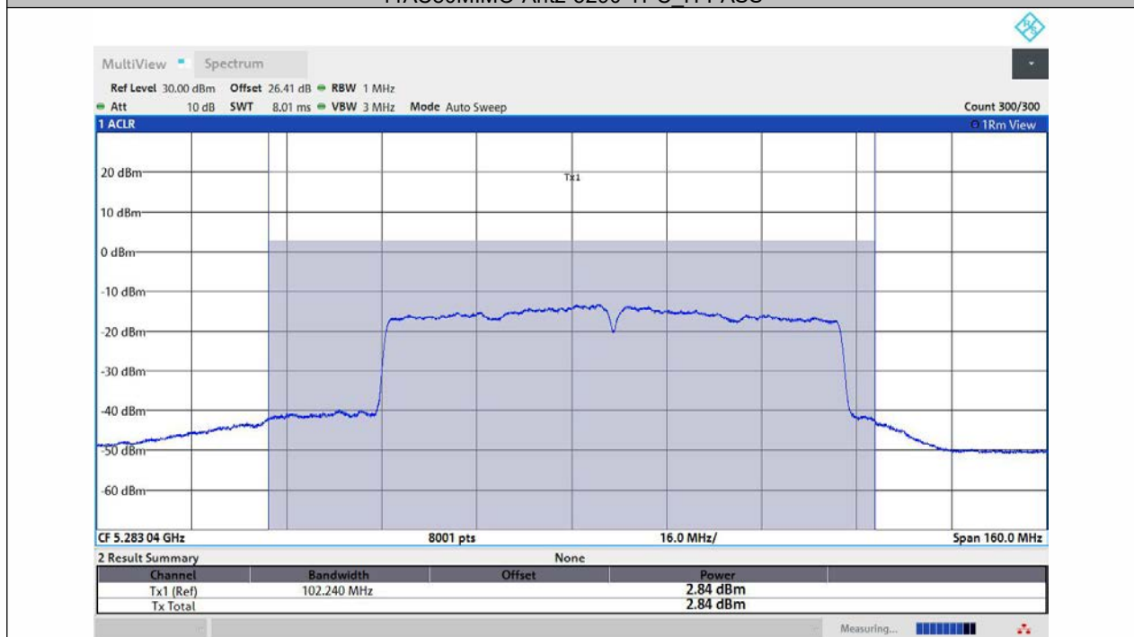
11AC80MIMO-Ant3-5290-TPC_H-PASS
