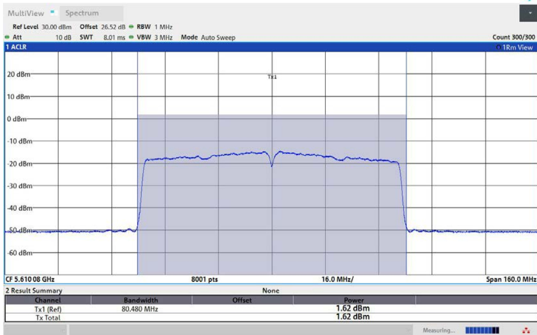
11AC80MIMO-Ant1-5610-TPC_H-PASS
