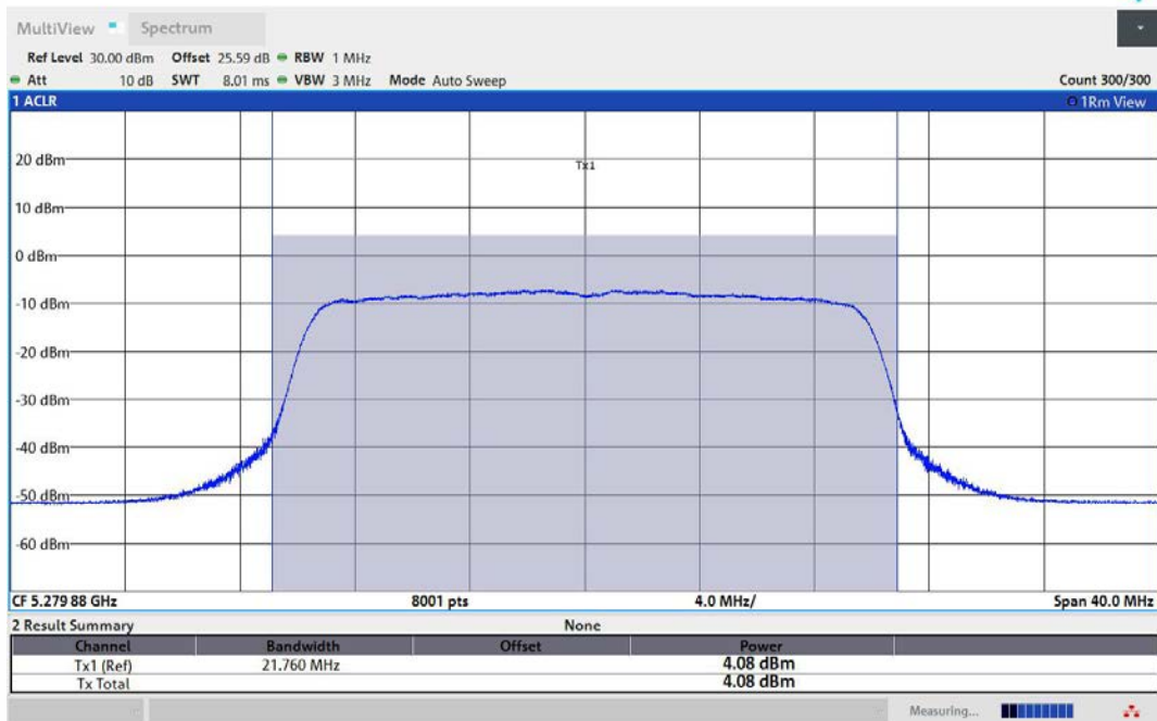
11AX20MIMO-Ant3-5280-TPC_H-PASS
