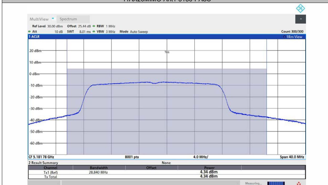
11AX20MIMO-Ant2-5180-PASS
