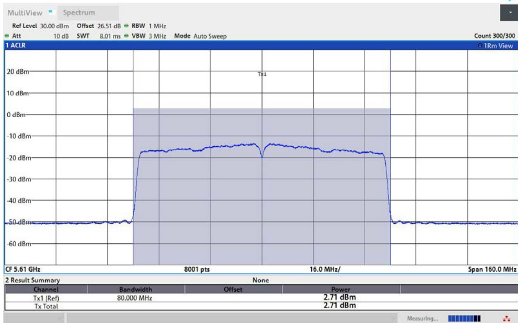
11AC80MIMO-Ant3-5610-TPC_H-PASS
