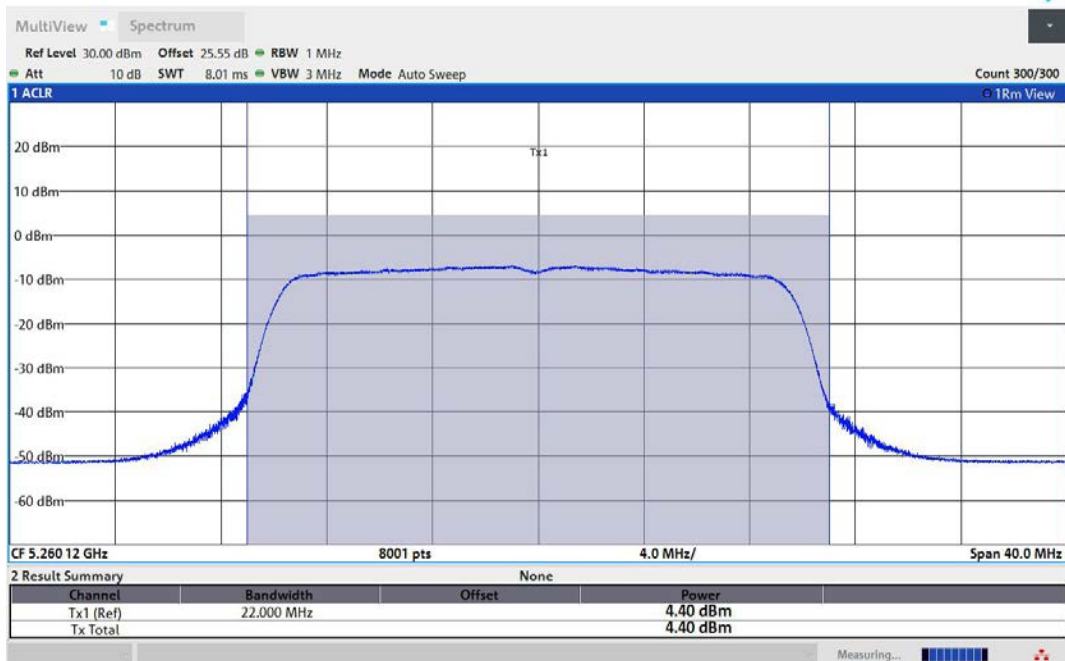
11AX20MIMO-Ant3-5260-TPC_H-PASS
