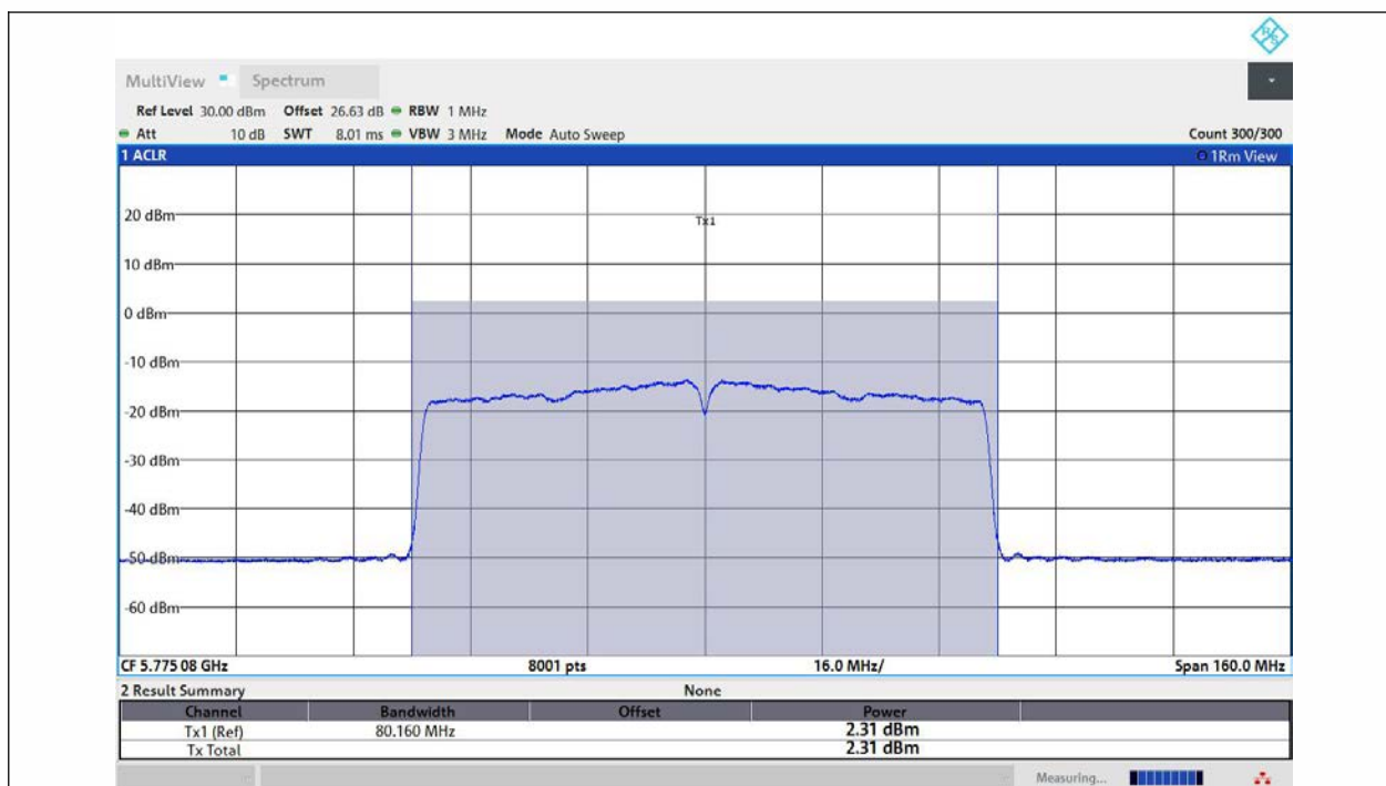
11AC80MIMO-Ant2-5775-PASS
