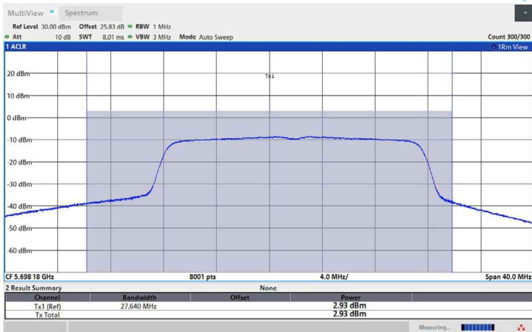
11AX20MIMO-Ant3-5700-TPC_H-PASS
