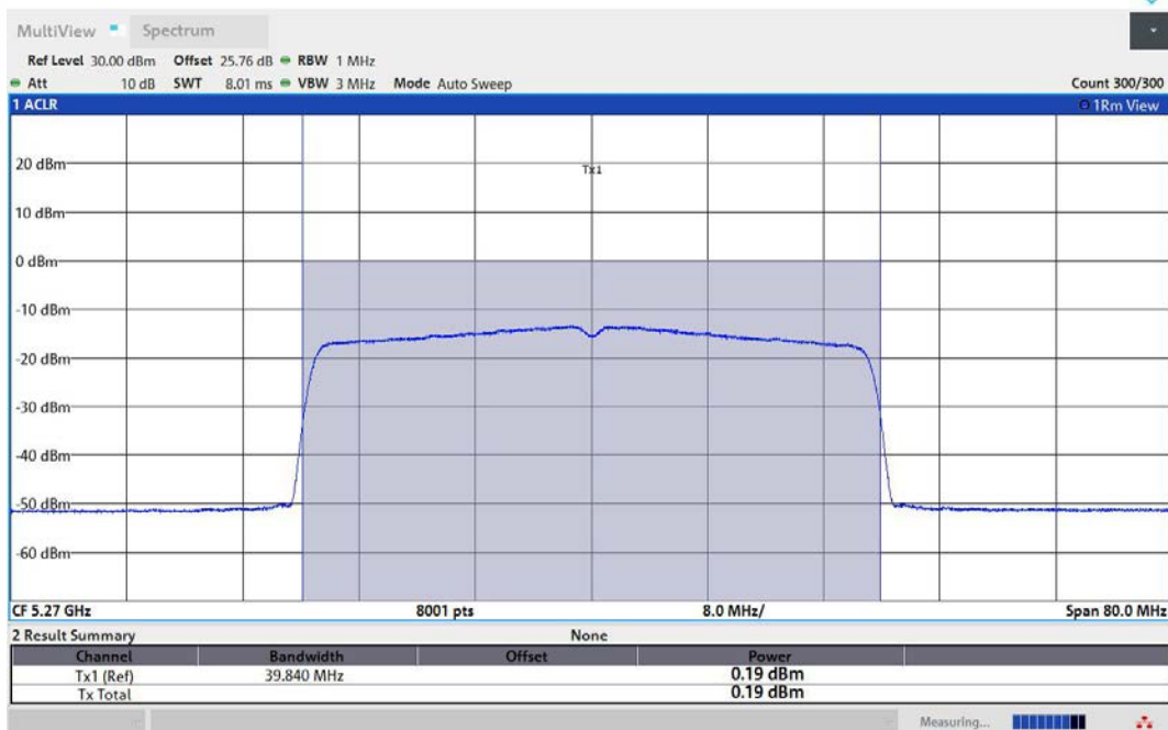
11AX40MIMO-Ant2-5270-TPC_L-PASS
