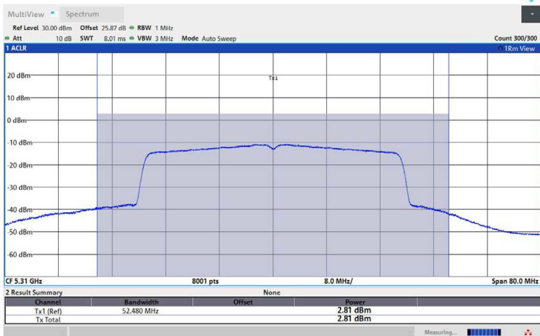
11AX40MIMO-Ant1-5310-TPC_H-PASS
