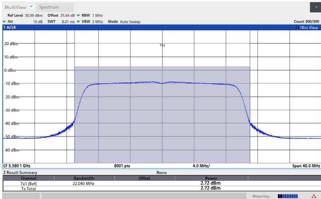
11AX20MIMO-Ant1-5580-TPC_H-PASS
