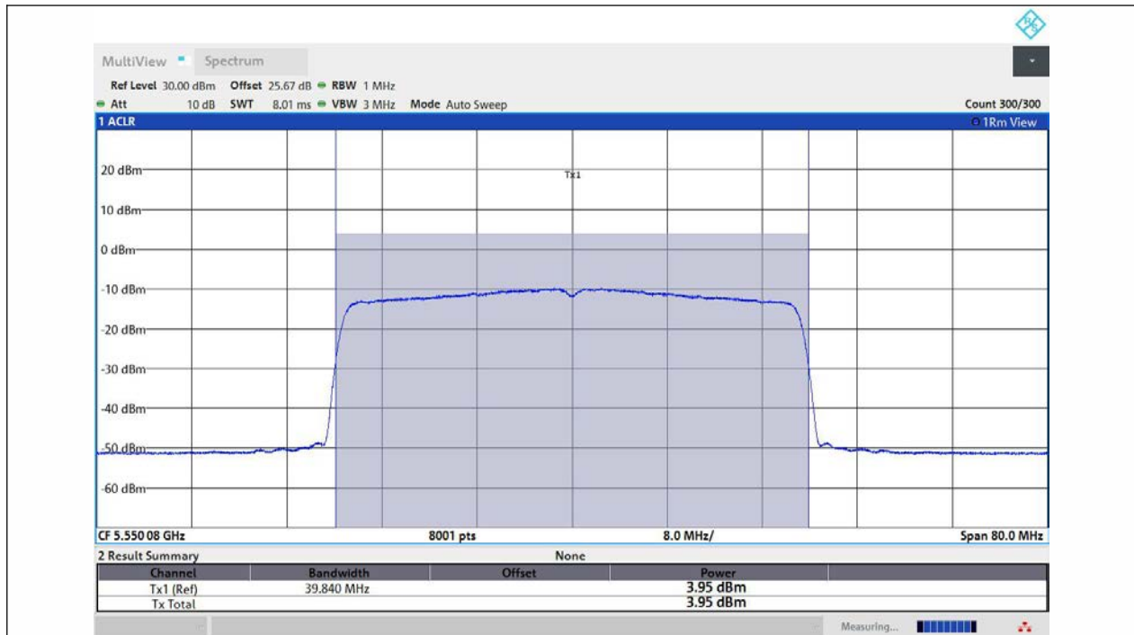
11AX40MIMO-Ant3-5550-TPC_H-PASS
