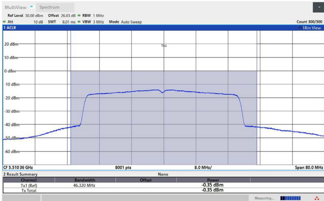
11AX40MIMO-Ant3-5510-TPC_L-PASS
