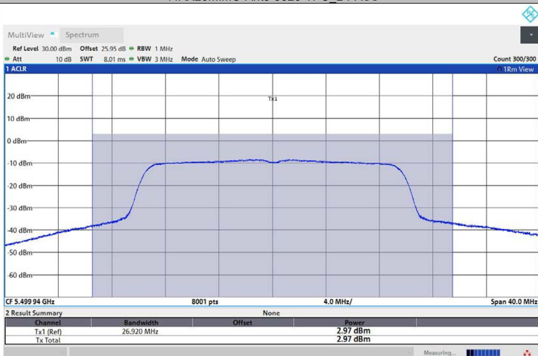
11AX20MIMO-Ant1-5500-TPC_H-PASS
