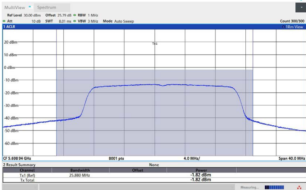
11AX20MIMO-Ant2-5700-TPC_L-PASS
