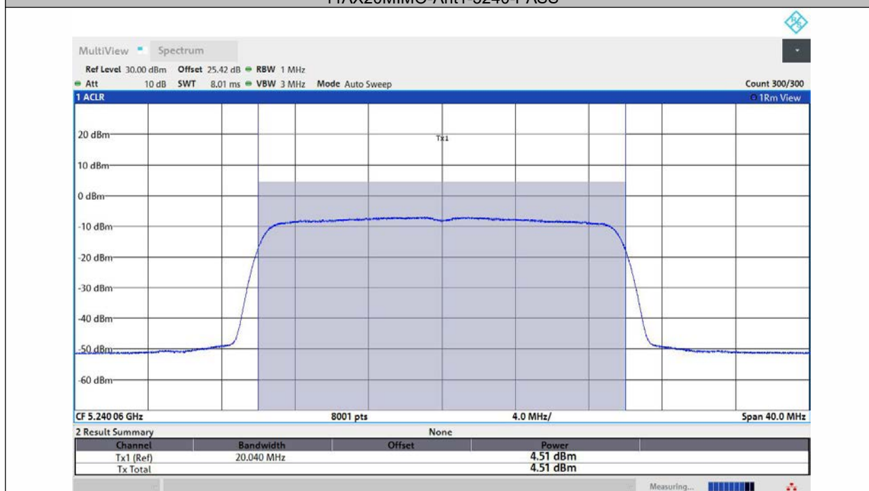
11AX20MIMO-Ant2-5240-PASS
