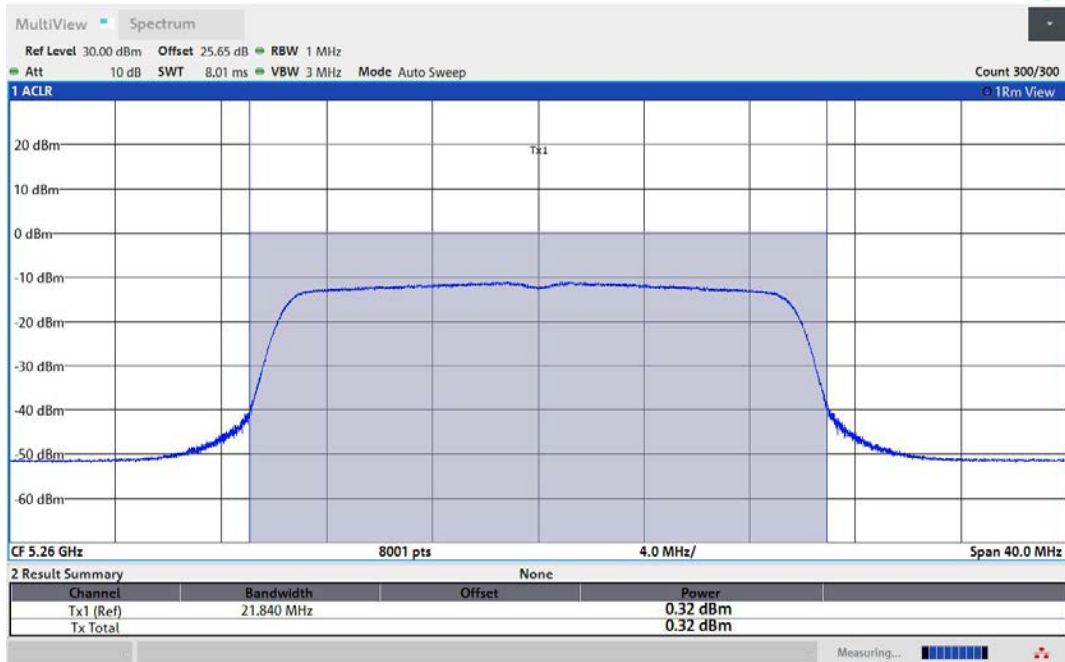
11AX20MIMO-Ant2-5260-TPC_L-PASS
