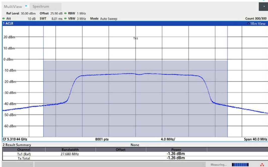
11AX20MIMO-Ant1-5320-TPC_L-PASS
