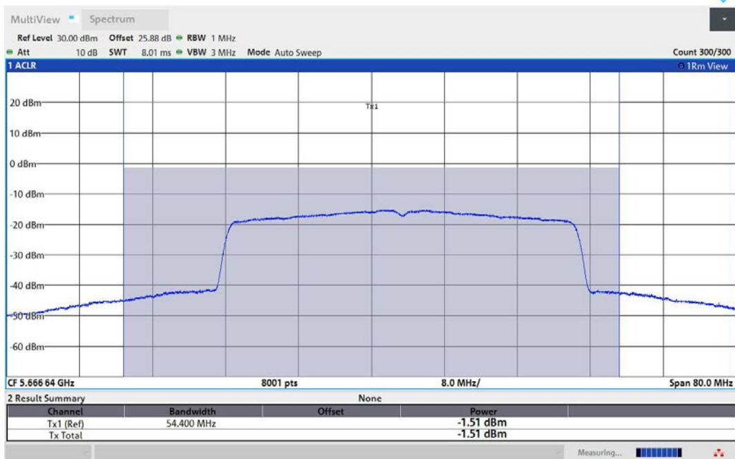
11AX40MIMO-Ant2-5670-TPC_L-PASS
