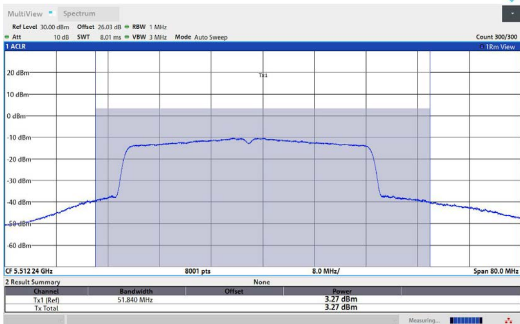
11AX40MIMO-Ant1-5510-TPC_H-PASS
