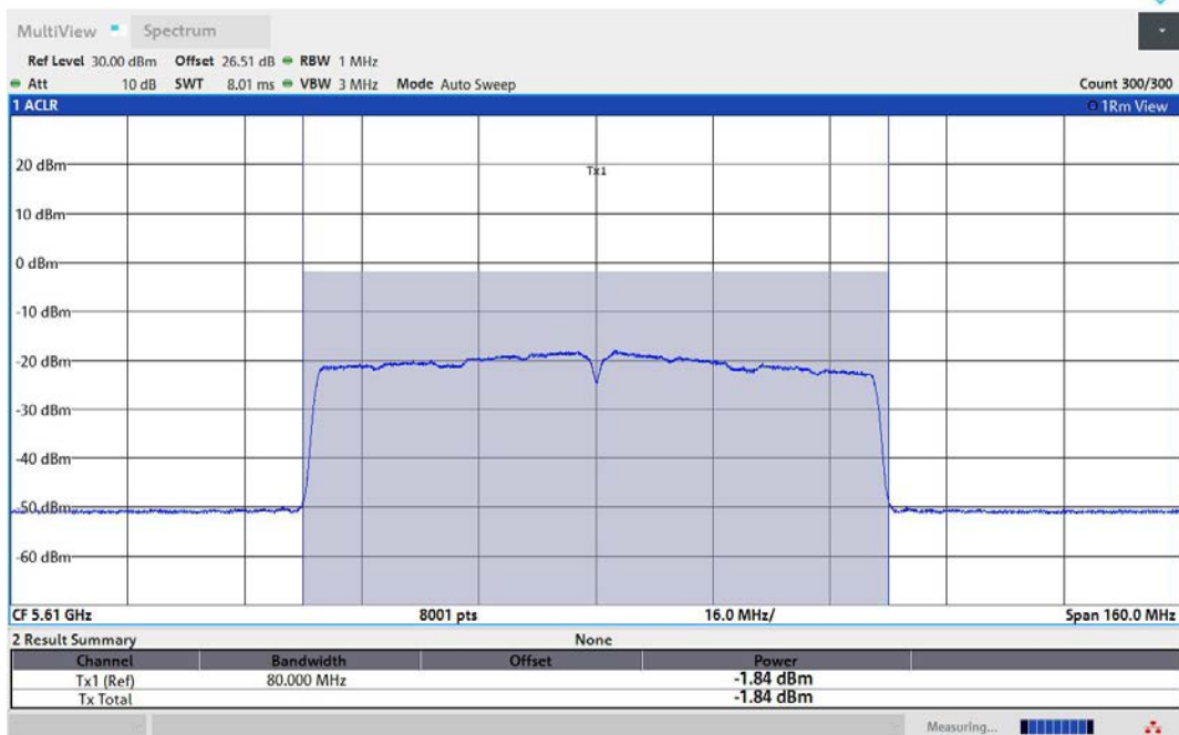
11AC80MIMO-Ant3-5610-TPC_L-PASS
