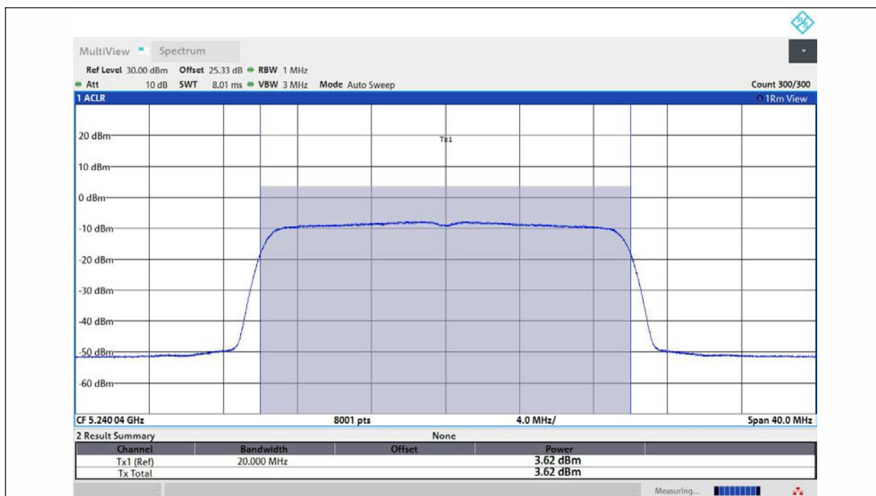
11AX20MIMO-Ant1-5240-PASS
