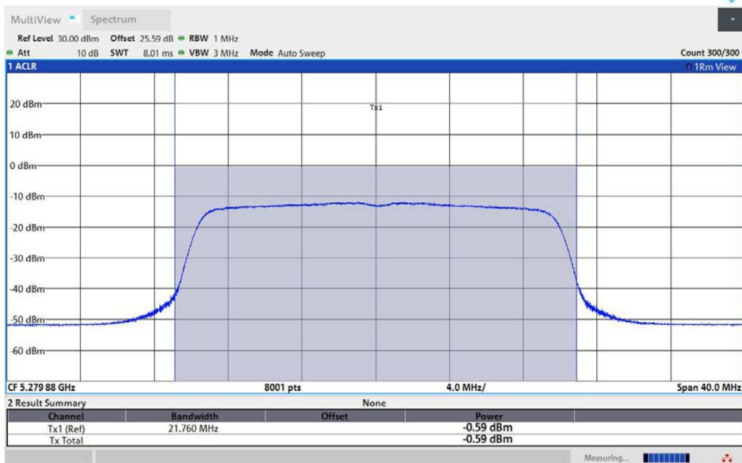
11AX20MIMO-Ant3-5280-TPC_L-PASS
