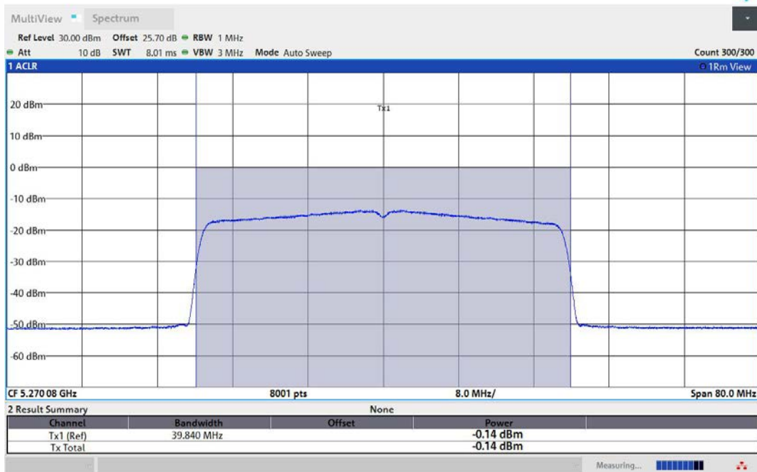
11AX40MIMO-Ant3-5270-TPC_L-PASS
