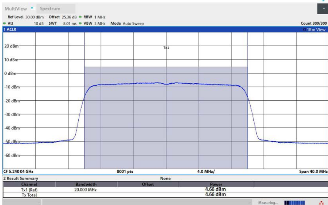
11AX20MIMO-Ant3-5240-PASS
