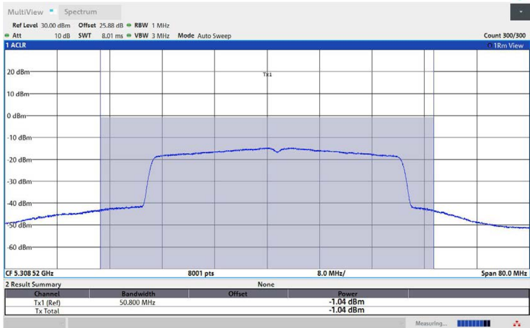
11AX40MIMO-Ant3-5310-TPC_L-PASS
