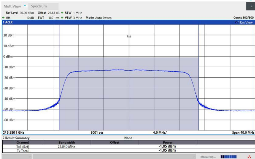
11AX20MIMO-Ant1-5580-TPC_L-PASS
