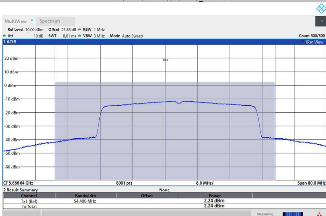
11AX40MIMO-Ant2-5670-TPC_H-PASS
