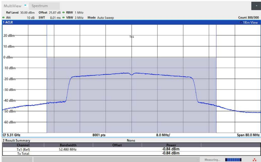
11AX40MIMO-Ant1-5310-TPC_L-PASS
