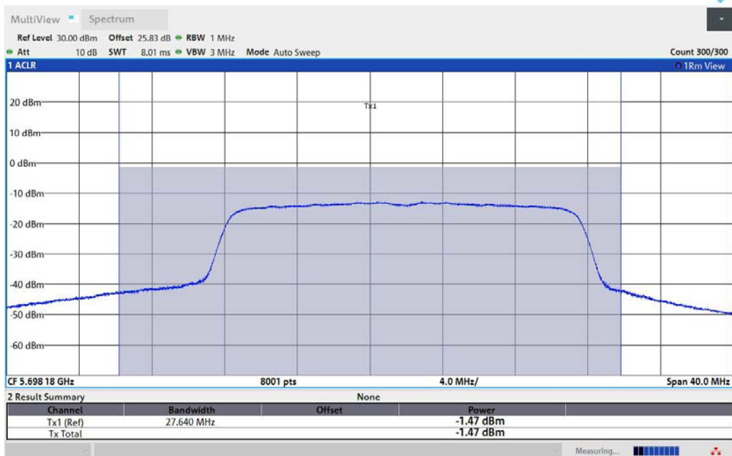
11AX20MIMO-Ant3-5700-TPC_L-PASS
