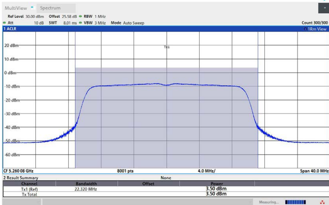
11AX20MIMO-Ant1-5260-TPC_H-PASS
