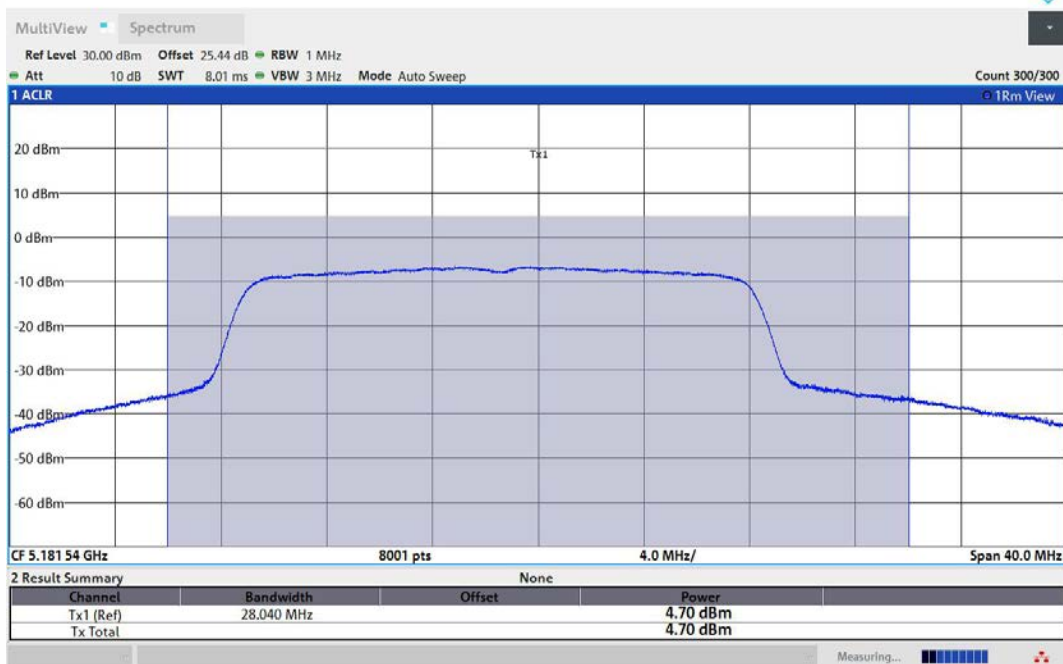
11AX20MIMO-Ant3-5180-PASS
