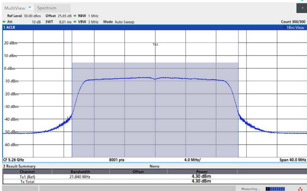
11AX20MIMO-Ant2-5260-TPC_H-PASS
