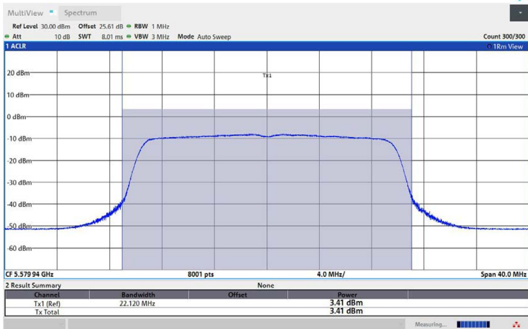
11AX20MIMO-Ant2-5580-TPC_H-PASS
