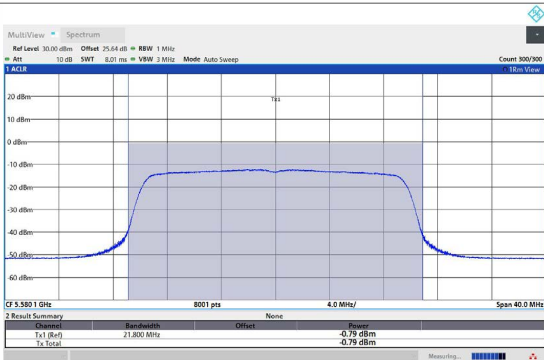
11AX20MIMO-Ant3-5580-TPC_L-PASS
