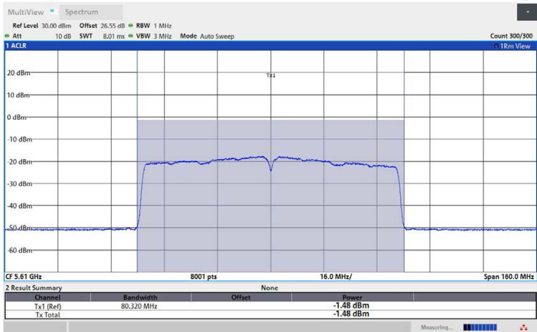
11AC80MIMO-Ant2-5610-TPC_L-PASS
