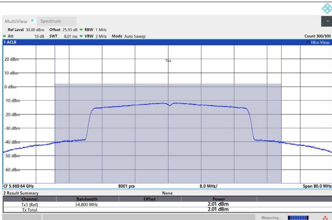
11AX40MIMO-Ant1-5670-TPC_H-PASS
