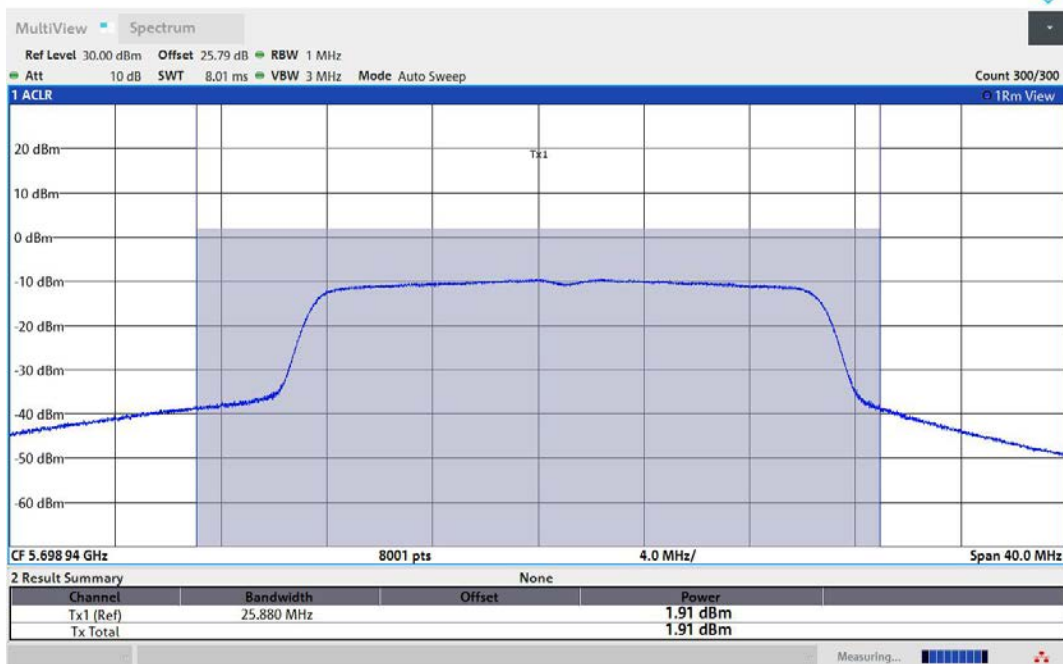
11AX20MIMO-Ant2-5700-TPC_H-PASS
