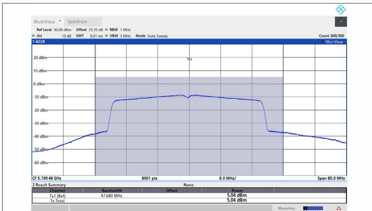
11AX40MIMO-Ant3-5190-PASS
