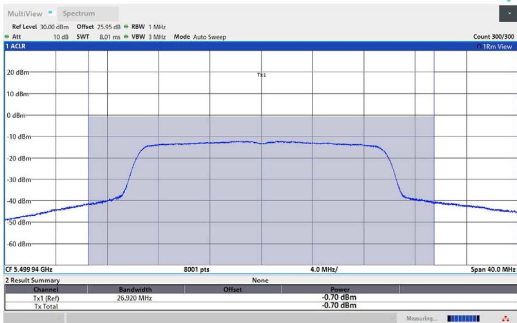
11AX20MIMO-Ant1-5500-TPC_L-PASS
