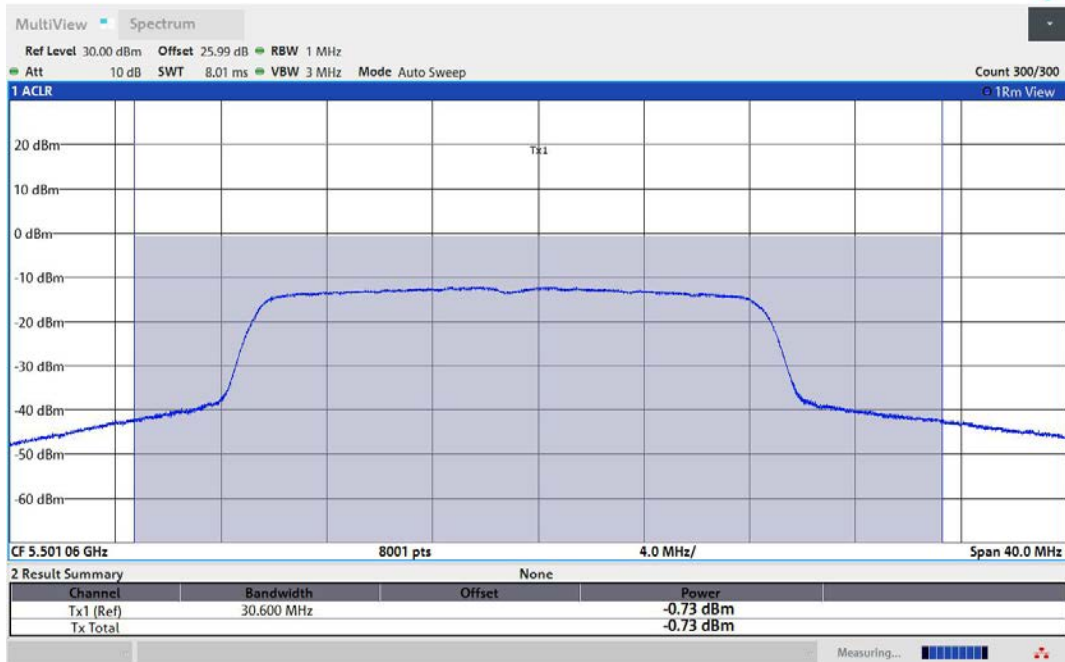
11AX20MIMO-Ant2-5500-TPC_L-PASS
