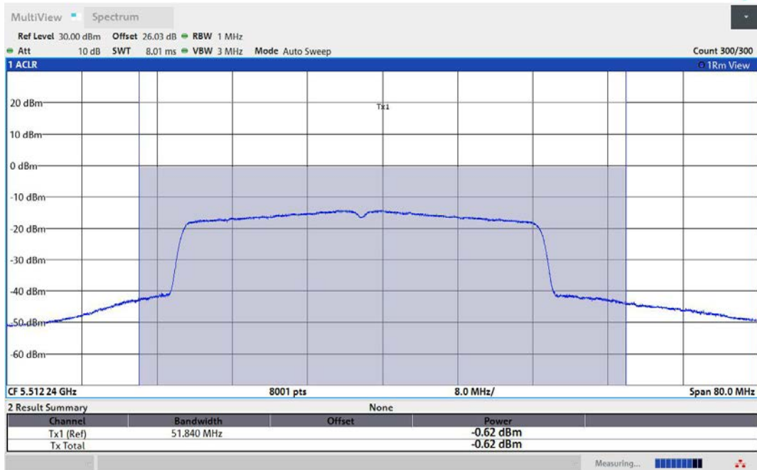
11AX40MIMO-Ant1-5510-TPC_L-PASS
