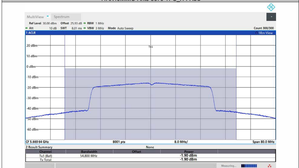
11AX40MIMO-Ant1-5670-TPC_L-PASS
