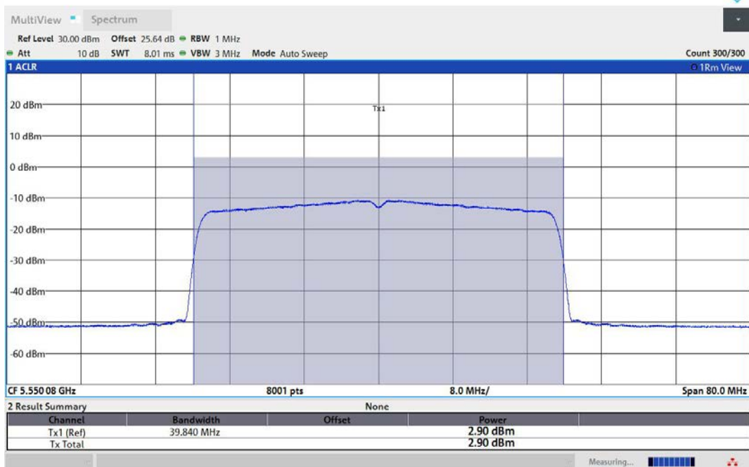
11AX40MIMO-Ant1-5550-TPC_H-PASS
