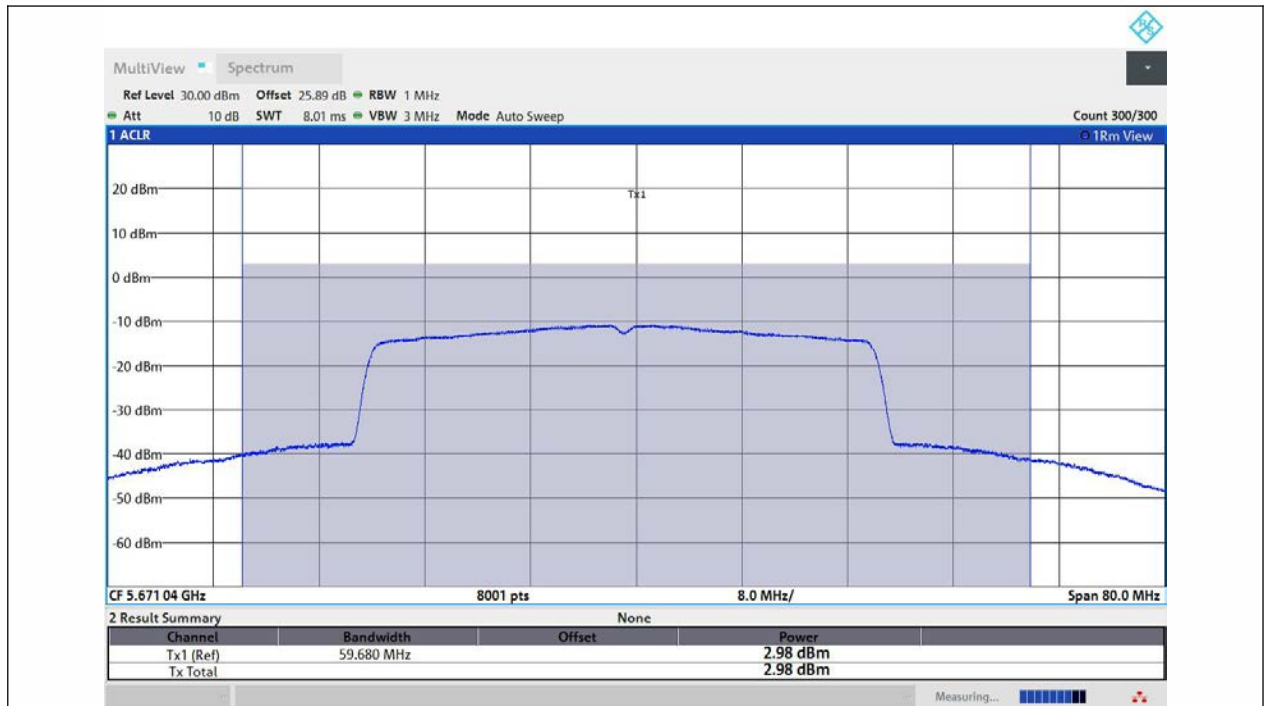
11AX40MIMO-Ant3-5670-TPC_H-PASS
