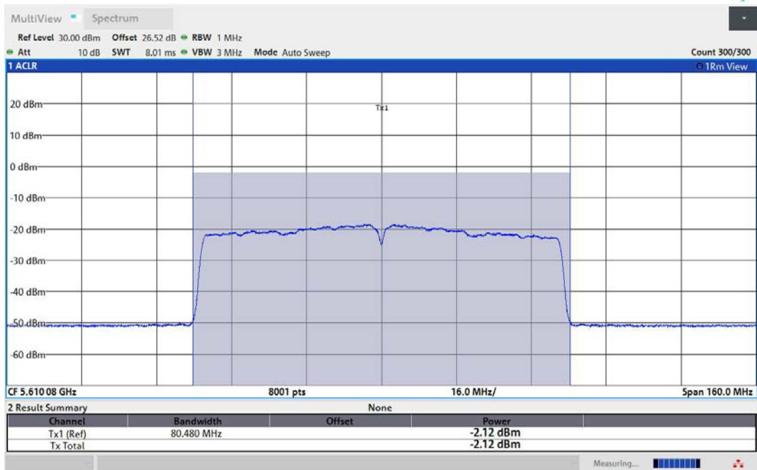
11AC80MIMO-Ant1-5610-TPC_L-PASS
