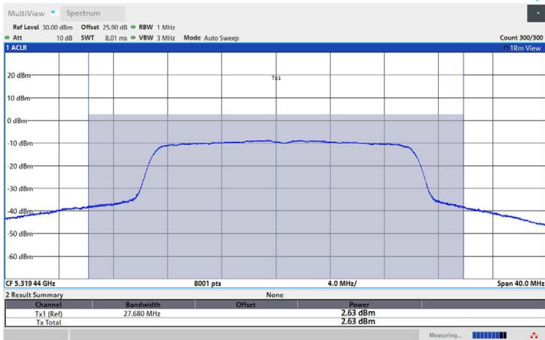
11AX20MIMO-Ant1-5320-TPC_H-PASS
