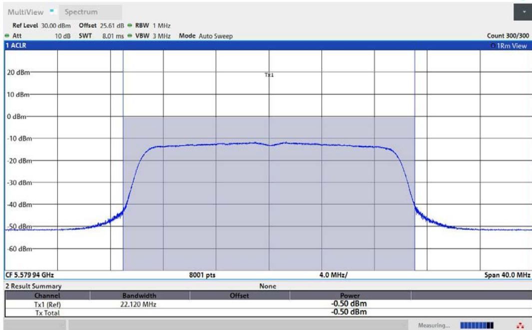
11AX20MIMO-Ant2-5580-TPC_L-PASS
