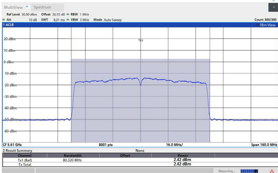
11AC80MIMO-Ant2-5610-TPC_H-PASS
