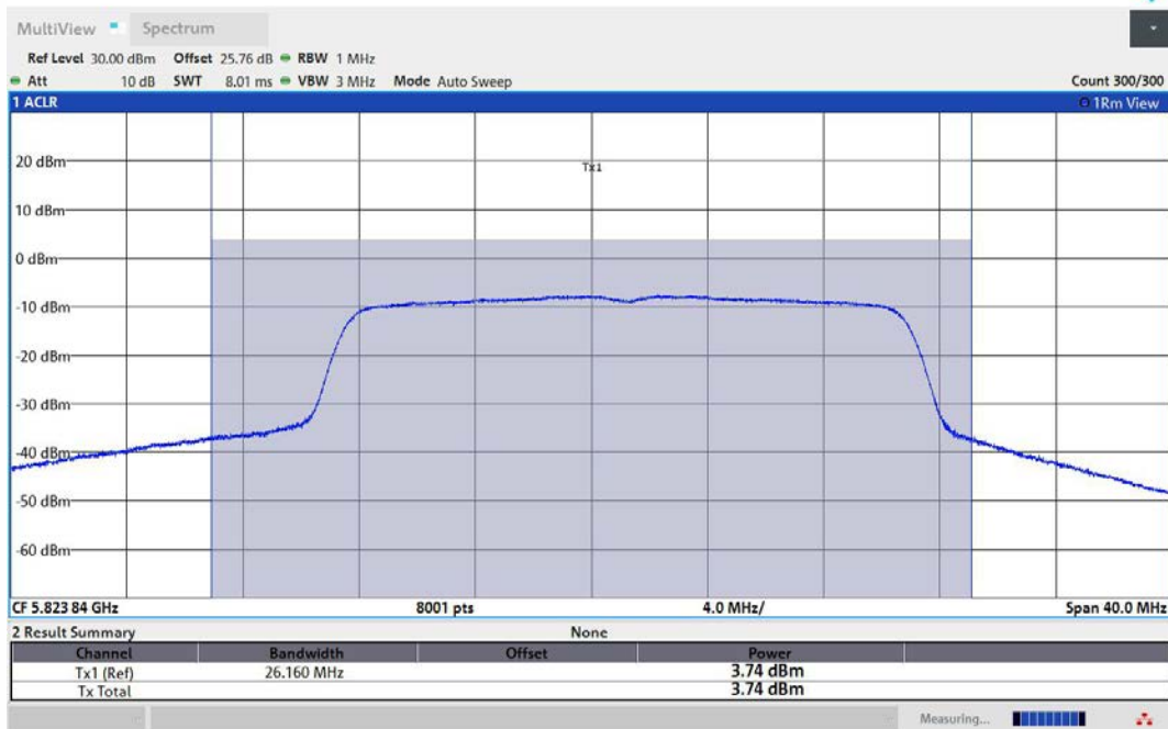
11AX20MIMO-Ant3-5825-PASS
