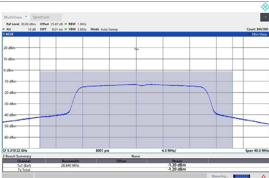
11AX20MIMO-Ant3-5320-TPC_L-PASS
