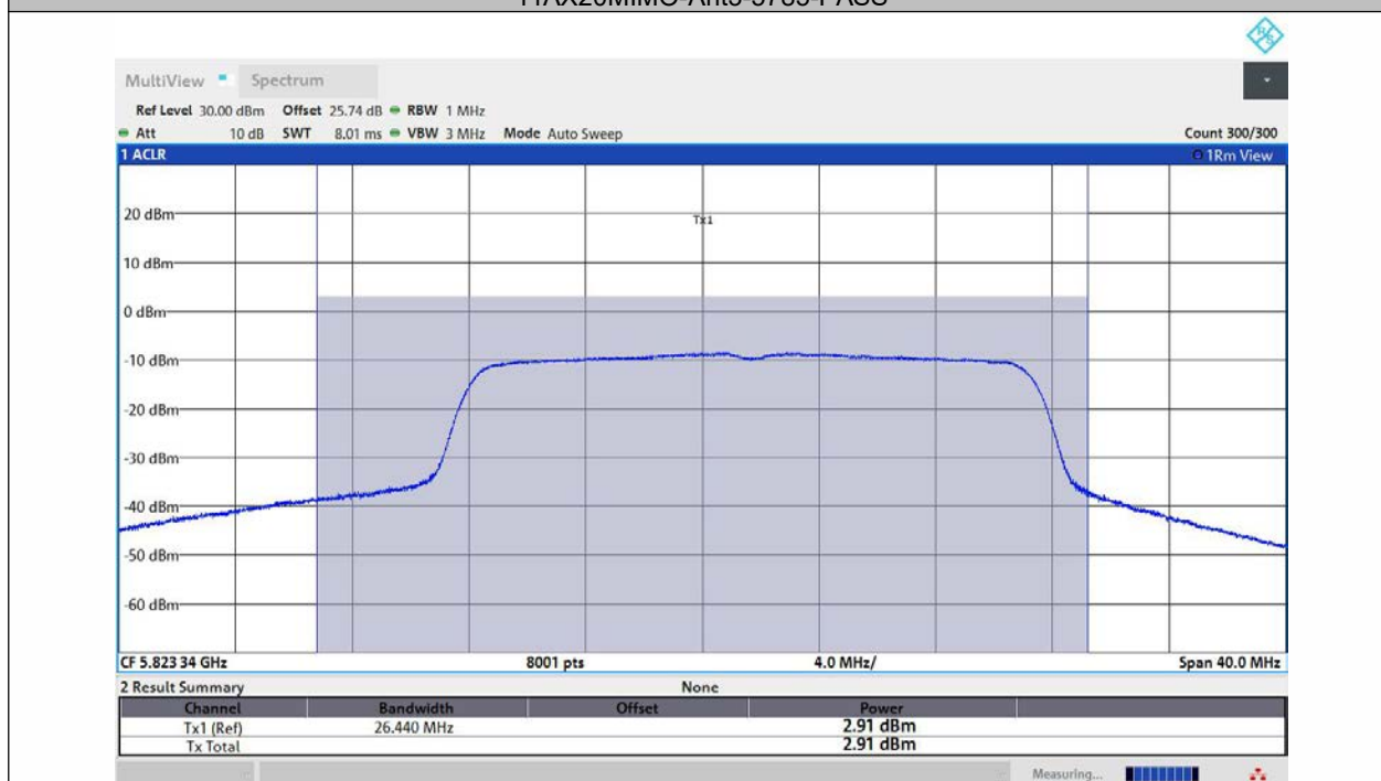
11AX20MIMO-Ant1-5825-PASS
