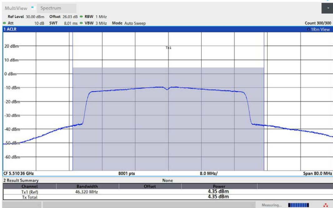
11AX40MIMO-Ant3-5510-TPC_H-PASS
