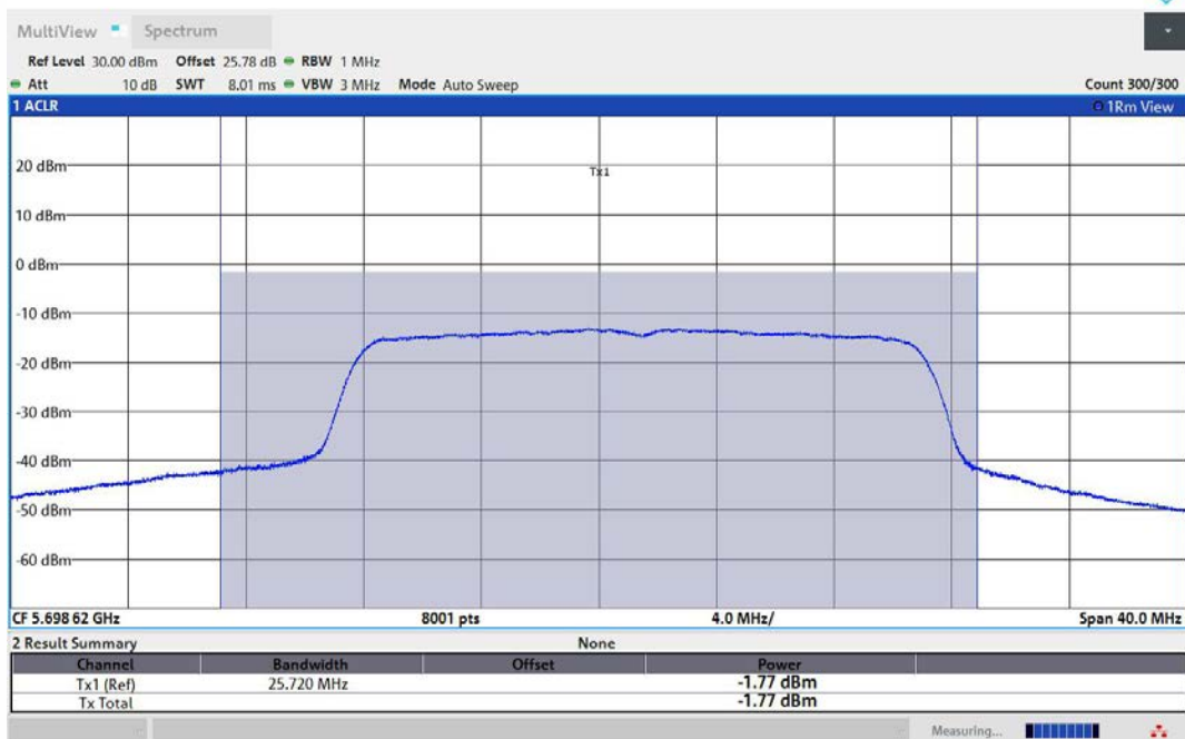
11AX20MIMO-Ant1-5700-TPC_L-PASS
