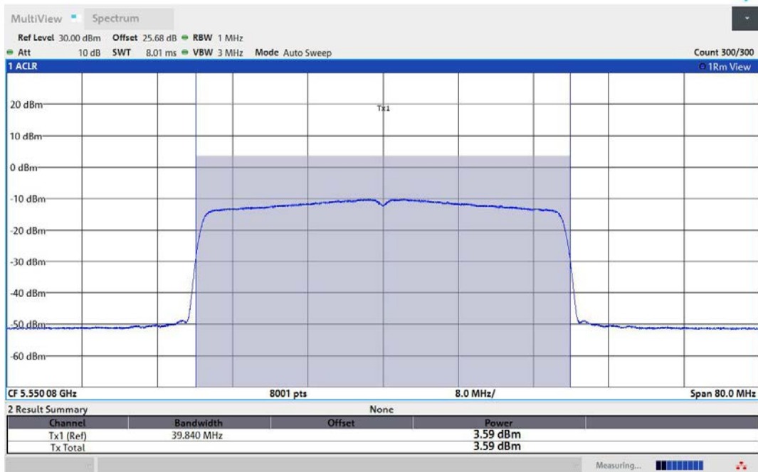
11AX40MIMO-Ant2-5550-TPC_H-PASS
