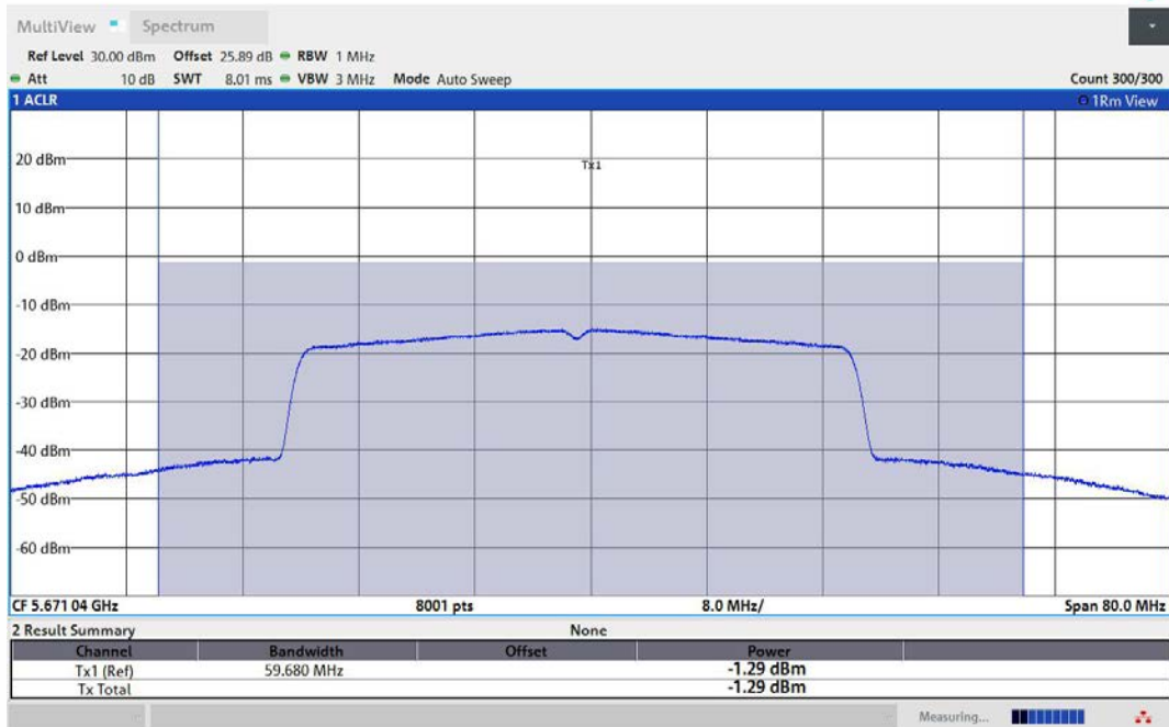
11AX40MIMO-Ant3-5670-TPC_L-PASS
