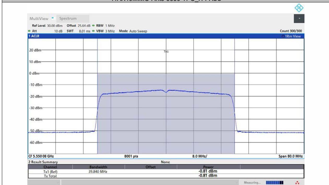
11AX40MIMO-Ant1-5550-TPC_L-PASS
