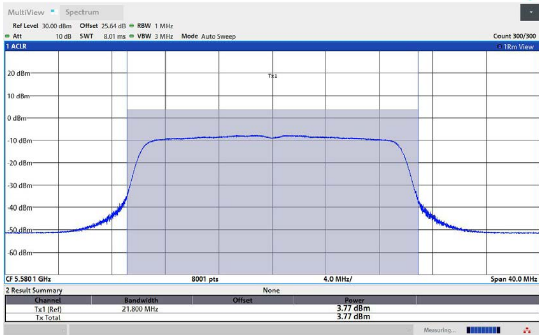
11AX20MIMO-Ant3-5580-TPC_H-PASS
