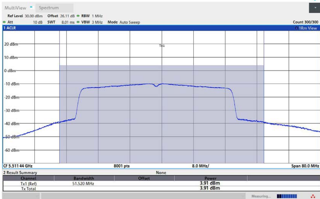
11AX40MIMO-Ant2-5510-TPC_H-PASS
