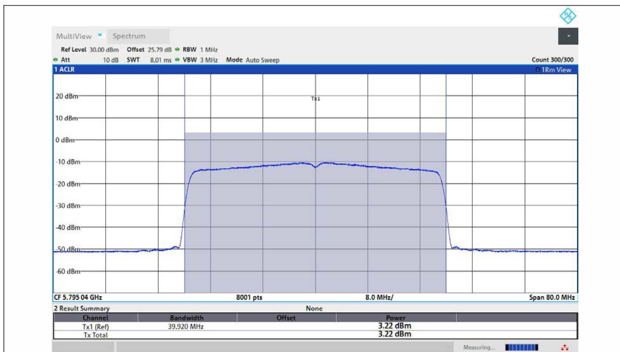
11AX40MIMO-Ant2-5795-PASS
