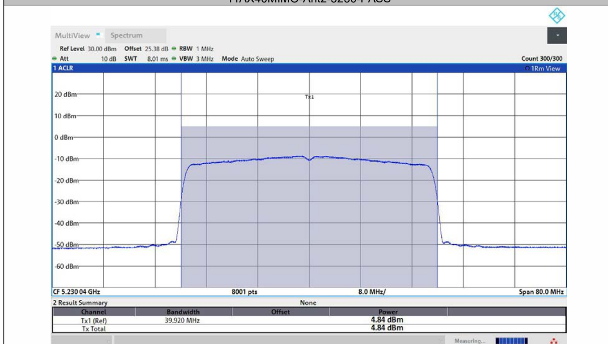
11AX40MIMO-Ant3-5230-PASS
