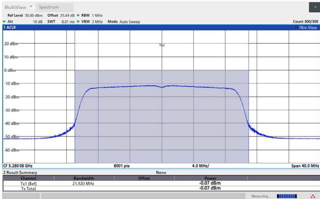
11AX20MIMO-Ant2-5280-TPC_L-PASS
