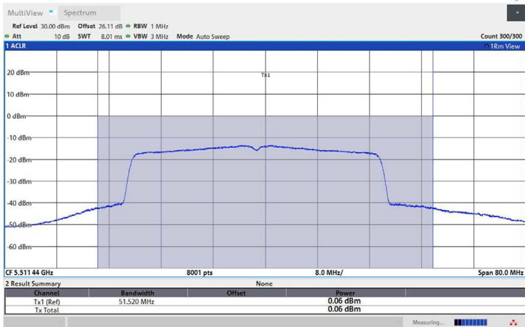
11AX40MIMO-Ant2-5510-TPC_L-PASS
