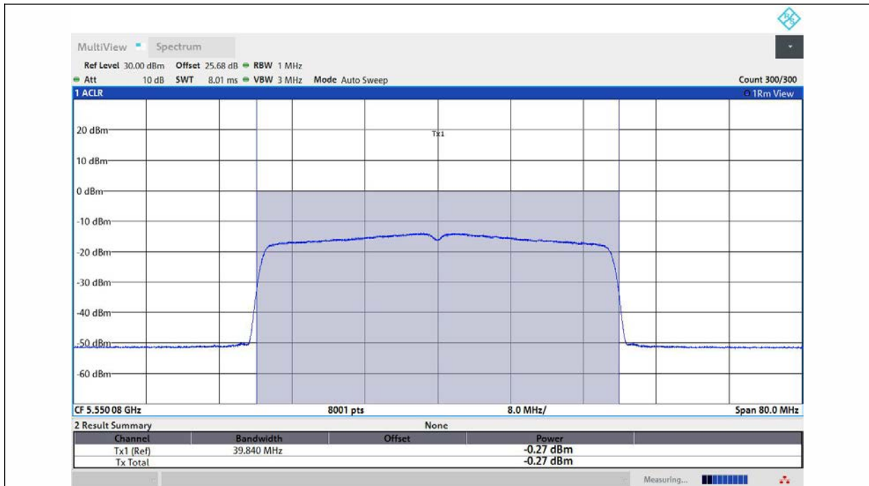
11AX40MIMO-Ant2-5550-TPC_L-PASS
