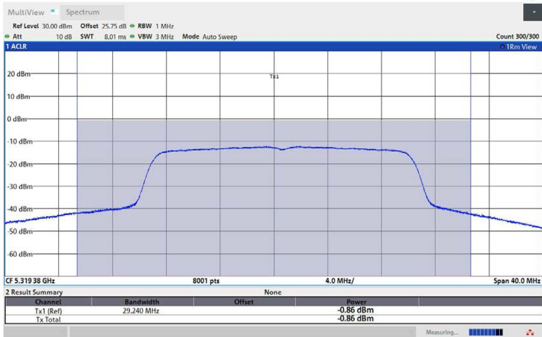
11AX20MIMO-Ant2-5320-TPC_L-PASS
