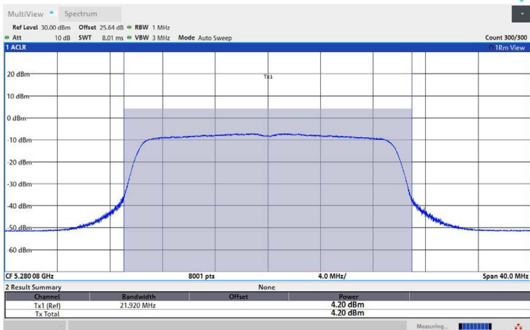
11AX20MIMO-Ant2-5280-TPC_H-PASS
