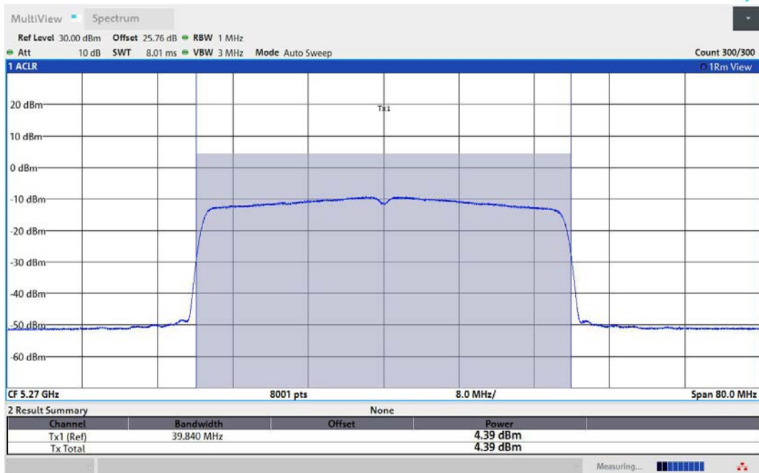
11AX40MIMO-Ant2-5270-TPC_H-PASS
