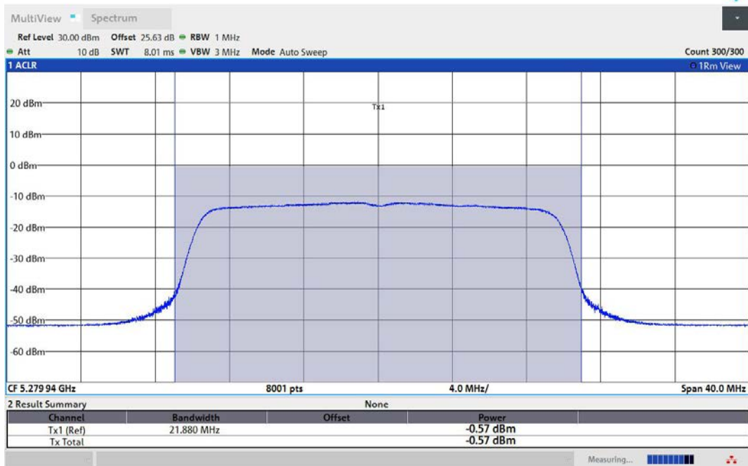
11AX20MIMO-Ant1-5280-TPC_L-PASS
