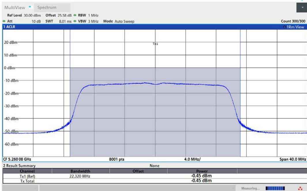
11AX20MIMO-Ant1-5260-TPC_L-PASS
