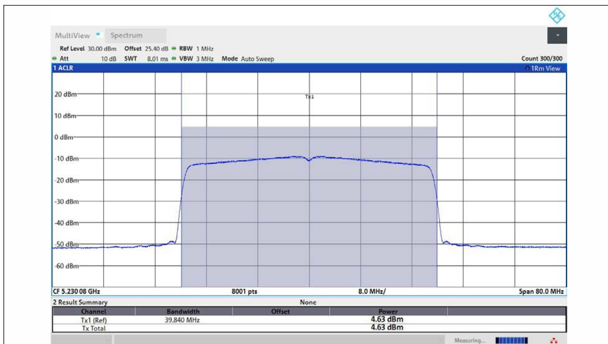
11AX40MIMO-Ant2-5230-PASS
