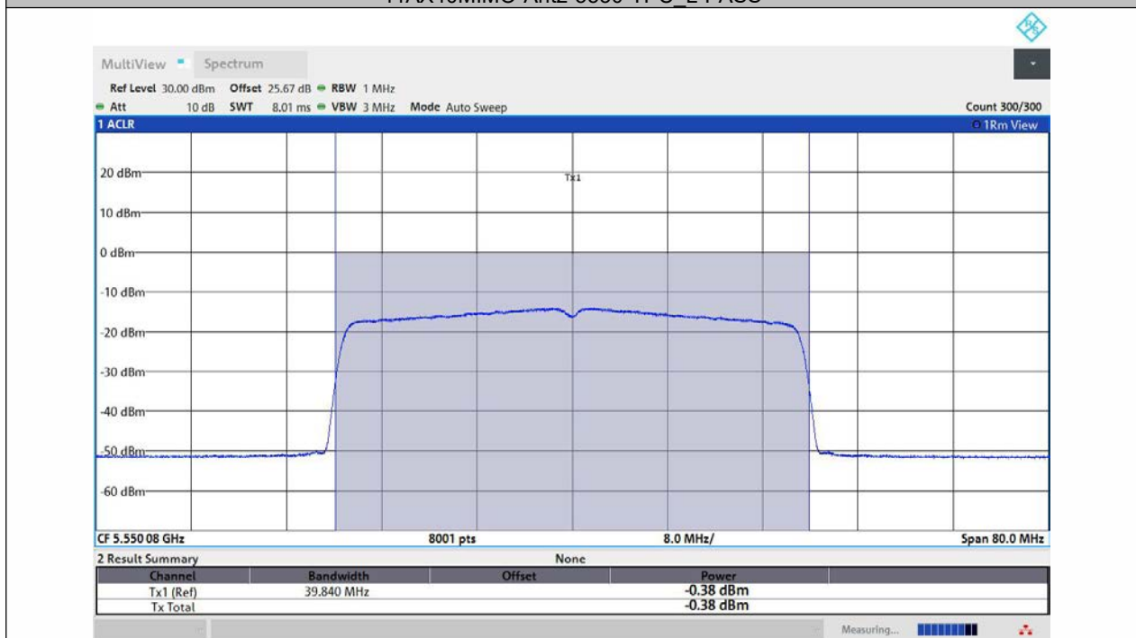
11AX40MIMO-Ant3-5550-TPC_L-PASS
