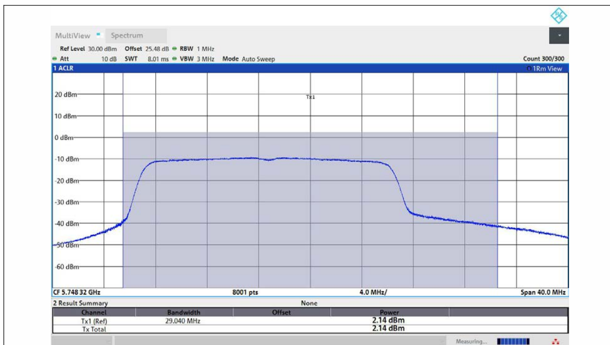
11AX20MIMO-Ant2-5745-PASS
