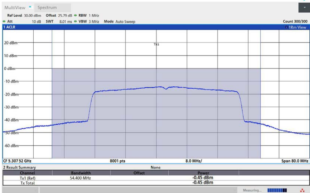
11AX40MIMO-Ant2-5310-TPC_L-PASS
