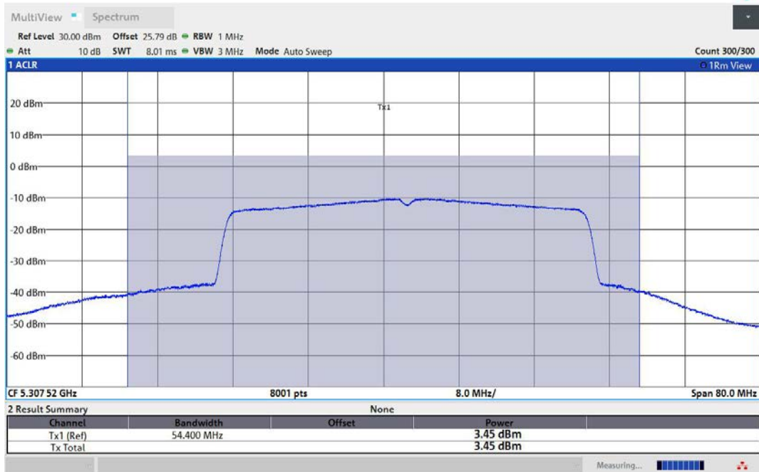
11AX40MIMO-Ant2-5310-TPC_H-PASS
