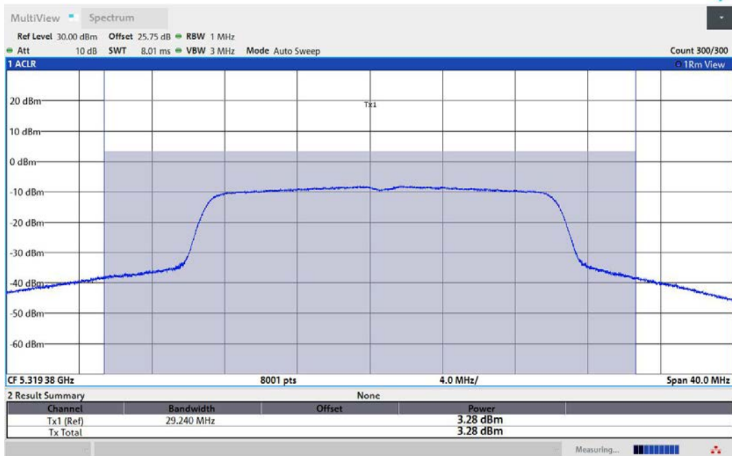
11AX20MIMO-Ant2-5320-TPC_H-PASS
