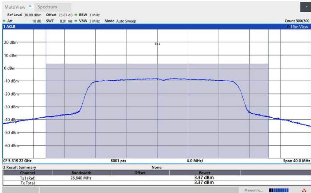
11AX20MIMO-Ant3-5320-TPC_H-PASS
