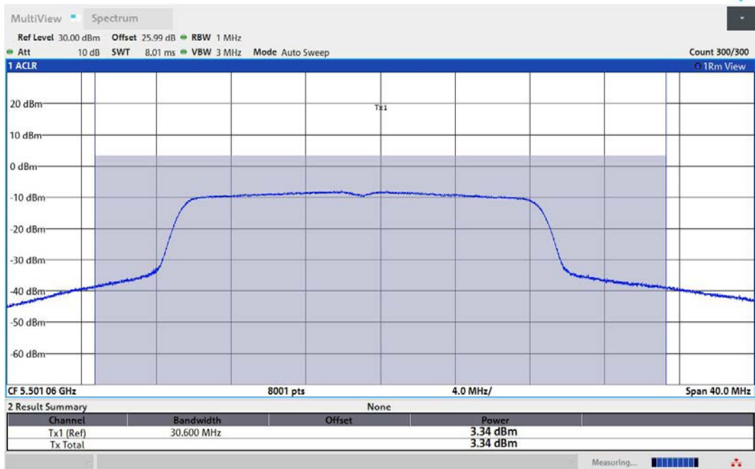
11AX20MIMO-Ant2-5500-TPC_H-PASS
