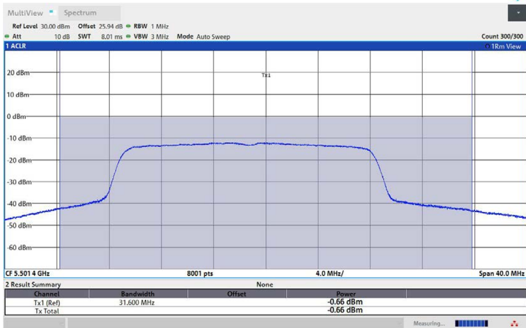
11AX20MIMO-Ant3-5500-TPC_L-PASS
