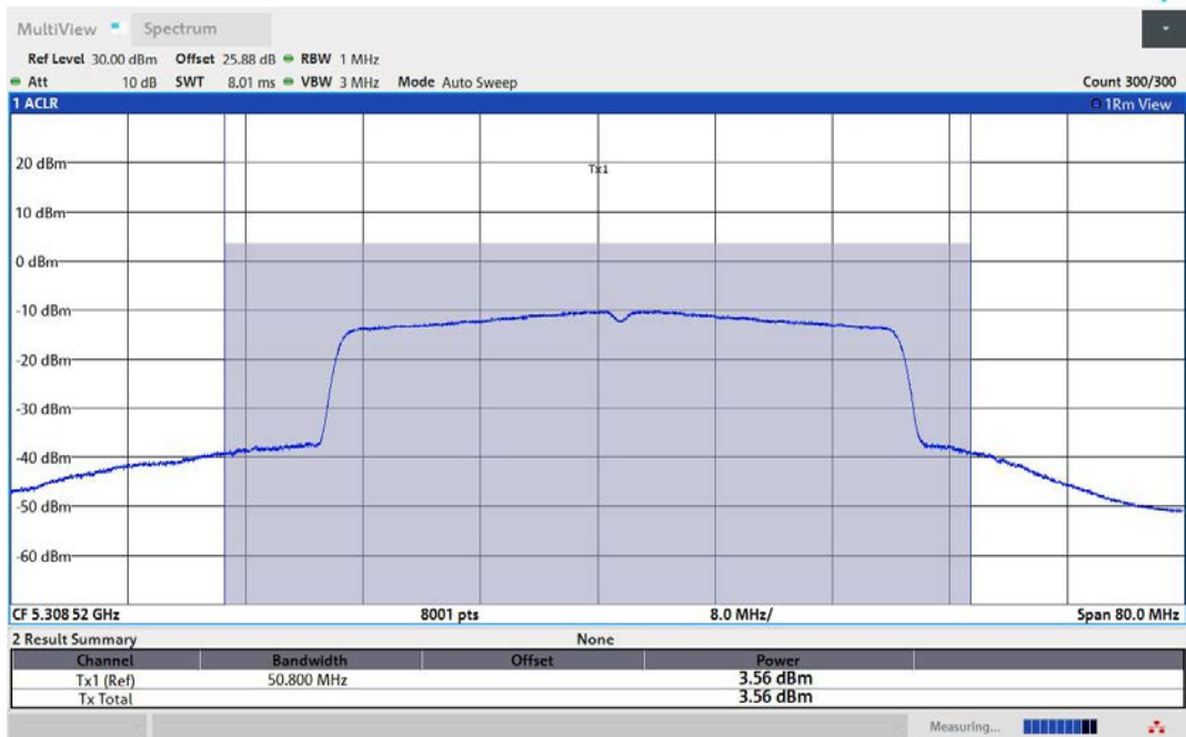
11AX40MIMO-Ant3-5310-TPC_H-PASS
