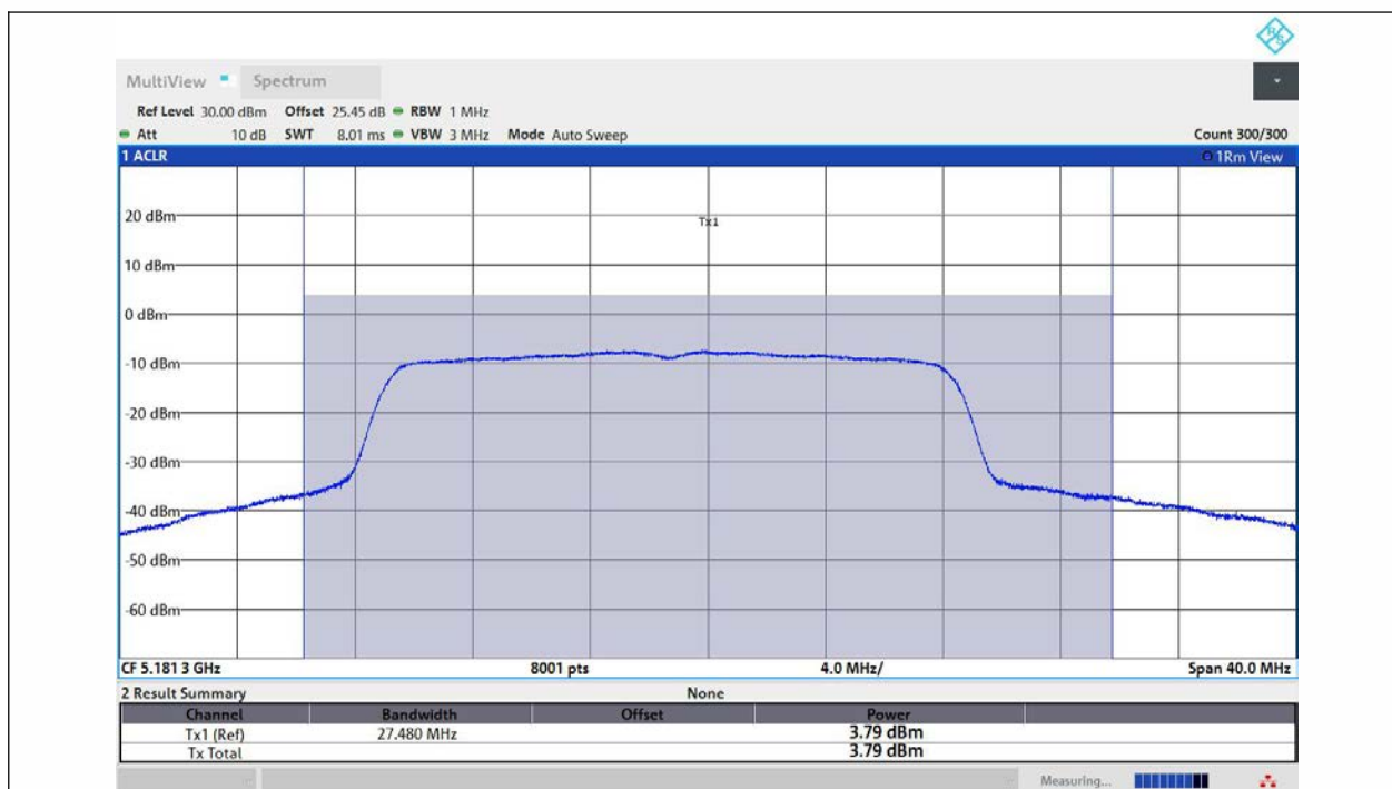
11AX20MIMO-Ant1-5180-PASS
