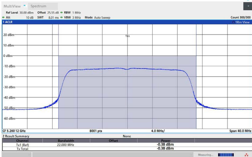
11AX20MIMO-Ant3-5260-TPC_L-PASS
