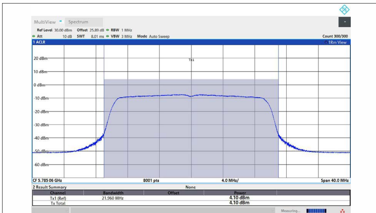
11AX20MIMO-Ant3-5785-PASS
