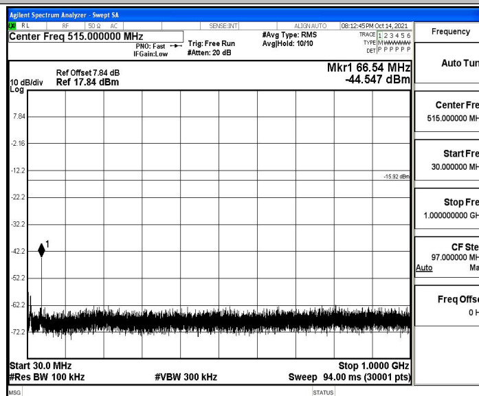
11B_Ant4_2437_30~1000
