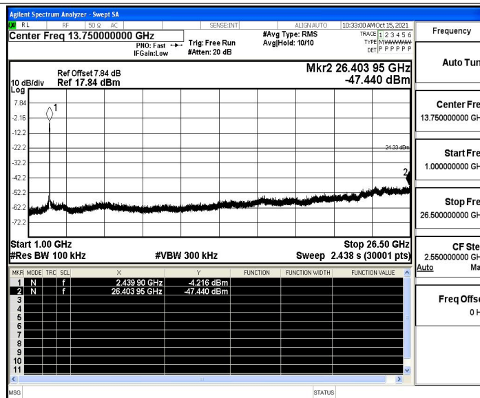
11N40SISO_Ant3_2452_0~Reference
