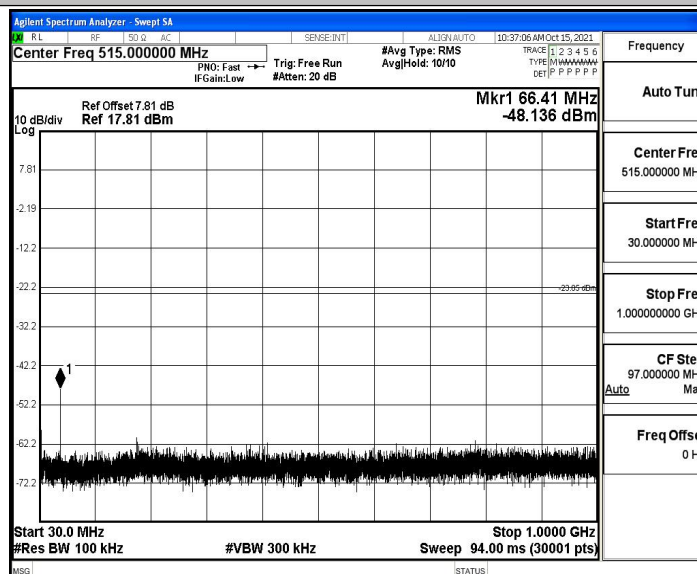
11N40SISO_Ant3_2452_30~1000
