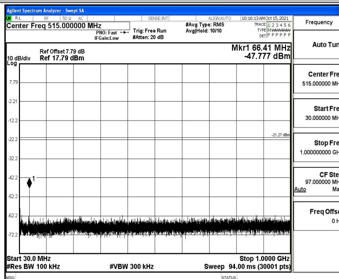
11N20SISO_Ant3_2412_30~1000
