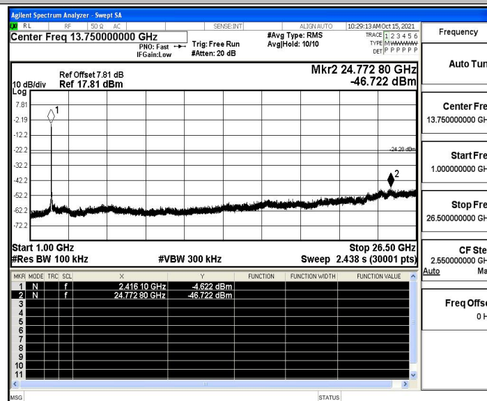
11N40SISO_Ant3_2422_1000~26500
