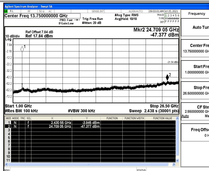
11G_Ant4_2437_1000~26500
