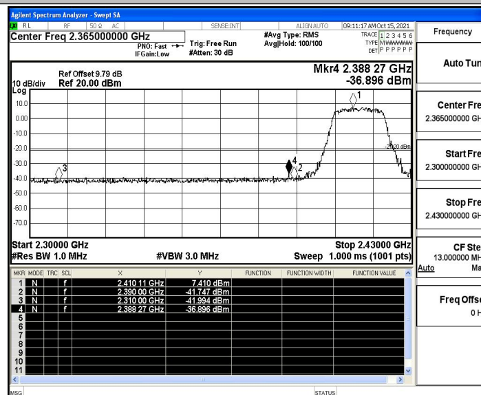
11N20SISO_Ant4_Low_2412_Peak
