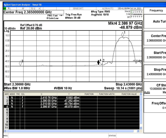
11B_Ant4_Low_2412_Peak
