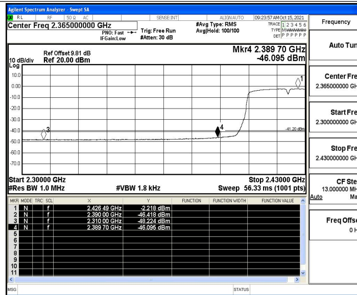
11N40SISO_Ant4_Low_2422_Peak
