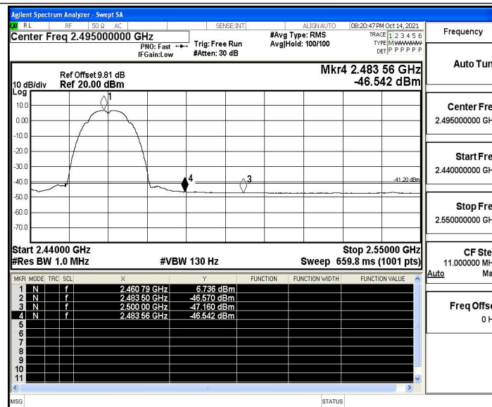
11B_Ant4_High_2462_Peak
