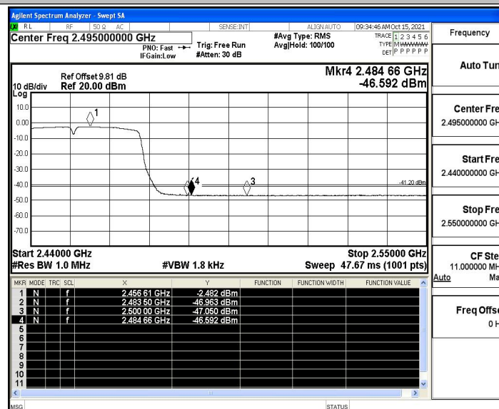
11N40SISO_Ant4_High_2452_AV
