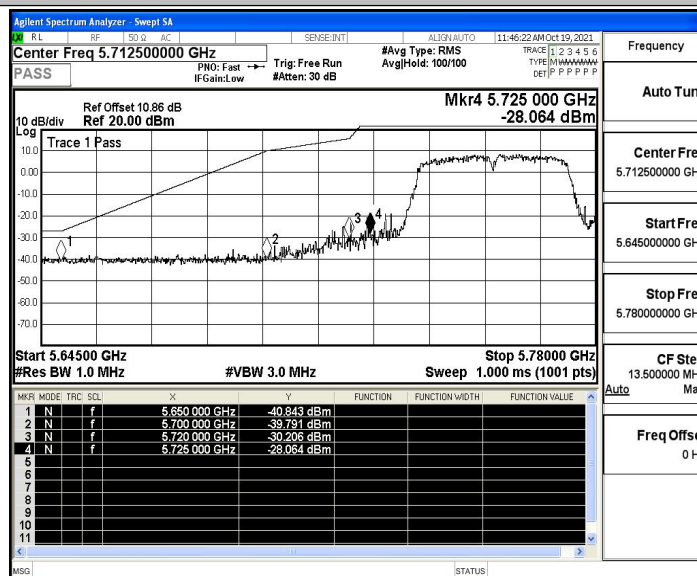
11N40SISO_Ant3_Low_5755_Peak
