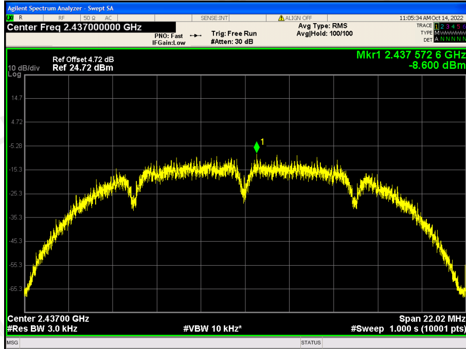
CH06: 2437MHz
