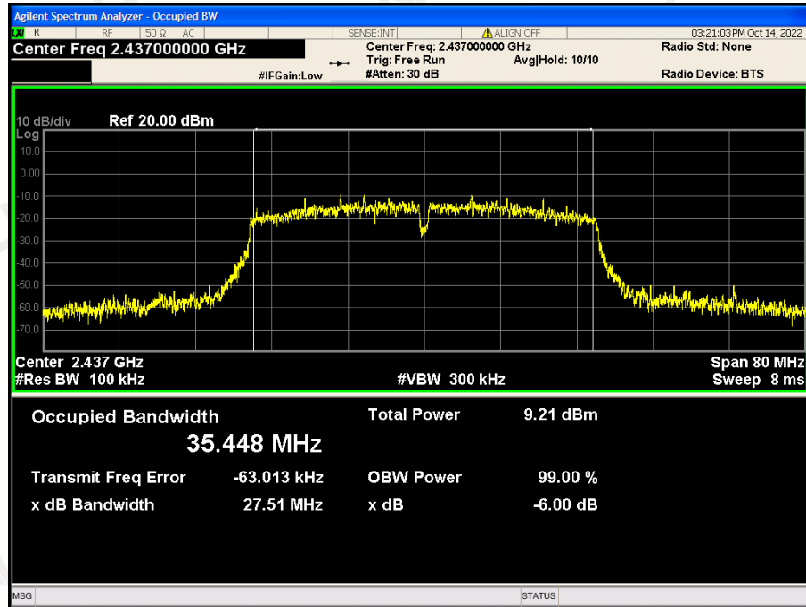
CH06: 2437MHz
