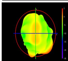
Phi=90 freq=2440MHz
