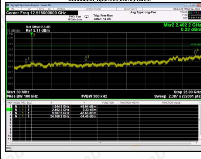
Conducted Spurious,3DH5,Lowest
