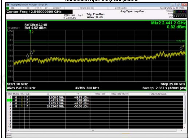
Conducted Spurious,3DH5,Middle
