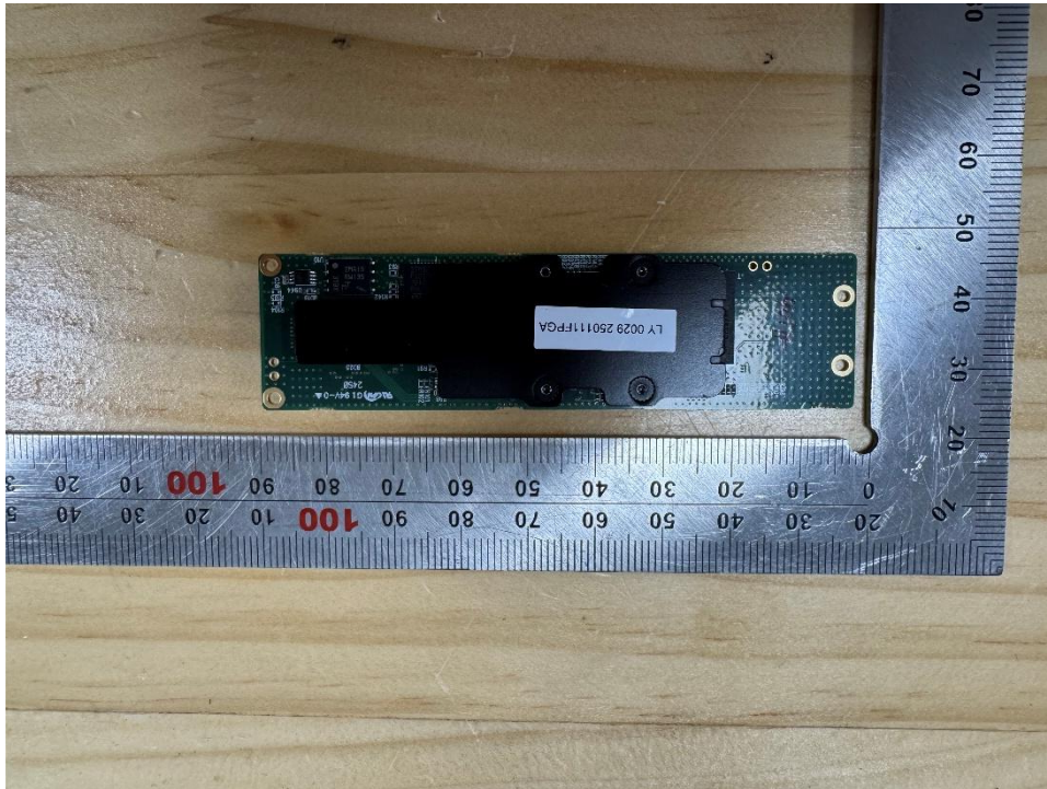
Front View of Camera Control Board
