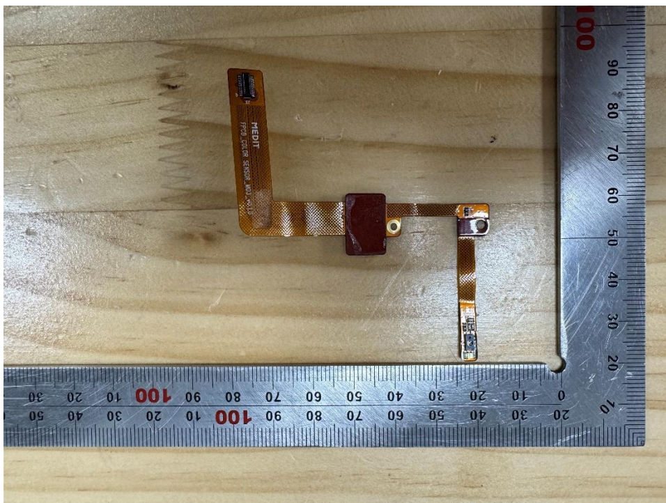
Rear View of Color Sensor Board
