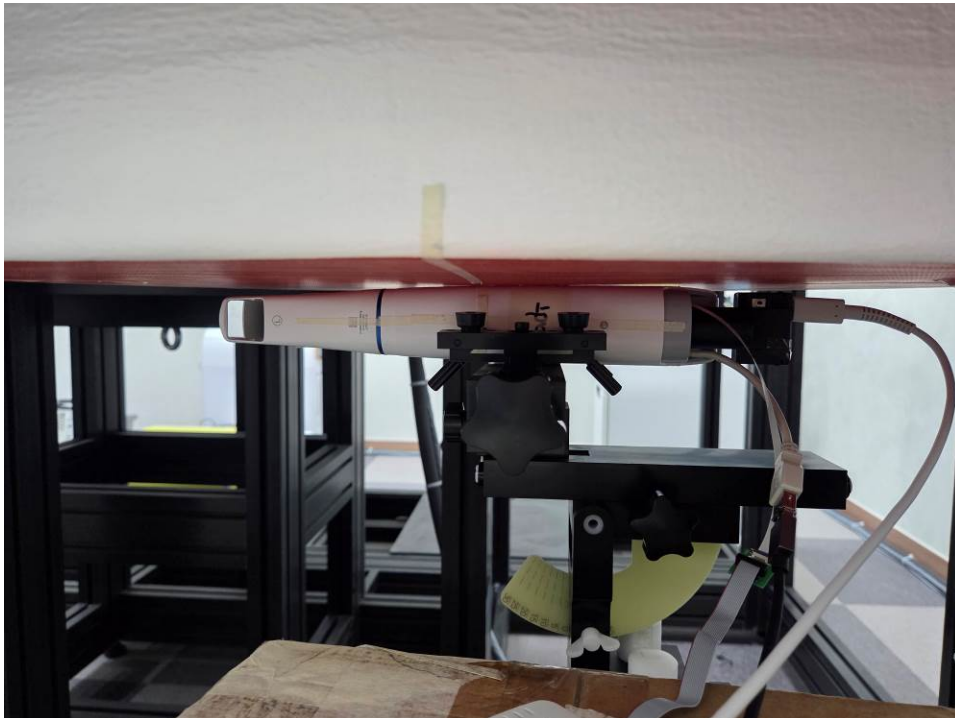
Right side of EUT, MIMO, Test separation distance : 0 mm
