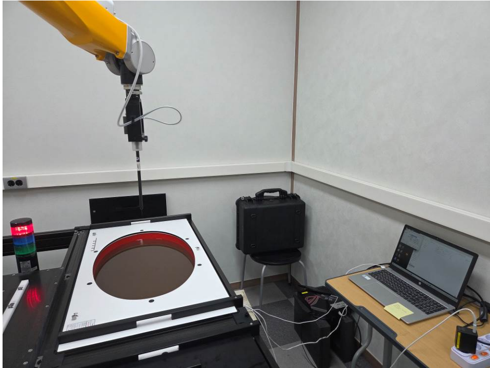
View of SAR Test Setup
