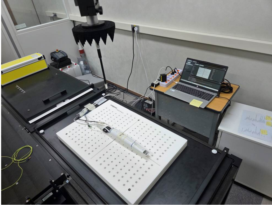
Front side of EUT, MIMO, Test separation distance : 2 mm
