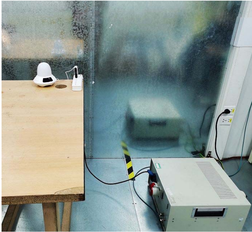
Conducted Emission Test Setup:
