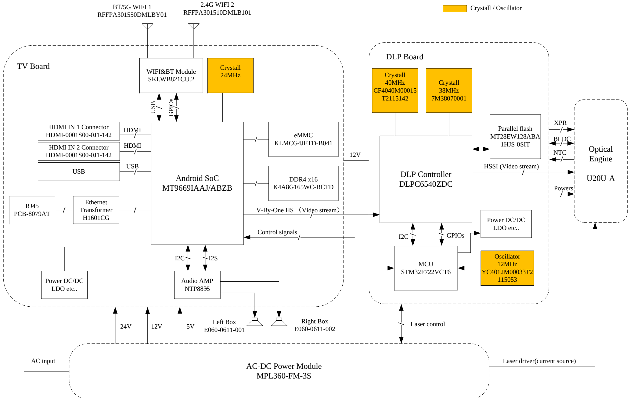
PE-LT002_Block Diagram
