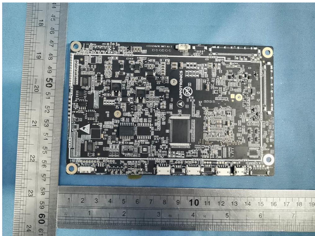
INTERNAL VIEW OF EUT (FIGURE 21)
