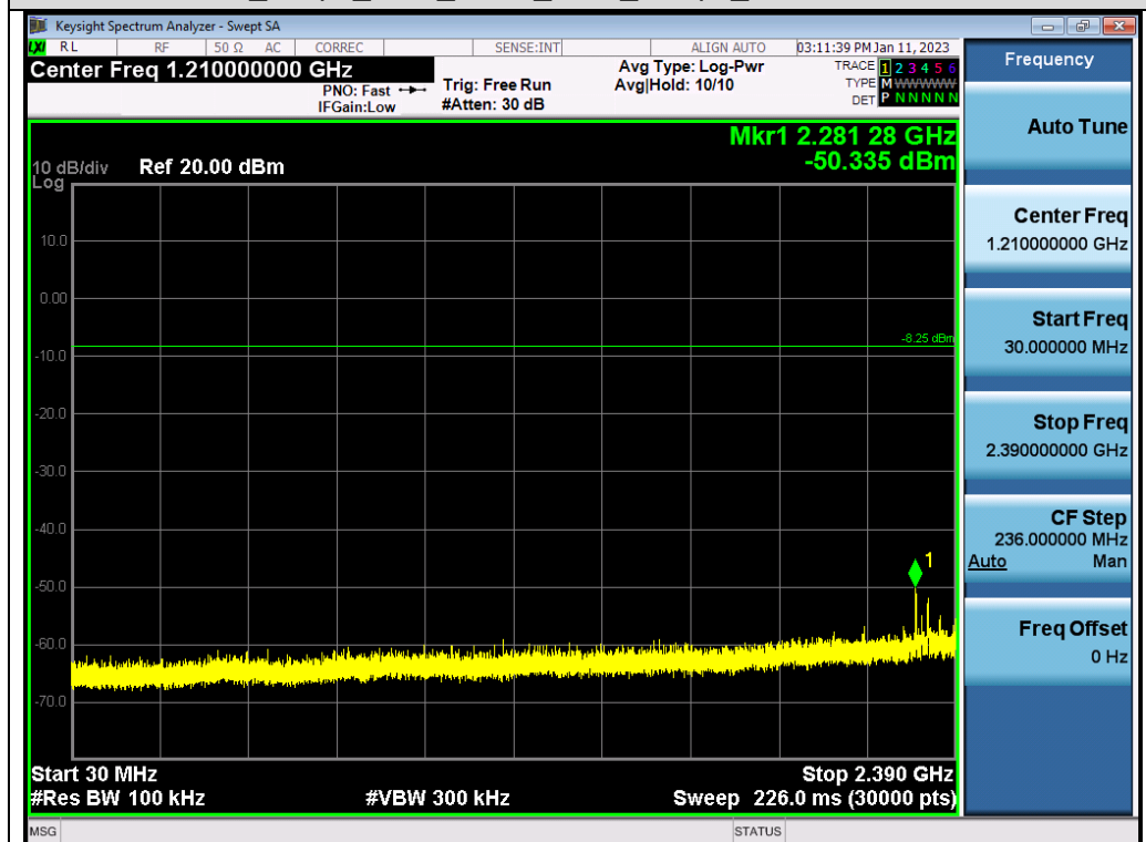
Test_Graph_2.4G_ANT1_2410_4Mbps_Lower Band Emissions
