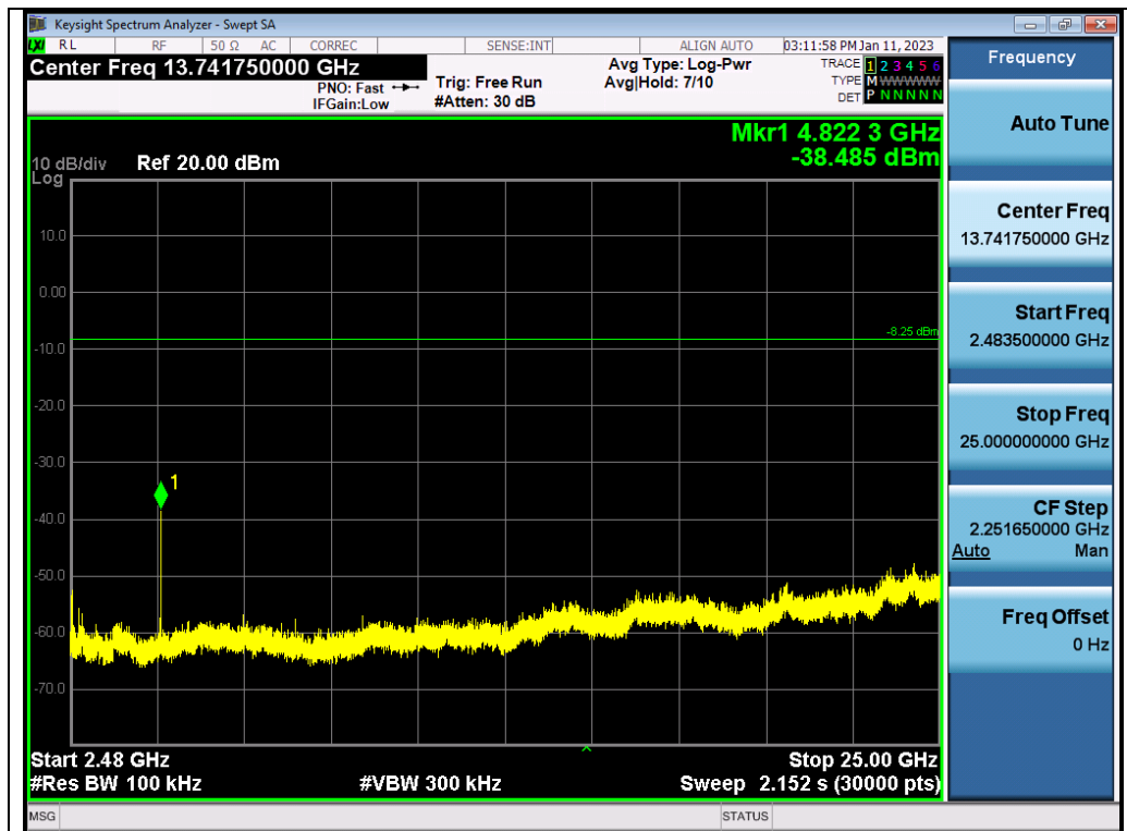
Test_Graph_2.4G_ANT1_2410_4Mbps_Higher Band Emissions
