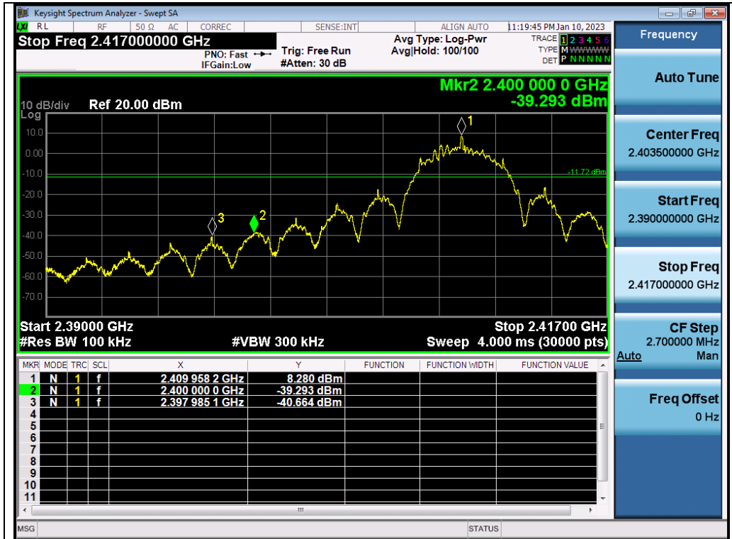
Test_Graph_2.4G_ANT1_2410_4Mbps_Lower Band Edge Emissions
