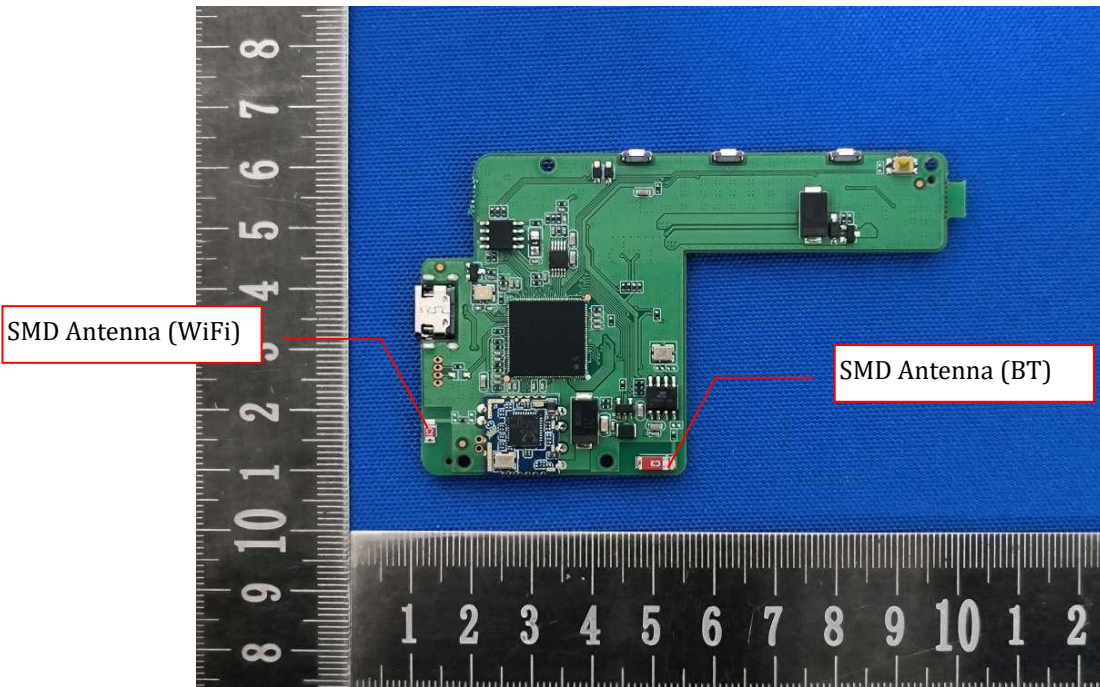
EUT Internal View 2
