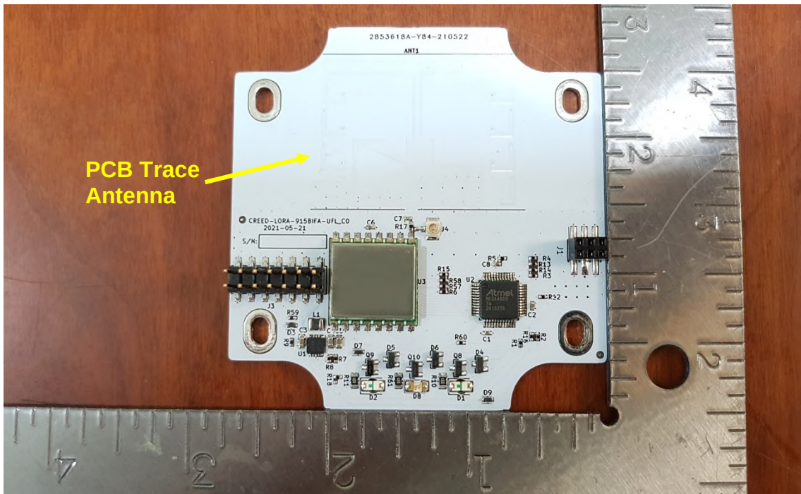
Figure 2 – EUT Internal Photo Back Transmitter PCB
