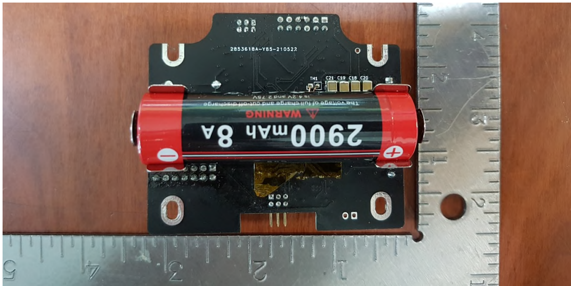
Figure 4 – EUT Internal Photo Back Digital Control PCB
