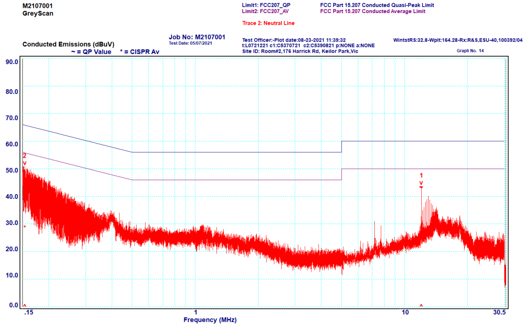
Graph 6-2: Neutral Line (0.15 MHz to 30 MHz)
