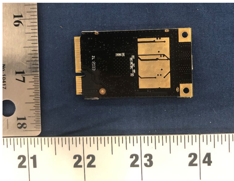
Back of 2A2SC-RDM21 Module
