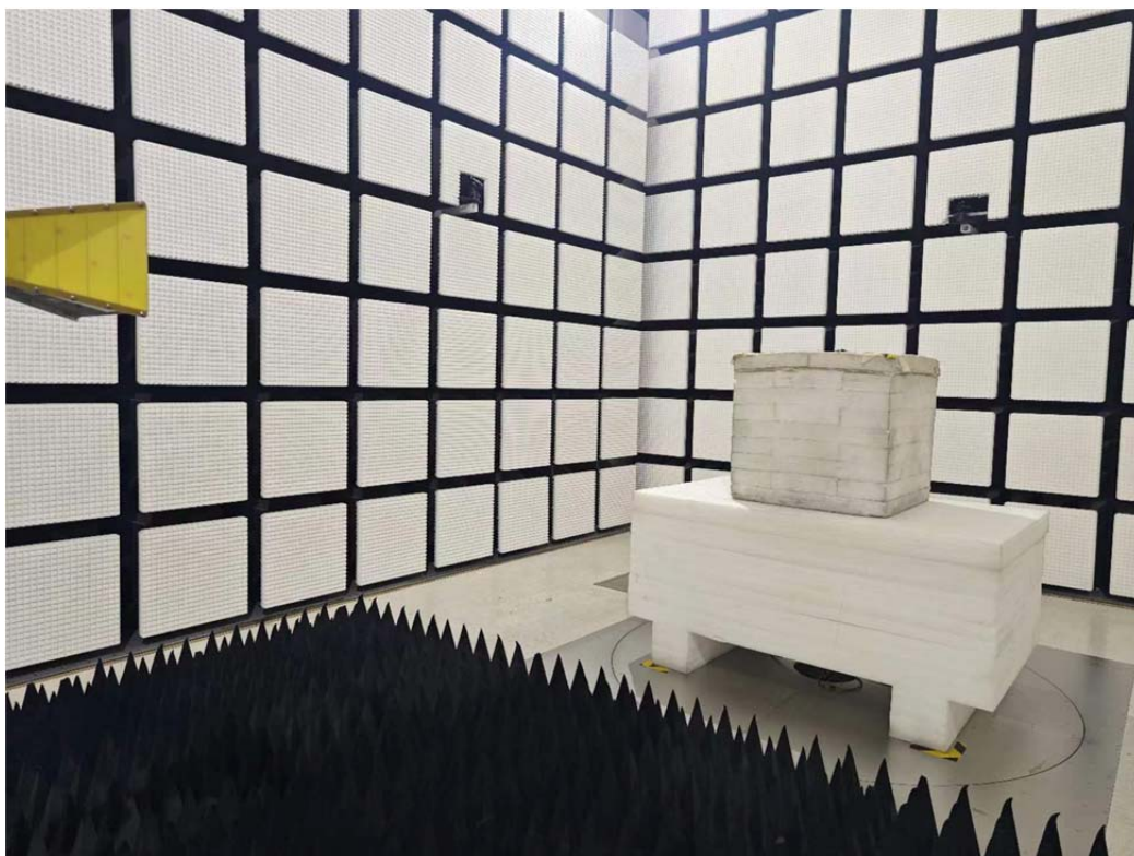
Radiated Emission 1-18GHz View
