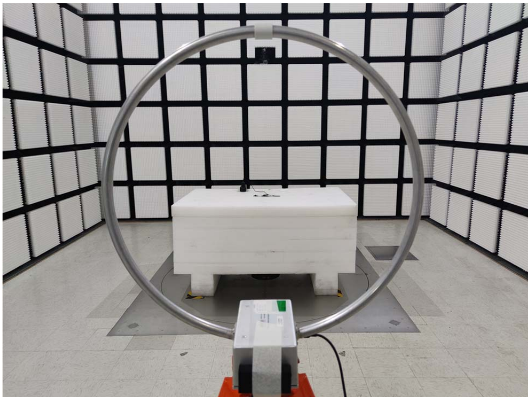
Radiated Emission 9 kHz-30 MHz Parallel View
