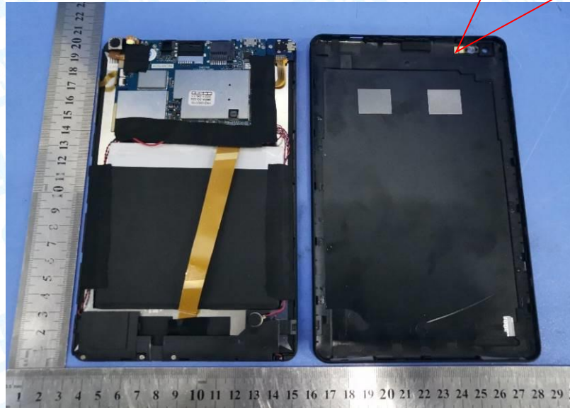
Photo 8 Internal of EUT
