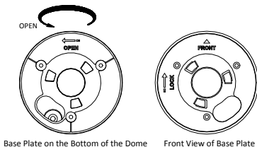
Figure 2-20 Base Plate for PTZIP4XX Series (IR) PTZ Camera
