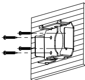
Figure 2-14 Install the Bracket Base
