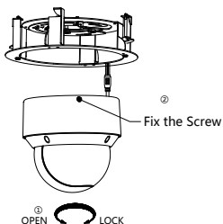
Figure 2-31 Fix the Camera
