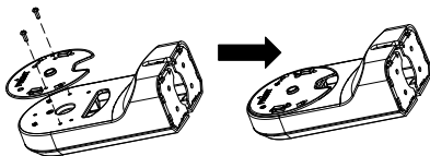
Figure 2-12 Install the Installation Plate
