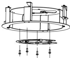
Figure 2-30 Fix the Base Plate to In-ceiling Bracket
