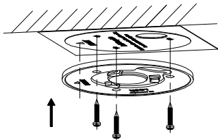
Figure 2-25 For PTZIP4XX Series (IR) PTZ Camera
