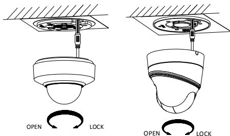
Figure 2-26 Secure the PTZ Camera
