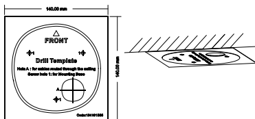
Figure 2-21 Attach the Drill Template
