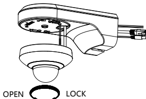
Figure 2-15 Install the Camera
