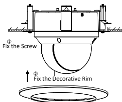
Figure 2-32 Assemble the Decorative Rim
