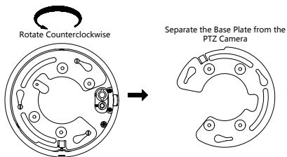
Figure 2-28 Separate the Base Plate from the PTZ camera
