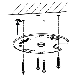
Figure 2-10 Fix the Installation Plate
