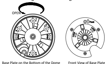
Figure 2-19 Base Plate for PTZIP4XX Series PTZ Camera
