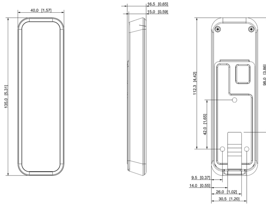
Figure 1-2 Dimensions of the L XK101-KD (mm [inch])
