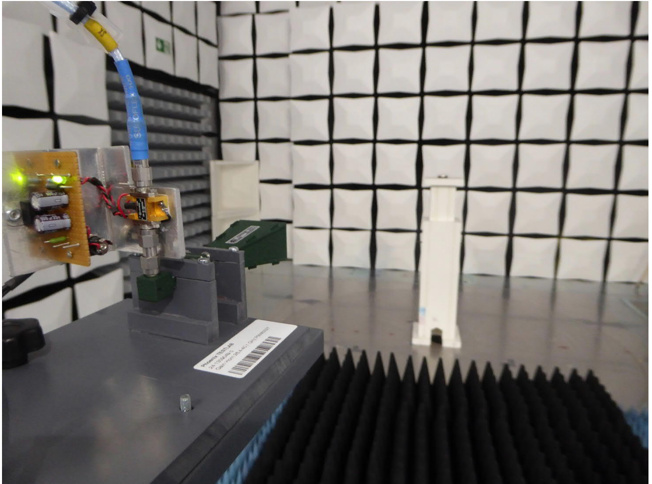
Test setup semi anechoic chamber with ground absorbers 26.5 – 40 GHz
