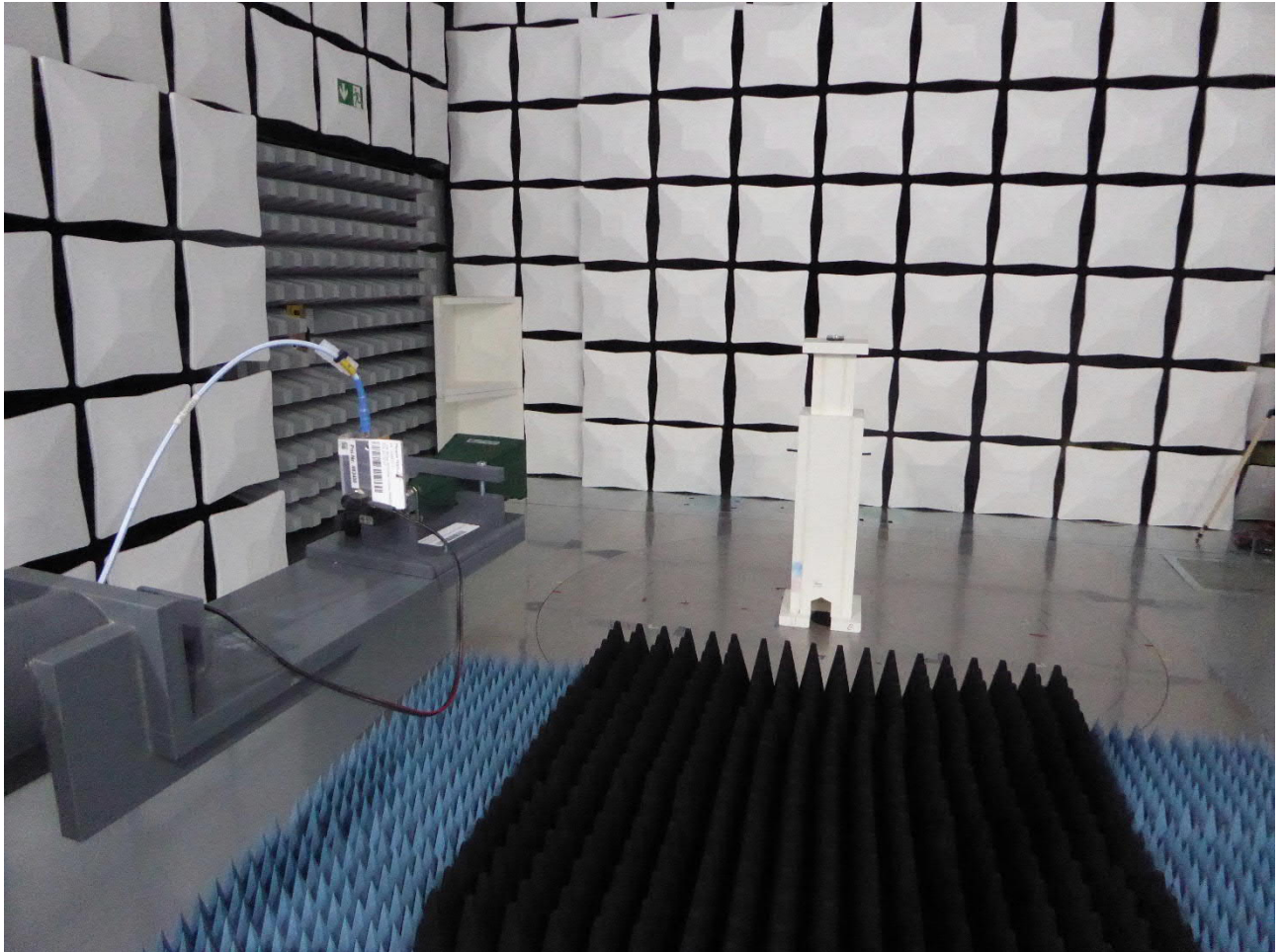
Test setup semi anechoic chamber with ground absorbers 12 – 18 GHz
