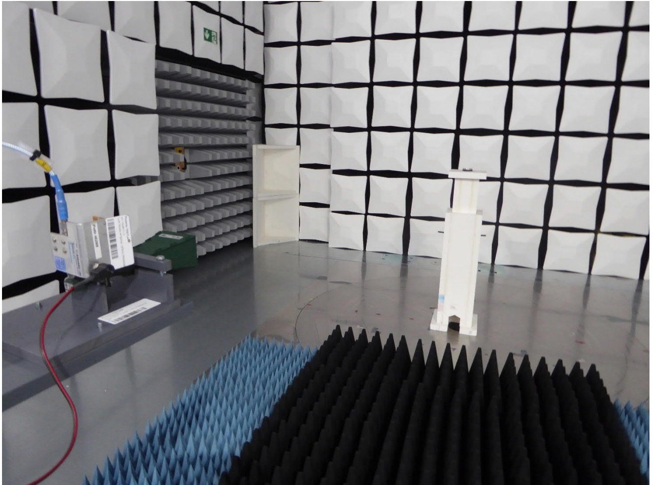
Test setup semi anechoic chamber with ground absorbers 18 – 26.5 GHz
