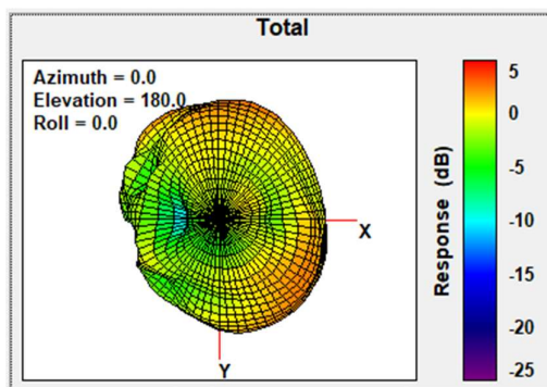
Total Gain Bottom view 2442MHz
