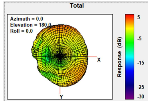
Total Gain Bottom view 2480MHz
