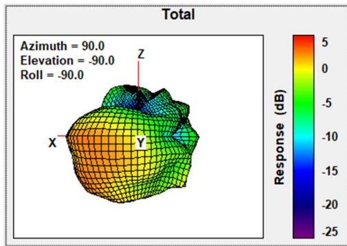
Total Gain Front Face view 2442MHz
