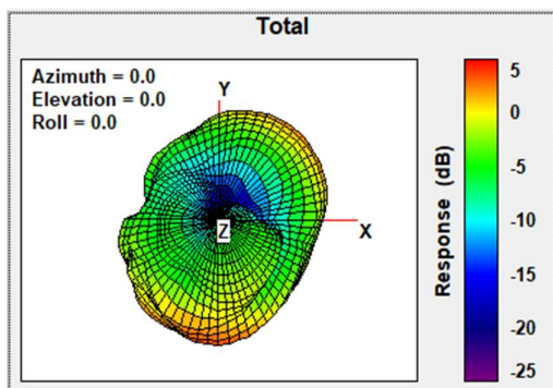
Total Gain Top view 2442MHz
