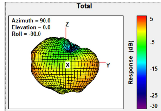
Total Gain Left Side view 2480MHz
