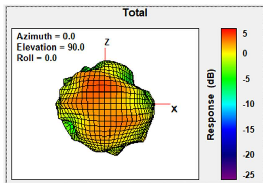
Total Gain Back Face view 2442MHz
