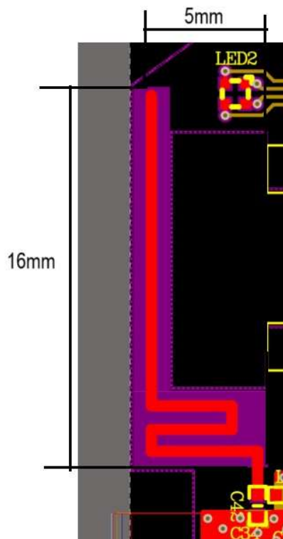
MWP552/553 Copper trace antenna dimension
