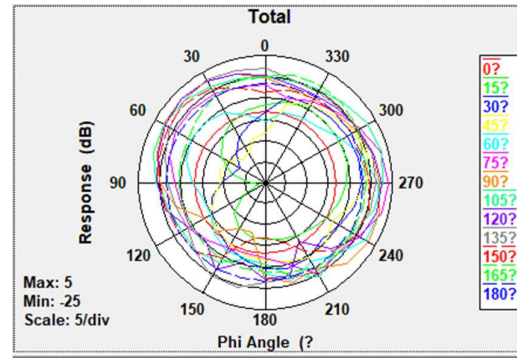
Total Gain Right Side view 2442MHz
