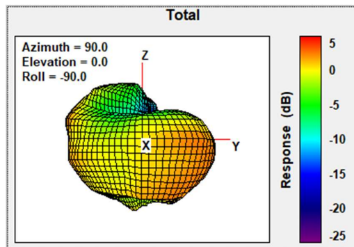
Total Gain Left Side view 2403MHz
