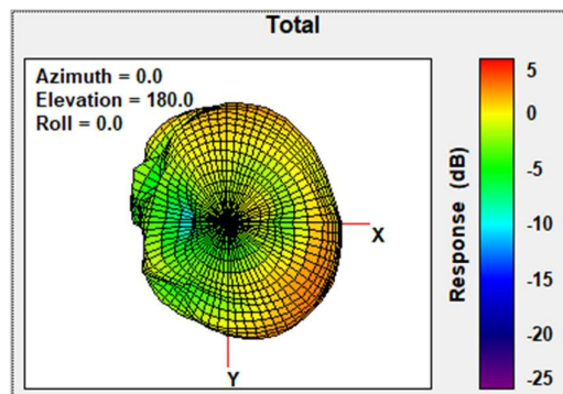
Total Gain Bottom view 2403MHz
