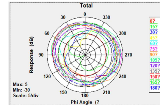
Total Gain Right Side view 2480MHz
