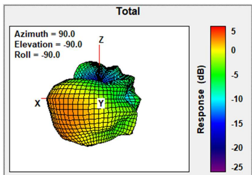
Total Gain Front Face view 2403MHz
