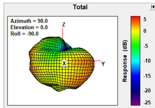
Total Gain Left Side view 2442MHz
