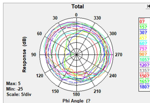
Total Gain Right Side view 2403MHz
