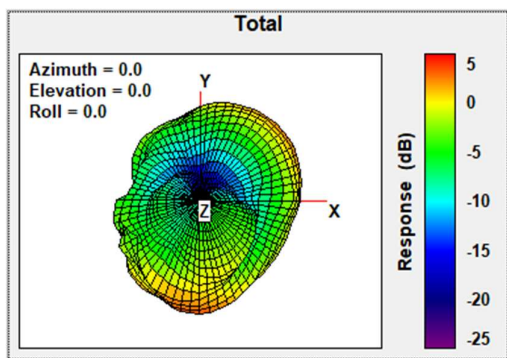
Total Gain Top view 2403MHz
