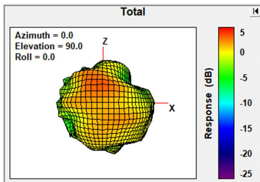
Total Gain Back Face view 2403MHz
