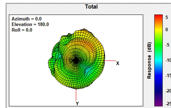
Total Gain Bottom view 2442MHz
