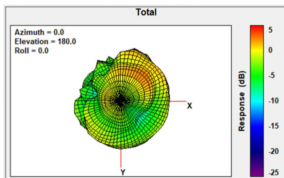
Total Gain Bottom view 2403MHz
