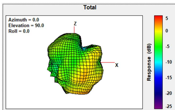
Total Gain Back Face view 2442MHz
