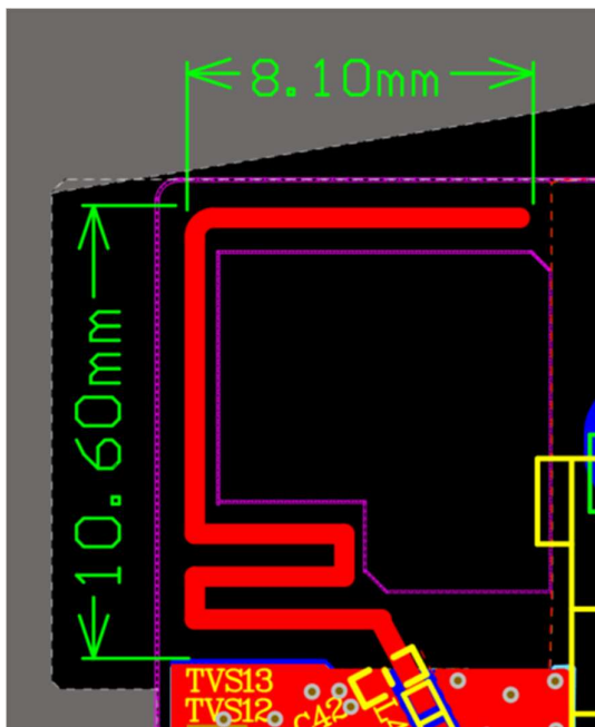
MWP554 Copper Trace Antenna Dimension
