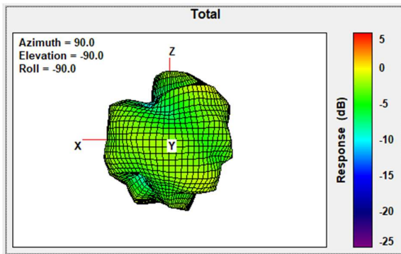
Total Gain Front Face view 2442MHz
