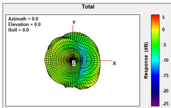
Total Gain Top view 2442MHz
