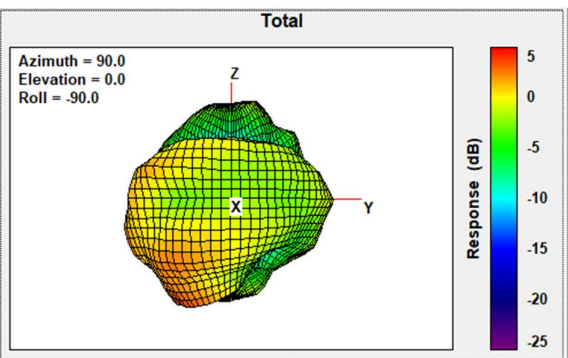
Total Gain Left Side view 2480MHz
