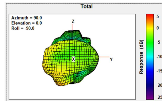
Total Gain Left Side view 2442MHz
