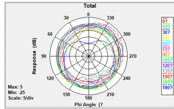
Total Gain Right Side view 2403MHz
