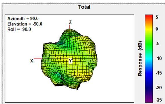
Total Gain Front Face view 2480MHz
