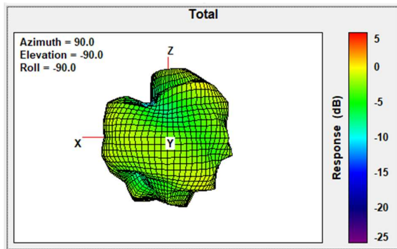
Total Gain Front Face view 2403MHz
