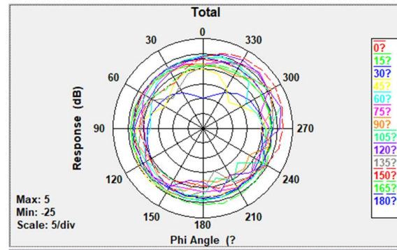
Total Gain Right Side view 2442MHz
