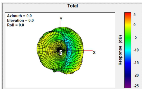
Total Gain Top view 2403MHz
