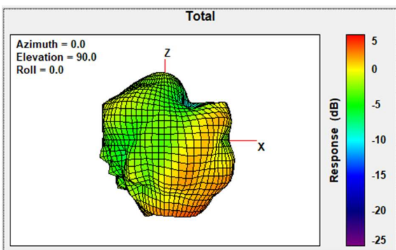
Total Gain Back Face view 2480MHz
