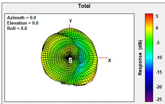
Total Gain Top view 2480MHz
