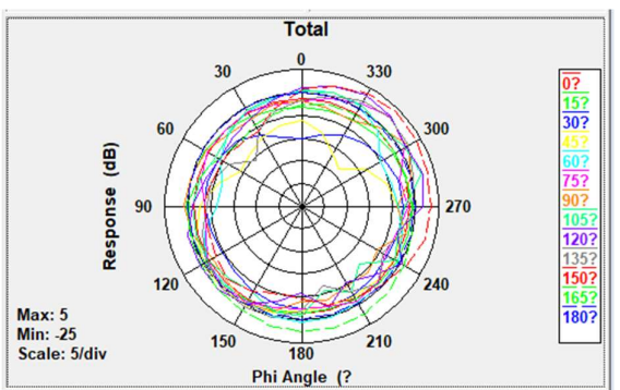
Total Gain Right Side view 2480MHz
