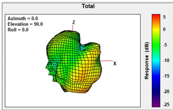
Total Gain Back Face view 2403MHz
