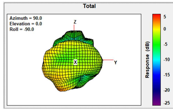
Total Gain Left Side view 2403MHz
