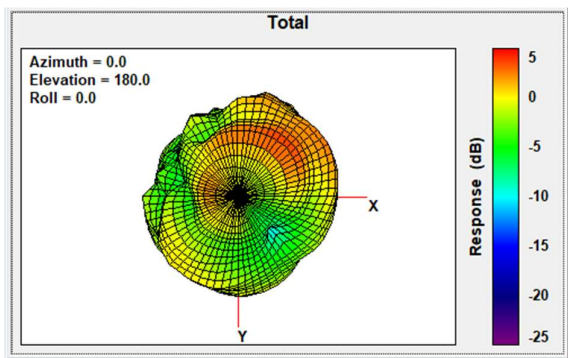
Total Gain Bottom view 2480MHz
