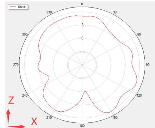
Phi=0 Freq=2454MHz
