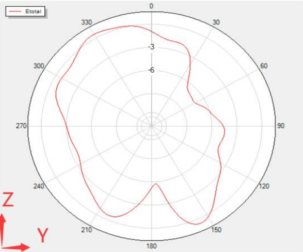
Phi=90 Freq=2460MHz
