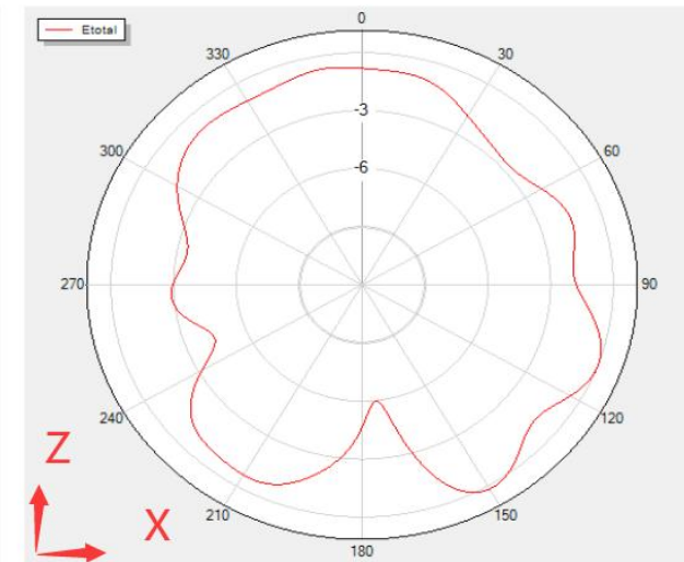
Phi=0 Freq=2446MHz
