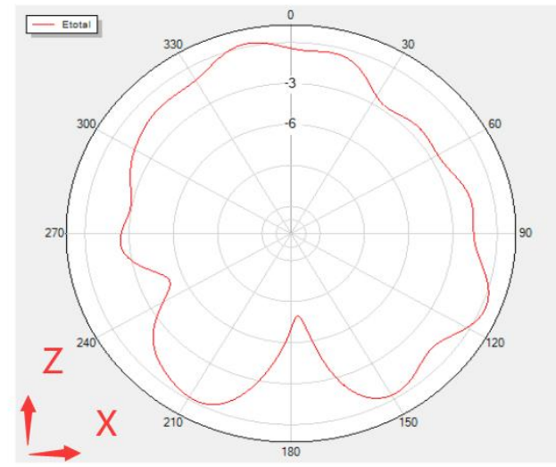
Phi=0 Freq=2480MHz
