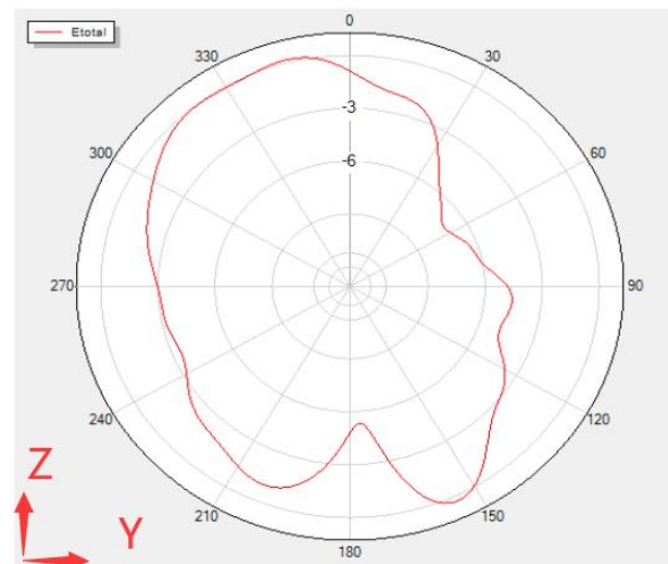
Phi=90 Freq=2434MHz
