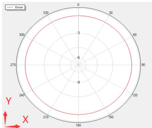
Theta=0 Freq=2434MHz
