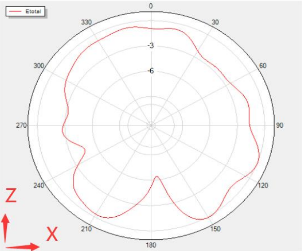
Phi=0 Freq=2460MHz
