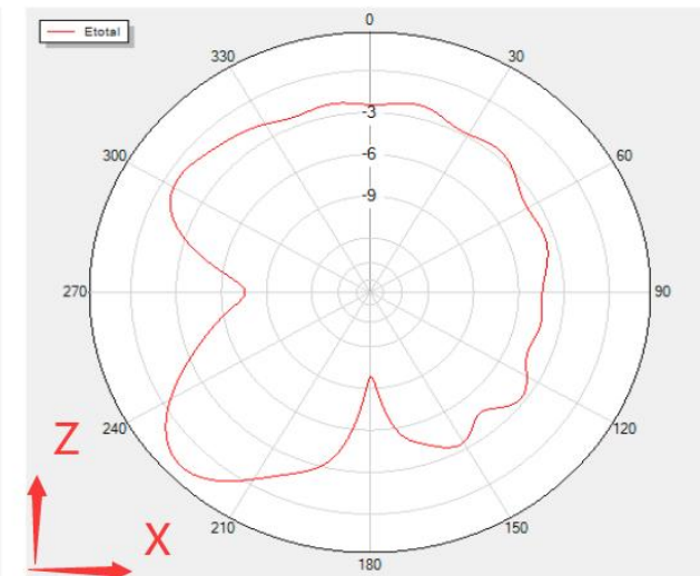
Phi=0 Freq=2402MHz
