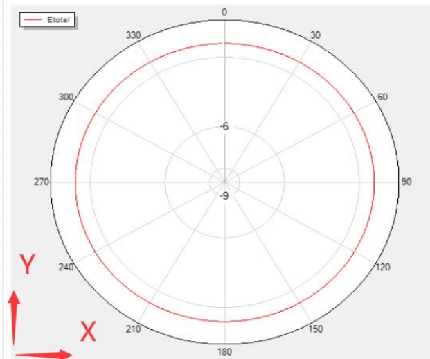
Theta=0 Freq=2402MHz
