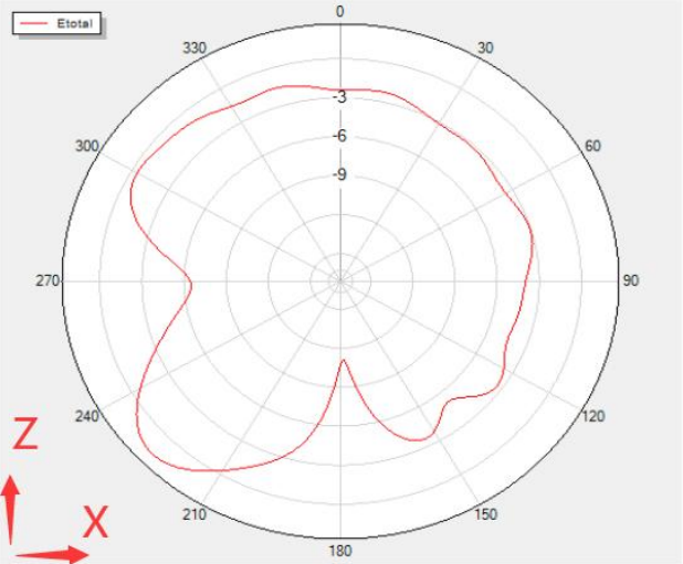
Phi=0 Freq=2446MHz
