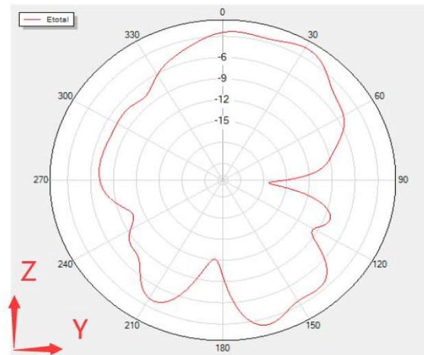
Phi=90 Freq=2402MHz
