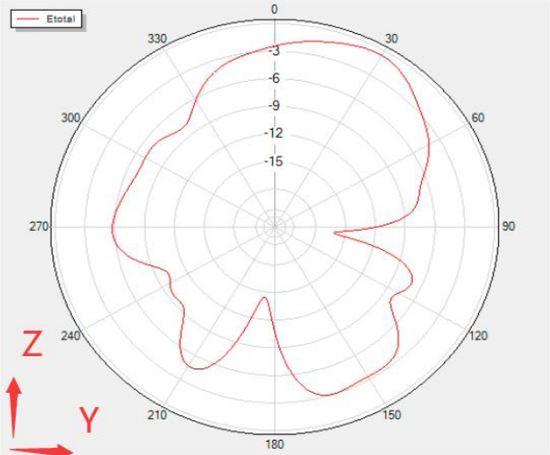
Phi=90 Freq=2446MHz
