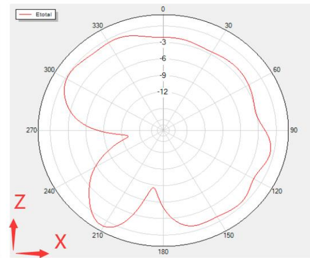
Phi=0 Freq=2428MHz
