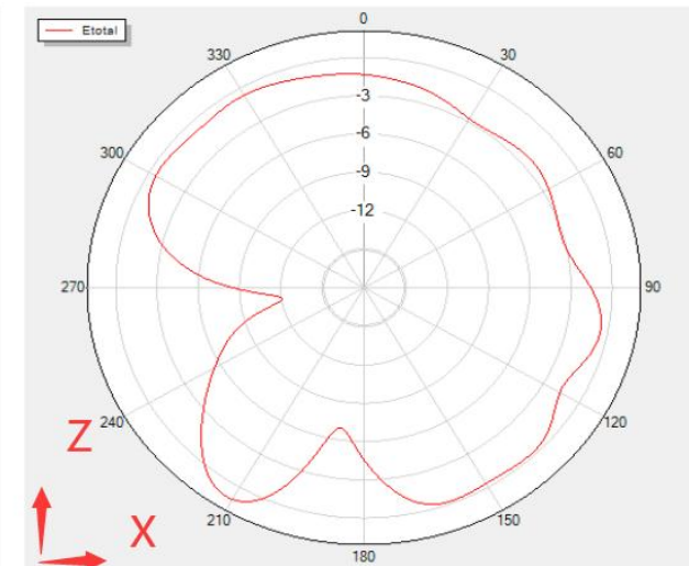
Phi=0 Freq=2402MHz
