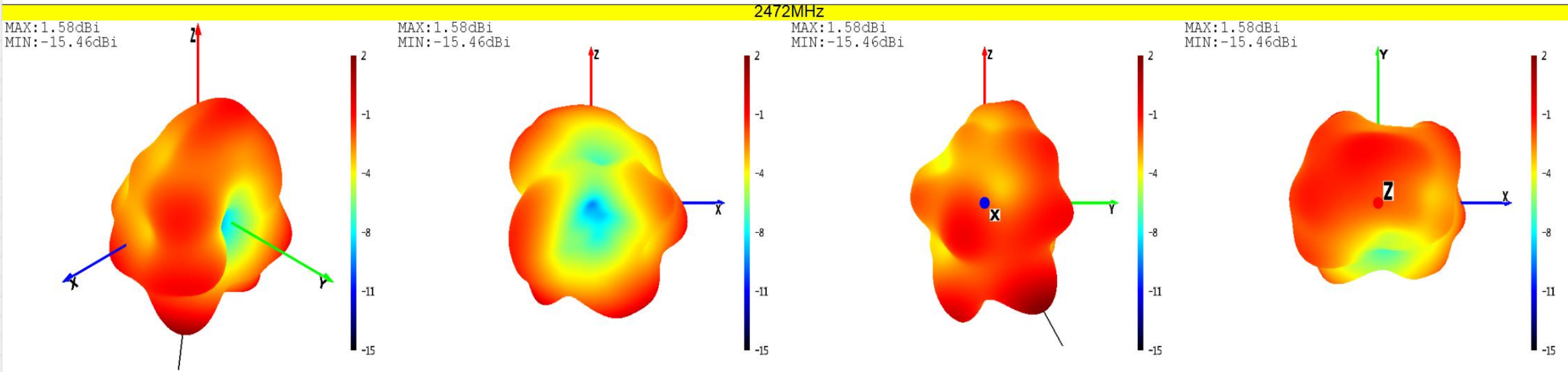
Theta=0 Freq=2472MHz
