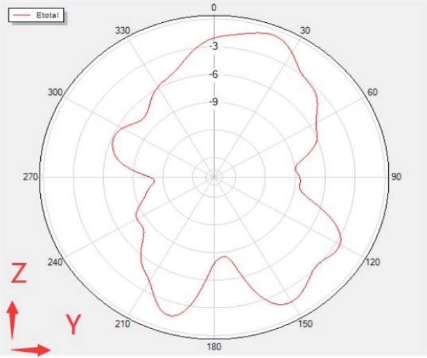
Phi=90 Freq=2472MHz
