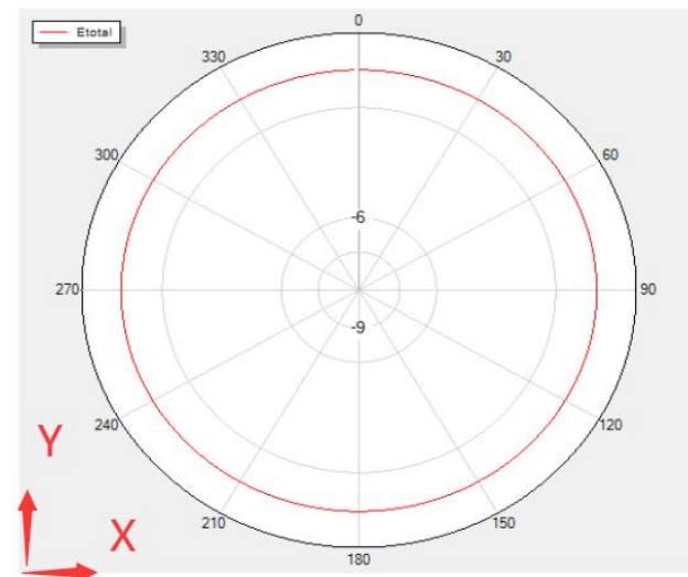
Theta=0 Freq=2434MHz
