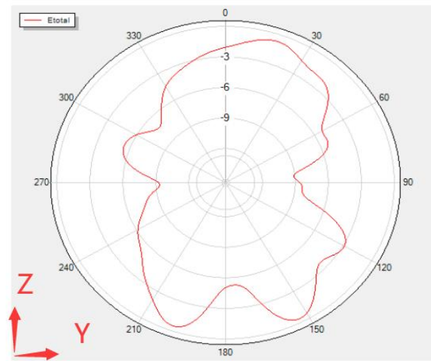
Phi=90 Freq=2428MHz
