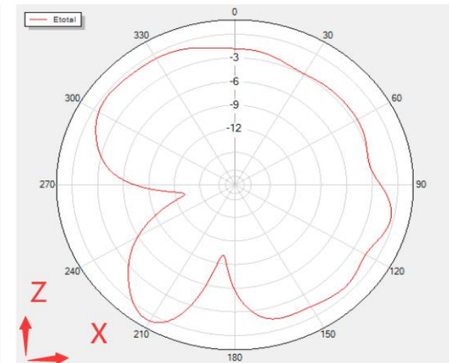
Phi=0 Freq=2446MHz
