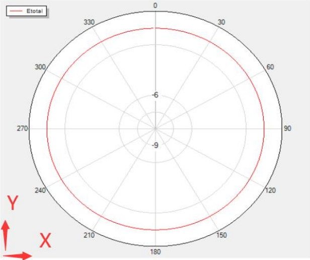
Theta=0 Freq=2472MHz
