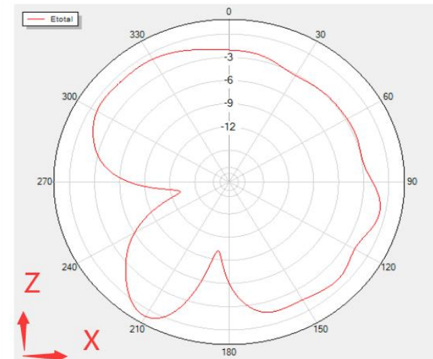
Phi=0 Freq=2454MHz
