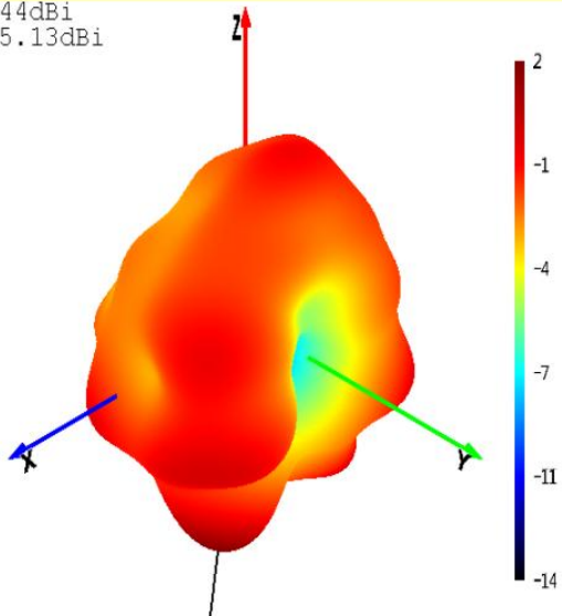
Theta=0 Freq=2454MHz
