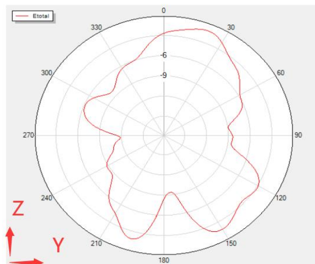
Phi=90 Freq=2480MHz
