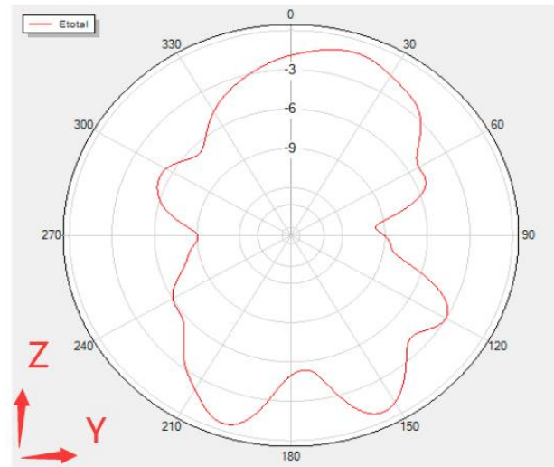
Phi=90 Freq=2416MHz
