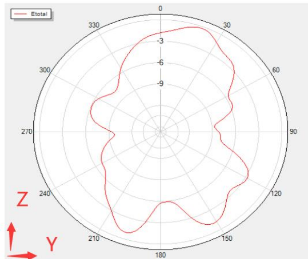
Phi=90 Freq=2446MHz
