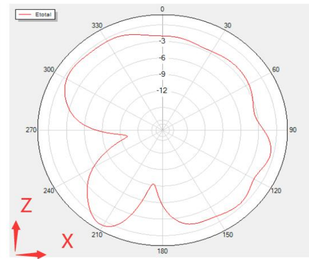
Phi=0 Freq=2434MHz
