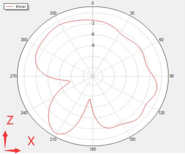
Phi=0 Freq=2472MHz
