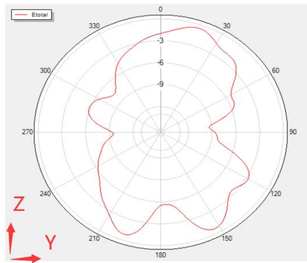
Phi=90 Freq=2434MHz
