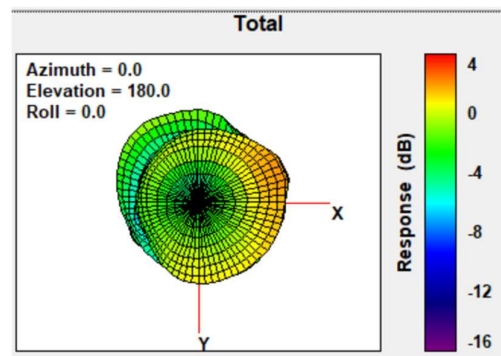
Total Gain Bottom view 2402MHz
