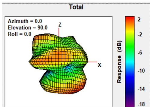
Total Gain Back Face view 2440MHz
