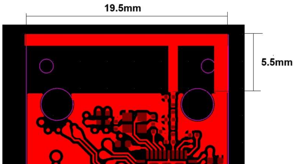
RX100 Dongle Copper trace antenna dimension
