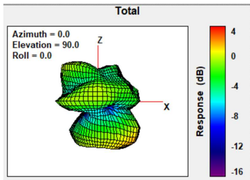
Total Gain Back Face view 2402MHz
