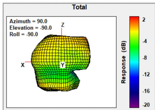
Total Gain Front Face view 2480MHz
