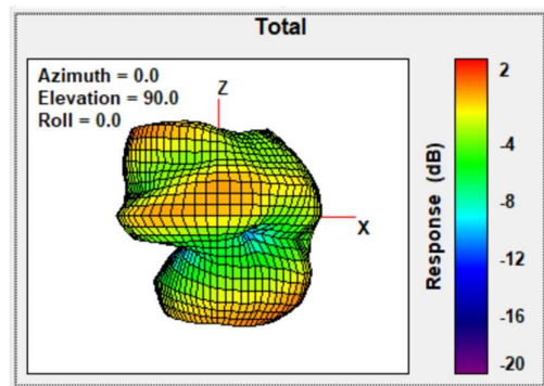
Total Gain Back Face view 2480MHz
