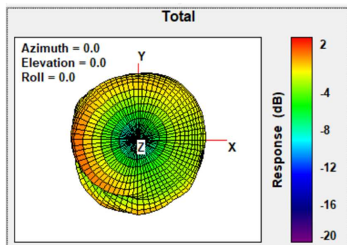
Total Gain Top view 2480MHz
