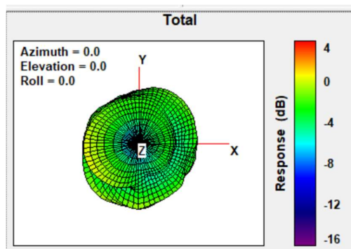
Total Gain Top view 2402MHz
