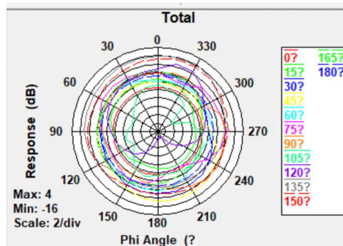
Total Gain Right Side view 2402MHz
