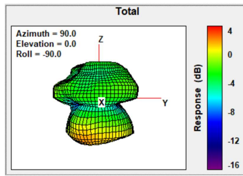
Total Gain Left Side view 2402MHz
