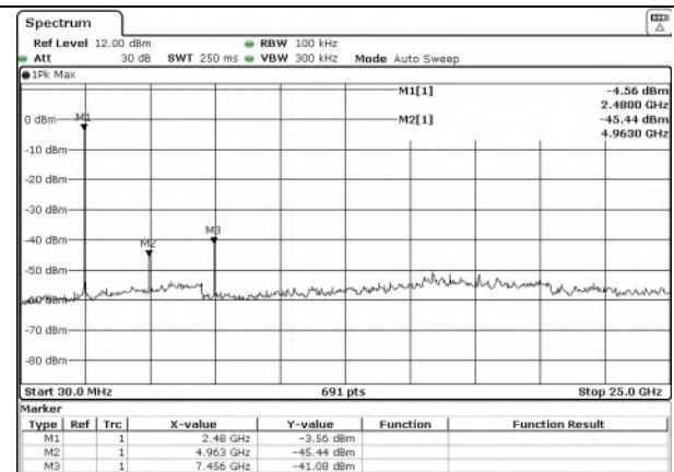
Test Mode: EDR--High
