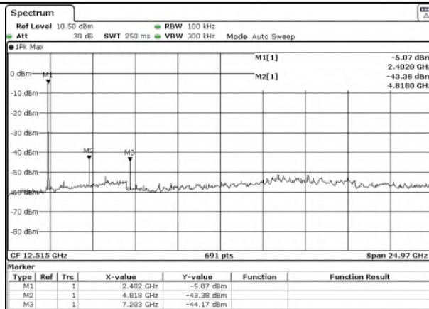
Test Mode: BDR---Low
