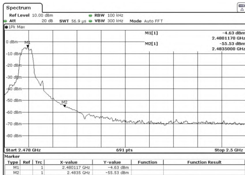
For 8DPSK Hopping Mode (High)
