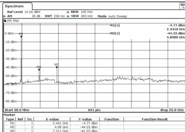
Test Mode: EDR---Mid
