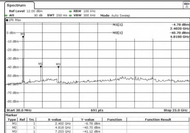
Test Mode: EDR---Low
