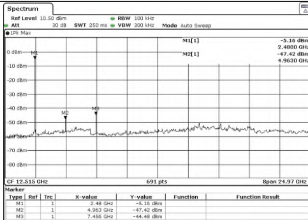
Test Mode: BDR---High
