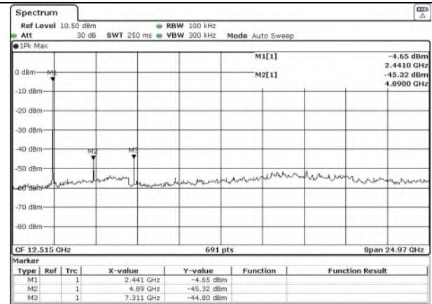
Test Mode: BDR---Mid
