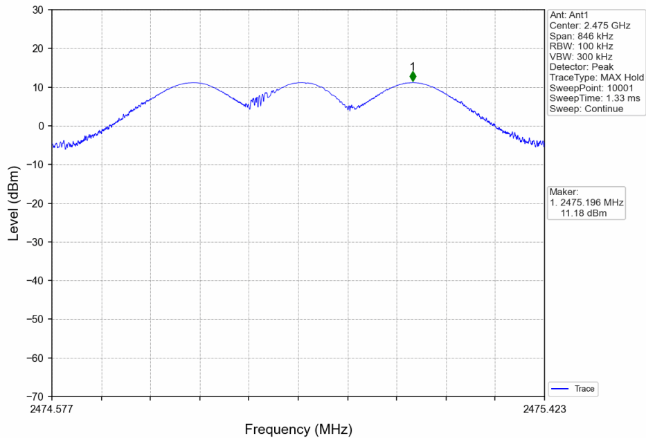
TX_HCH_2475MHz_Ant1_NTNV
