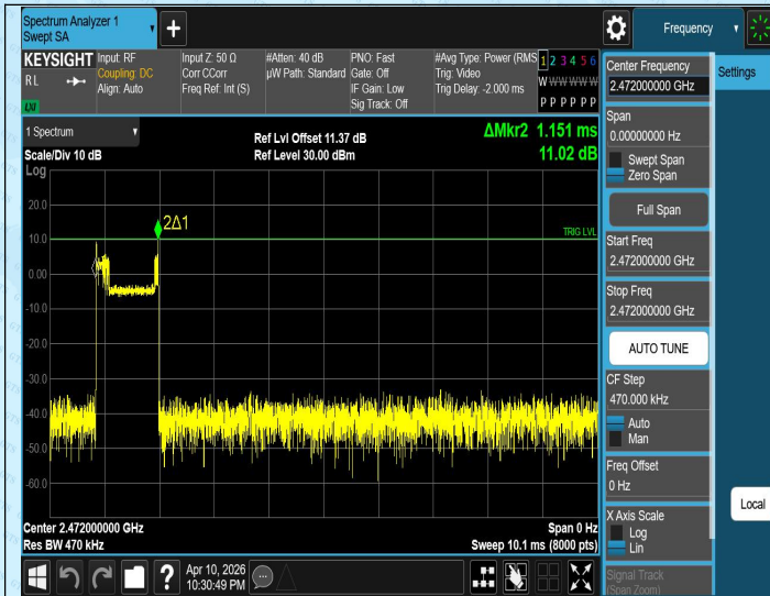
TX-Ant2-Hop_2472-PASS
