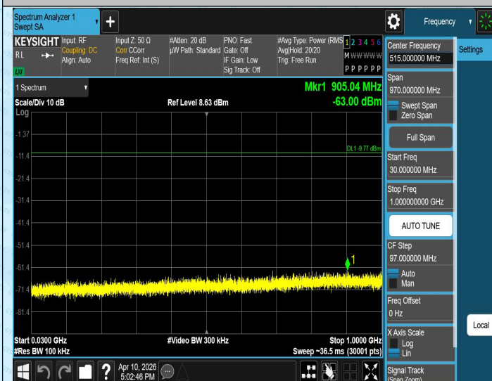
TX-Ant2-2472-30~1000-PASS
