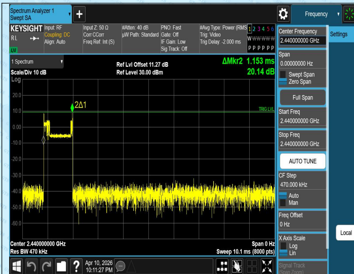
TX-Ant1-Hop_2440-PASS
