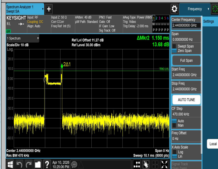
TX-Ant2-Hop_2440-PASS
