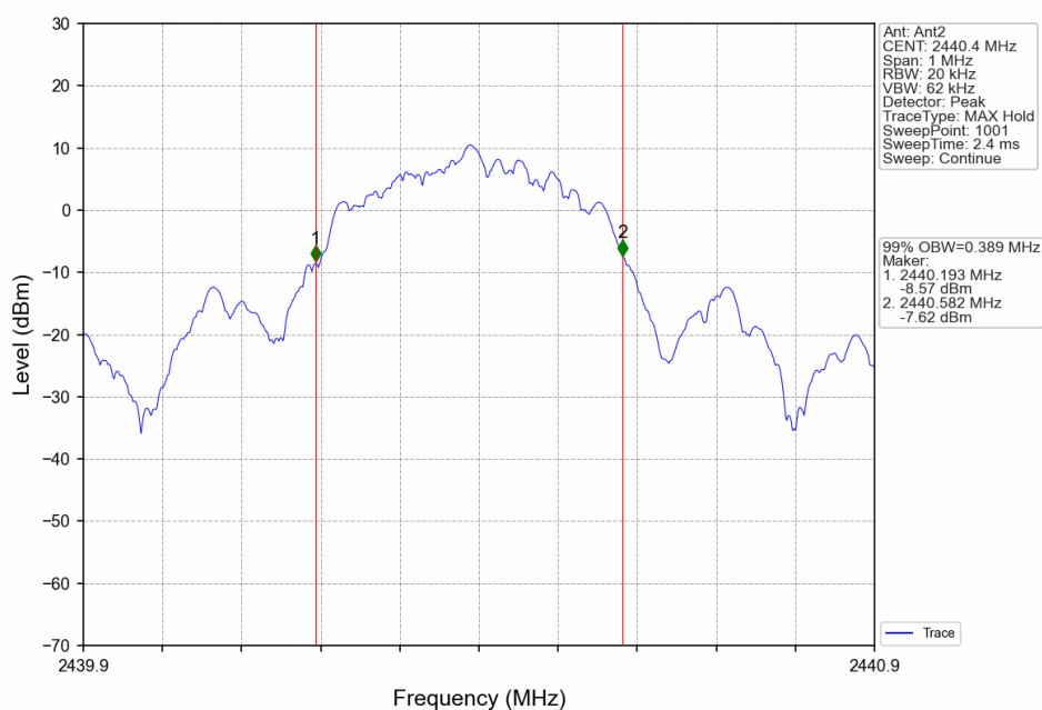
GMSK_MCH_2440.4MHz_Ant2_NTNV
