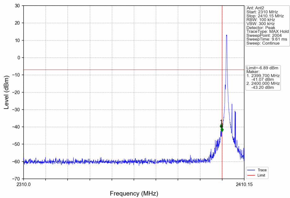
GMSK_LCH_2402.15MHz_Ant2_NTNV
