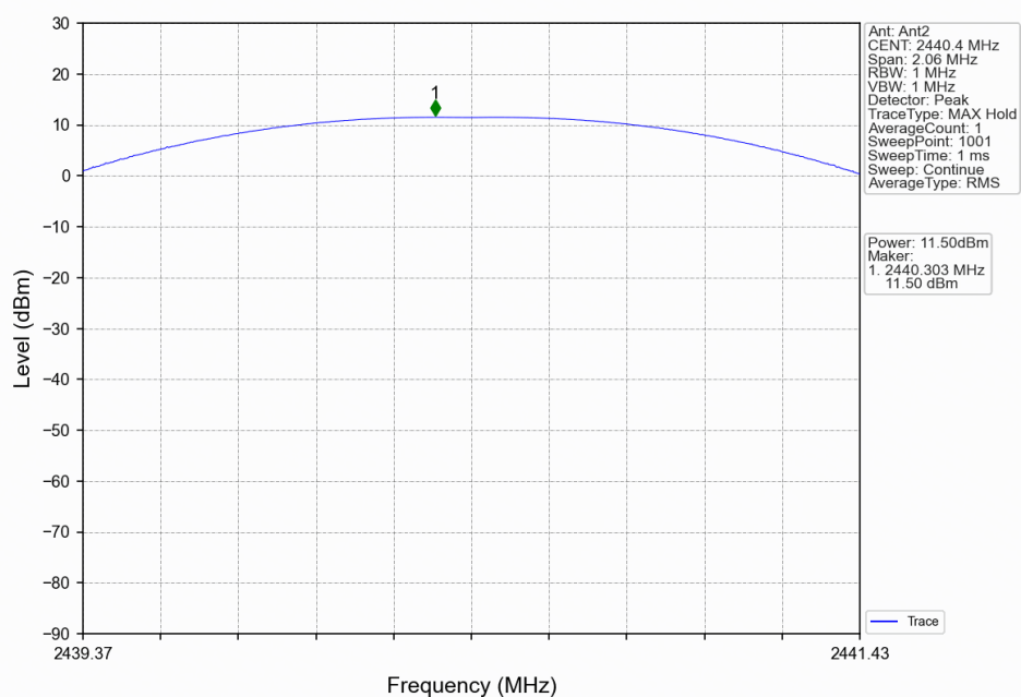
GMSK_MCH_2440.4MHz_Ant2_NTNV
