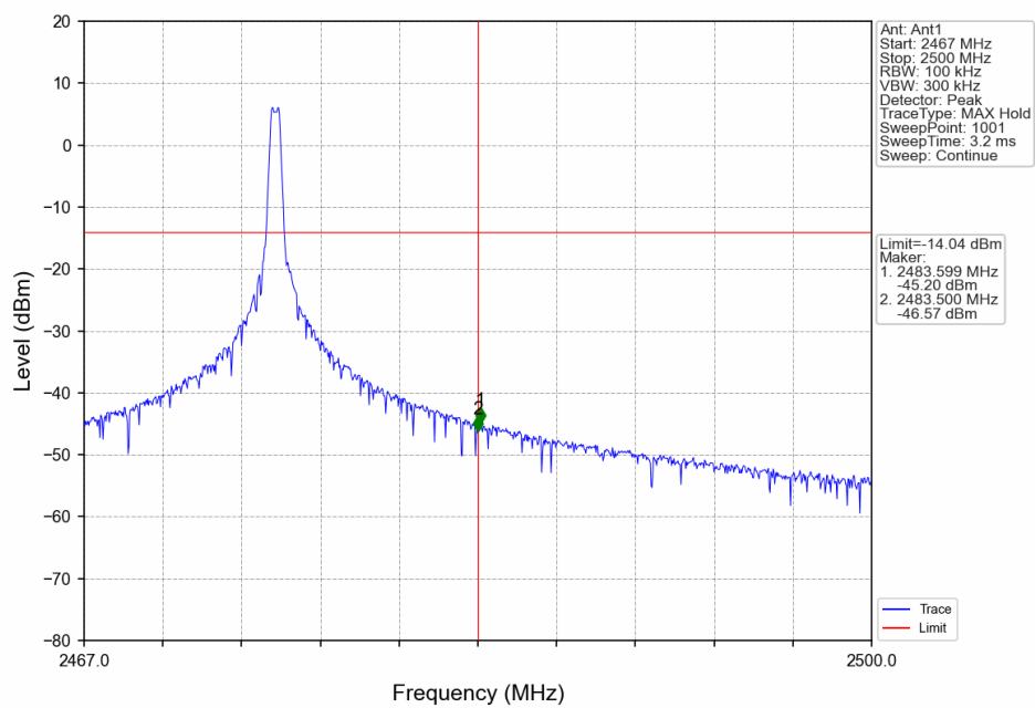
GFSK_HCH_2475MHz_Ant1_NTNV
