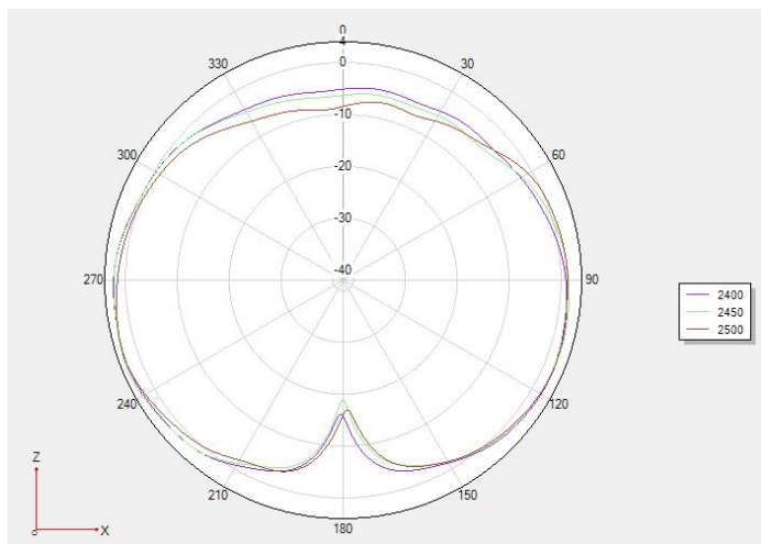
Phi0°2D
