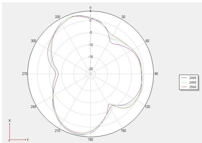
Theta90°2D
