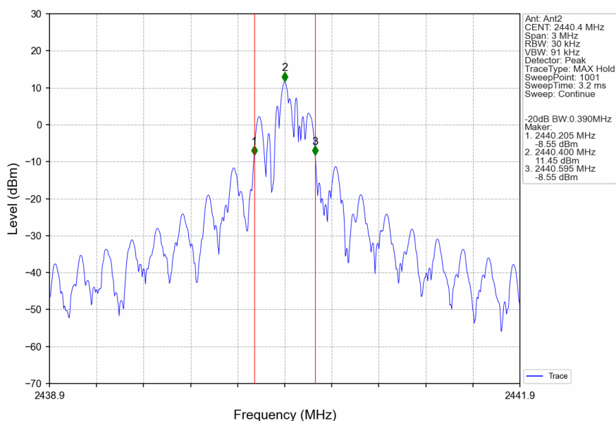
2.4G_MCH_2440.4MHz_Ant2_NTNV
