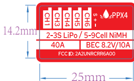
B-TRCRR6AESC-02 RCR-R6A-ESC侧面贴 50#拉丝龙+3M9448A胶 25*14.2mm
