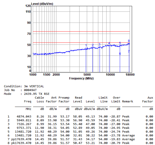
2.4G SRD_TX_CH_M_Vertical
