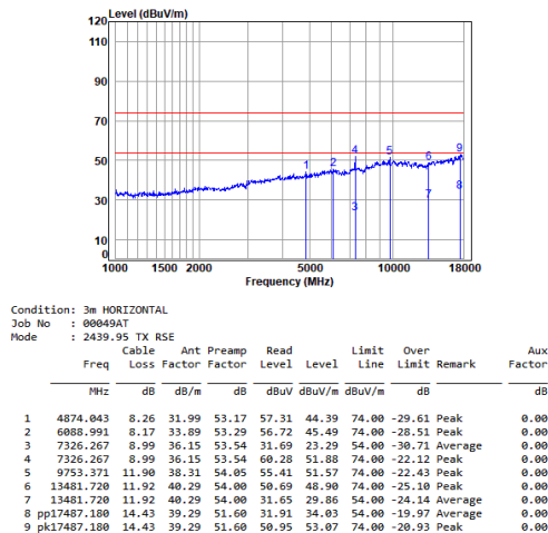
2.4G SRD_TX_CH_M_Horizontal
