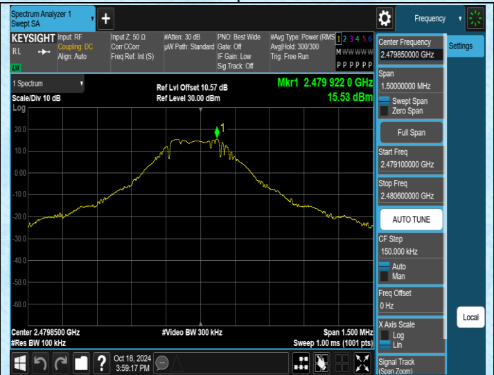
TX-Ant2-2479.85-0~Reference-PASS
