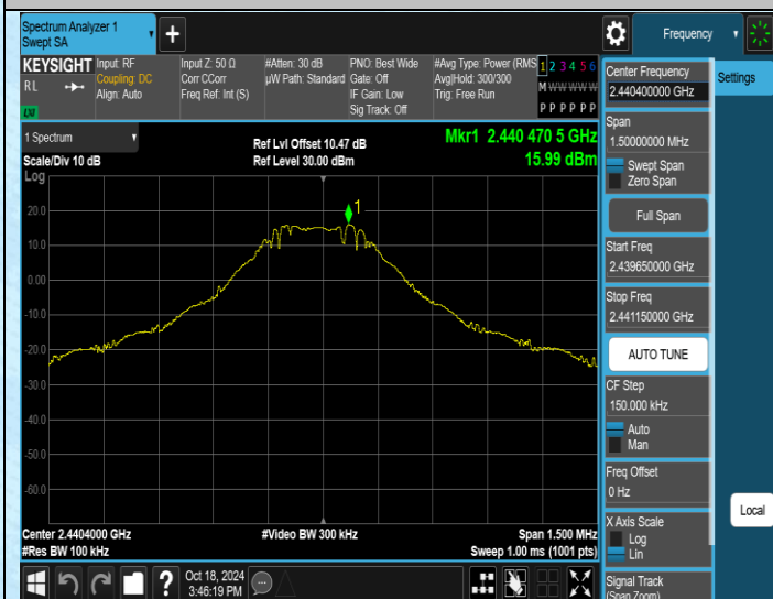
TX-Ant1-2440.4-0~Reference-PASS
