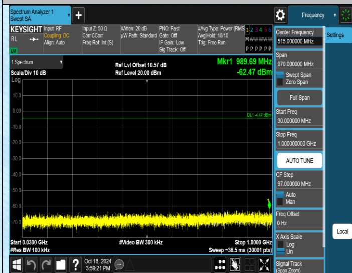
TX-Ant2-2479.85-30~1000-PASS
