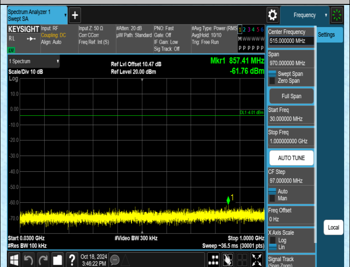
TX-Ant1-2440.4-30~1000-PASS
