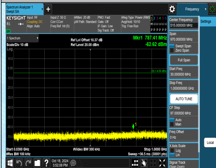
TX-Ant2-2402.15-30~1000-PASS
