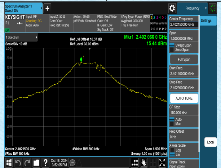
TX-Ant2-2402.15-0~Reference-PASS
