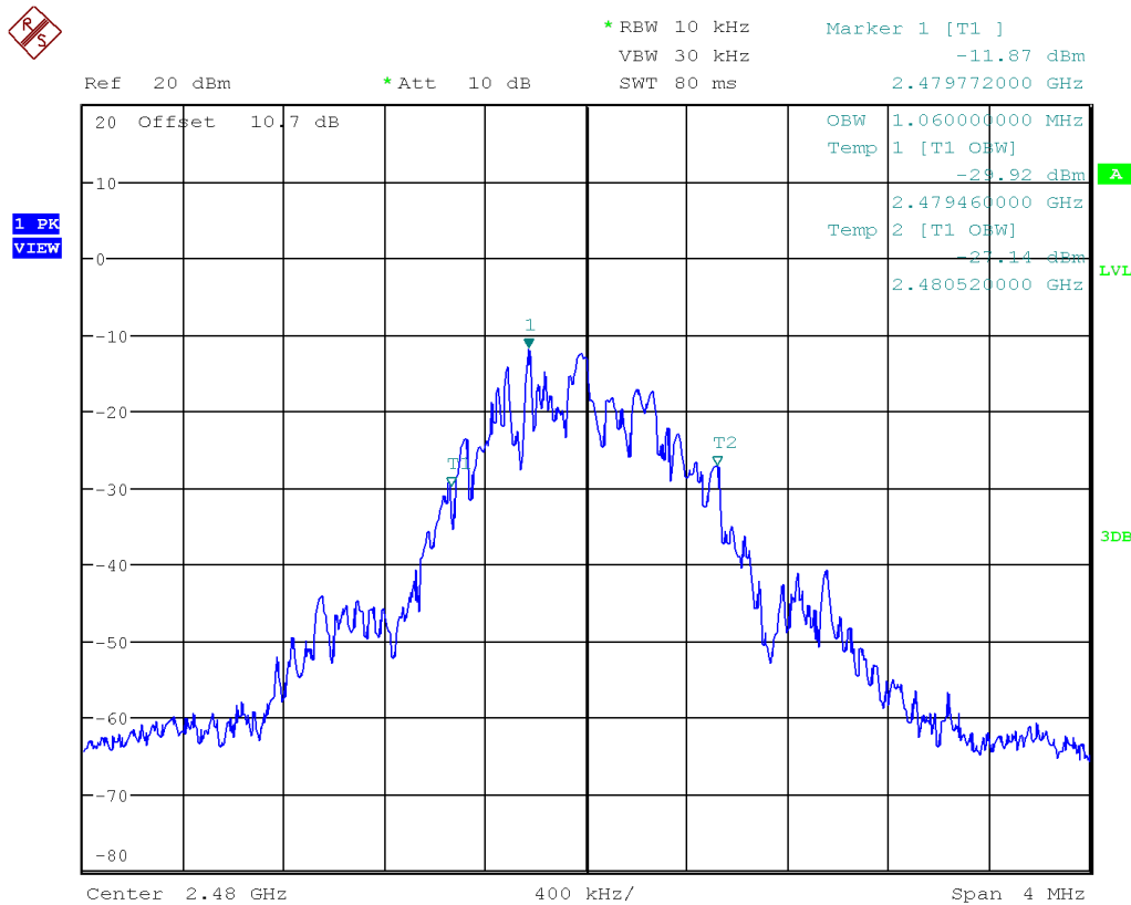
Plot 10. 2480 MHz, 99% Bandwidth
