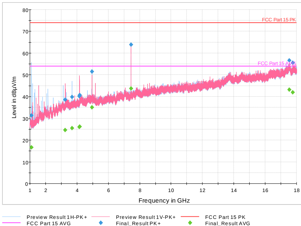
Plot 25. 1-18 GHz, 2480 MHz
