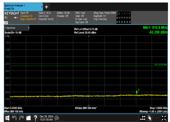
Band4-1.4MHz-QPSK-20175-6RB#0-30~1000-PASS
