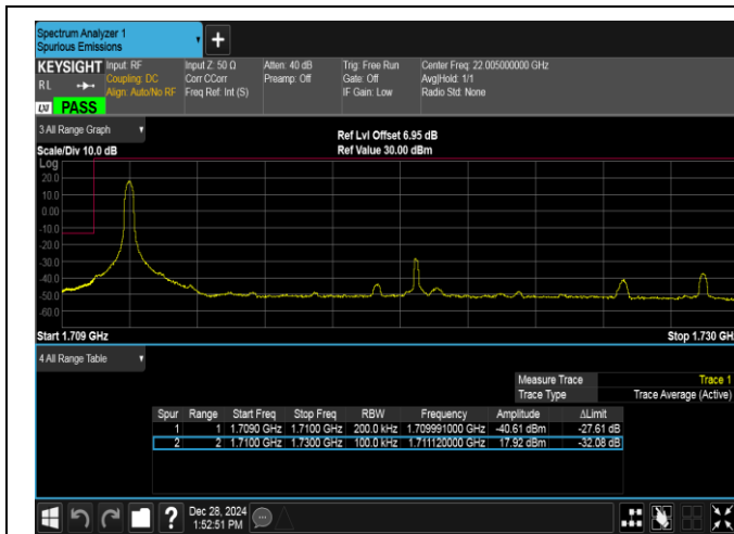
Band4-20MHz-16QAM-20050-1RB#0-PASS
