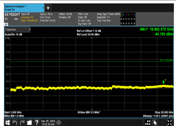
Band4-1.4MHz-QPSK-20175-6RB#0-3000~20000-PASS
