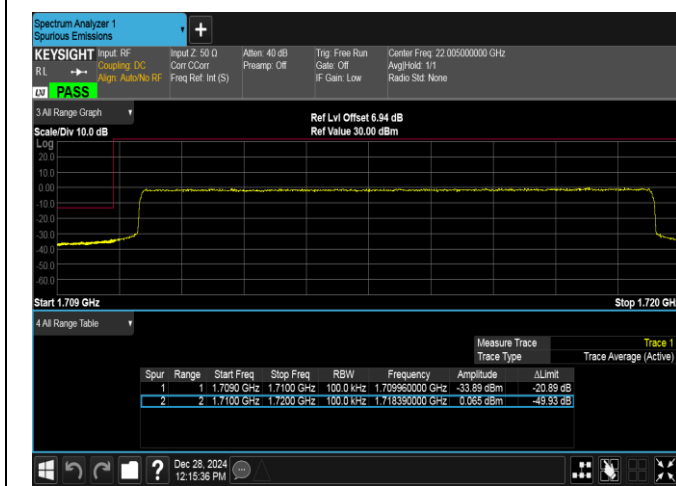
Band4-10MHz-16QAM-20000-50RB#0-PASS
