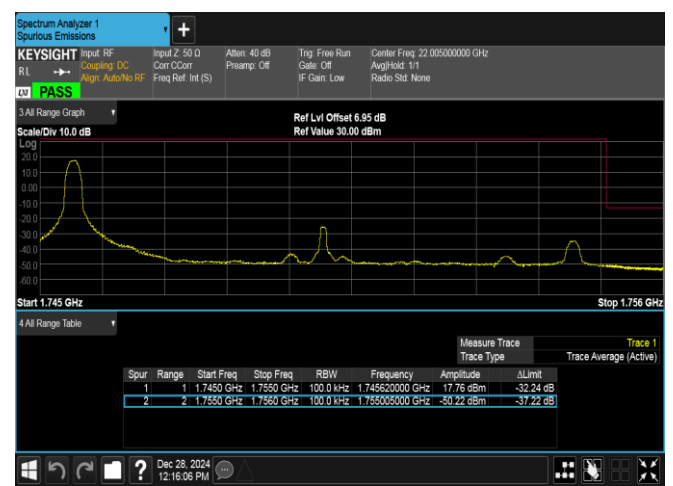
Band4-10MHz-16QAM-20350-1RB#0-PASS
