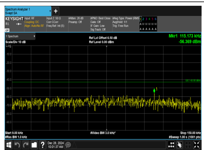
Band4-1.4MHz-QPSK-20175-6RB#0-0.009~0.15-PASS
