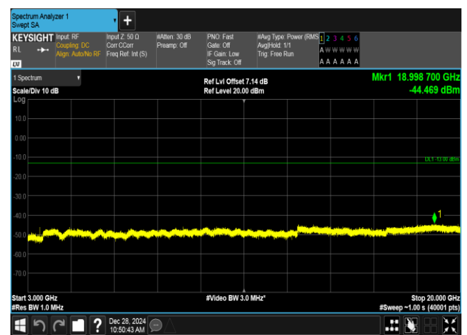
Band4-3MHz-16QAM-20175-1RB#14-3000~20000-PASS
