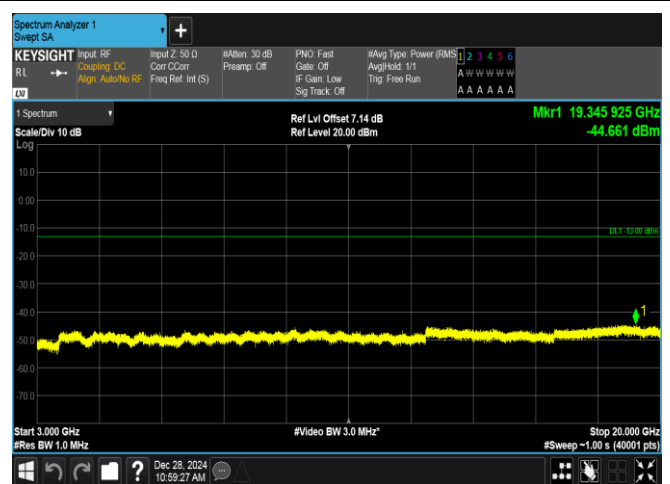
Band4-3MHz-16QAM-20385-15RB#0-3000~20000-PASS
