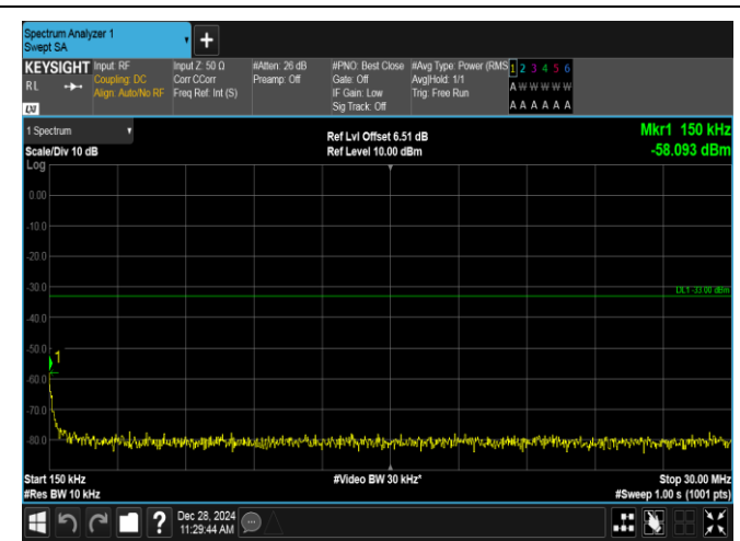
Band4-5MHz-QPSK-19975-1RB#0-0.15~30-PASS
