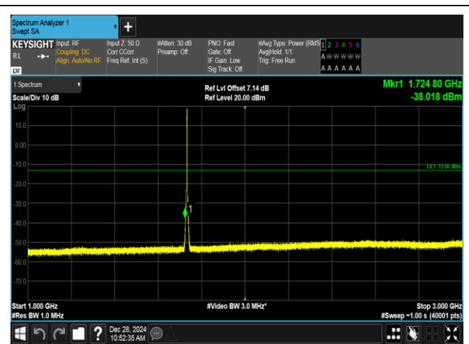
Band4-3MHz-16QAM-20175-15RB#0-1000~3000-PASS
