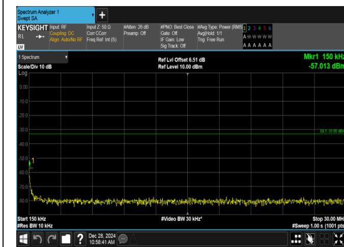
Band4-3MHz-16QAM-20385-15RB#0-0.15~30-PASS
