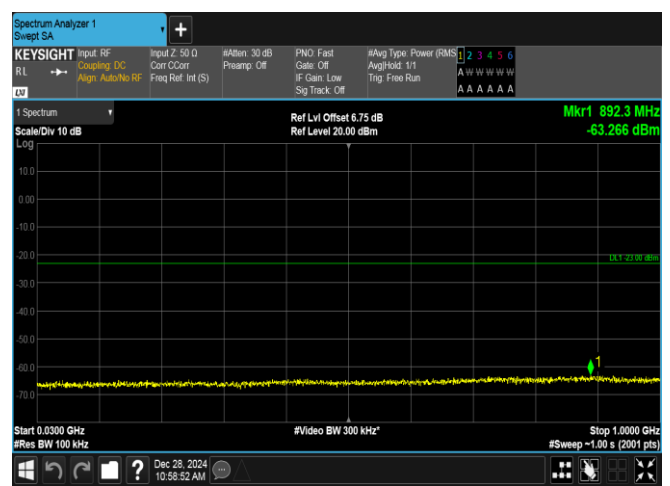
Band4-3MHz-16QAM-20385-15RB#0-30~1000-PASS
