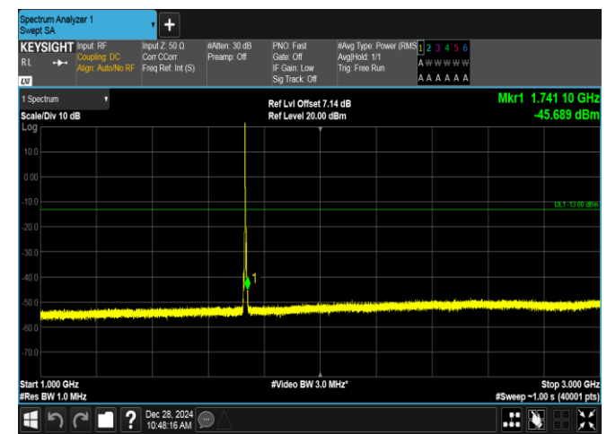
Band4-3MHz-16QAM-20175-1RB#0-1000~3000-PASS
