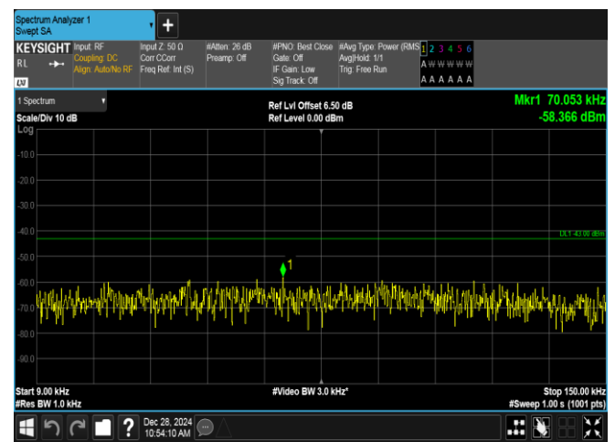
Band4-3MHz-16QAM-20385-1RB#0-0.009~0.15-PASS
