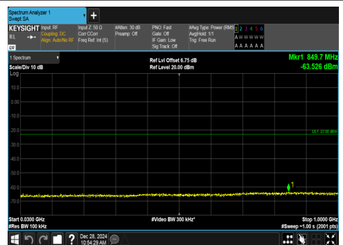
Band4-3MHz-16QAM-20385-1RB#0-30~1000-PASS
