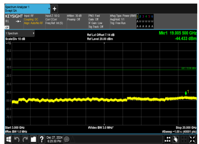
Band2-10MHz-QPSK-18650-1RB#49-3000~20000-PASS
