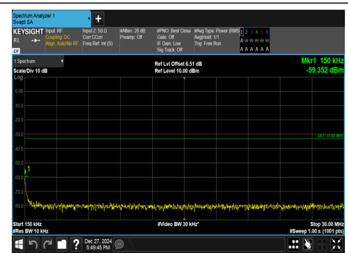
Band2-5MHz-QPSK-19175-1RB#0-0.15~30-PASS
