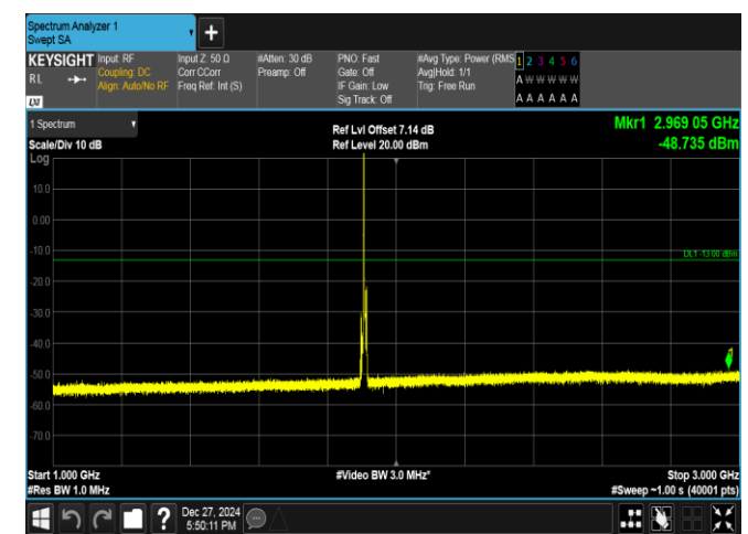
Band2-5MHz-QPSK-19175-1RB#0-1000~3000-PASS
