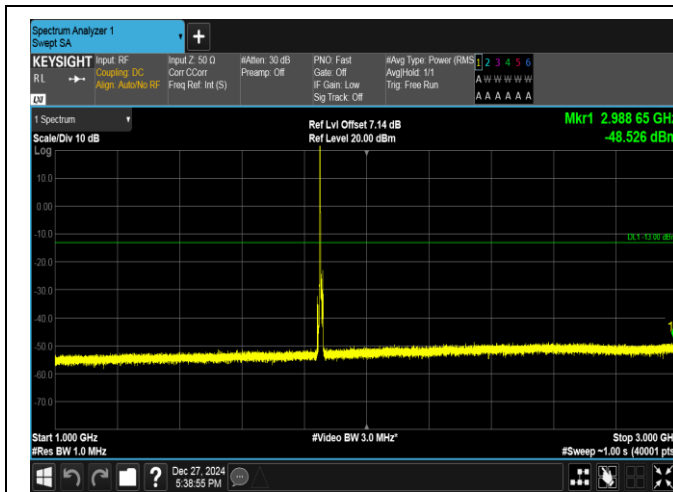
Band2-5MHz-16QAM-18625-1RB#0-1000~3000-PASS
