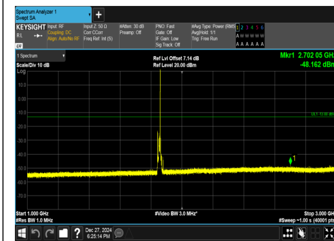
Band2-10MHz-QPSK-18650-1RB#49-1000~3000-PASS
