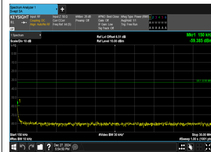
Band2-5MHz-16QAM-19175-25RB#0-0.15~30-PASS
