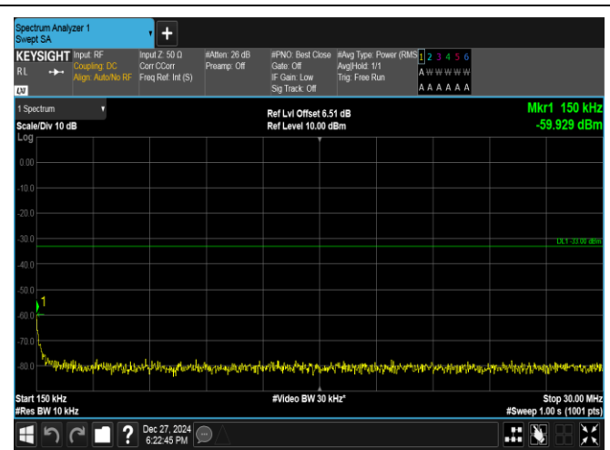
Band2-10MHz-QPSK-18650-1RB#0-0.15~30-PASS
