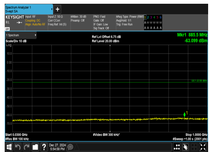
Band2-5MHz-16QAM-19175-25RB#0-30~1000-PASS
