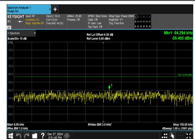
Band2-5MHz-QPSK-19175-1RB#24-0.009~0.15-PASS
